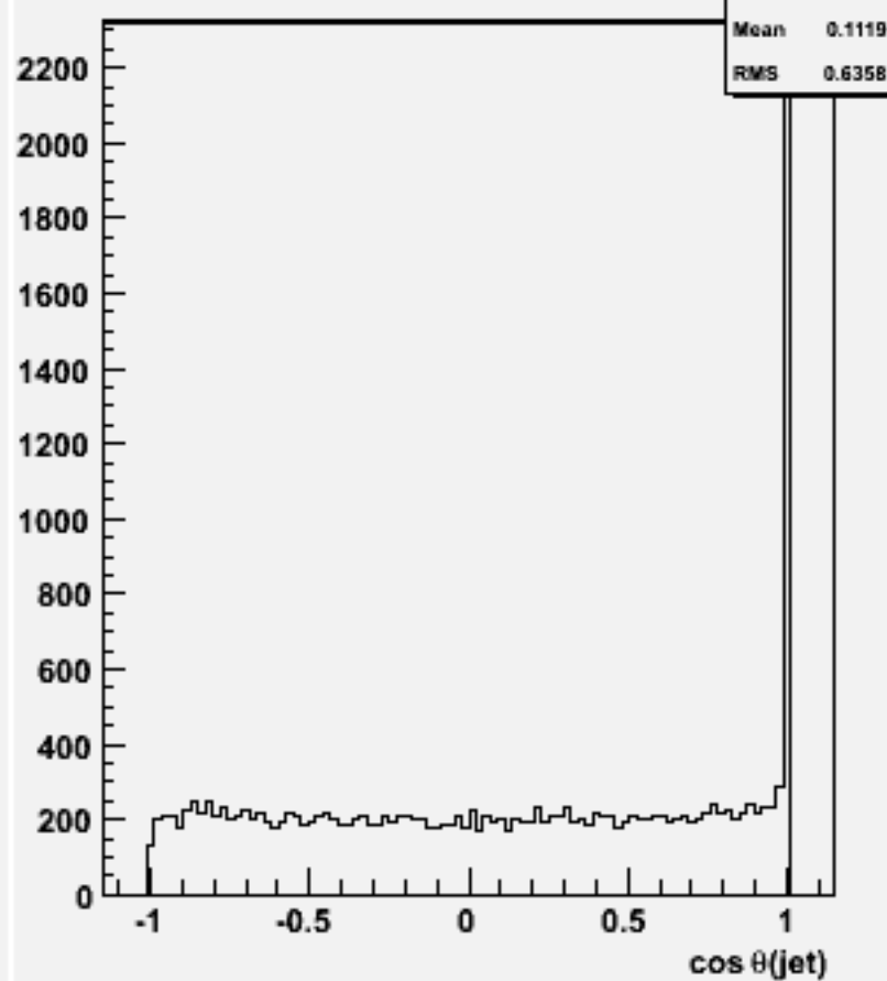
cos \theta for 2-jets :w101928 n1n1n2n2bb_o
