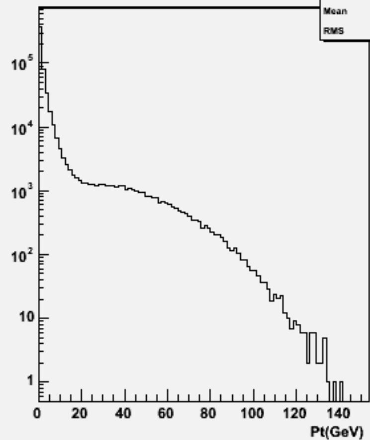
Particle Pt : w101928 n1n1n2n2bb_o
