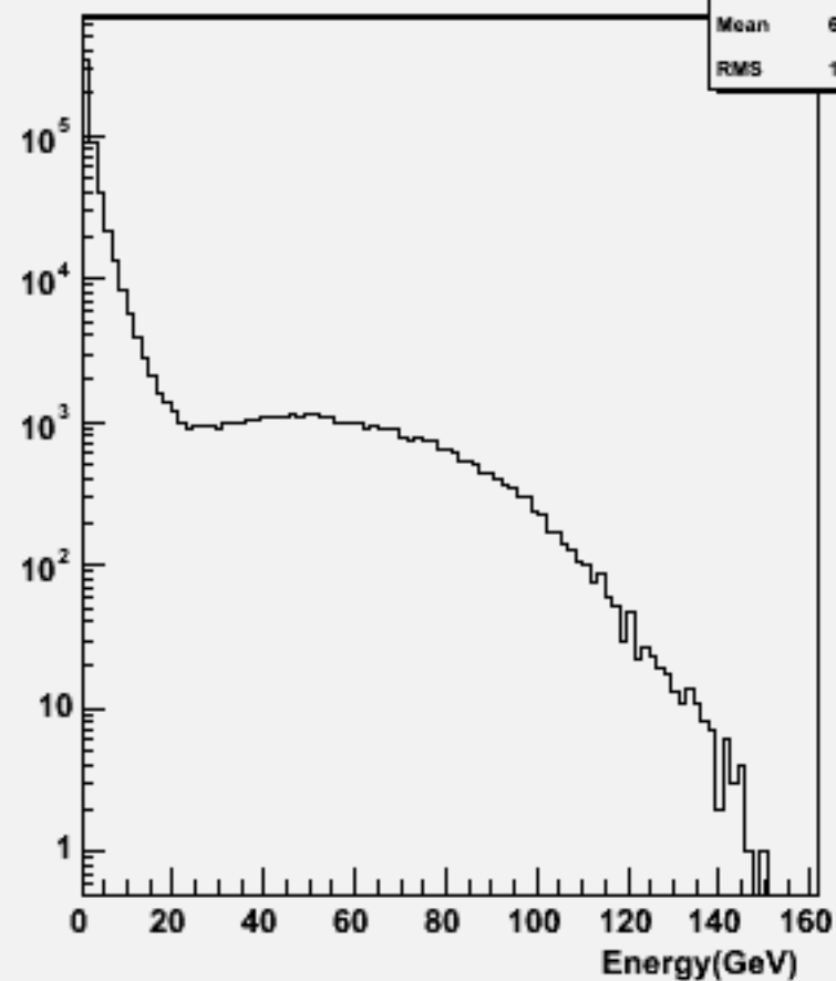
Particle Energy : w101928 n1n1n2n2bb_o
