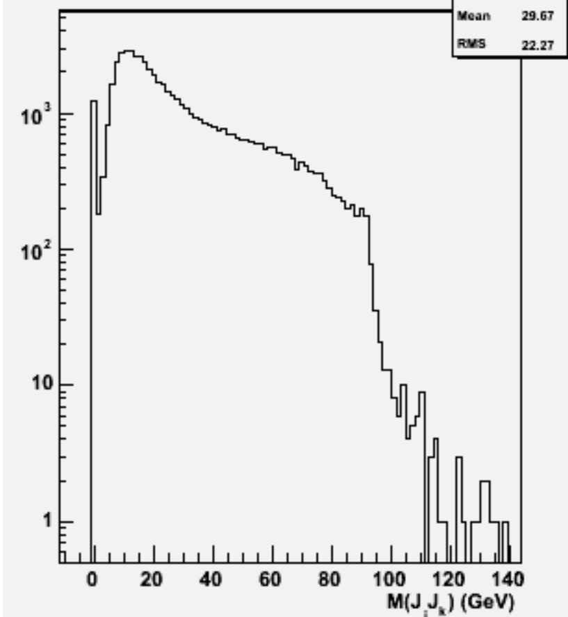
2jets mass(All comb)w101928 n1n1n2n2bb_o
