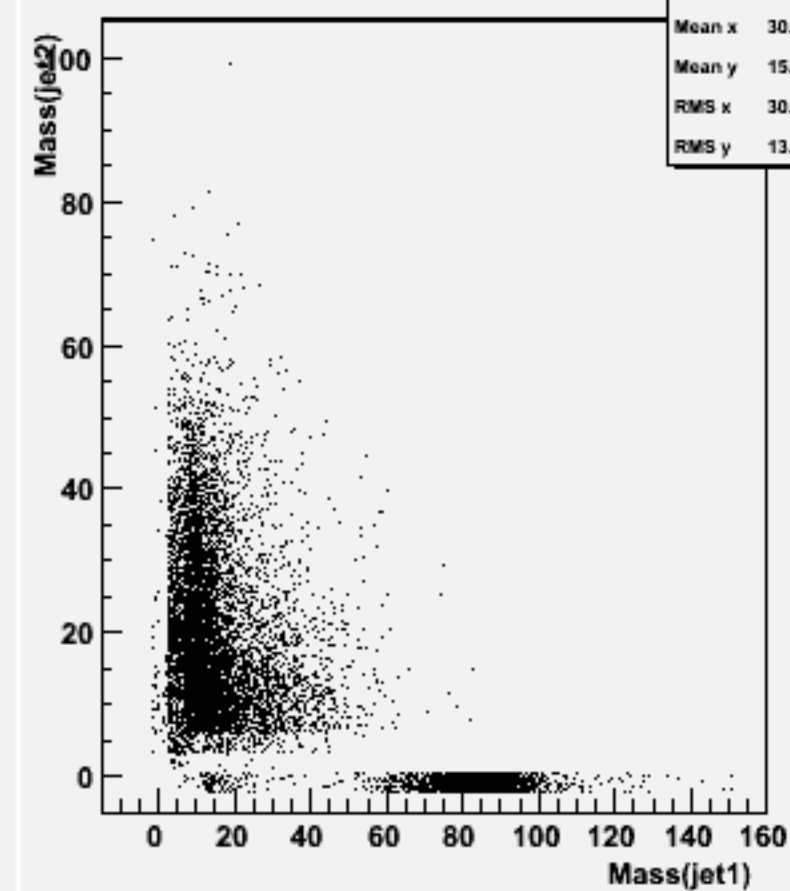
Jet mass for forced 2-jets : w101928 n1n1n2n2bb_o
