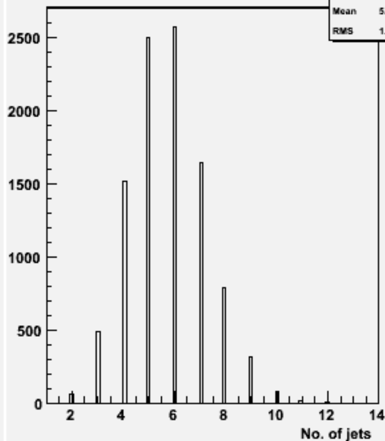
No. jets (ycut=0.001) : w101928 n1n1n2n2bb_o
