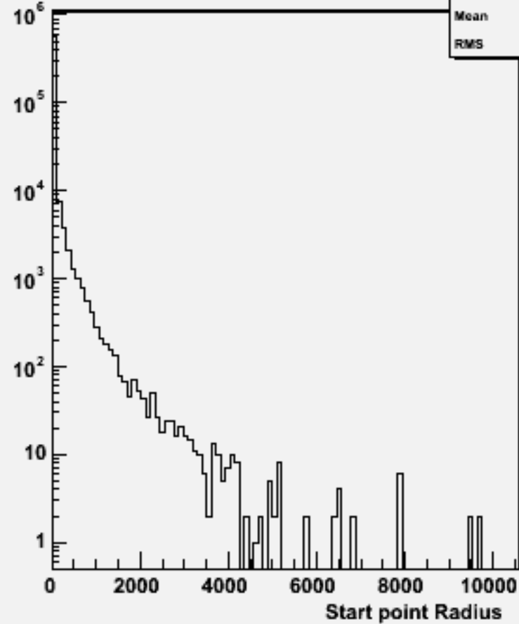
Start point R : w101928 n1n1n2n2bb_o
