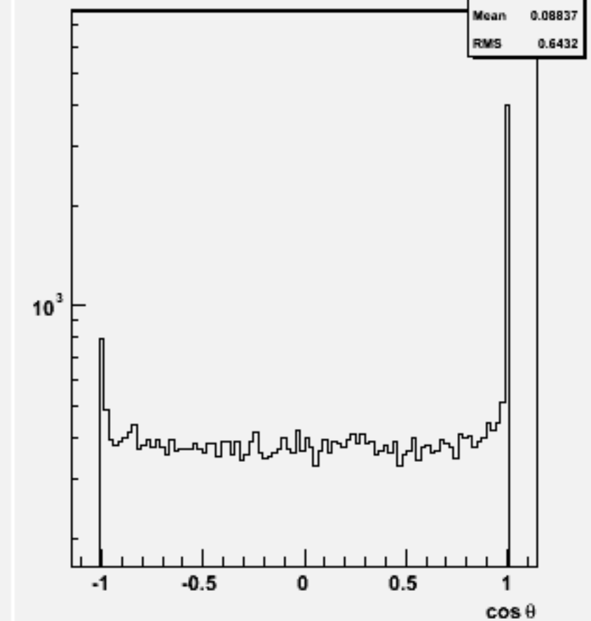
Jet cos \theta (All jets)w101928 n1n1n2n2bb_o
