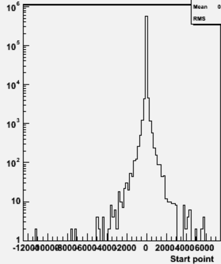
Start point Z : w101928 n1n1n2n2bb_o
