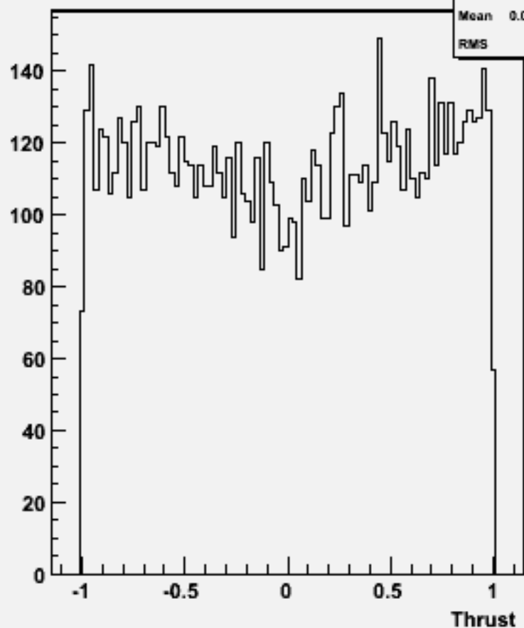
cos \Theta (thrust) w101928 n1n1n2n2bb_o
