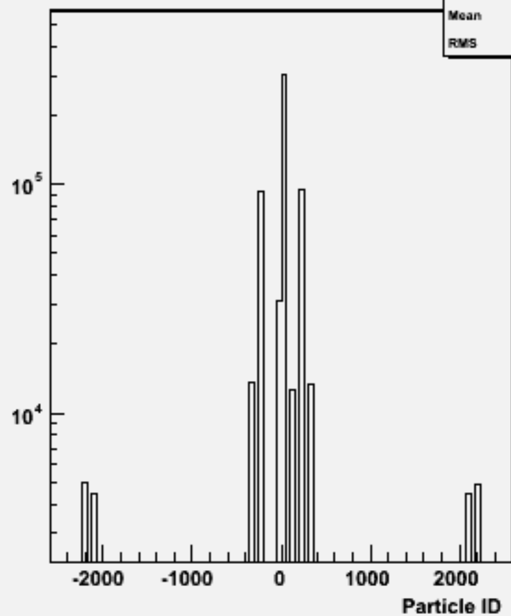
Particle ID : w101928 n1n1n2n2bb_o
