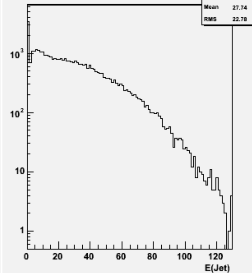
Jet energies(All jets)w101928 n1n1n2n2bb_o
