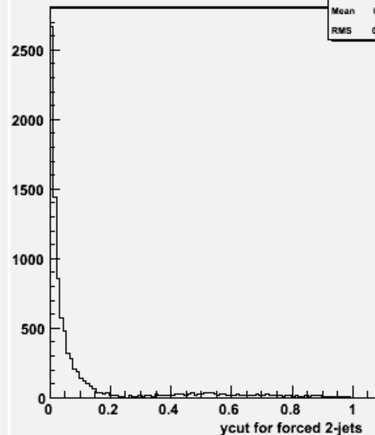
Ycut for 2-jets :w101928 n1n1n2n2bb_o
