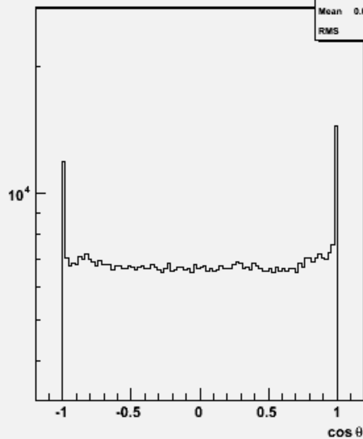
Particle cosθ : w101928 n1n1n2n2bb_o
