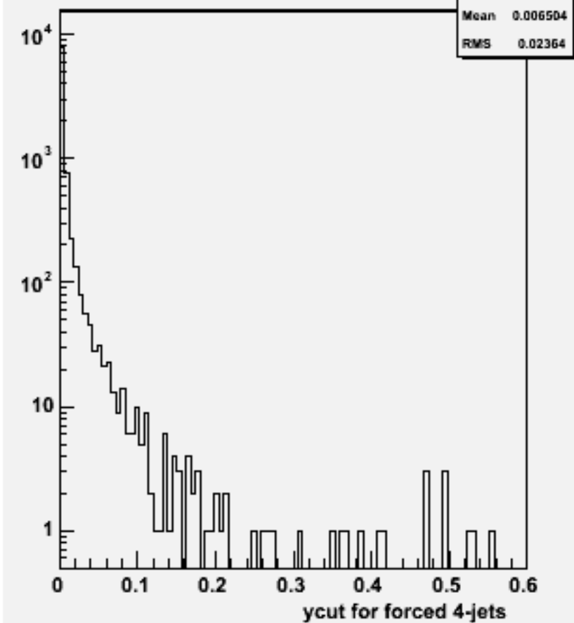
Ycut for 4-jets :w101928 n1n1n2n2bb_o
