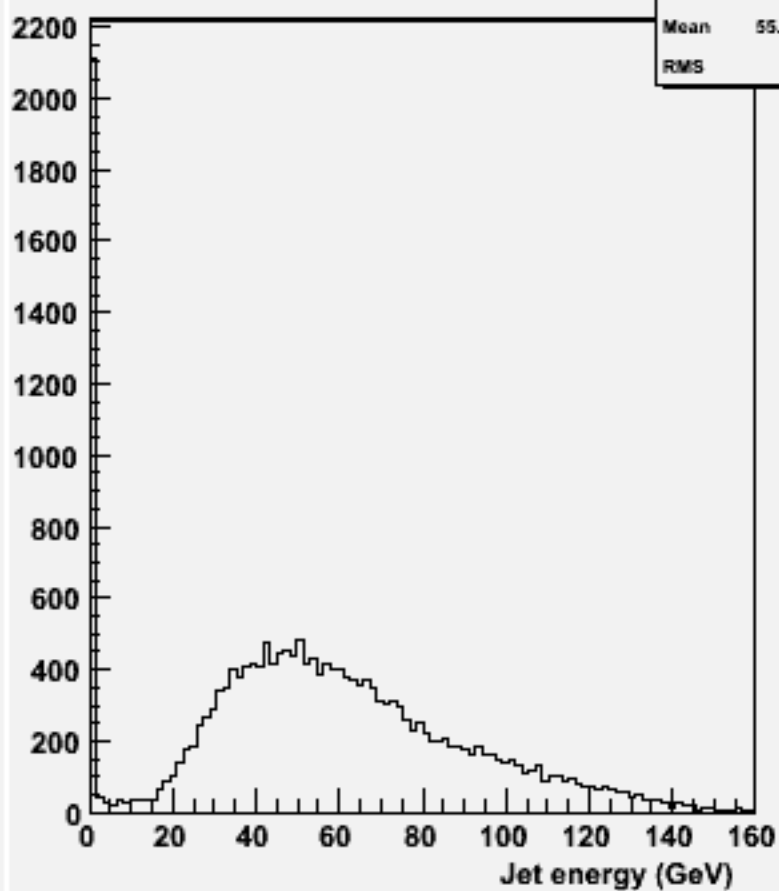
energy for 2-jets :w101928 n1n1n2n2bb_o
