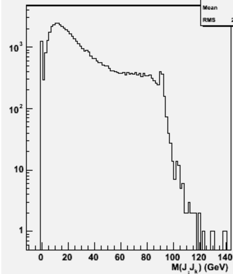
2jets mass(All comb)w101925 n1n1n2n2ss_o
