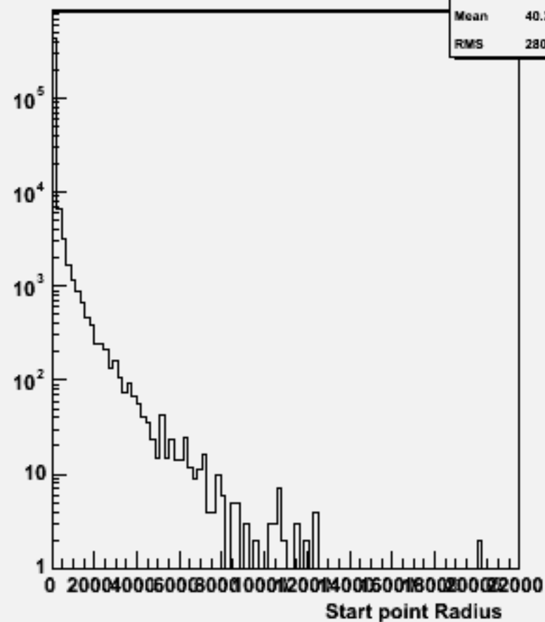
Start point R : w101925 n1n1n2n2ss_o
