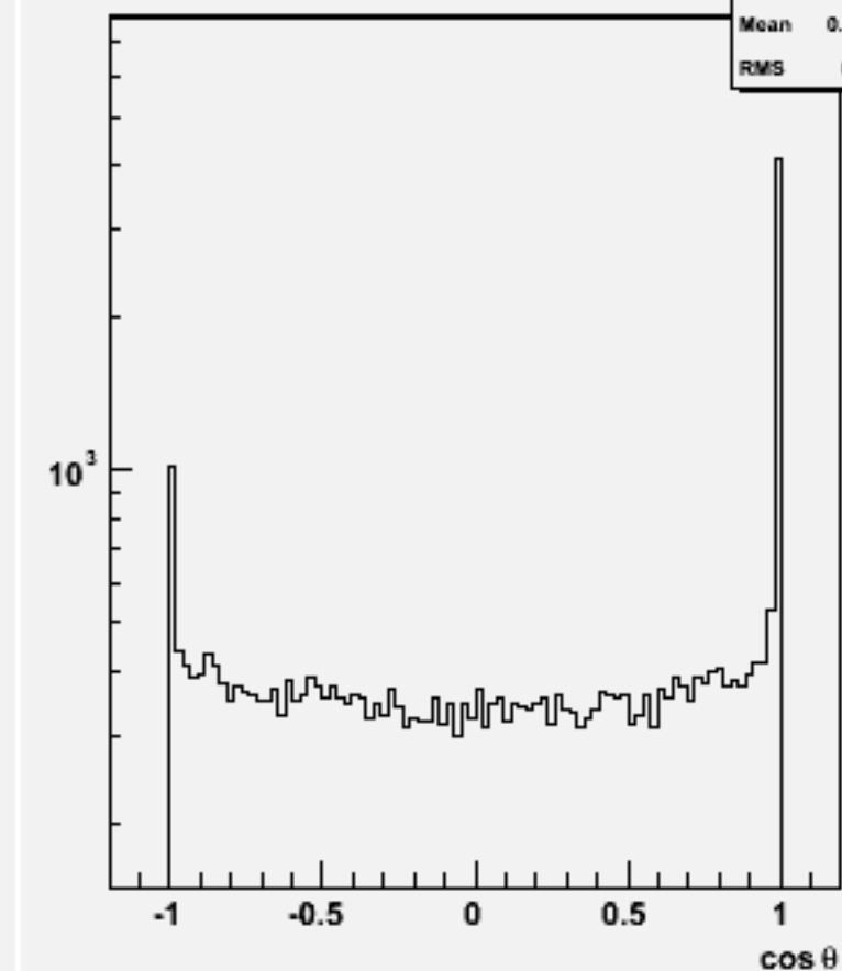
Jet cos \theta (All jets)w101925 n1n1n2n2ss_o
