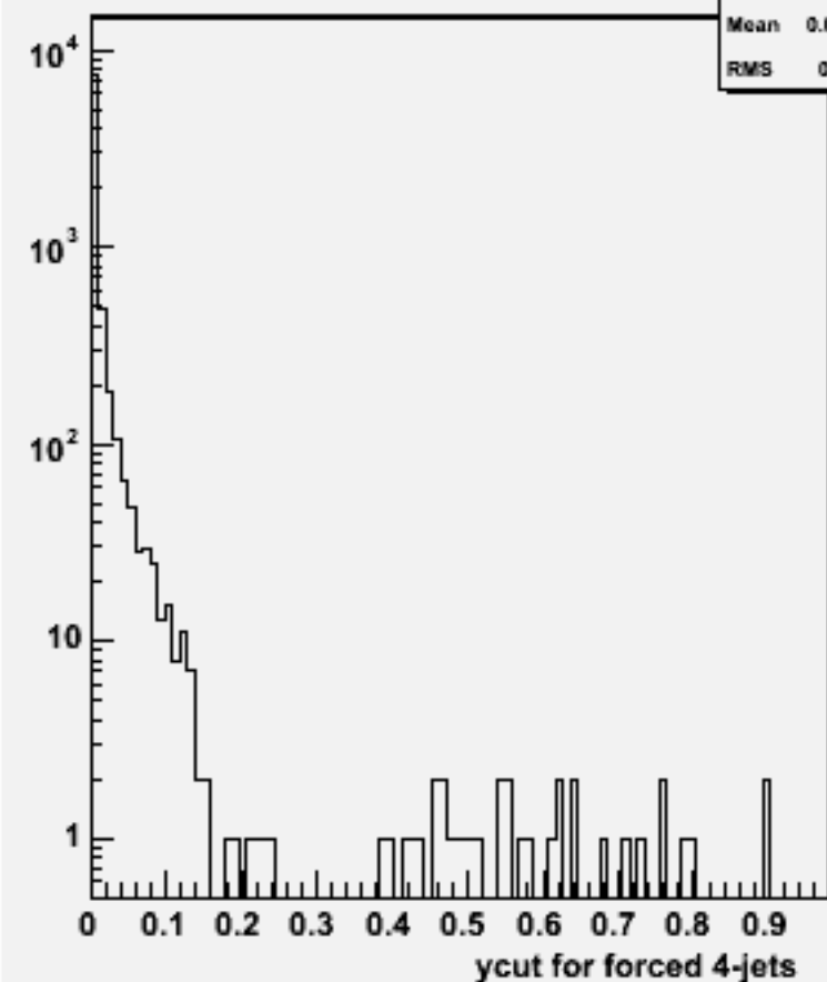
Ycut for 4-jets :w101925 n1n1n2n2ss_o
