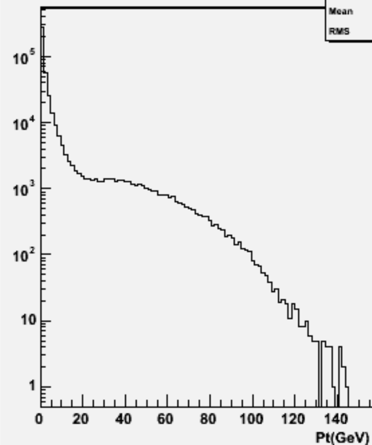
Start point Z : w101925 n1n1n2n2ss_o
