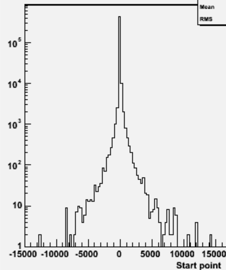
Start point Z : w101925 n1n1n2n2ss_o
