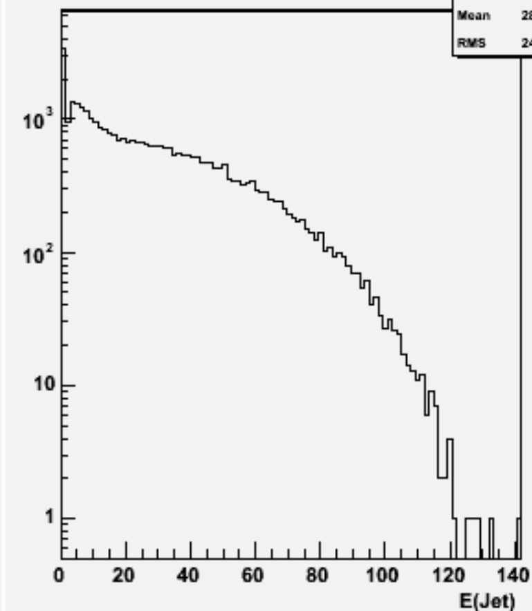
Jet energies(All jets)w101925 n1n1n2n2ss_o
