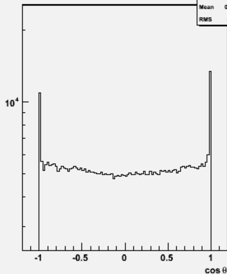
Particle cosθ : w101925 n1n1n2n2ss_o
