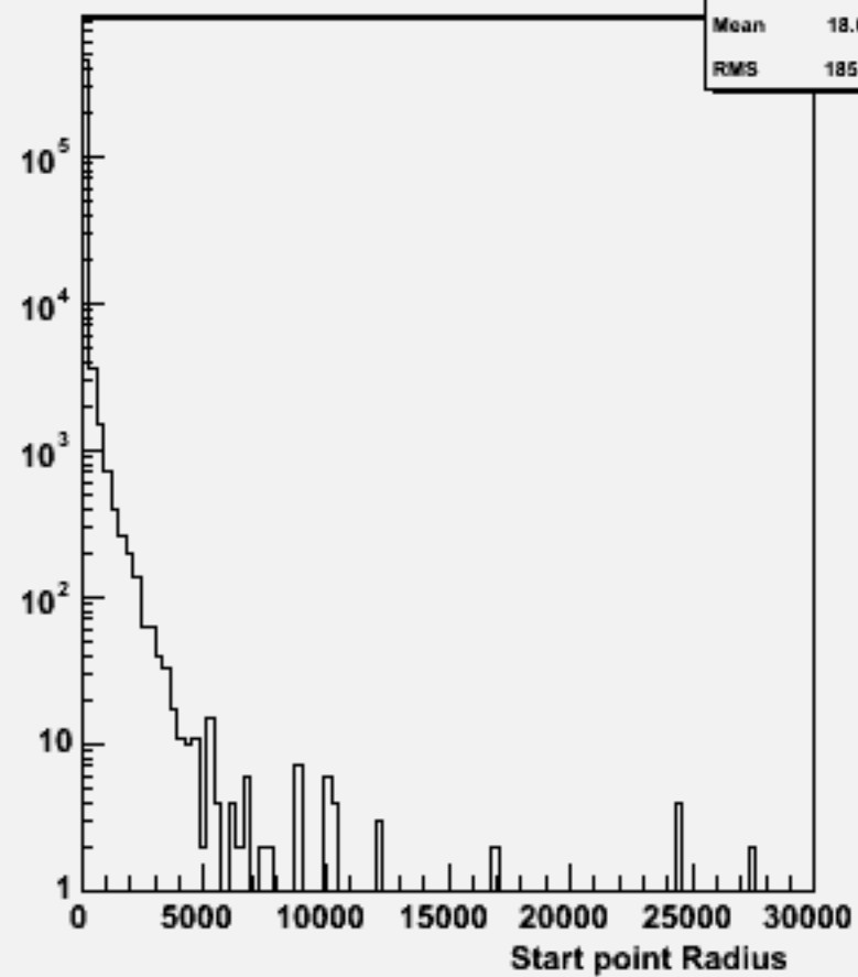
Start point R : w101921 n1n1n2n2dd_o
