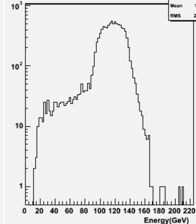
Thrust w101921 n1n1n2n2dd_o
