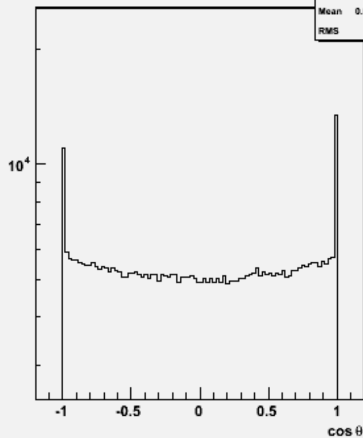
Particle cosθ : w101921 n1n1n2n2dd_o
