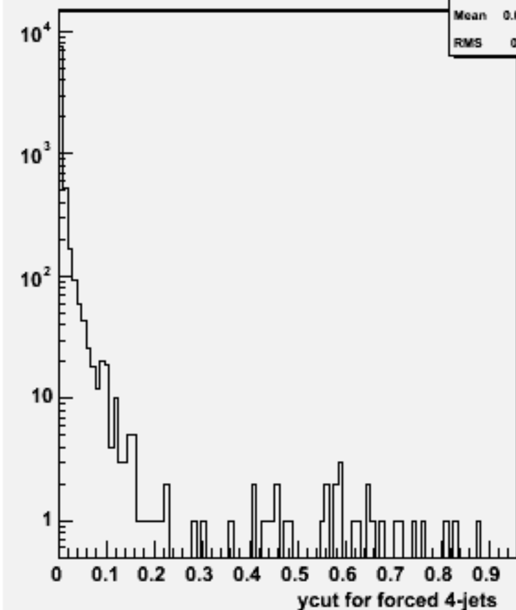
Ycut for 4-jets :w101921 n1n1n2n2dd_o
