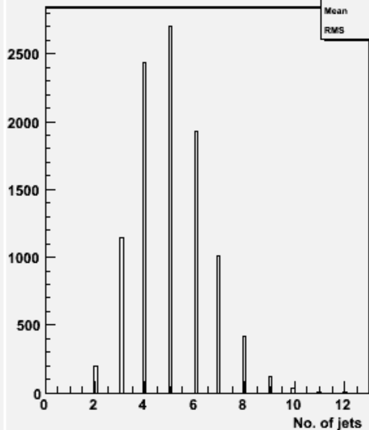
No. jets (ycut=0.001) : w101921 n1n1n2n2dd_o
