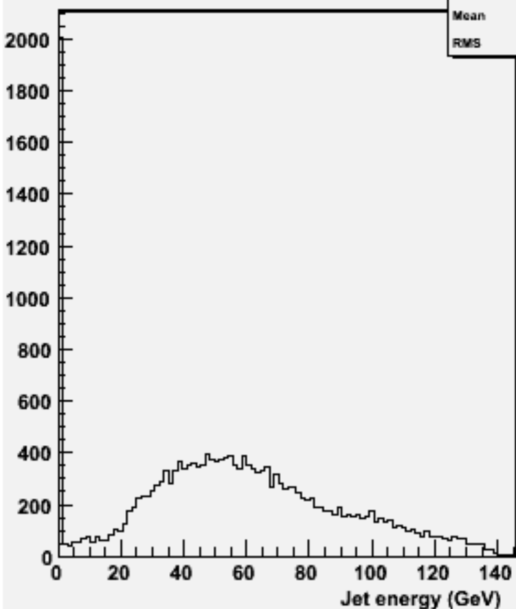
energy for 2-jets :w101921 n1n1n2n2dd_o
