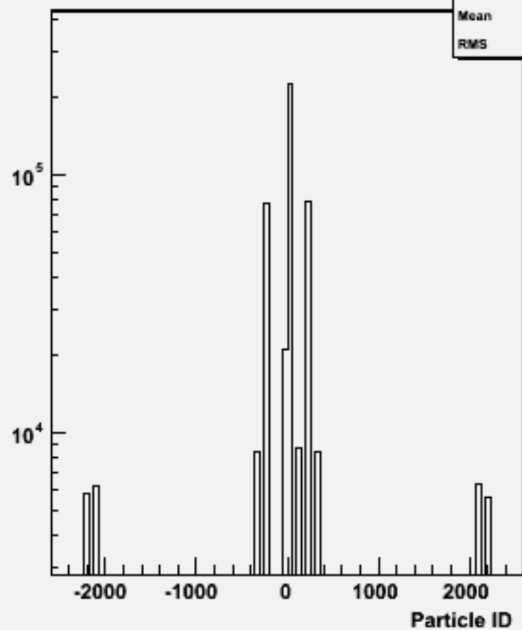
Particle ID : w101921 n1n1n2n2dd_o
