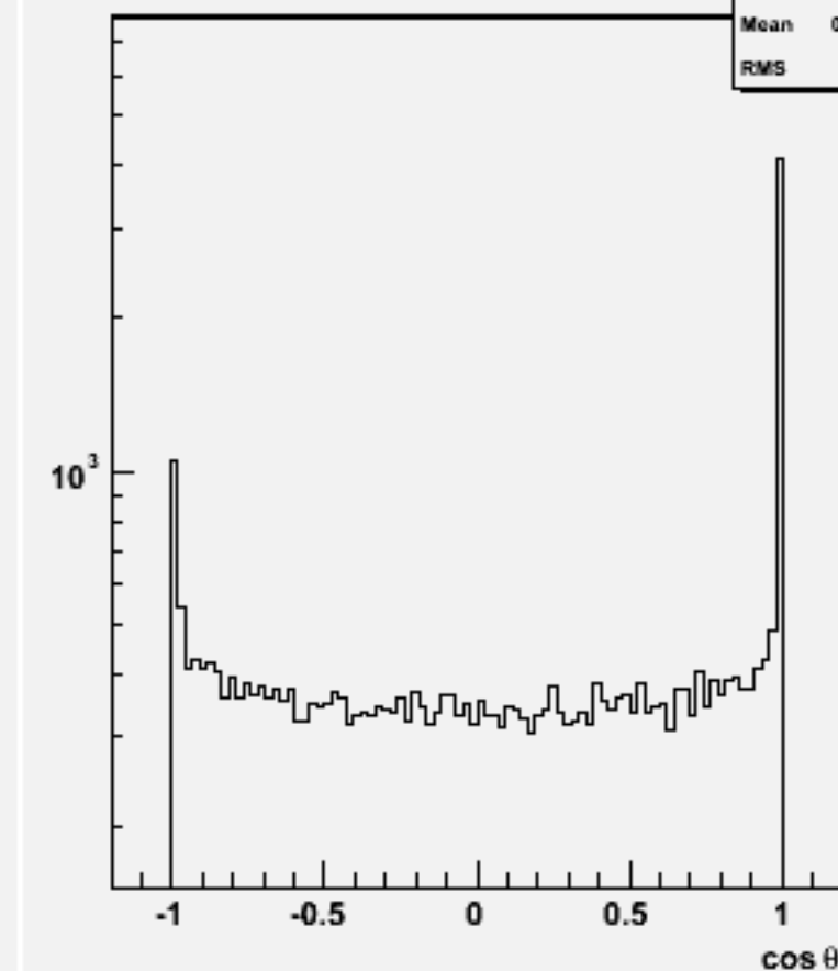
Jet cos \theta (All jets)w101921 n1n1n2n2dd_o
