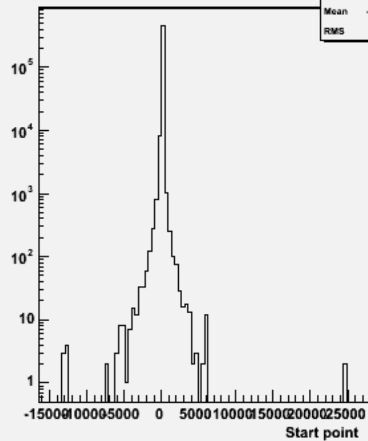
Start point Z : w101921 n1n1n2n2dd_o
