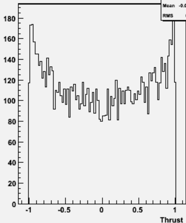
cos \Theta (thrust) w101921 n1n1n2n2dd_o
