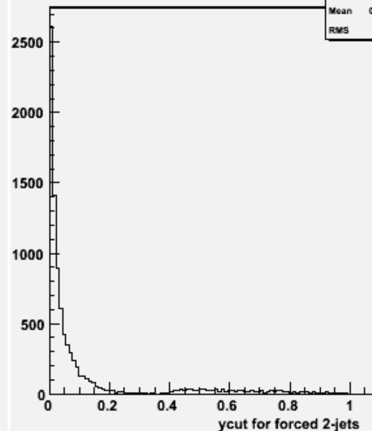
Ycut for 2-jets :w101921 n1n1n2n2dd_o
