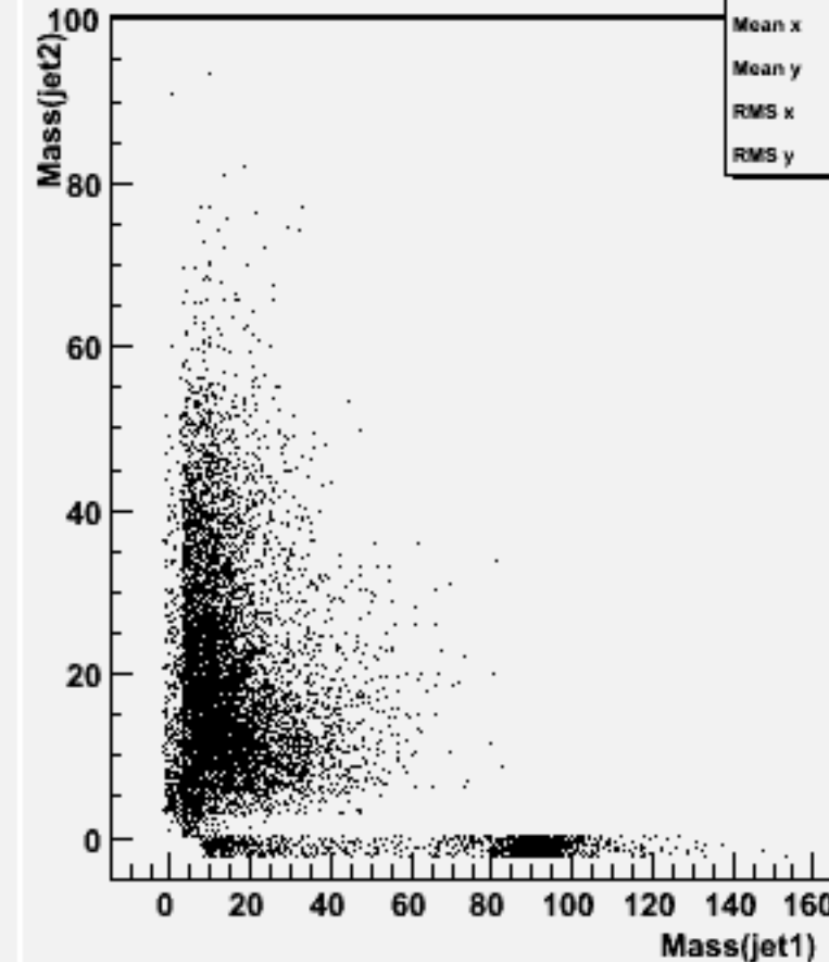
Jet mass for forced 2-jets : w101921 n1n1n2n2dd_o
