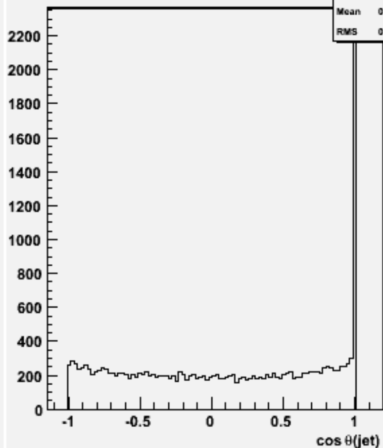
cos \theta for 2-jets :w101921 n1n1n2n2dd_o
