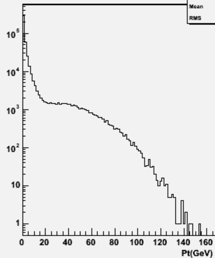
Particle Pt : w101921 n1n1n2n2dd_o
