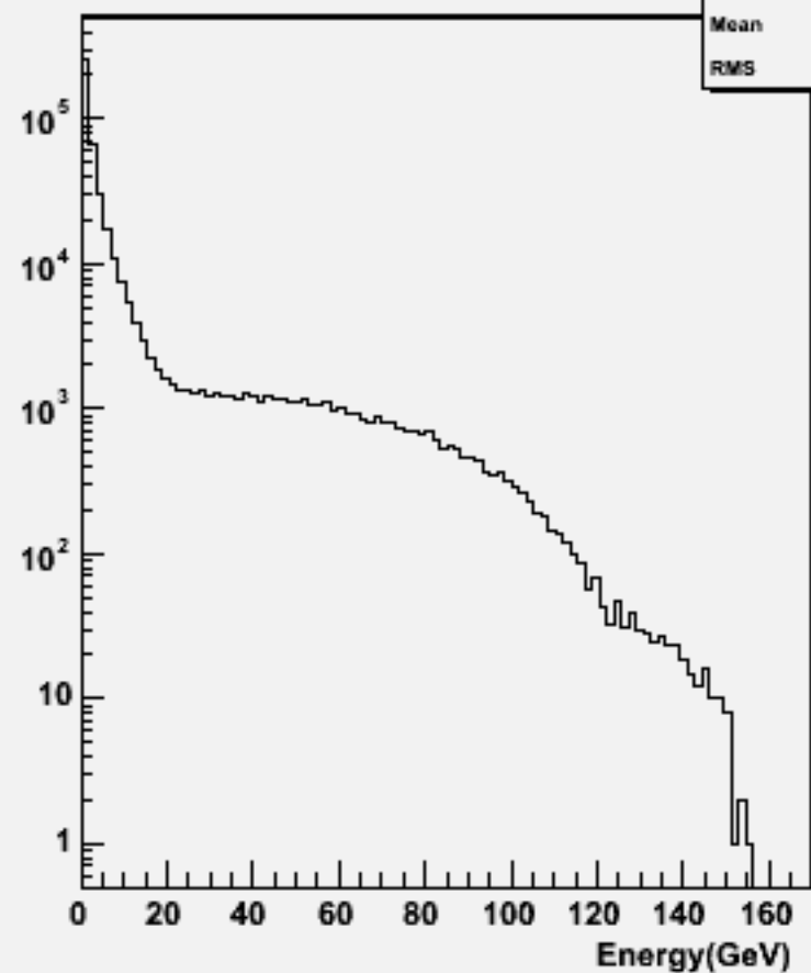
Particle Energy : w101921 n1n1n2n2dd_o
