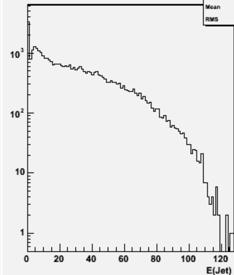
Jet energies(All jets)w101921 n1n1n2n2dd_o
