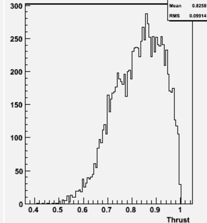
Thrust w101921 n1n1n2n2dd_o
