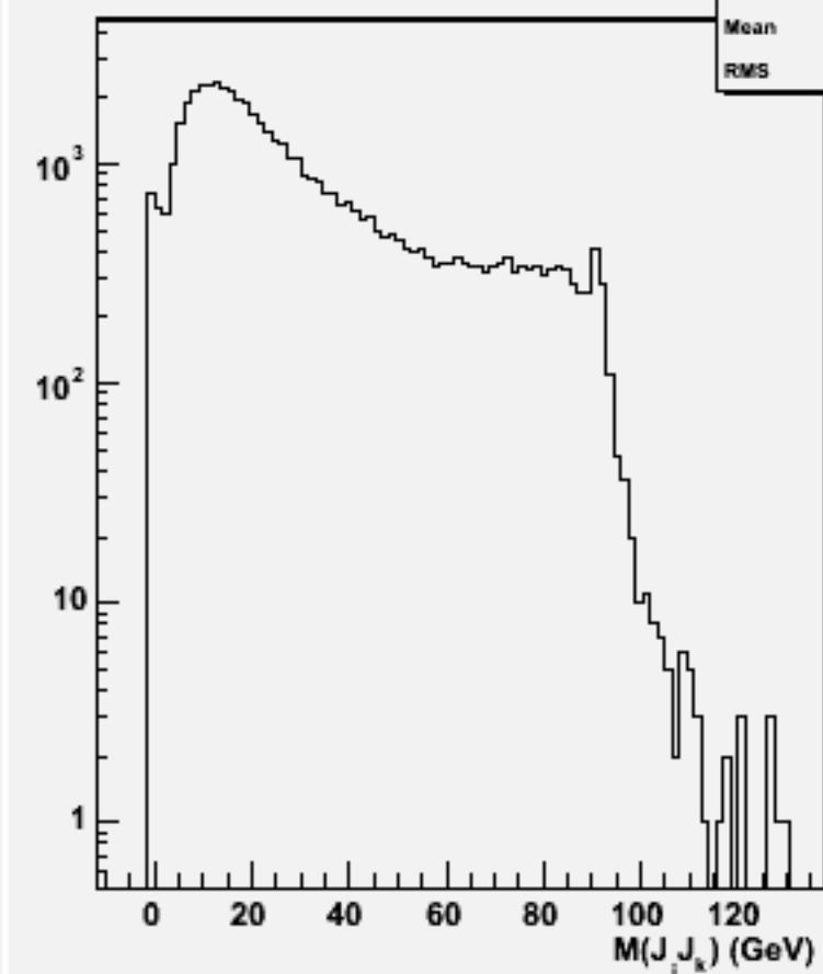
2jets mass(All comb)w101921 n1n1n2n2dd_o
