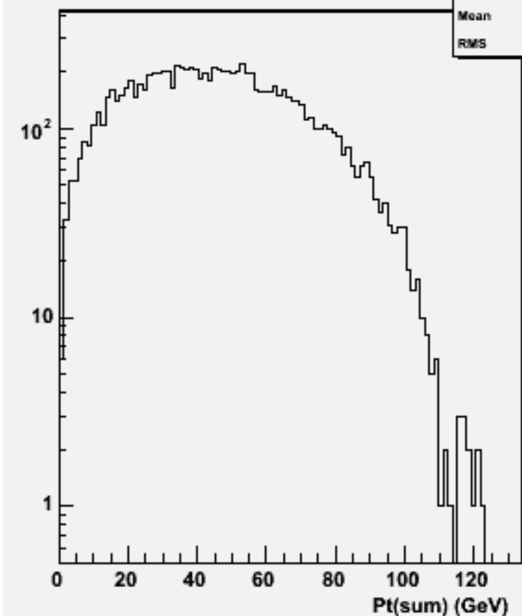
Pt Sum: w101921 n1n1n2n2dd_o
