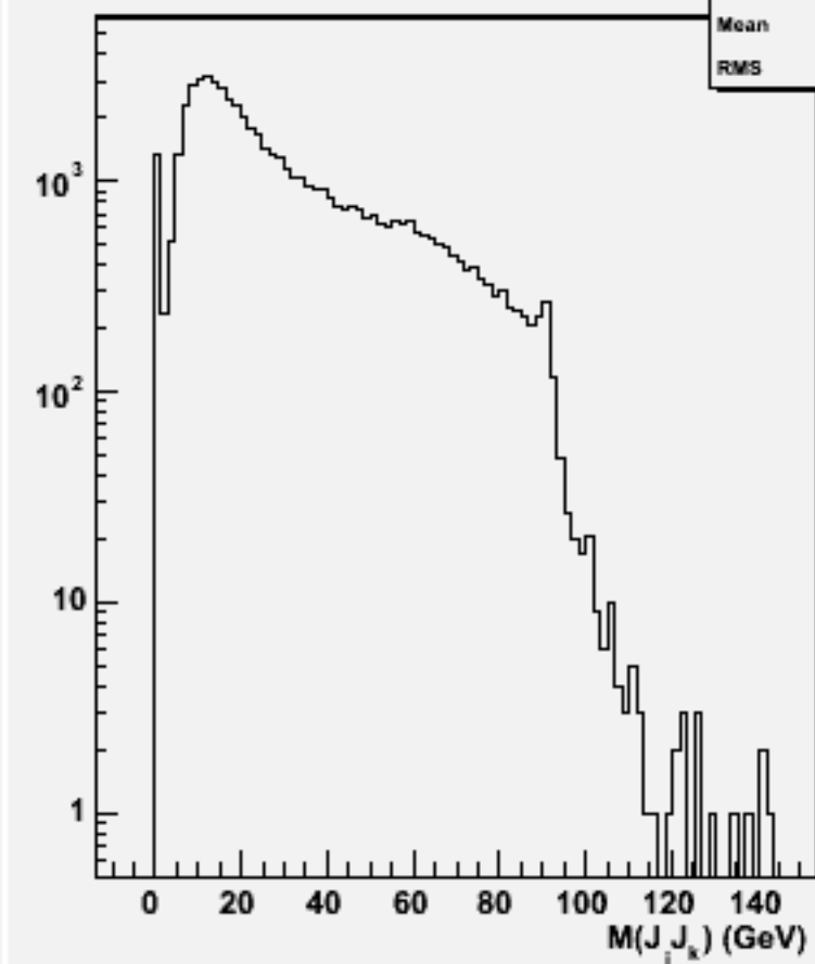
2jets mass(All comb)w101912 n1n1n1n1bb_o
