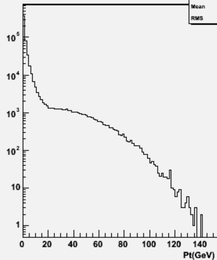
Particle Pt : w101912 n1n1n1n1bb_o
