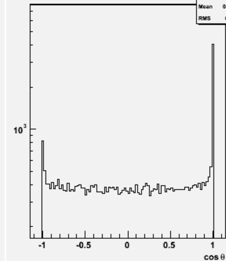
Jet cos \theta (All jets)w101912 n1n1n1n1bb_o
