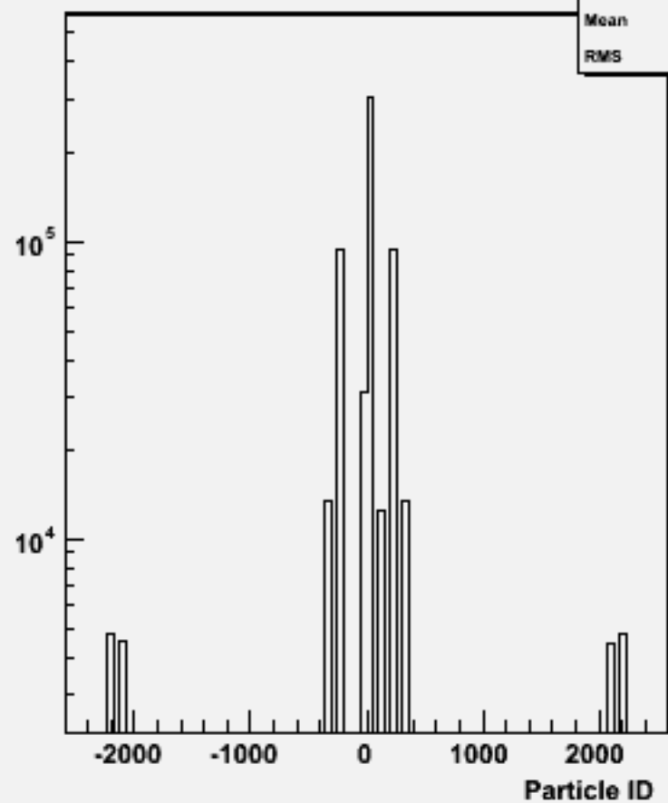
Particle ID : w101912 n1n1n1n1bb_o
