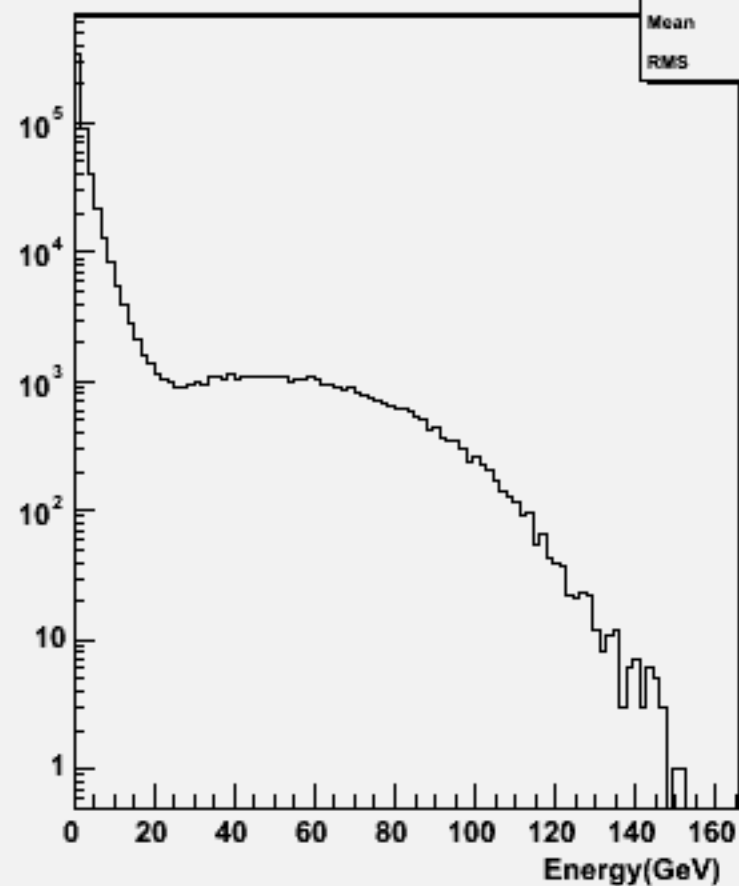
Particle Energy : w101912 n1n1n1n1bb_o
