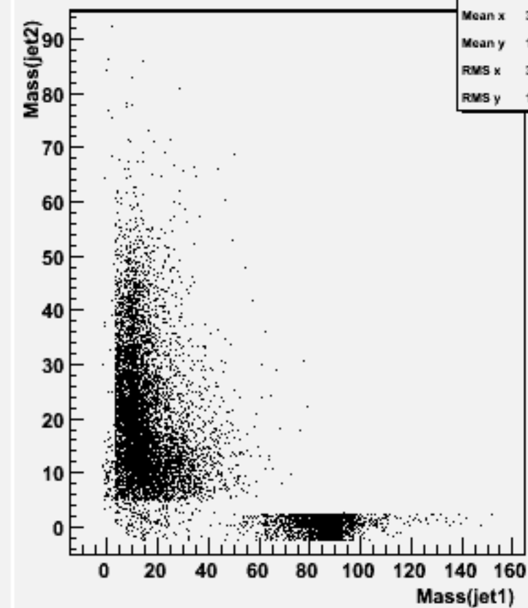
Jet mass for forced 2-jets : w101912 n1n1n1n1bb_o
