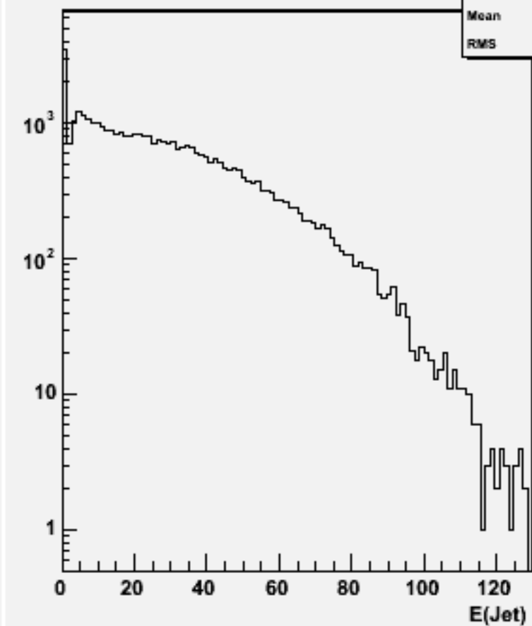
Jet energies(All jets)w101912 n1n1n1n1bb_o
