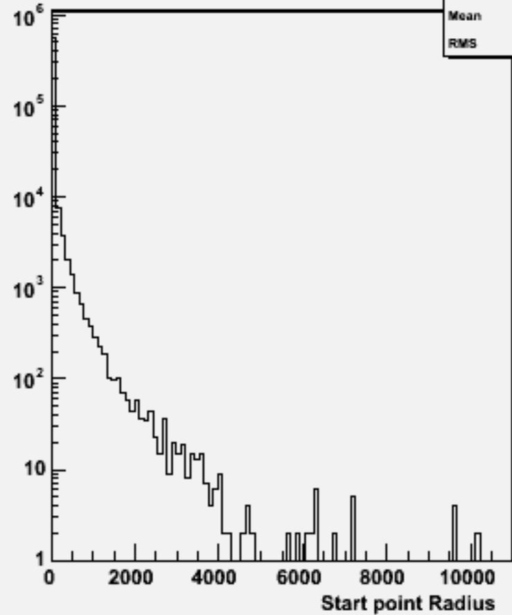
Start point R : w101912 n1n1n1n1bb_o
