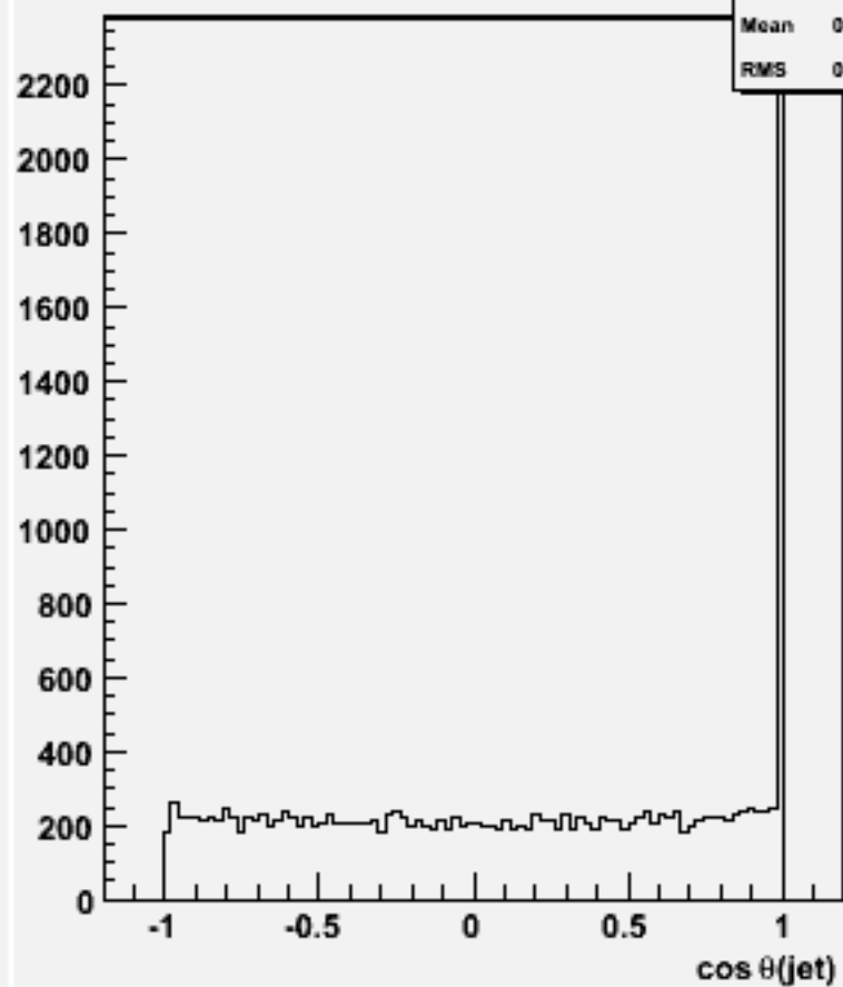
cos \theta for 2-jets :w101912 n1n1n1n1bb_o
