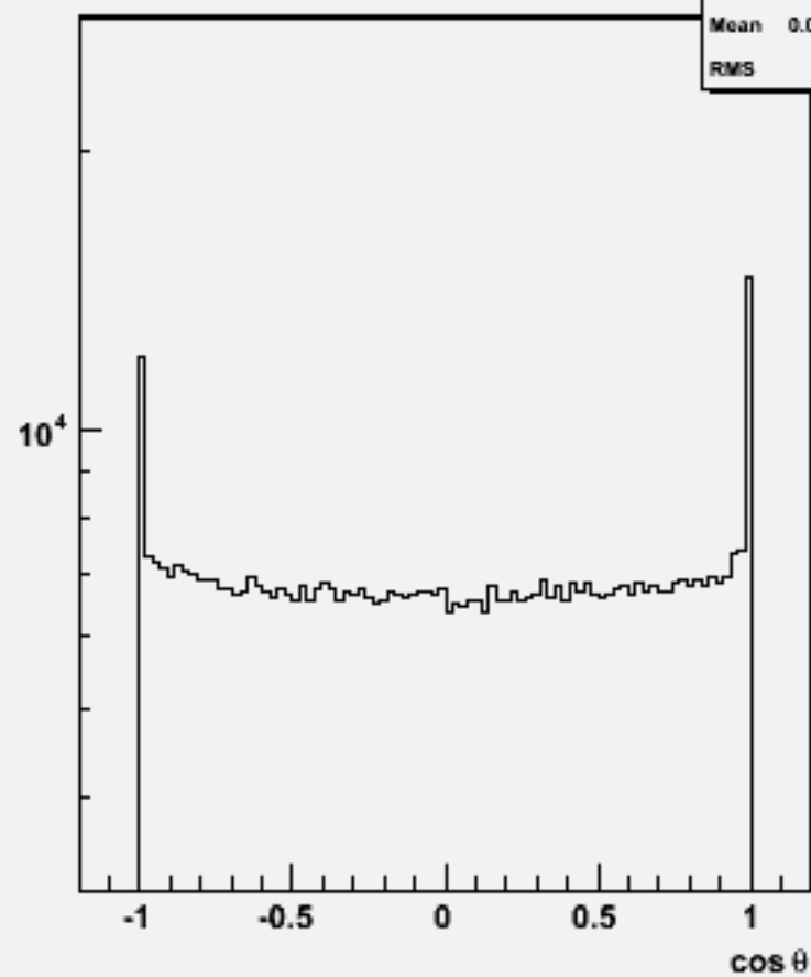
Particle cosθ : w101912 n1n1n1n1bb_o
