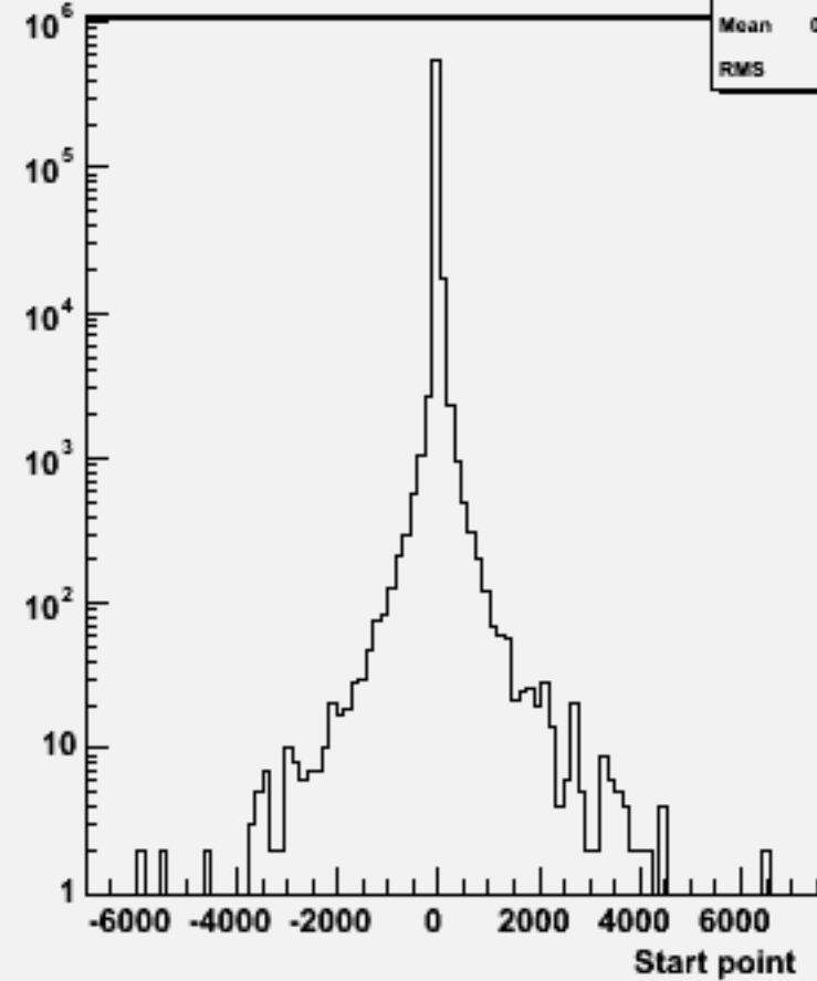
Start point Z : w101912 n1n1n1n1bb_o
