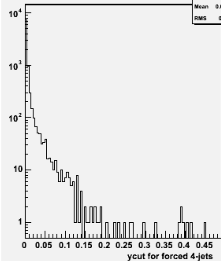
Ycut for 4-jets :w101912 n1n1n1n1bb_o
