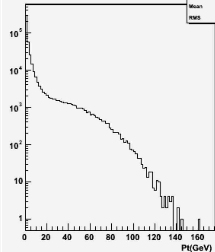
Particle Pt : w101908 n1n1n1n1ss_o
