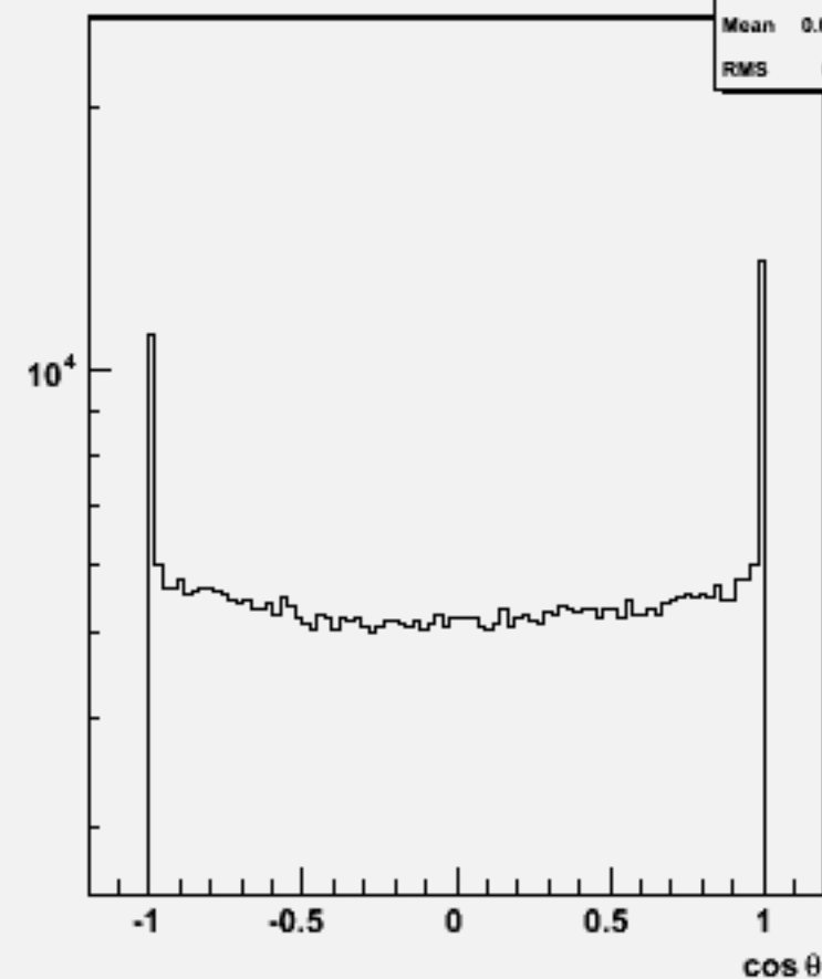
Particle cos \theta : w101908 n1n1n1n1ss_o
