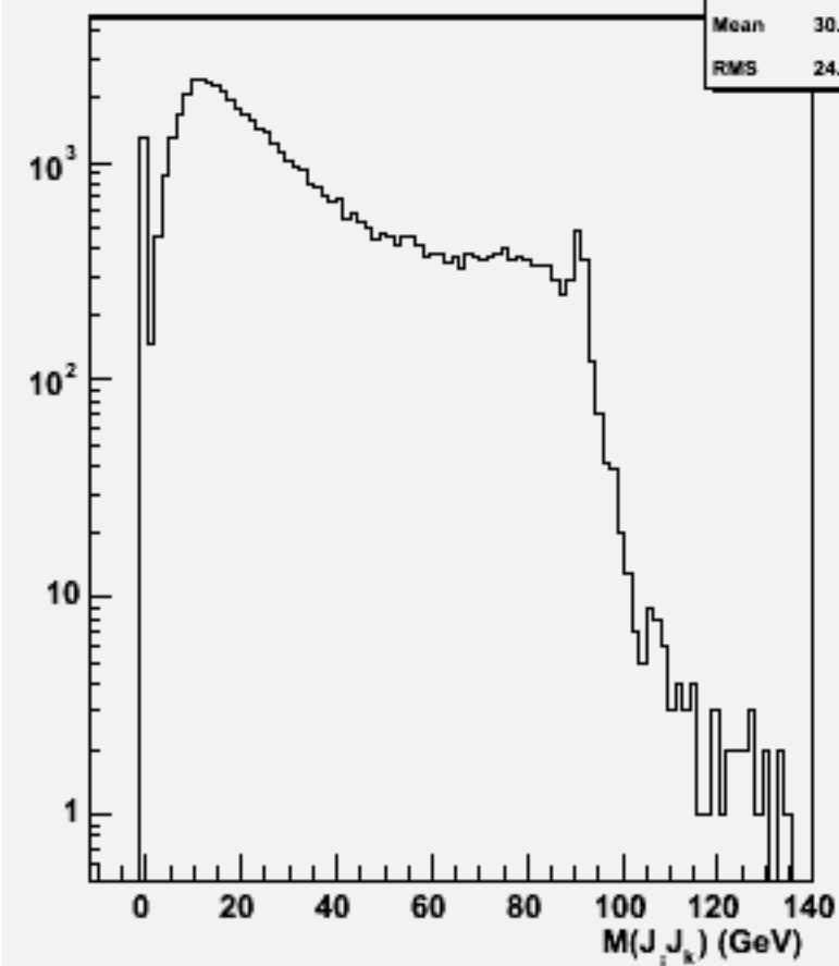
2jets mass(All comb)w101908 n1n1n1n1ss_o
