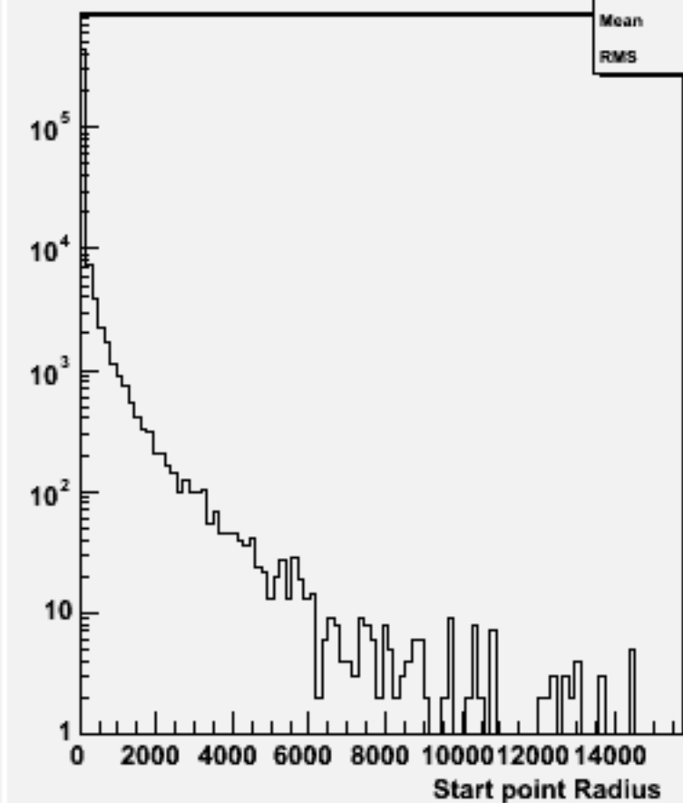
Start point R : w101908 n1n1n1n1ss_o
