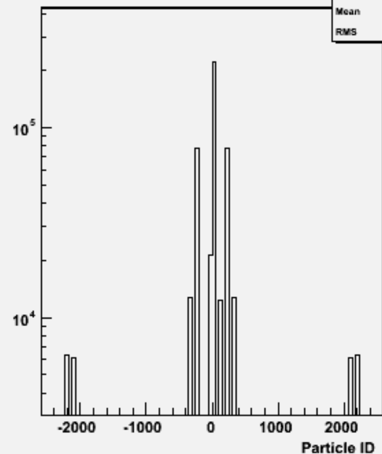
Particle ID : w101908 n1n1n1n1ss_o
