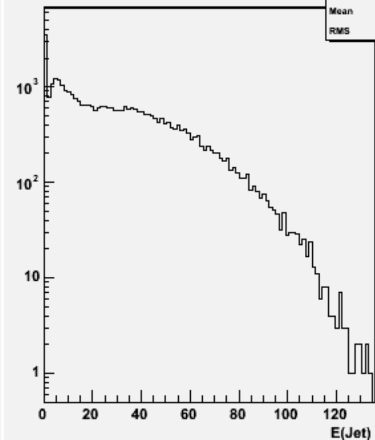
Jet energies(All jets)w101908 n1n1n1n1ss_o
