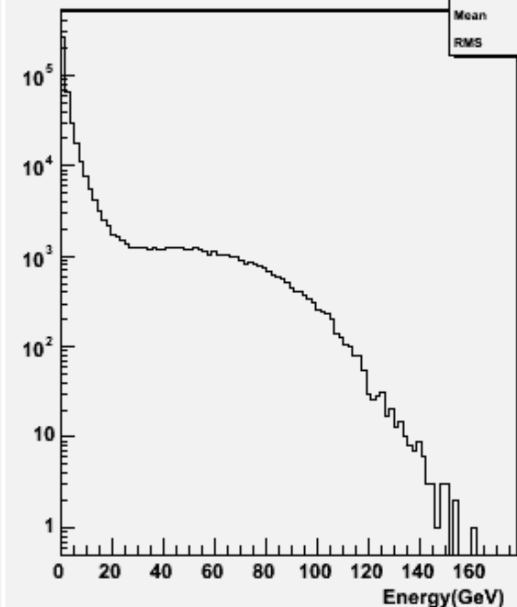
Particle Energy : w101908 n1n1n1n1ss_o
