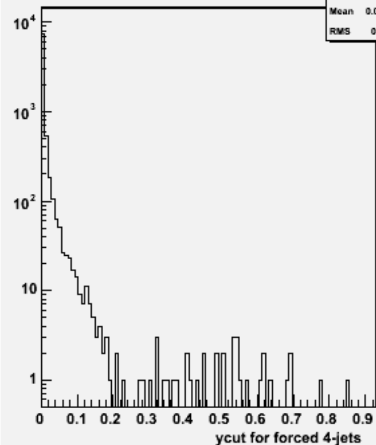
Ycut for 4-jets :w101908 n1n1n1n1ss_o
