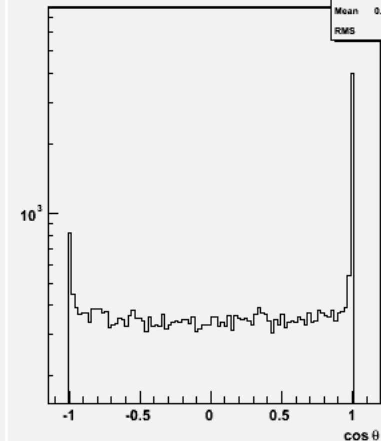
Jet cos \theta (All jets)w101908 n1n1n1n1ss_o
