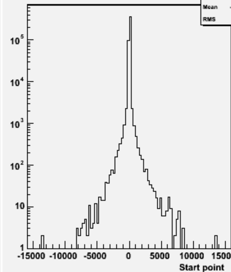
Start point Z : w101908 n1n1n1n1ss_o
