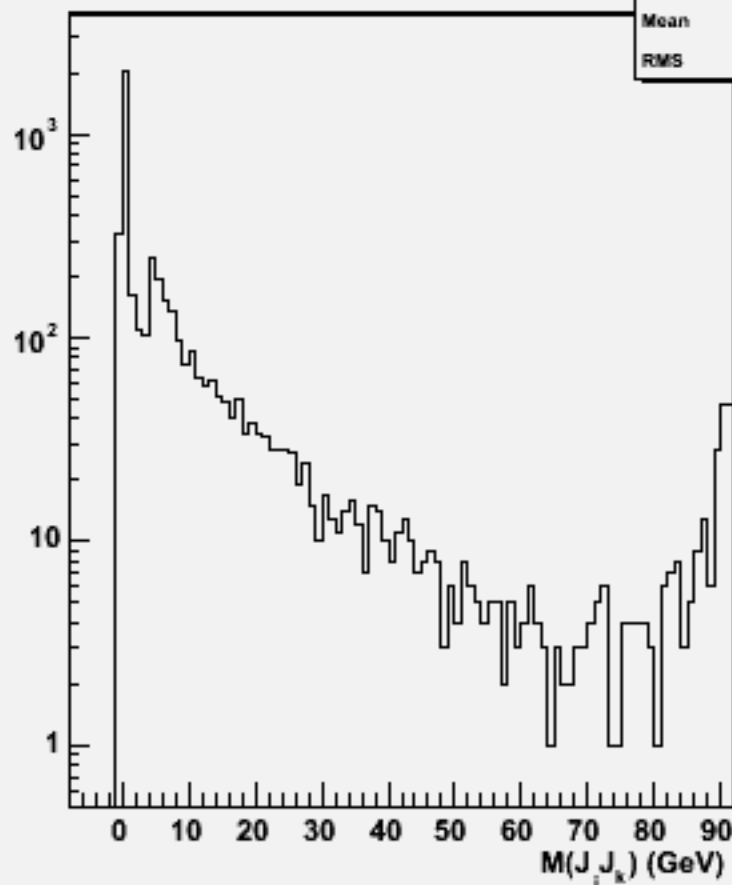
2jets mass(All comb)w101896 n1n1n1n1e2e2_o
