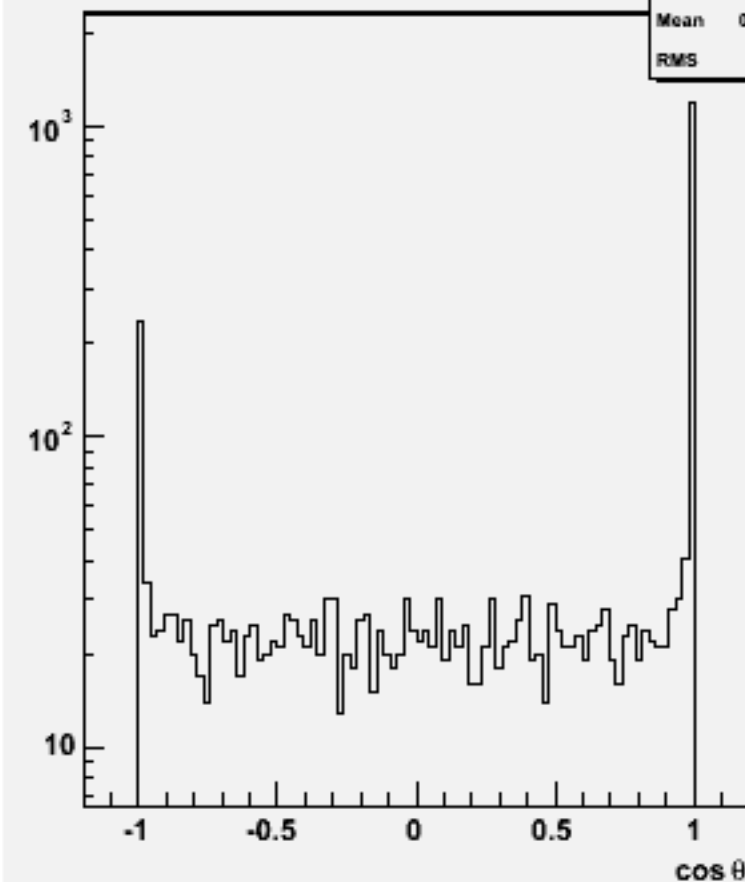
Jet cos \theta (All jets)w101896 n1n1n1n1e2e2_o
