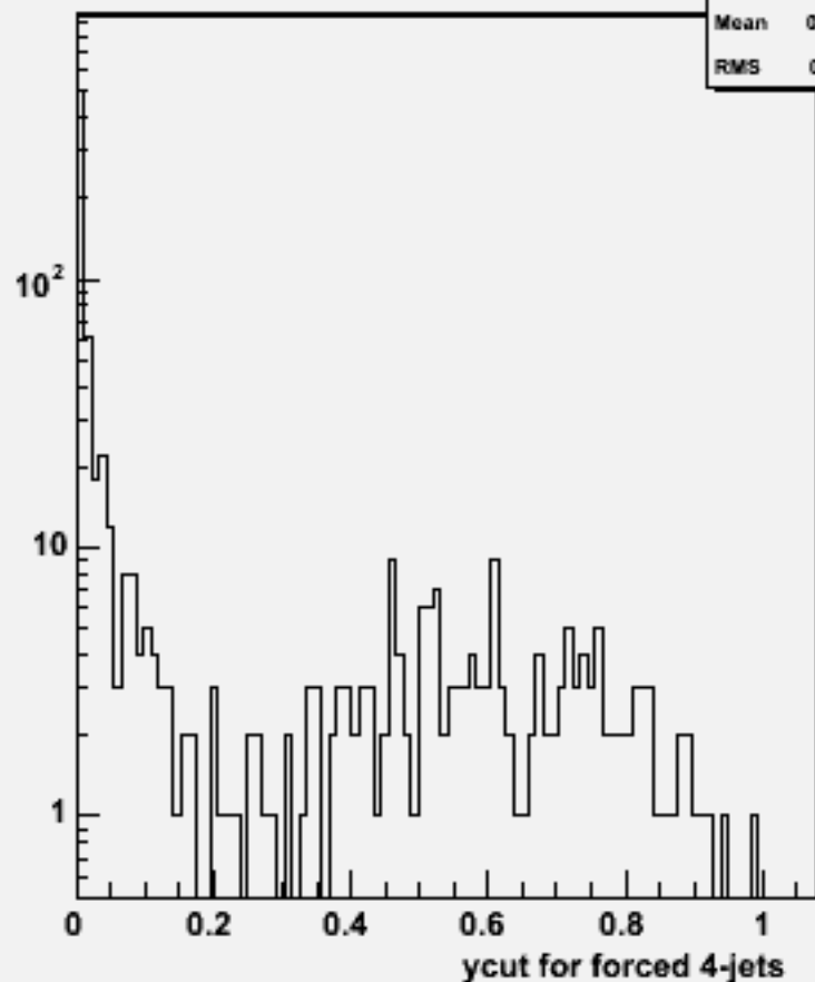
Ycut for 4-jets :w101896 n1n1n1n1e2e2_o
