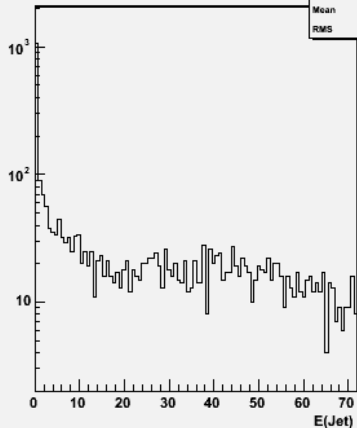
Jet energies(All jets)w101896 n1n1n1n1e2e2_o
