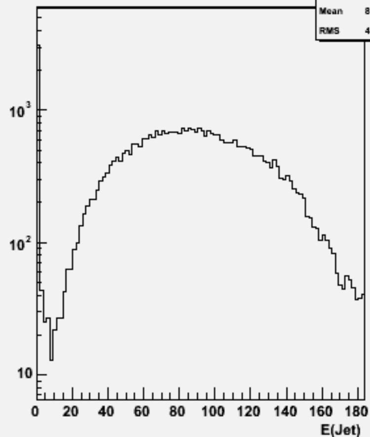
Jet energies(All jets)w101893 ccccc_o
