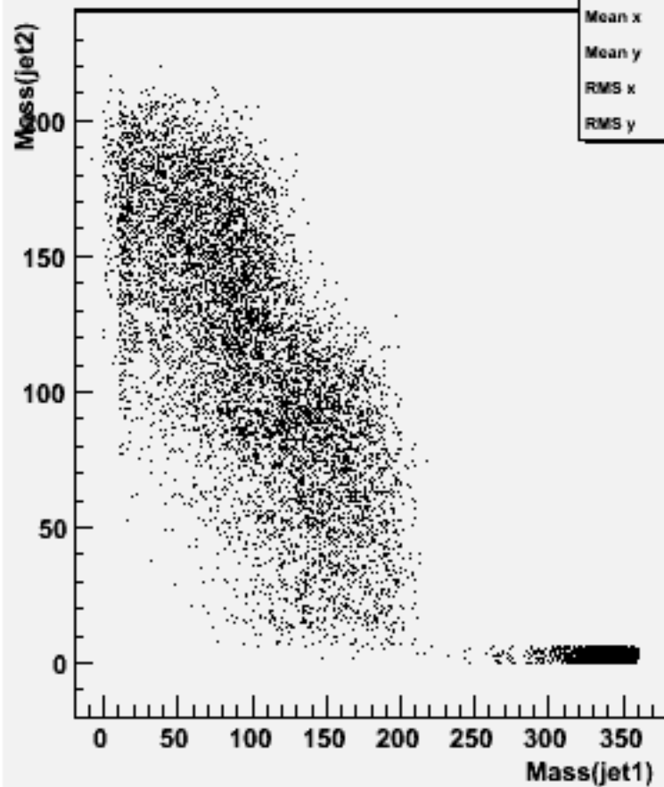
Jet mass for forced 2-jets : w101893 ccccc_o
