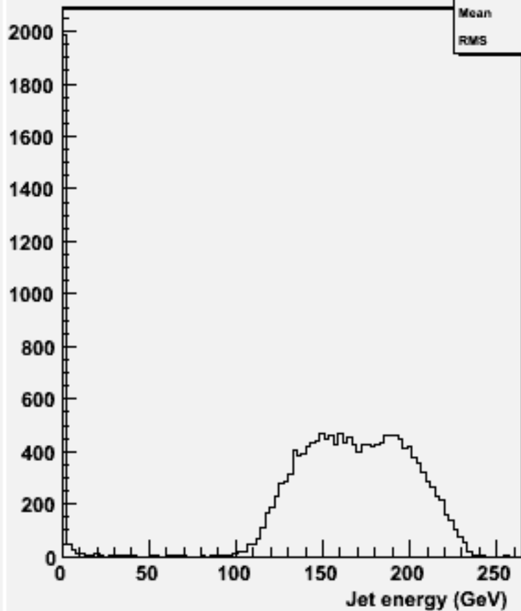
energy for 2-jets :w101893 ccccc_o
