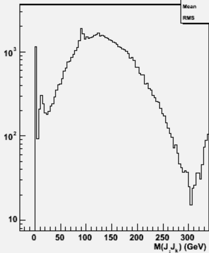
2jets mass(All comb)w101893 ccccc_o
