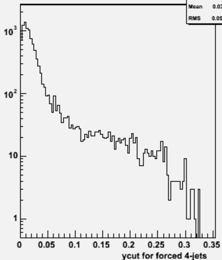
Ycut for 4-jets :w101893 ccccc_o
