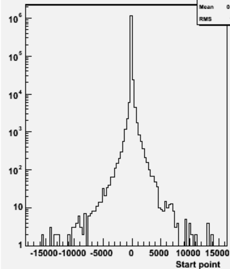
Start point Z : w101893 ccccc_o
