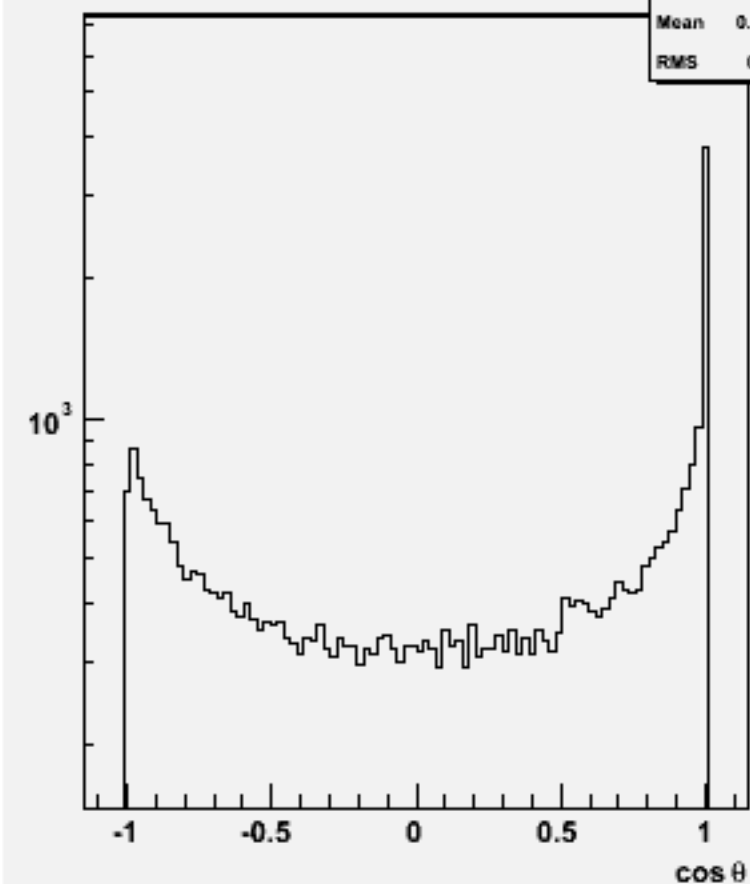
Jet cosθ (All jets)w101893 ccccc_o
