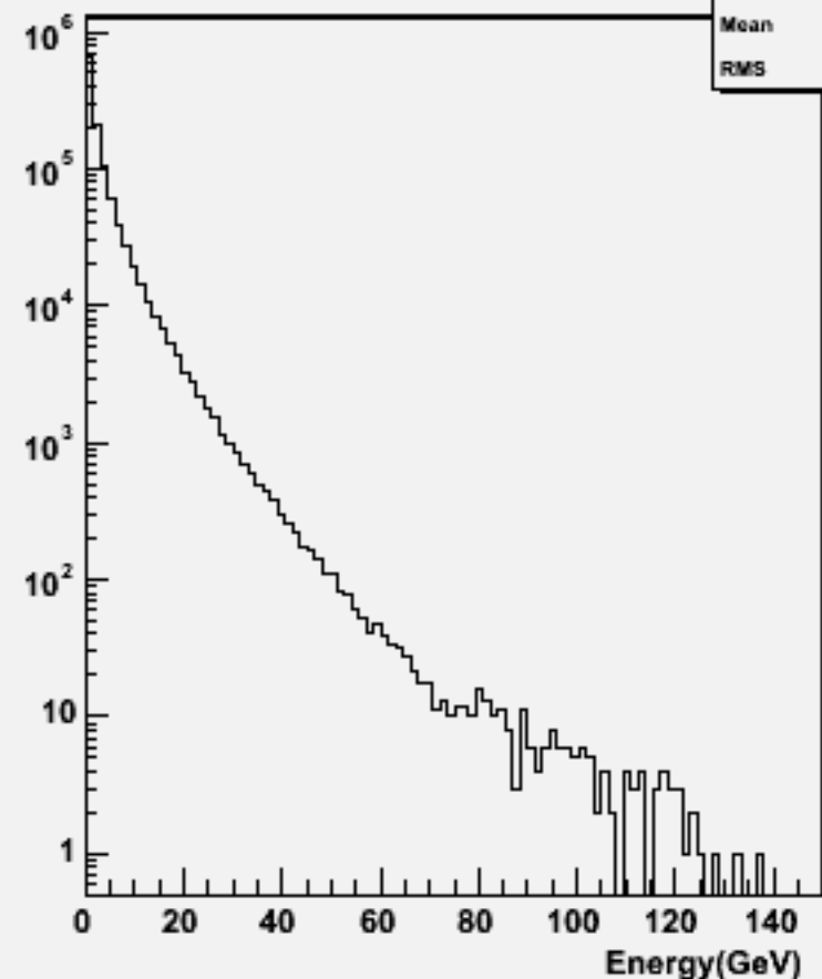
Start point R : w101893 ccccc_o
