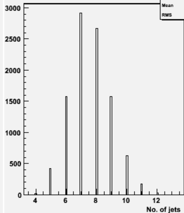
No. jets (ycut=0.001) : w101892 ccccccc_o
