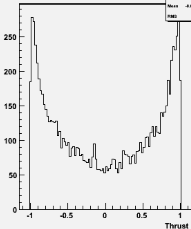
cos \Theta (thrust) w101892 ccccccc_o
