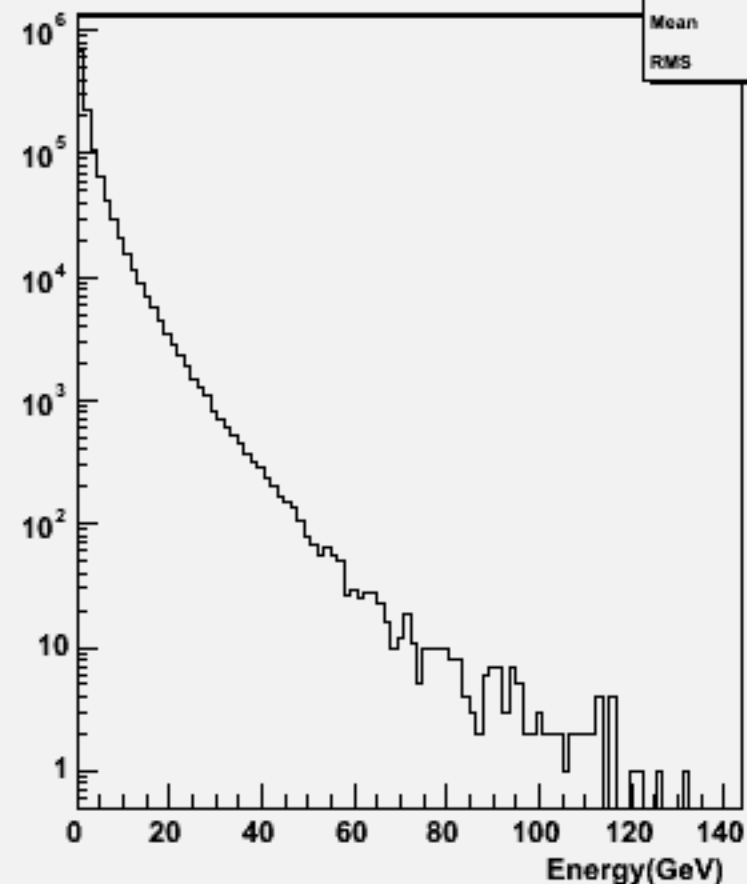
Particle Energy : w101892 ccccccc_o
