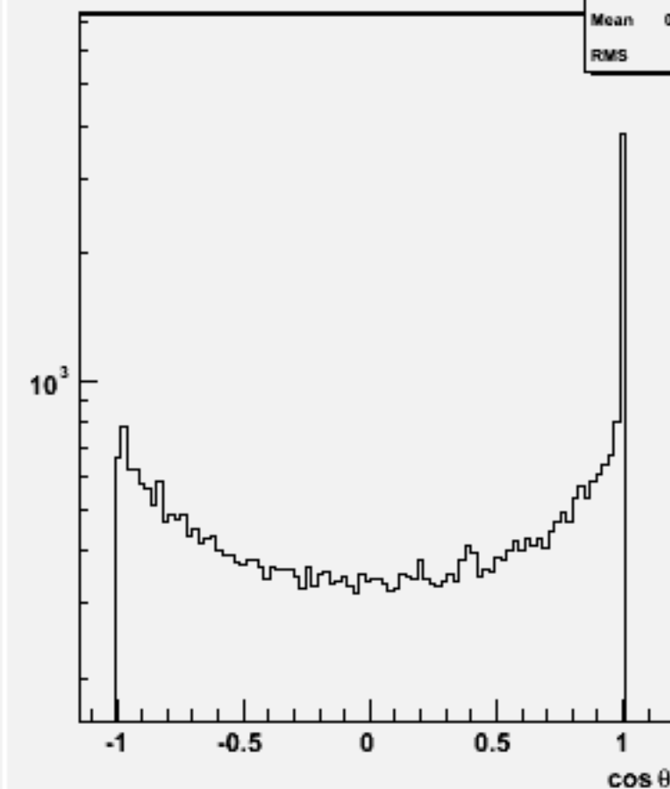
Jet cos \theta (All jets)w101892 ccccc_o
