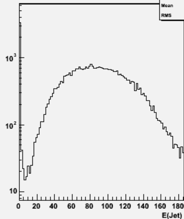
Jet energies(All jets)w101892 ccccc_o
