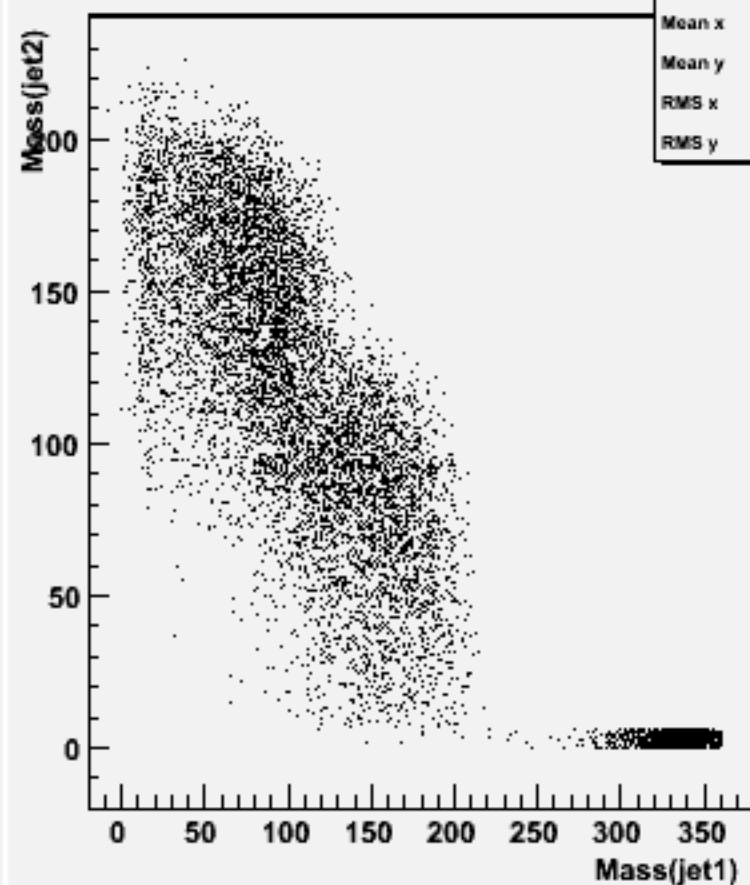
Jet mass for forced 2-jets : w101892 ccccccc_o
