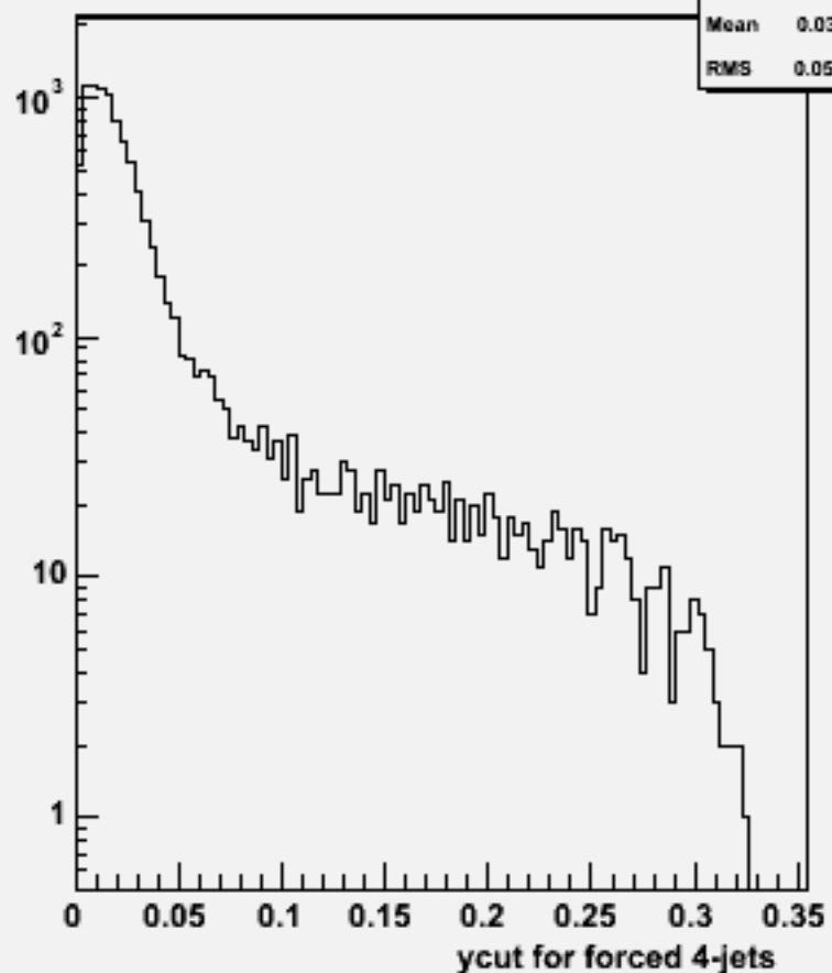
Ycut for 4-jets :w101892 ccccc_o
