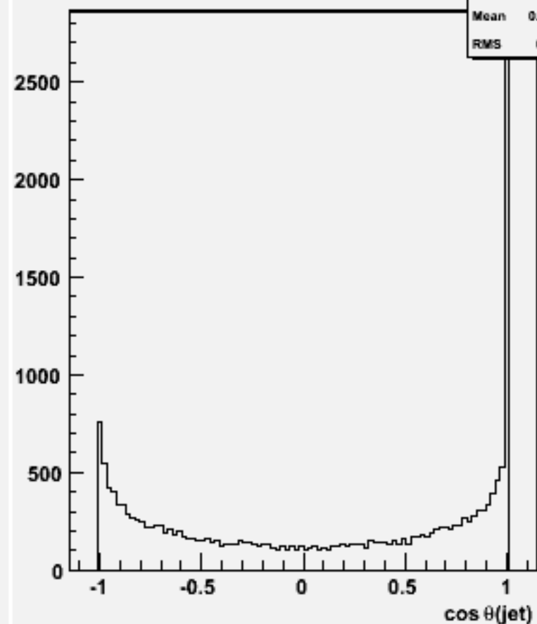
cos \Theta for 2-jets :w101892 ccccccc_o
