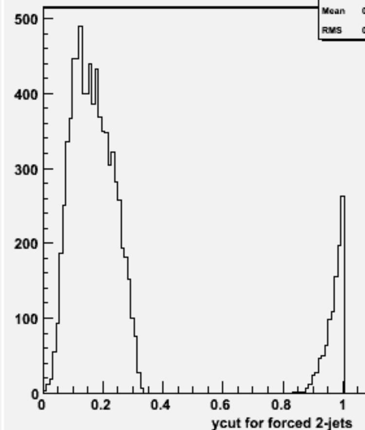
Ycut for 2-jets :w101892 ccccccc_o
