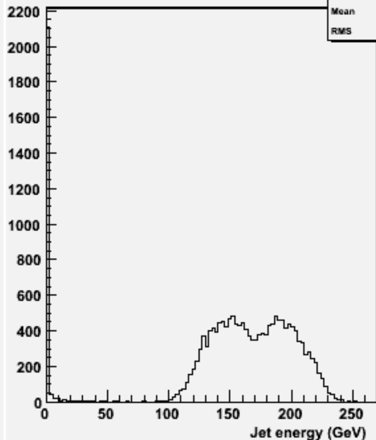
energy for 2-jets :w101892 ccccccc_o
