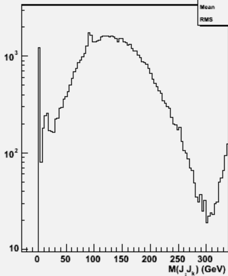
2jets mass(All comb)w101892 ccccc_o
