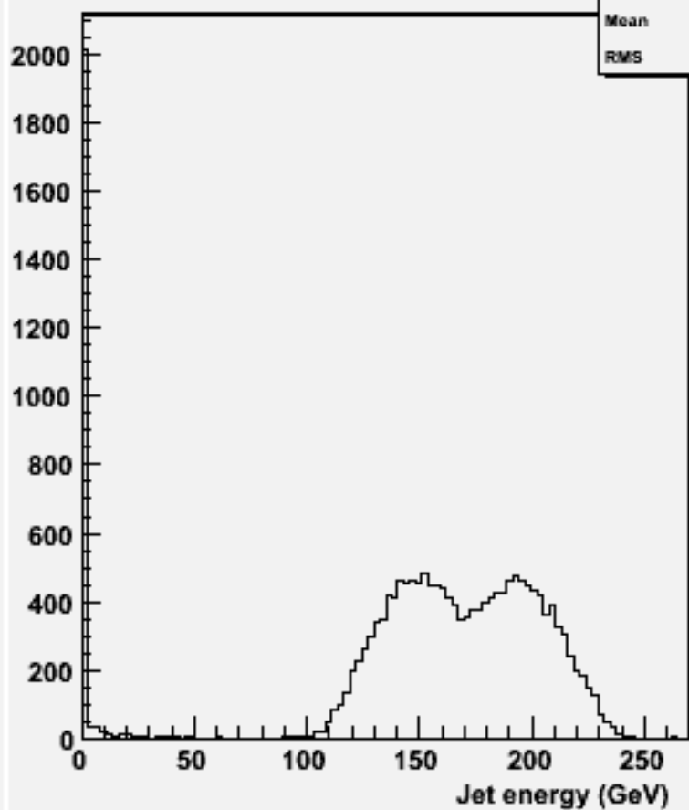
energy for 2-jets :w101888 uucccc_o
