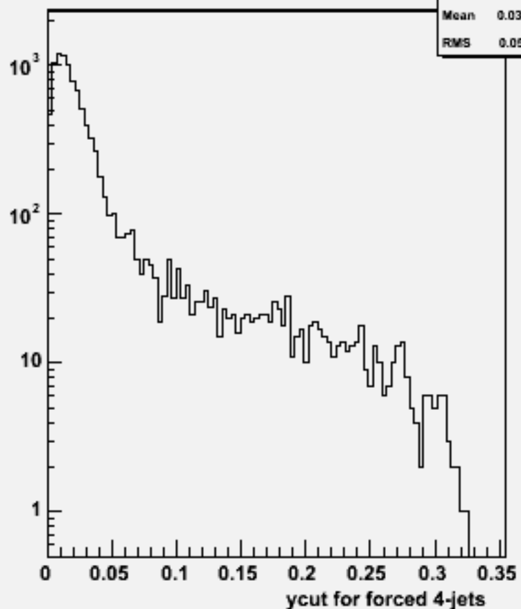
Ycut for 4-jets :w101888 uucccc_o
