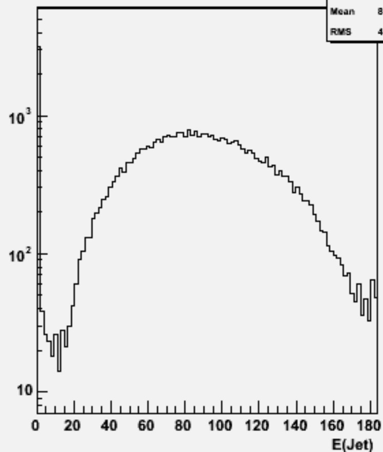
Jet energies(All jets)w101888 uucccc_o
