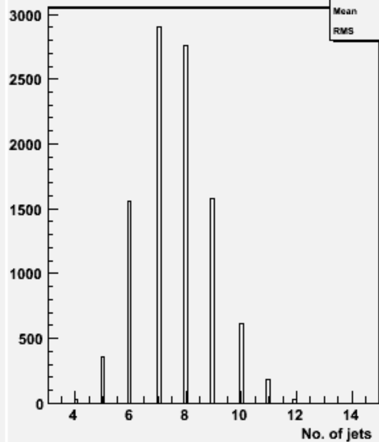
No. jets (ycut=0.001) : w101888 uucccc_o
