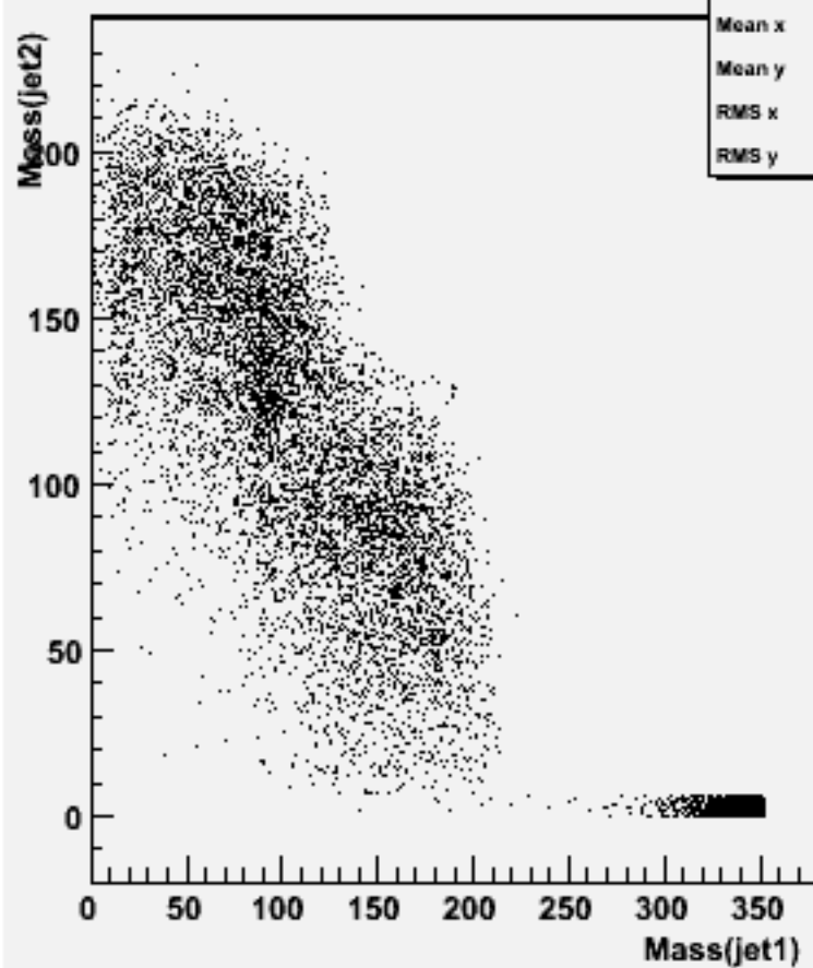
Jet mass for forced 2-jets : w101888 uucccc_o
