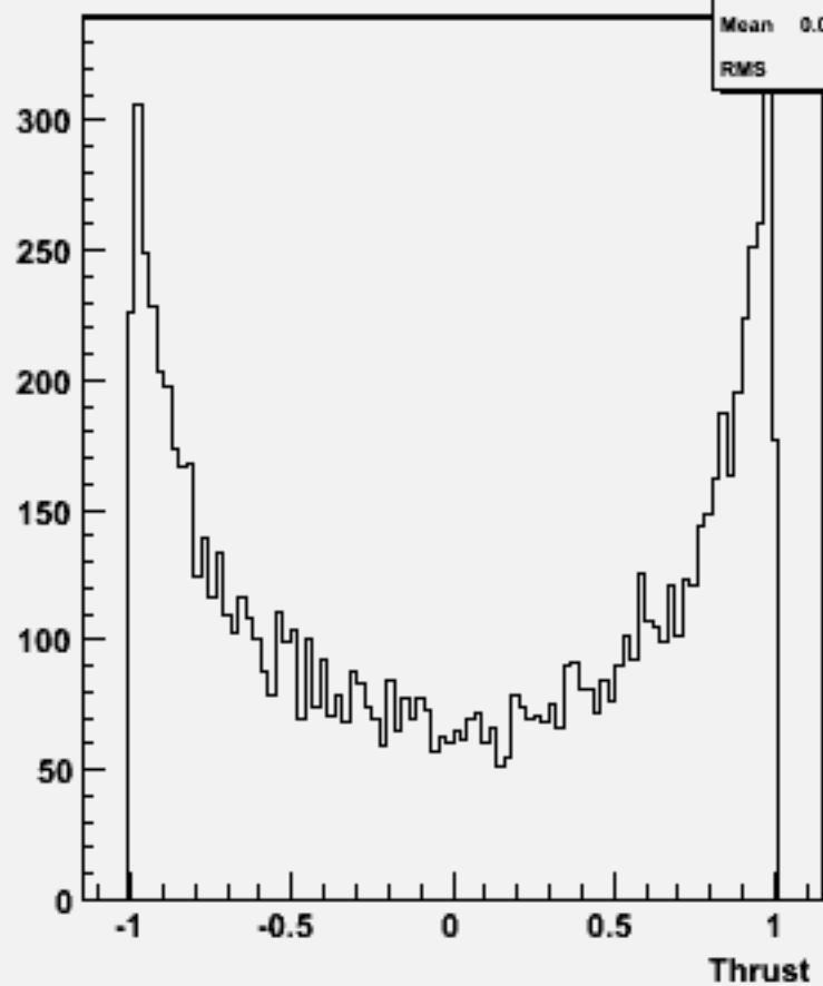
cos \Theta (thrust) w101888 uucccc_o
