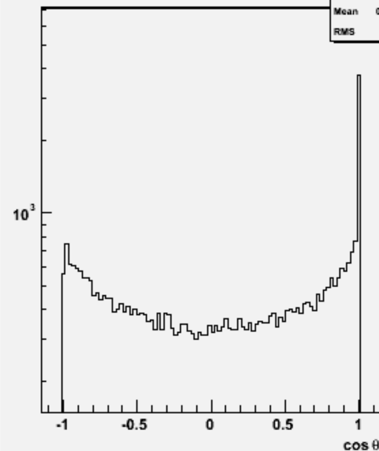
Jet cos \theta (All jets)w101888 uucccc_o
