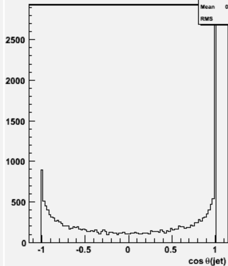
cos \theta for 2-jets :w101888 uucccc_o
