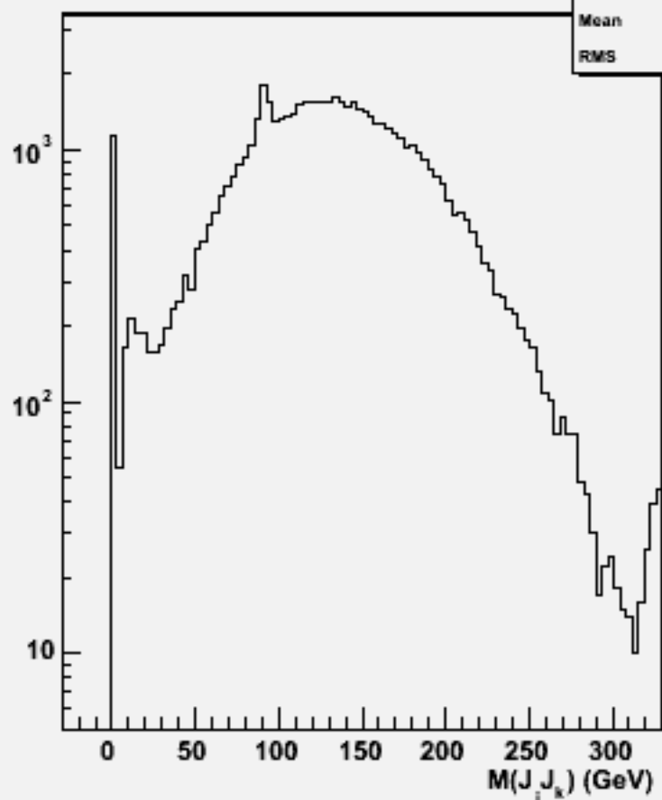
2jets mass(All comb)w101888 uucccc_o
