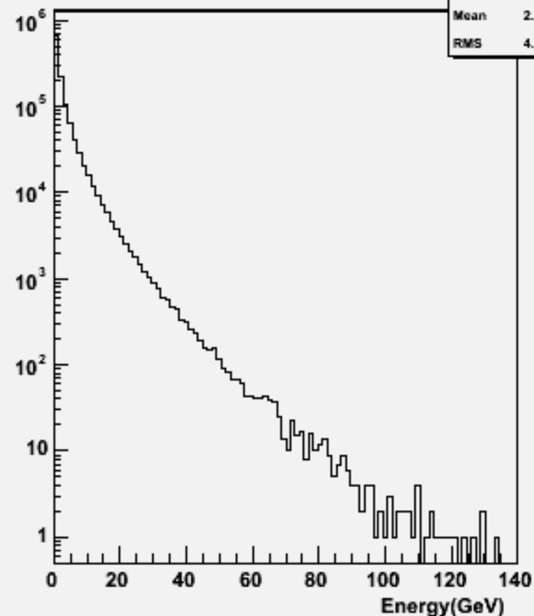
Particle Energy : w101888 uucccc_o
