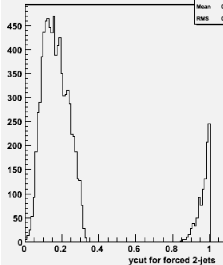
Ycut for 2-jets :w101888 uucccc_o
