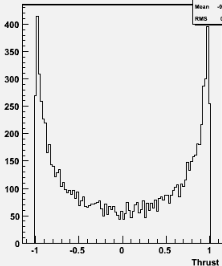
cos \Theta (thrust) w101885 uuuucc_o
