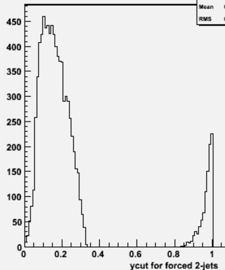
Ycut for 2-jets :w101885 uuuucc_o
