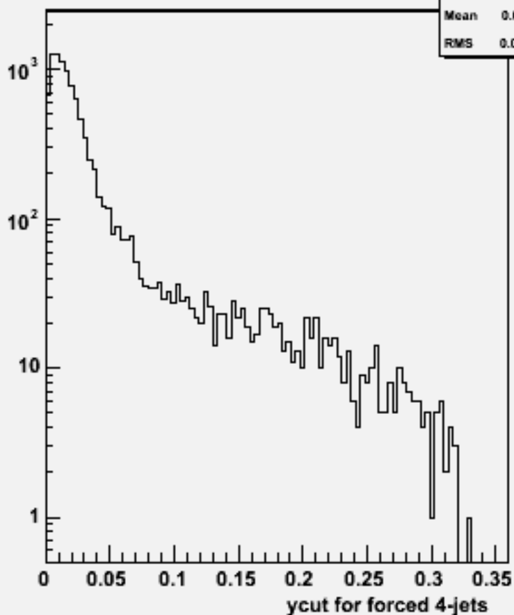
Ycut for 4-jets :w101885 uuuucc_o
