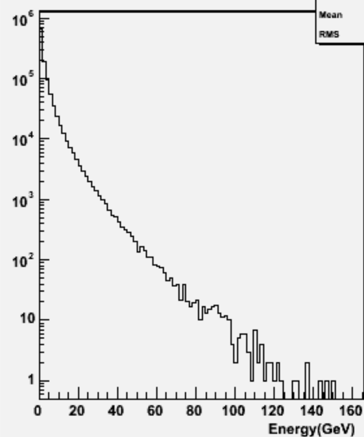
Particle Energy : w101885 uuucc_o
