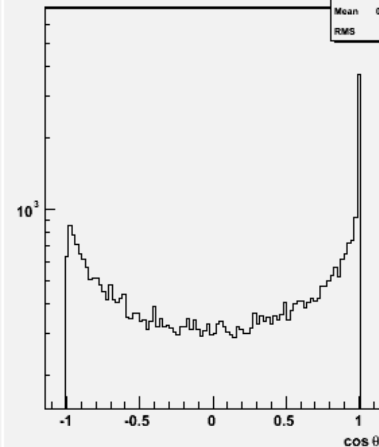
Jet cos \theta (All jets)w101885 uuuucc_o
