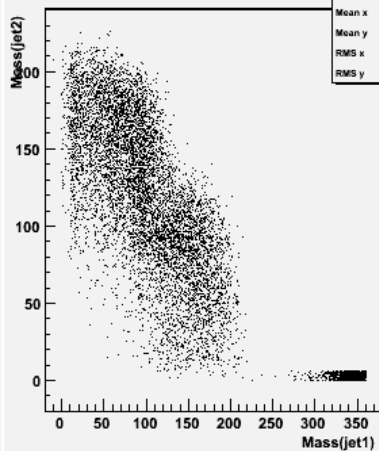
Jet mass for forced 2-jets : w101885 uuuucc_o
