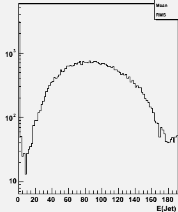
Jet energies(All jets)w101885 uuuucc_o
