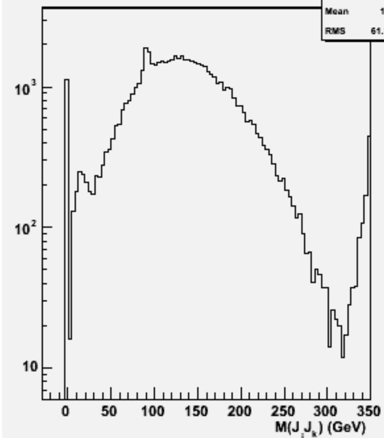
2jets mass(All comb)w101885 uuuucc_o
