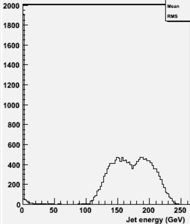
energy for 2-jets :w101885 uuuucc_o
