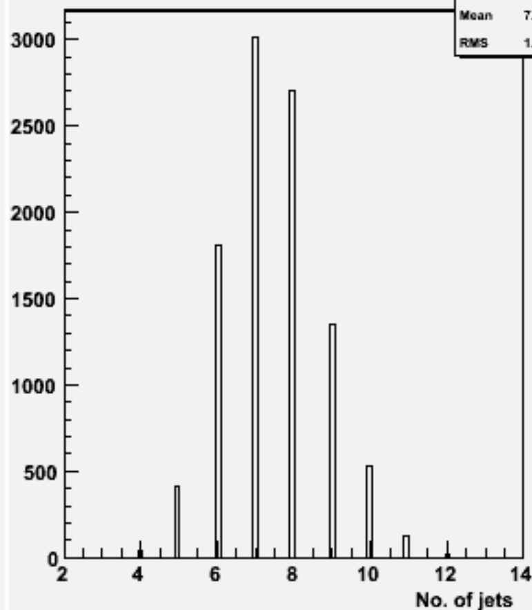
No. jets (ycut=0.001) : w101885 uuuucc_o
