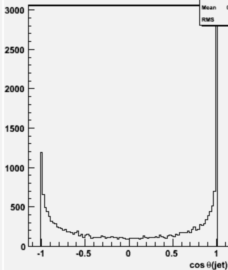
cos \theta for 2-jets :w101885 uuuucc_o
