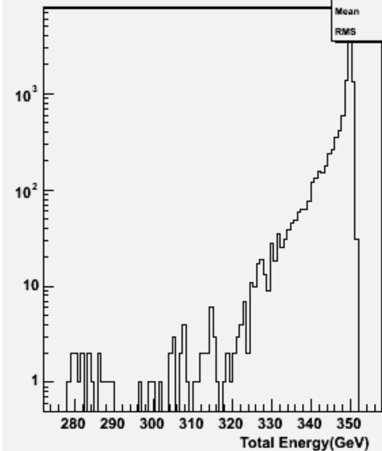
Total Energy (inc. \nu ): w101881 uuuuuu_o
