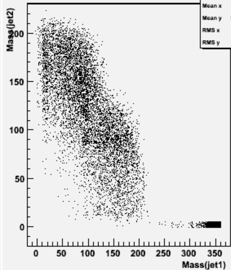
Jet mass for forced 2-jets : w101881 uuuuuu_o
