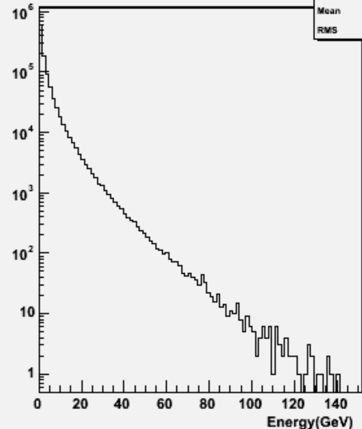
Particle Energy : w101881 uuuuuu_o
