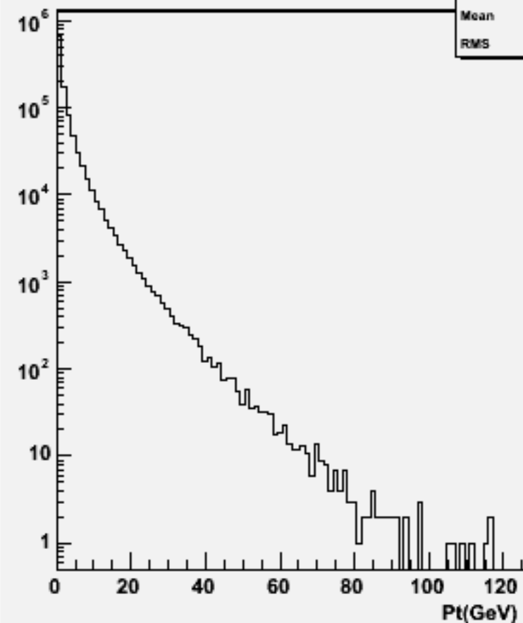
Particle Pt : w101881 uuuuuu_o
