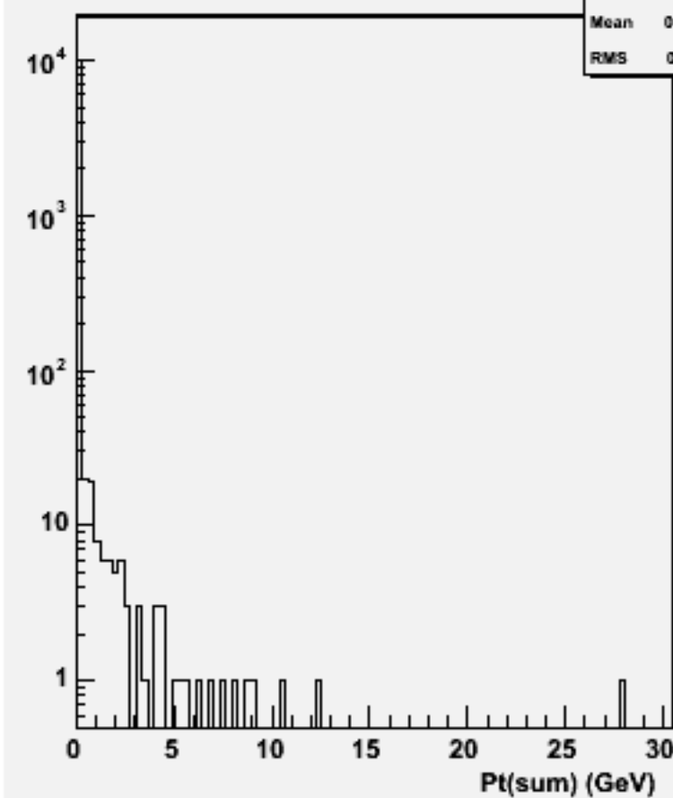
Pt Sum: w101881 uuuuuu_o
