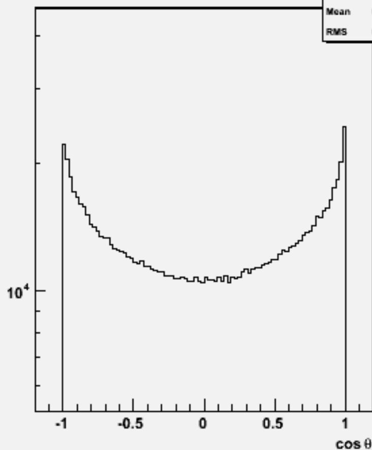
Particle cosθ : w101881 uuuuuu_o
