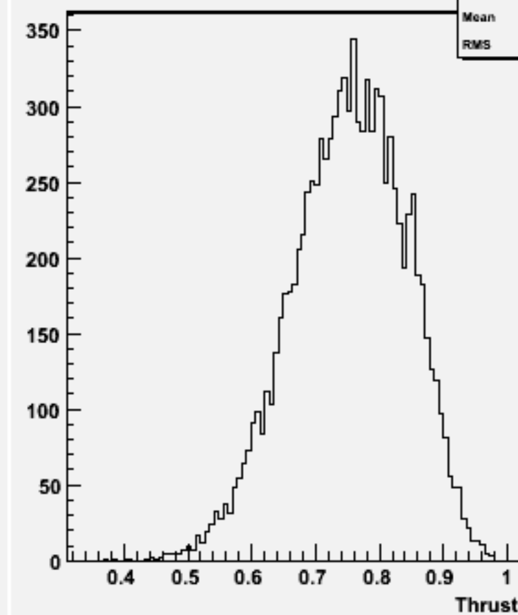
Thrust w101881 uuuuuu_o
