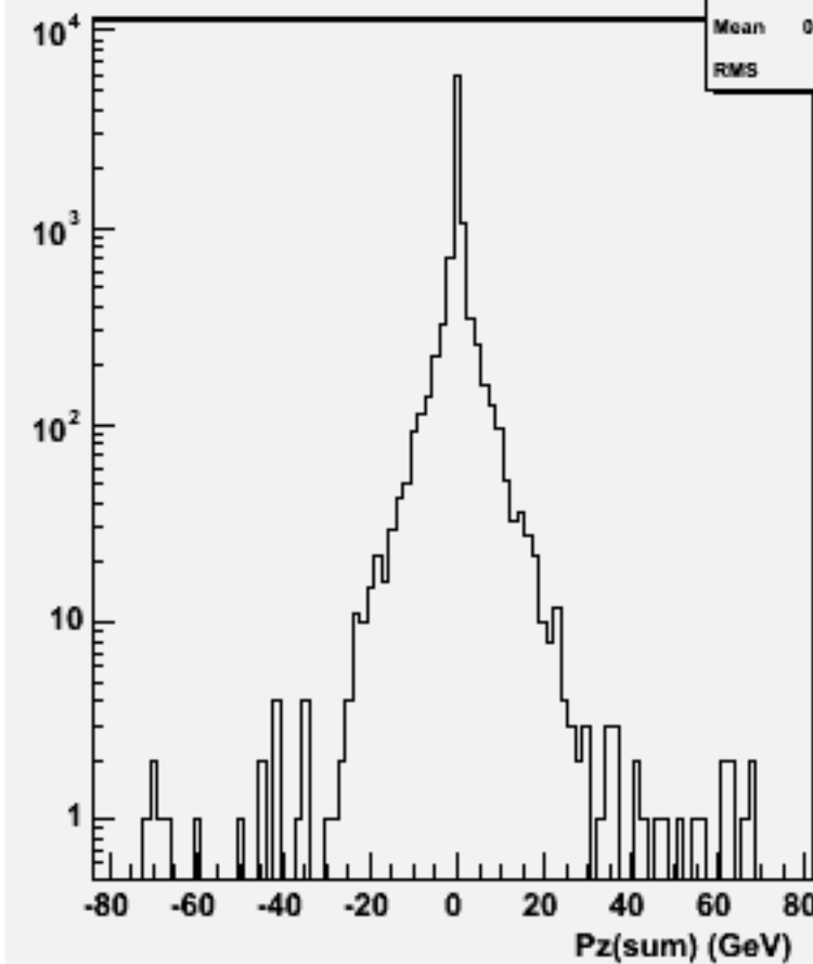
Pz Sum: w101881 uuuuuu_o
