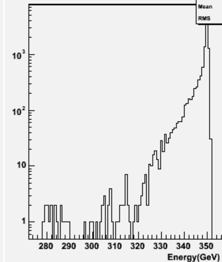
Total Energy (w/o \nu ): w101881 uuuuuu_o
