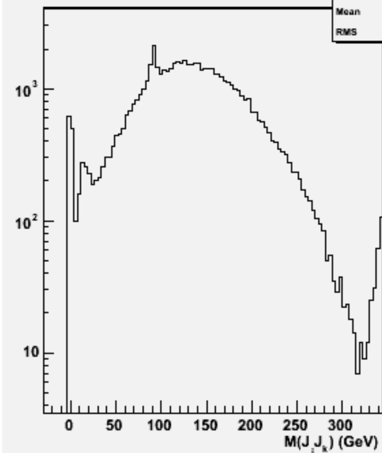
2jets mass(All comb)w101881 uuuuuu_o
