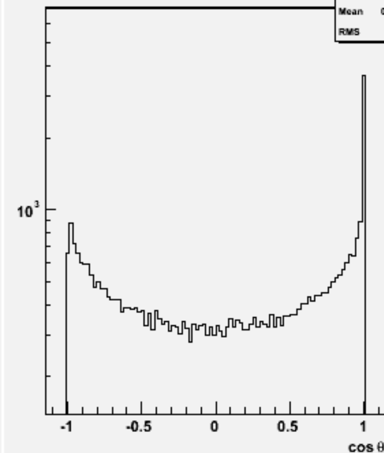
Jet cos \theta (All jets)w101881 uuuuuu_o
