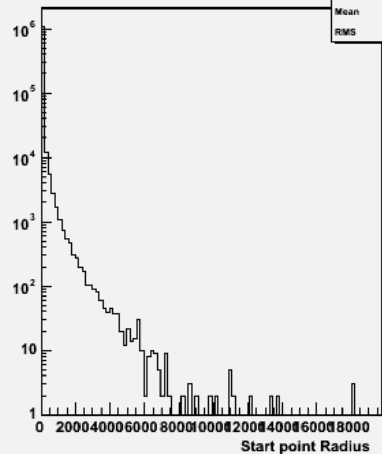
Start point R : w101881 uuuuuu_o
