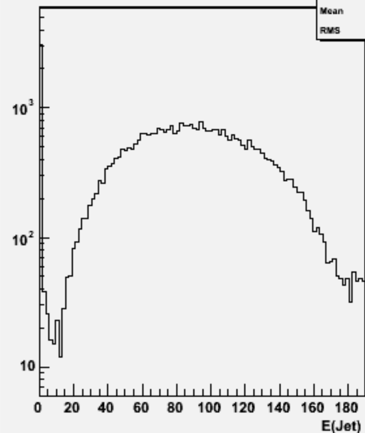
Jet energies(All jets)w101881 uuuuuu_o
