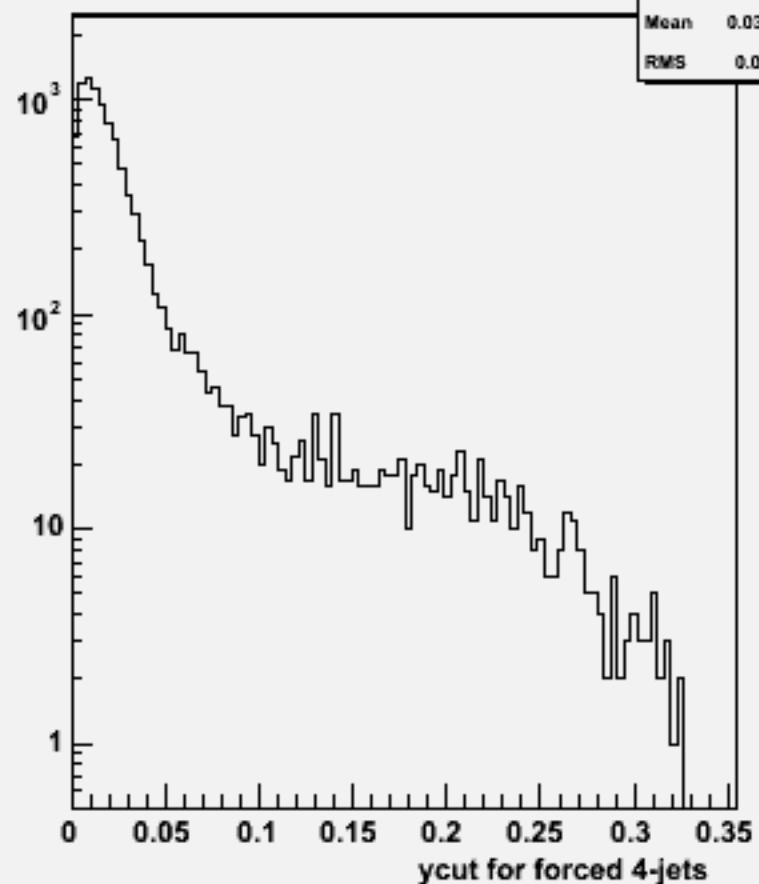
Ycut for 4-jets :w101881 uuuuuu_o
