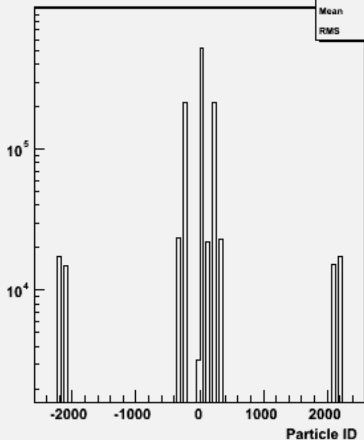
Particle ID : w101881 uuuuuu_o
