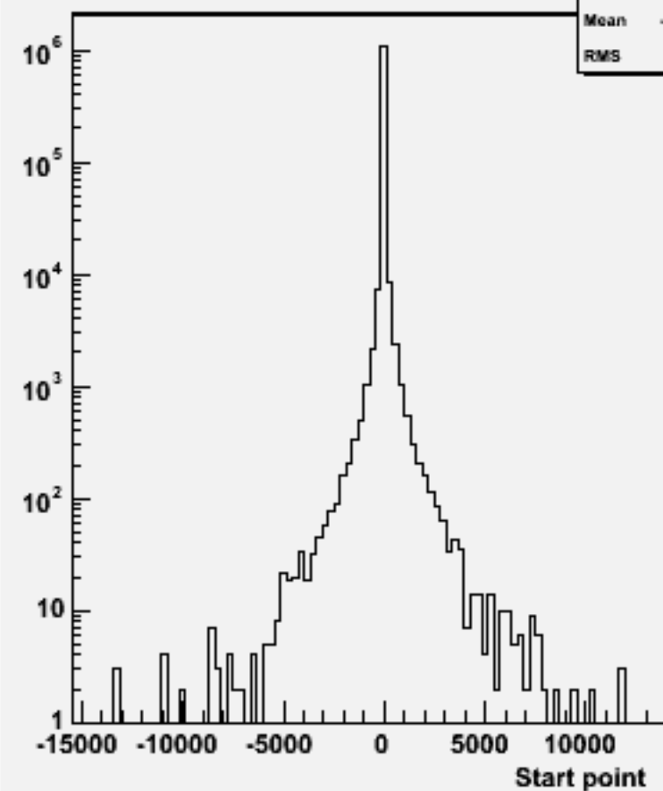
Start point Z : w101881 uuuuuu_o
