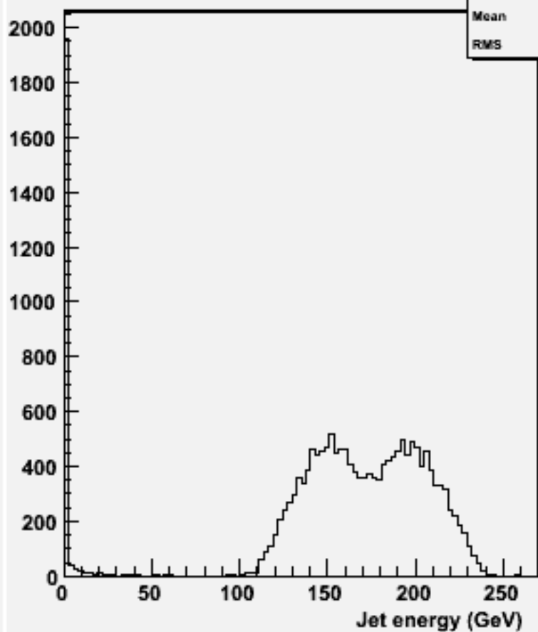
energy for 2-jets :w101880 uuuuuu_o
