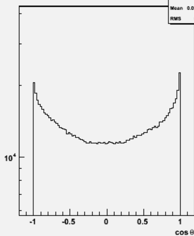
Particle cosθ : w101880 uuuuuu_o
