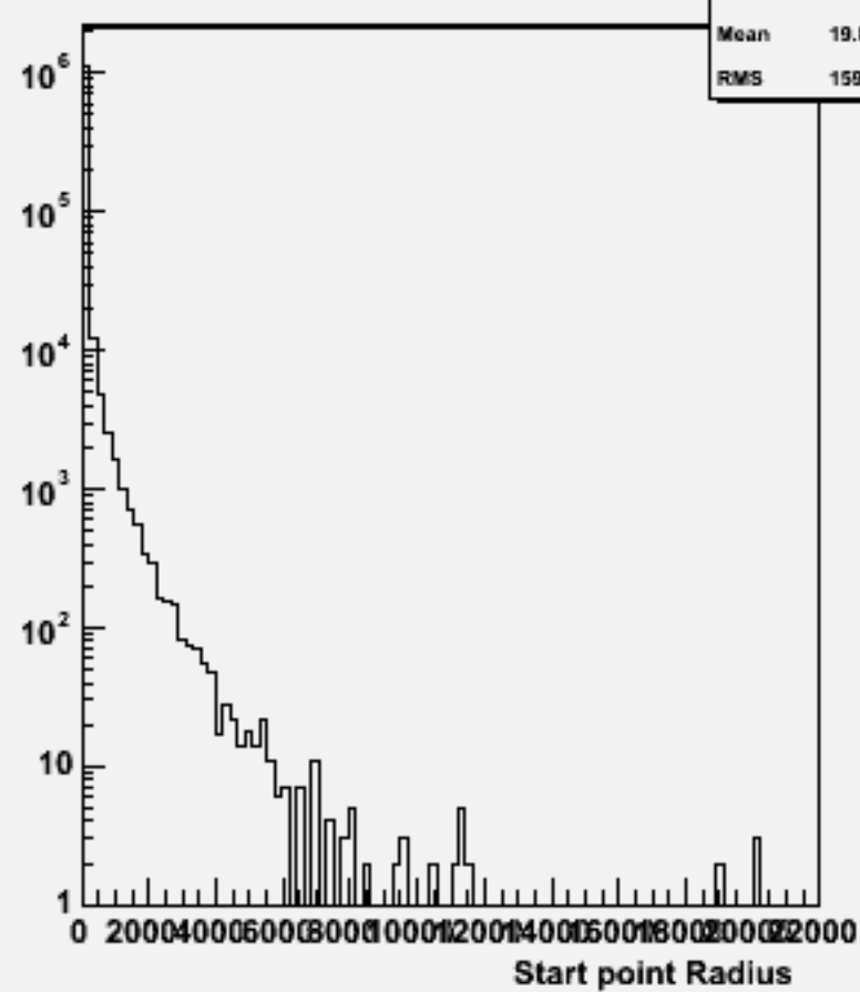
Start point R : w101880 uuuuuu_o
