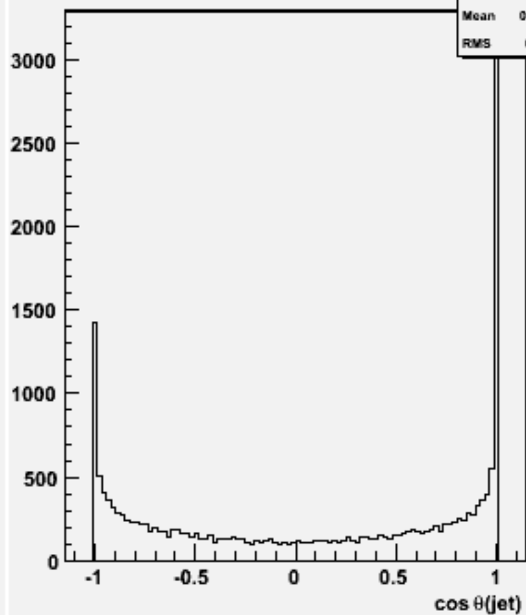
cos \theta for 2-jets :w101880 uuuuuu_o
