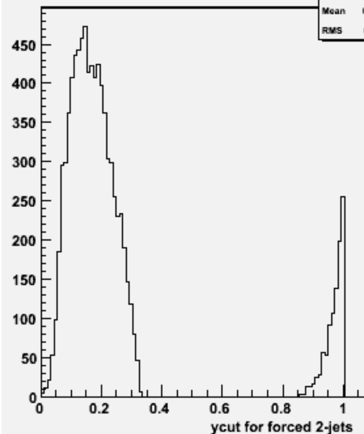
Ycut for 2-jets :w101880 uuuuuu_o
