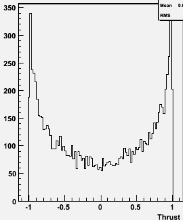
cos \Theta (thrust) w101880 uuuuuu_o
