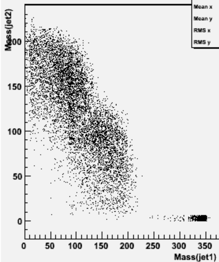
Jet mass for forced 2-jets : w101880 uuuuuu_o
