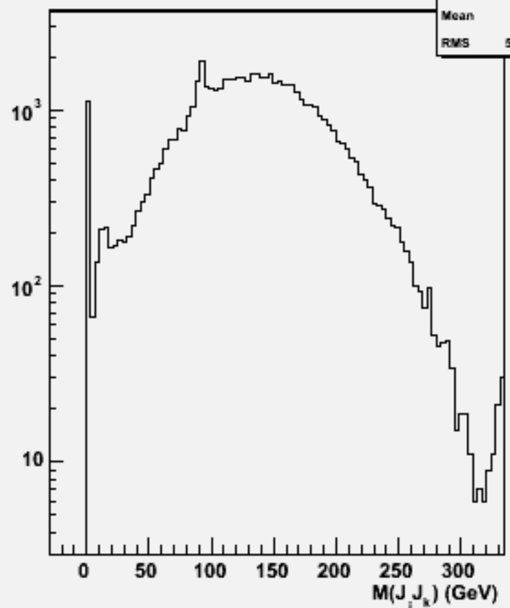
2jets mass(All comb)w101880 uuuuuu_o
