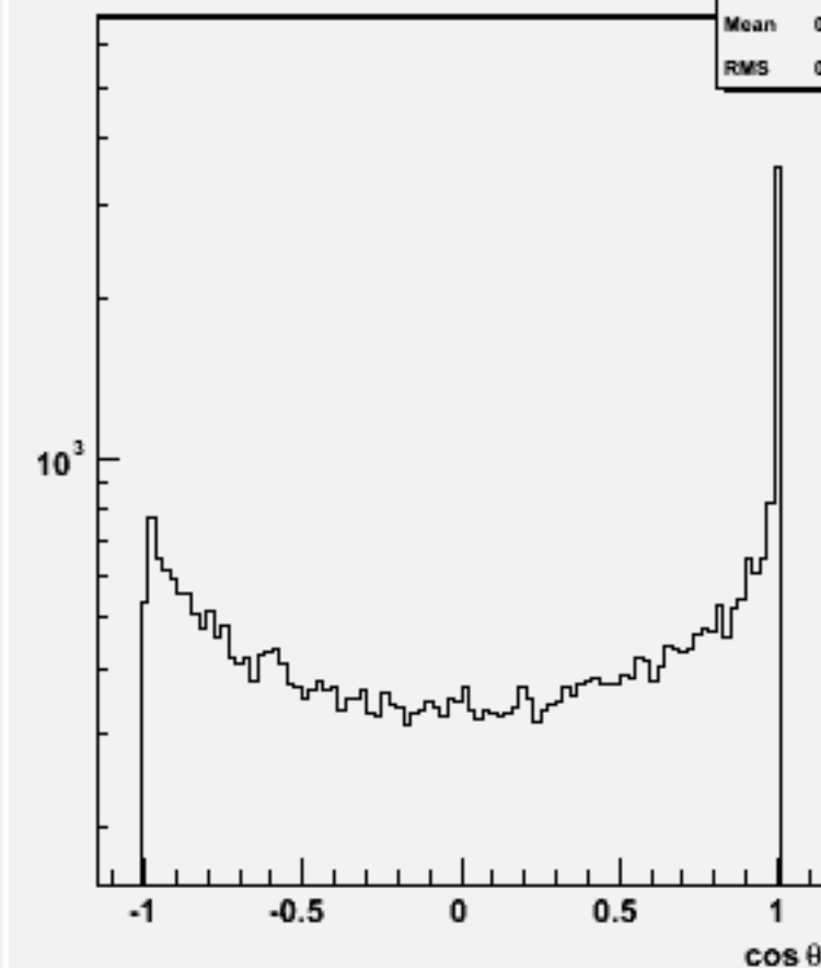
Jet cos \theta (All jets)w101880 uuuuuu_o
