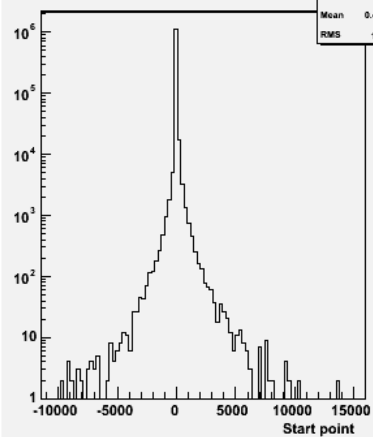
Start point Z : w101880 uuuuuu_o
