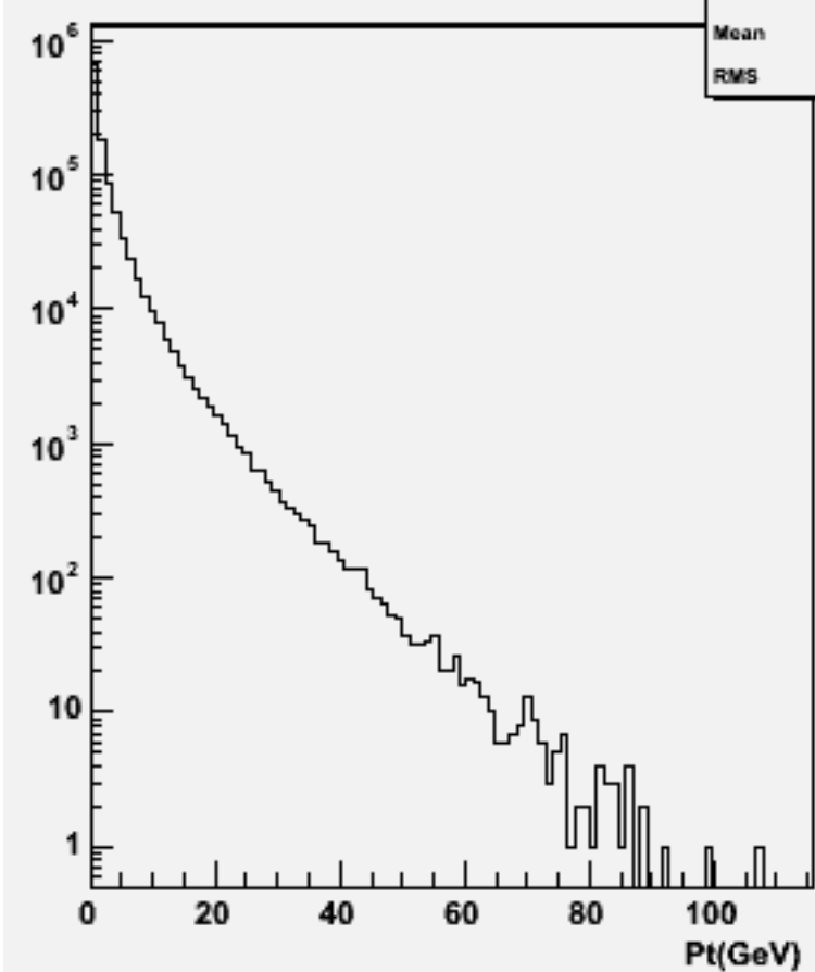
Particle Pt : w101880 uuuuuu_o
