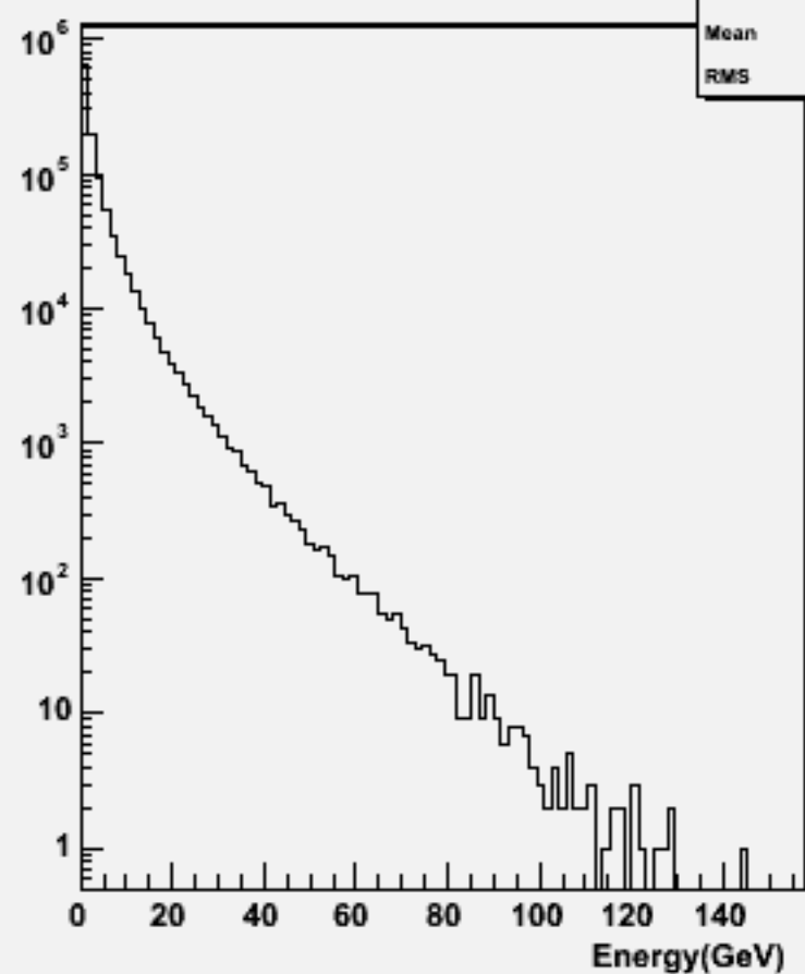
Particle Energy : w101880 uuuuuu_o
