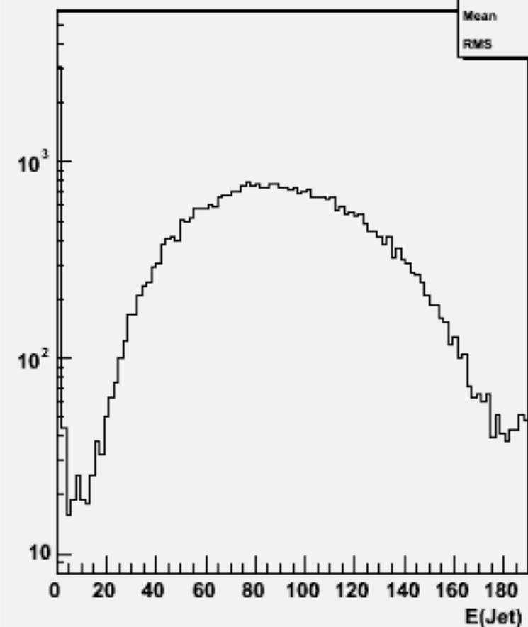
Jet energies(All jets)w101880 uuuuuu_o
