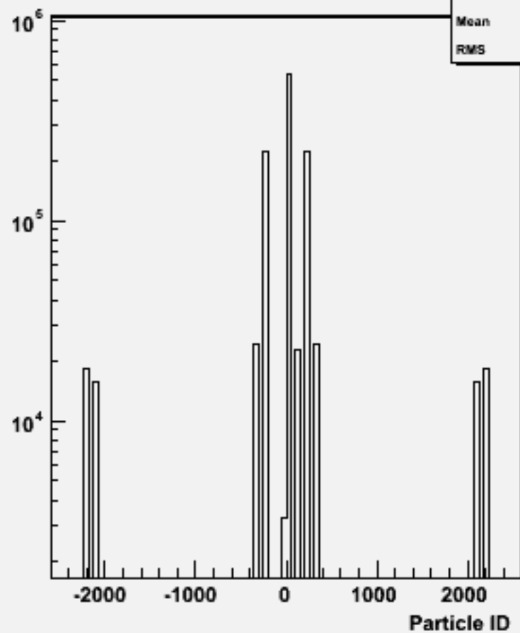
Particle ID : w101880 uuuuuu_o
