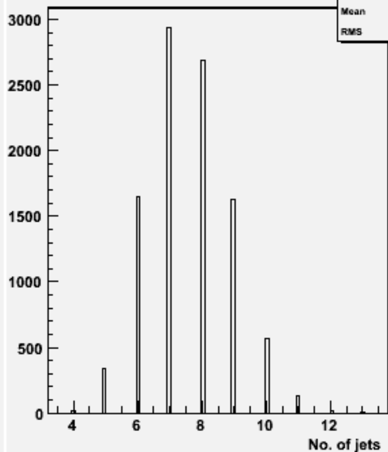
No. jets (ycut=0.001) : w101880 uuuuuu_o
