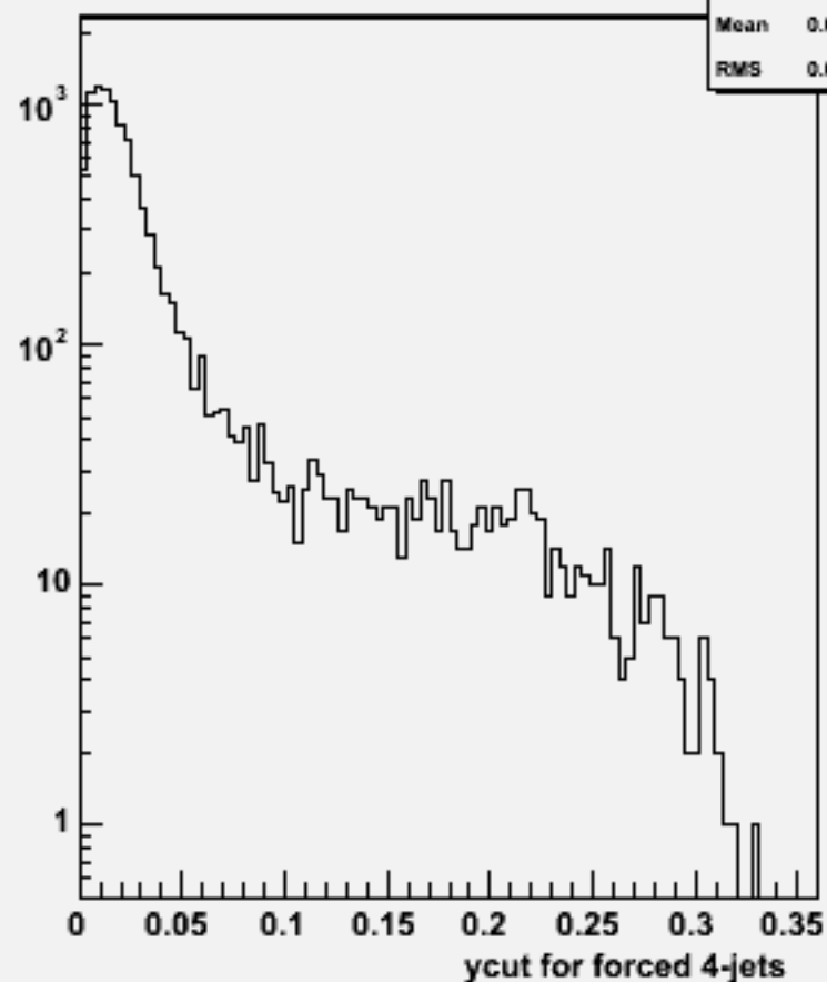
Ycut for 4-jets :w101880 uuuuuu_o
