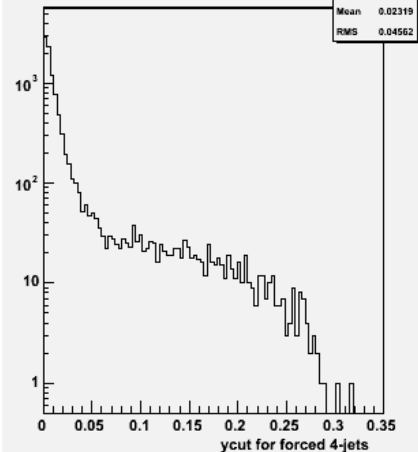
Ycut for 4-jets :w101876 n3n3cccc_o
