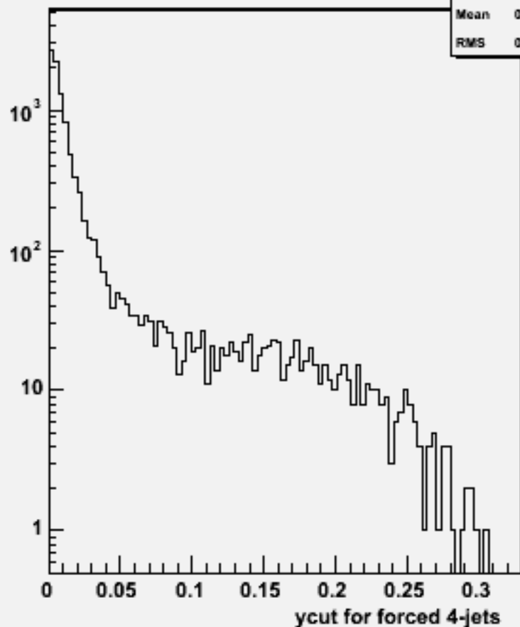
Ycut for 4-jets :w101872 n3n3uucc_o
