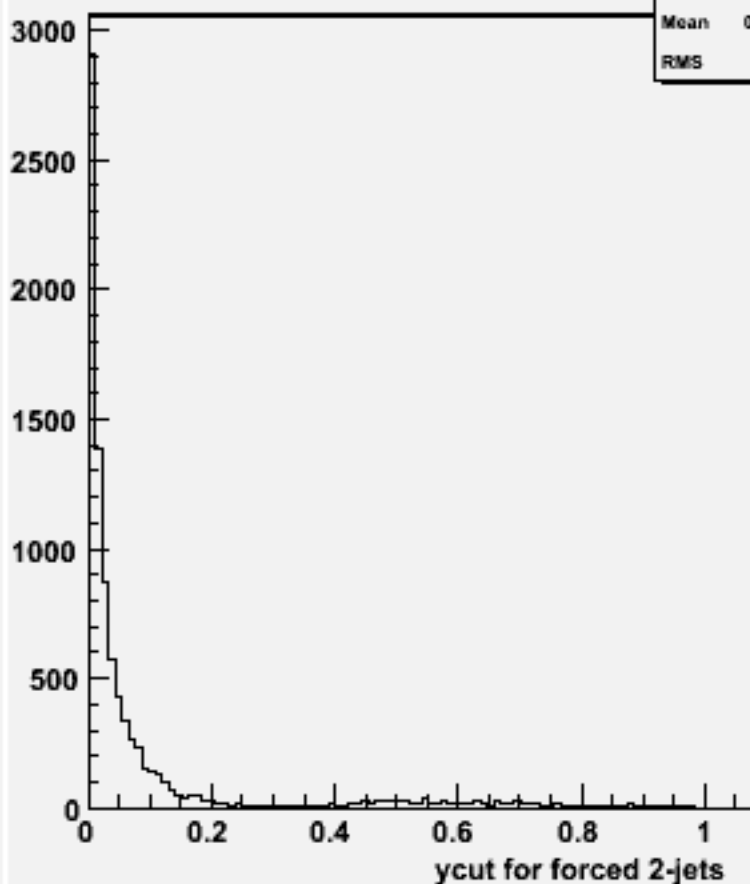
Ycut for 2-jets :w101864 n3n3n3n3cc_o
