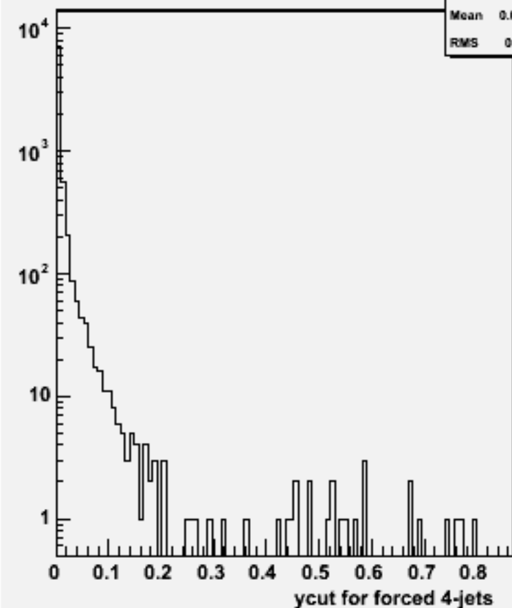
Ycut for 4-jets :w101864 n3n3n3n3cc_o
