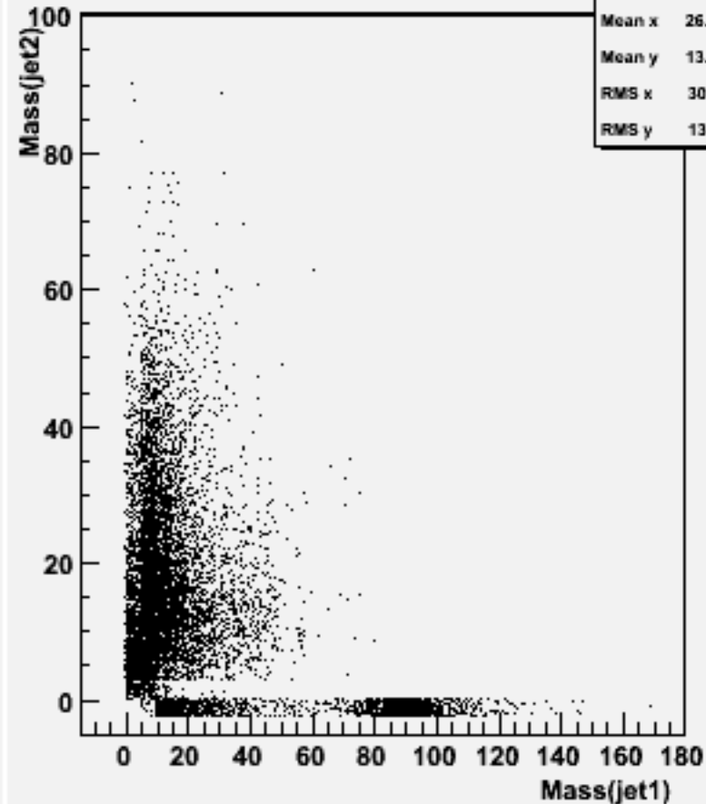
Jet mass for forced 2-jets : w101864 n3n3n3n3cc_o
