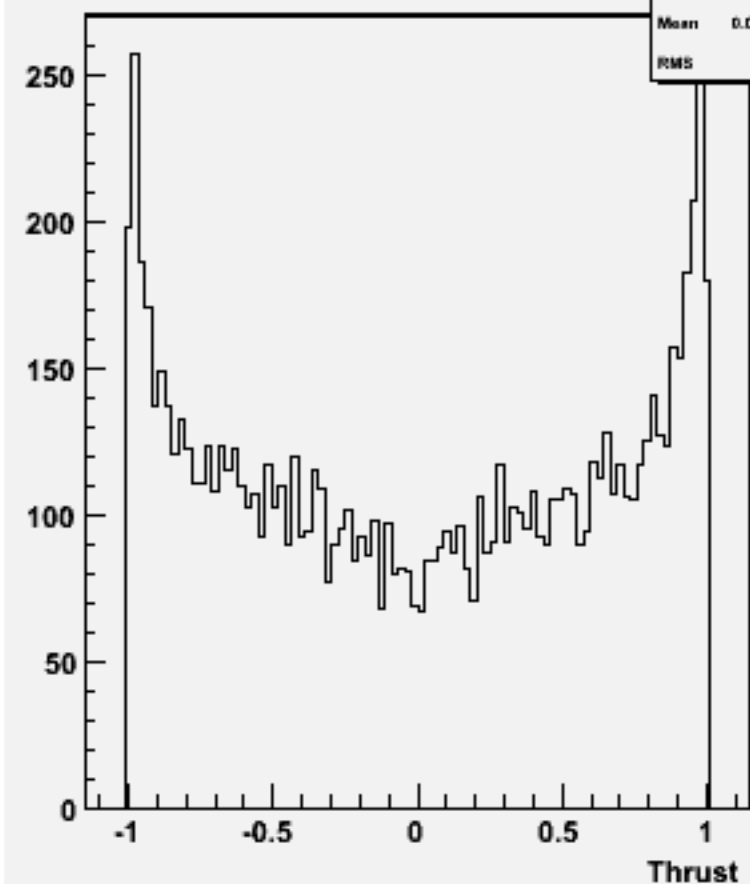
cos \Theta (thrust) w101864 n3n3n3n3cc_o
