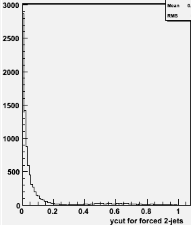
Ycut for 2-jets :w101860 n3n3n3uu_o
