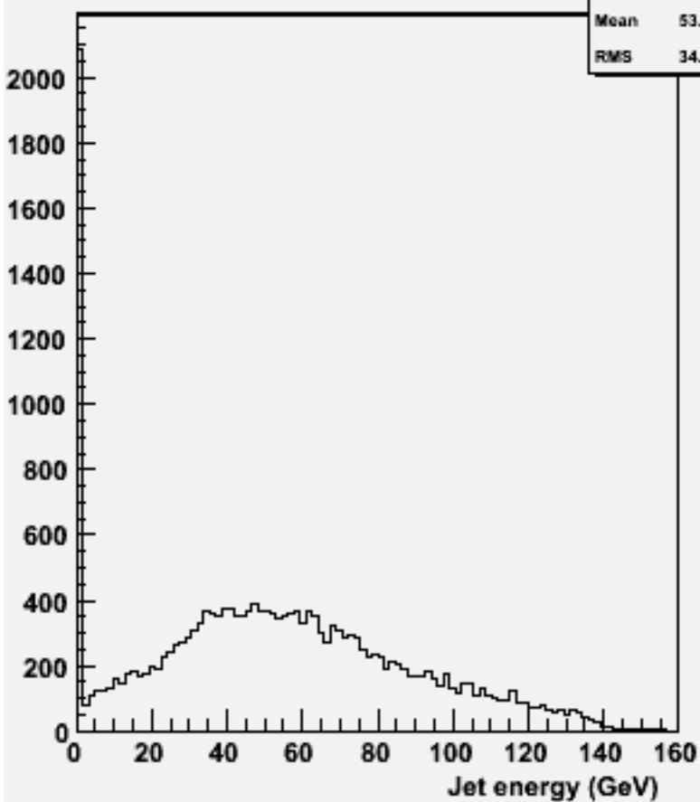
energy for 2-jets :w101860 n3n3n3uu_o
