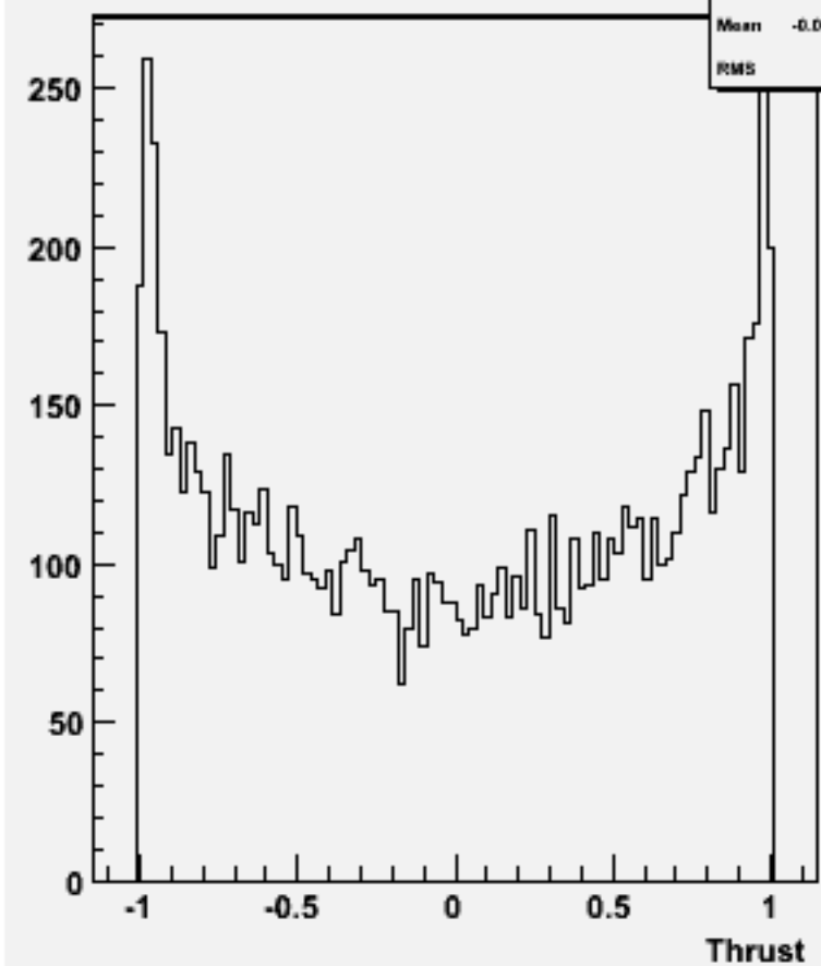
cos \Theta (thrust) w101860 n3n3n3uu_o
