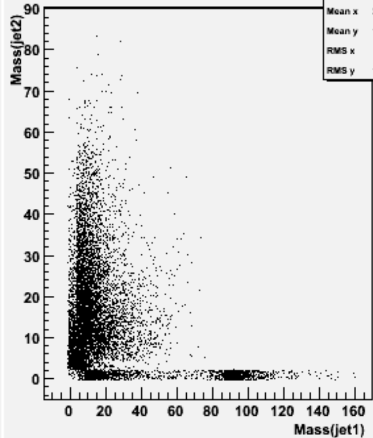
Jet mass for forced 2-jets : w101860 n3n3n3uu_o
