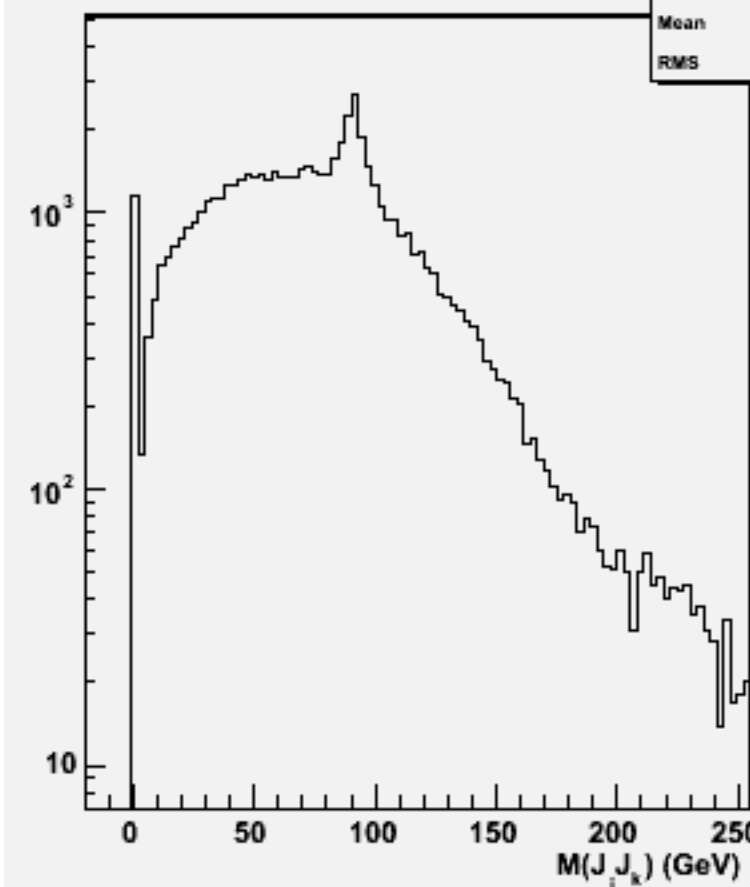
2jets mass(All comb)w101852 n2n2uucc_o
