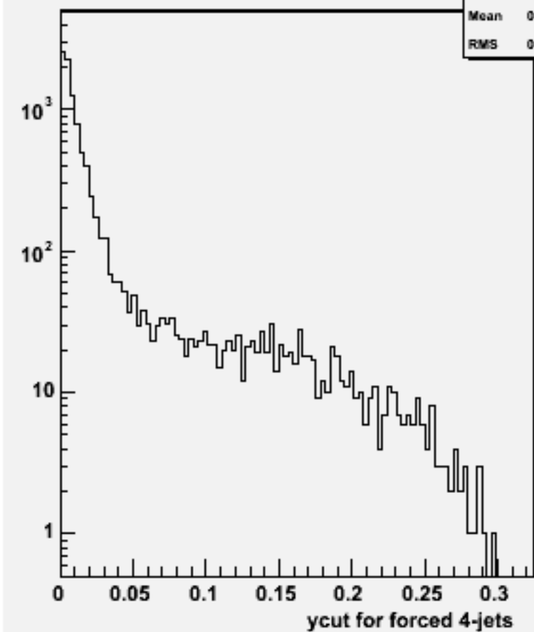
Ycut for 4-jets :w101852 n2n2uucc_o
