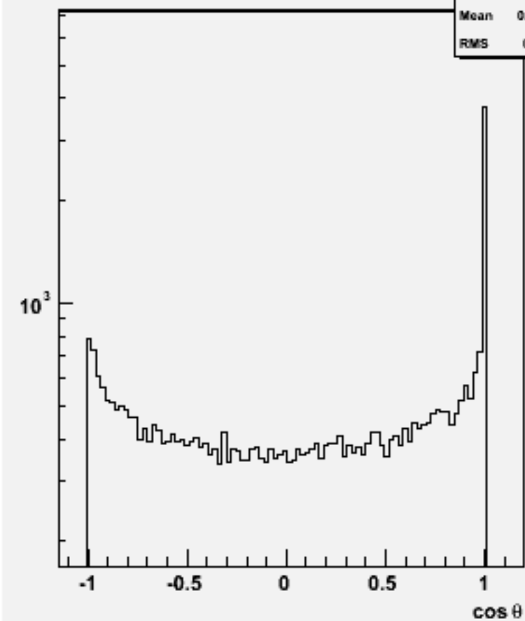
Jet cos \theta (All jets)w101852 n2n2uucc_o
