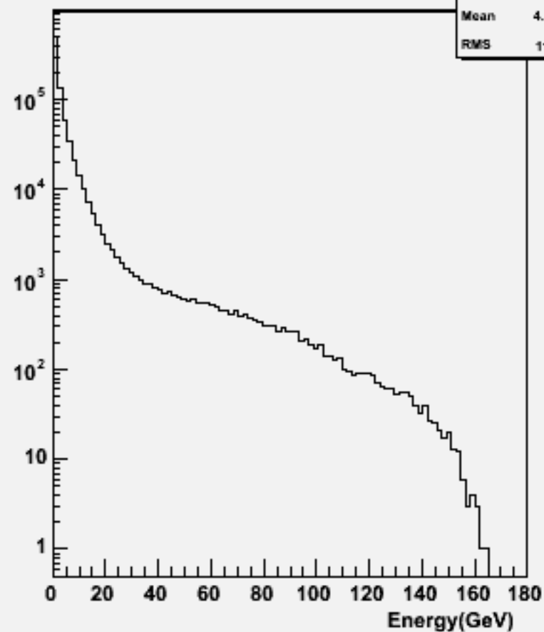
Particle Energy : w101852 n2n2uucc_o
