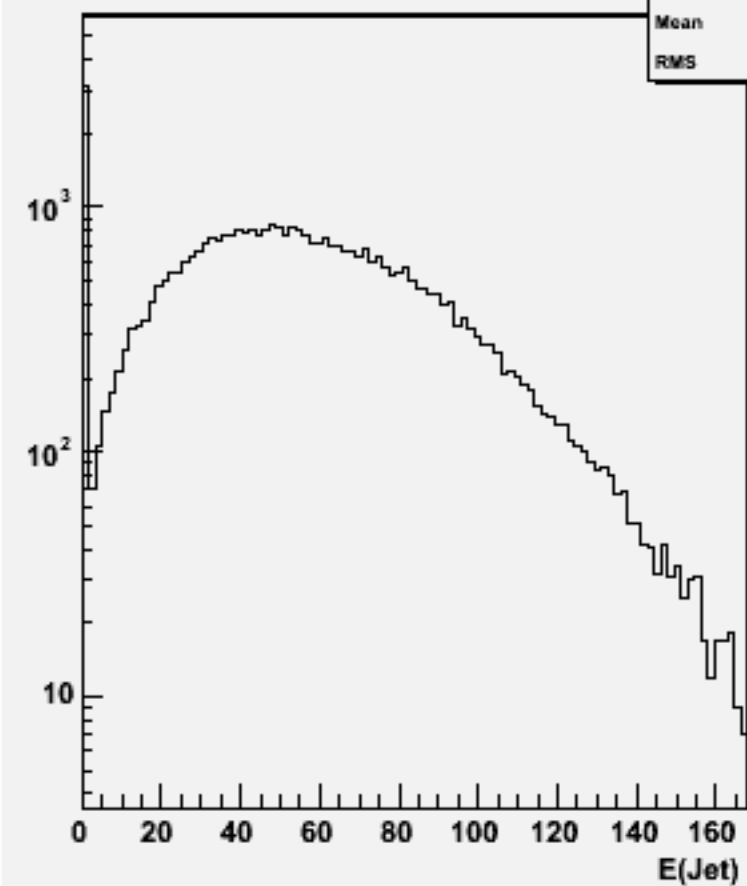
Jet energies(All jets)w101852 n2n2uucc_o
