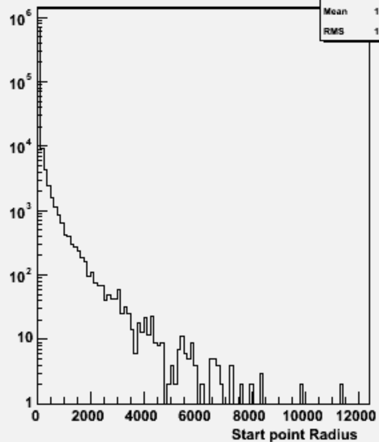
Start point R : w101849 n2n2uuuu_o
