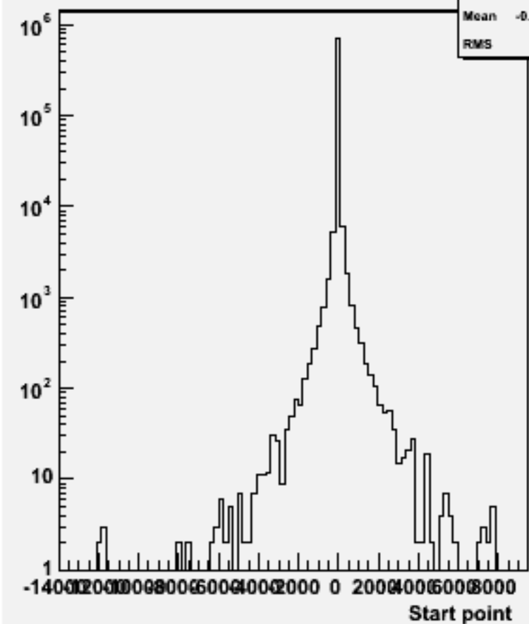
Start point Z : w101849 n2n2uuuu_o
