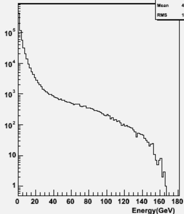
Particle Energy : w101849 n2n2uuuu_o
