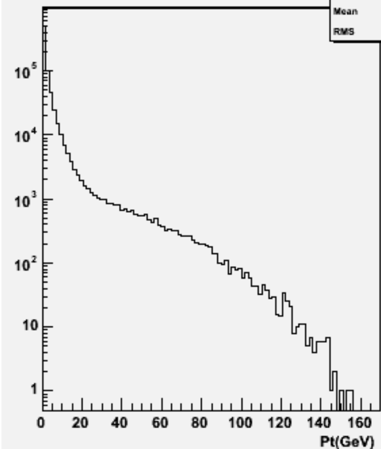
Particle Pt : w101849 n2n2uuuu_o
