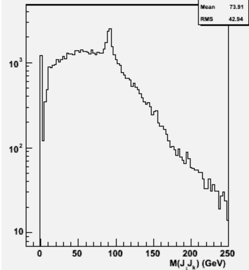
2jets mass(All comb)w101849 n2n2uuuu_o
