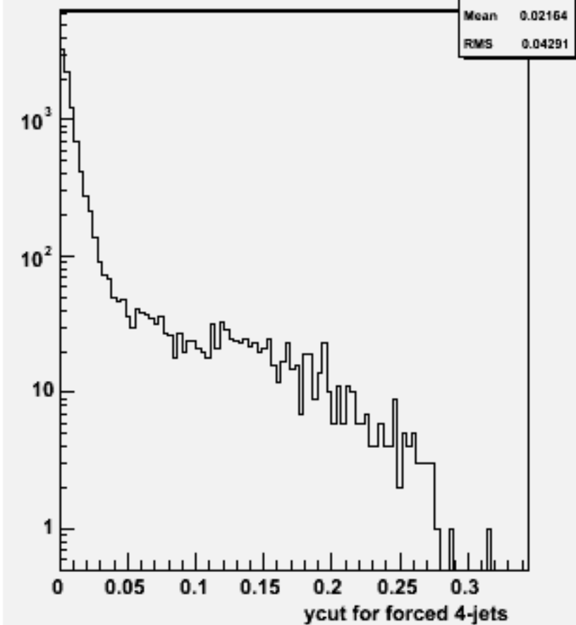
Ycut for 4-jets :w101849 n2n2uuuu_o
