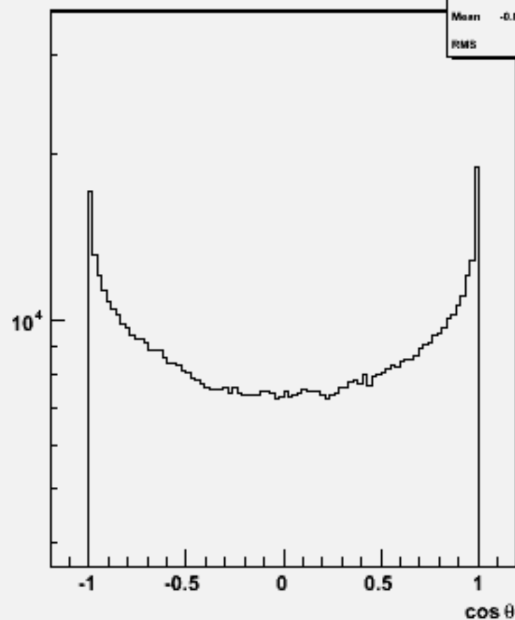
Particle cos \theta : w101849 n2n2uuuu_o
