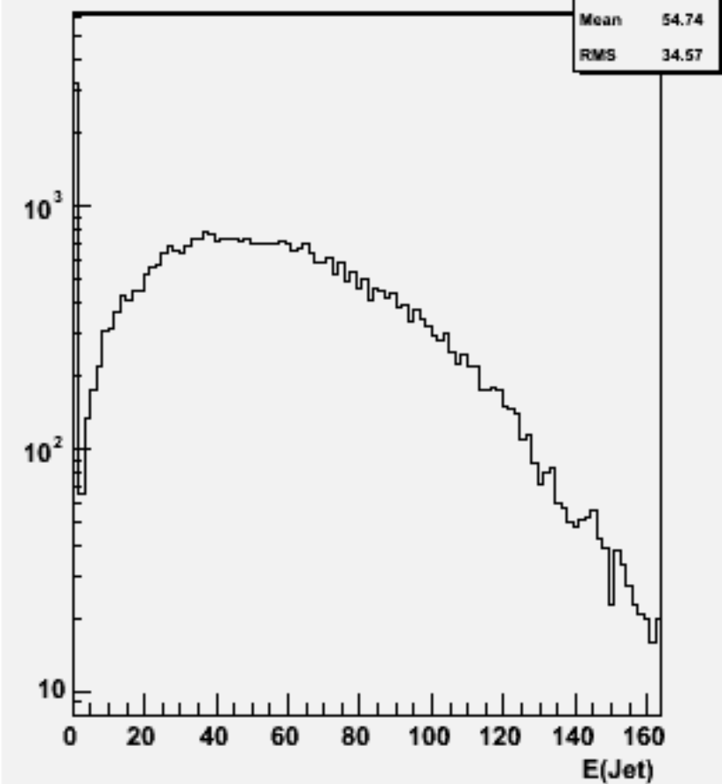
Jet energies(All jets)w101849 n2n2uuuu_o
