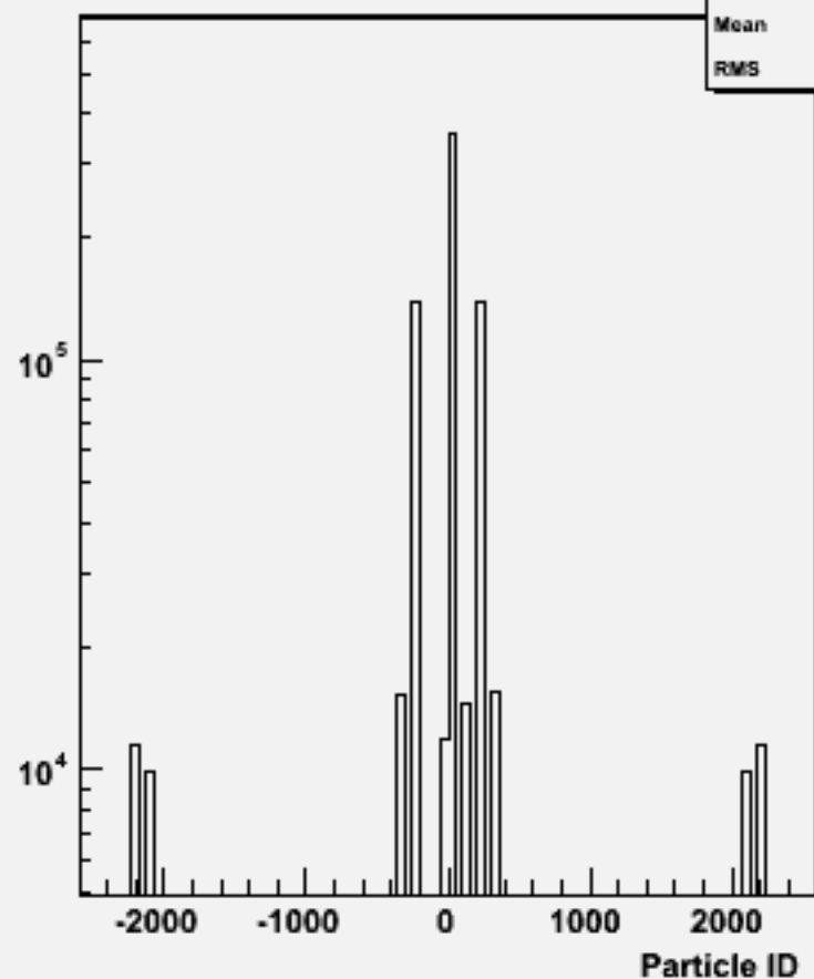
Particle ID : w101849 n2n2uuuu_o
