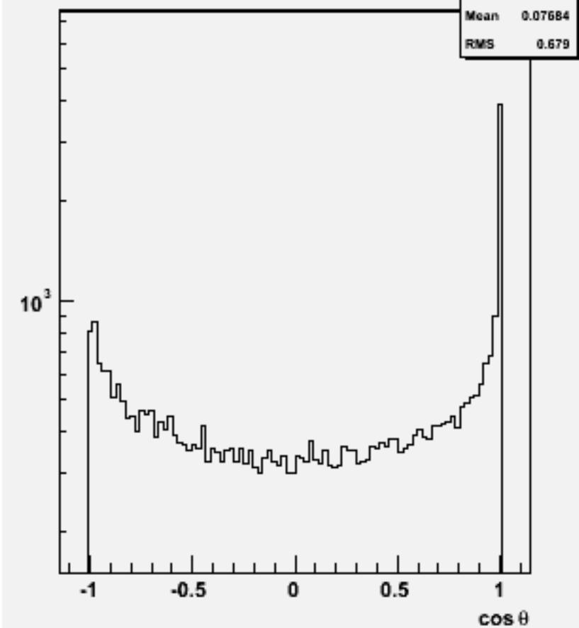
Jet cos \theta (All jets)w101849 n2n2uuuu_o
