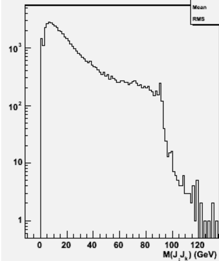
2jets mass(All comb)w101845 n2n2n3n3cc_o
