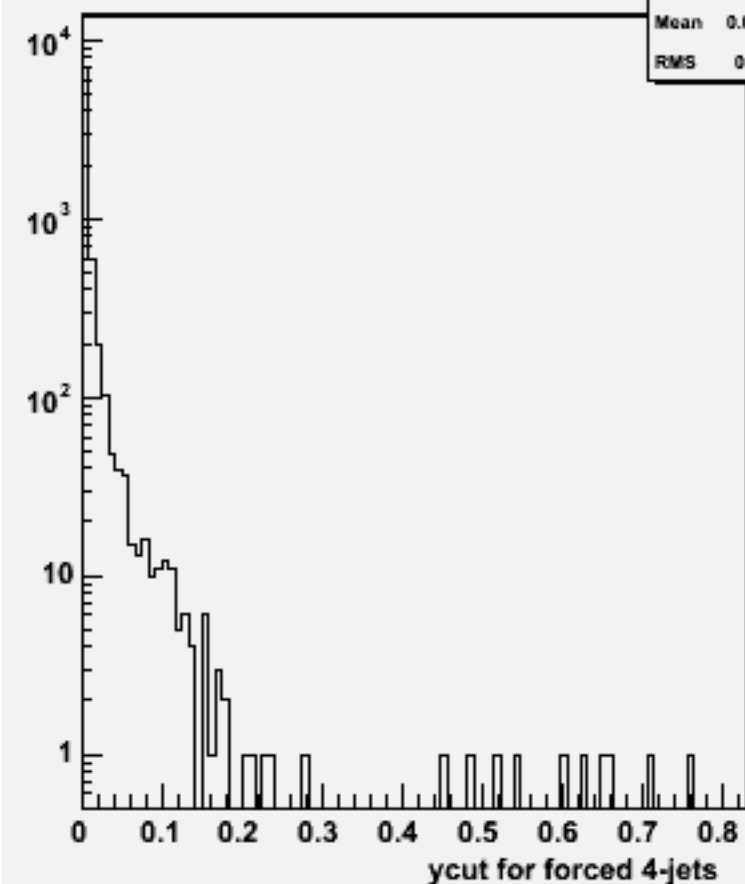
Ycut for 4-jets :w101845 n2n2n3n3cc_o
