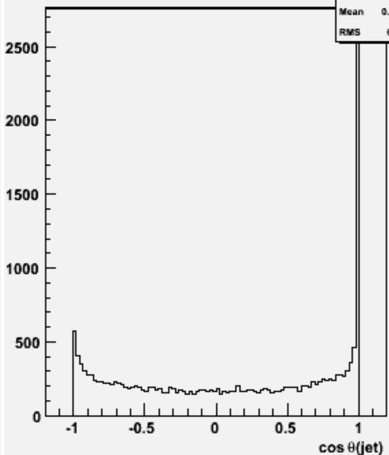
cos \theta for 2-jets :w101845 n2n2n3n3cc_o
