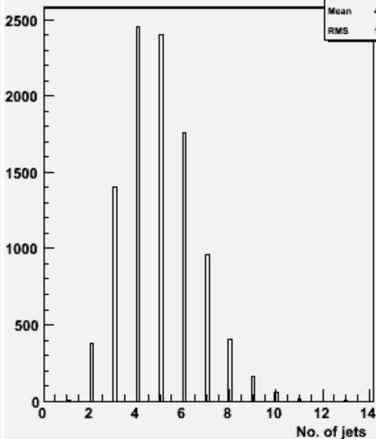
No. jets (ycut=0.001) : w101845 n2n2n3n3cc_o
