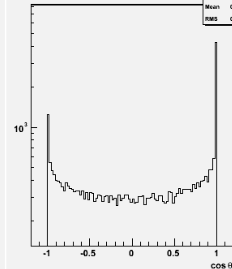
Jet cos \theta (All jets)w101845 n2n2n3n3cc_o
