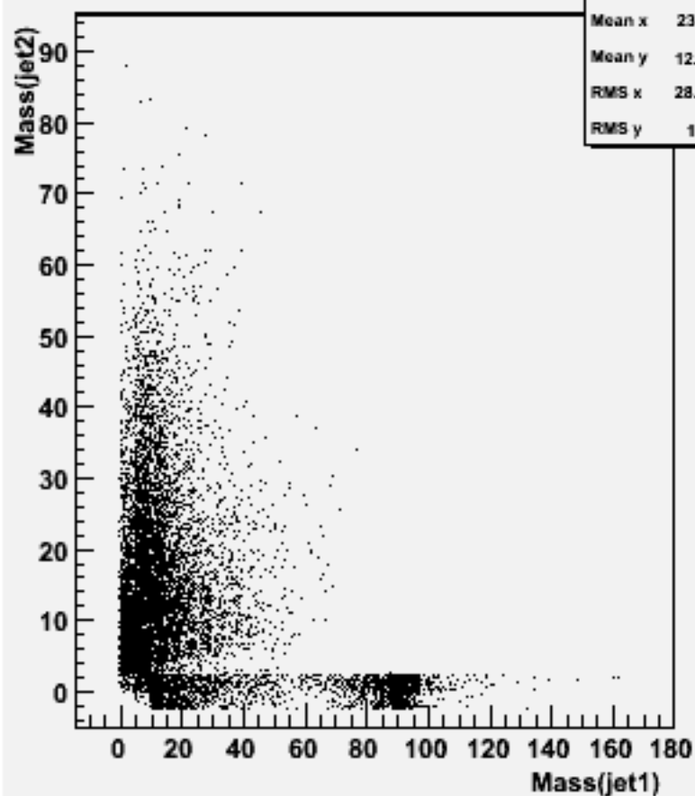
Jet mass for forced 2-jets : w101845 n2n2n3n3cc_o
