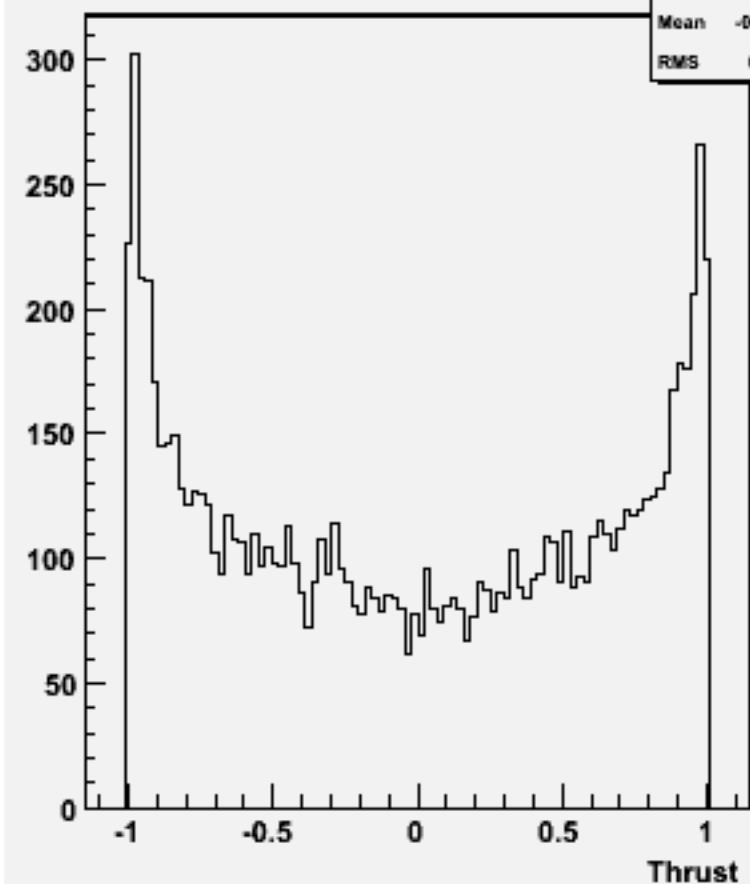
cos \Theta (thrust) w101845 n2n2n3n3cc_o
