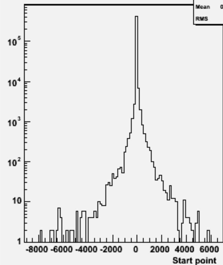
Start point Z : w101845 n2n2n3n3cc_o
