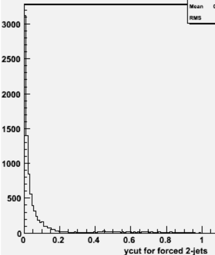
Ycut for 2-jets :w101845 n2n2n3n3cc_o
