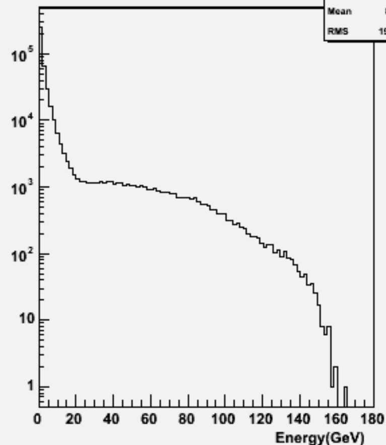
Start point R : w101845 n2n2n3n3cc_o
