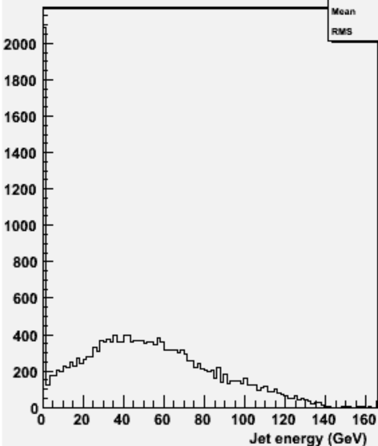
energy for 2-jets :w101845 n2n2n3n3cc_o
