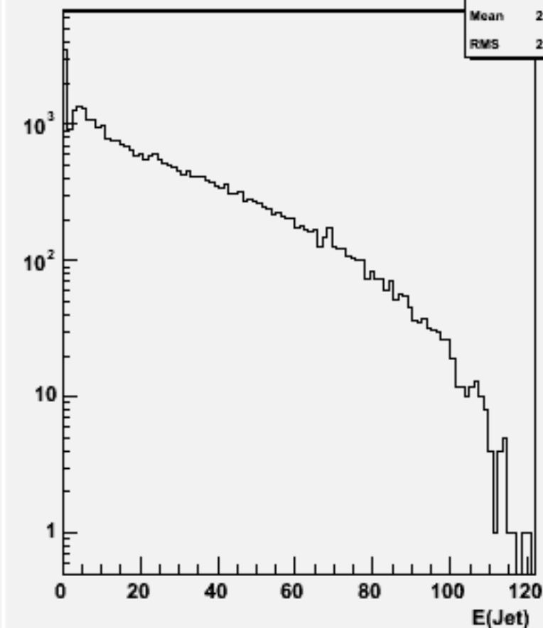
Jet energies(All jets)w101845 n2n2n3n3cc_o
