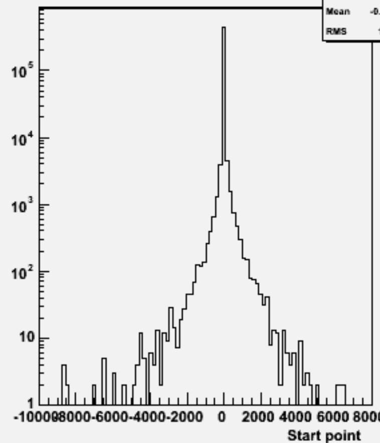
Start point Z : w101844 n2n2n3n3cc_o
