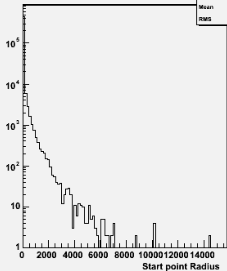
Start point R : w101844 n2n2n3n3cc_o
