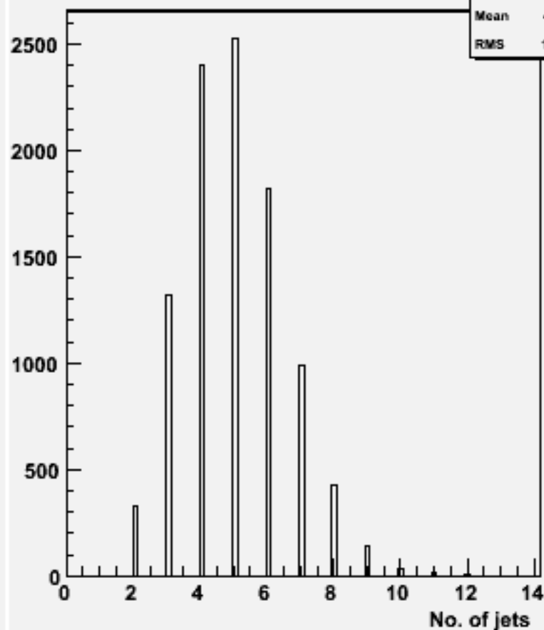
No. jets (ycut=0.001) : w101844 n2n2n3n3cc_o
