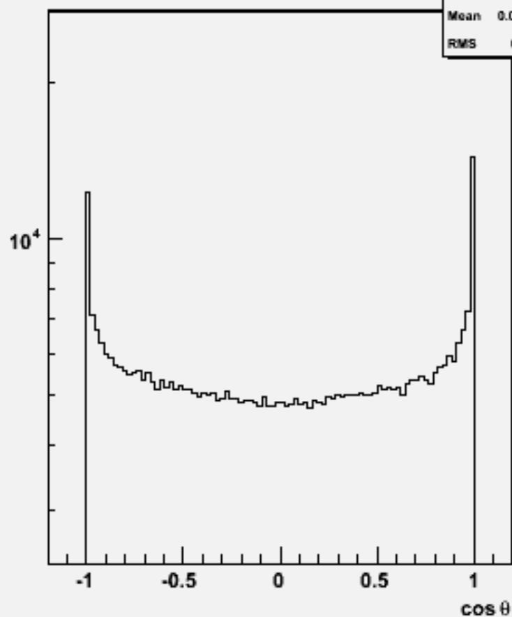
Particle cosθ : w101844 n2n2n3n3cc_o
