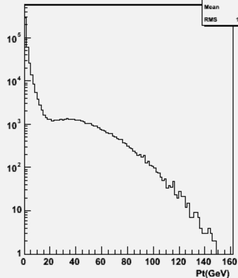
Particle Pt : w101844 n2n2n3n3cc_o
