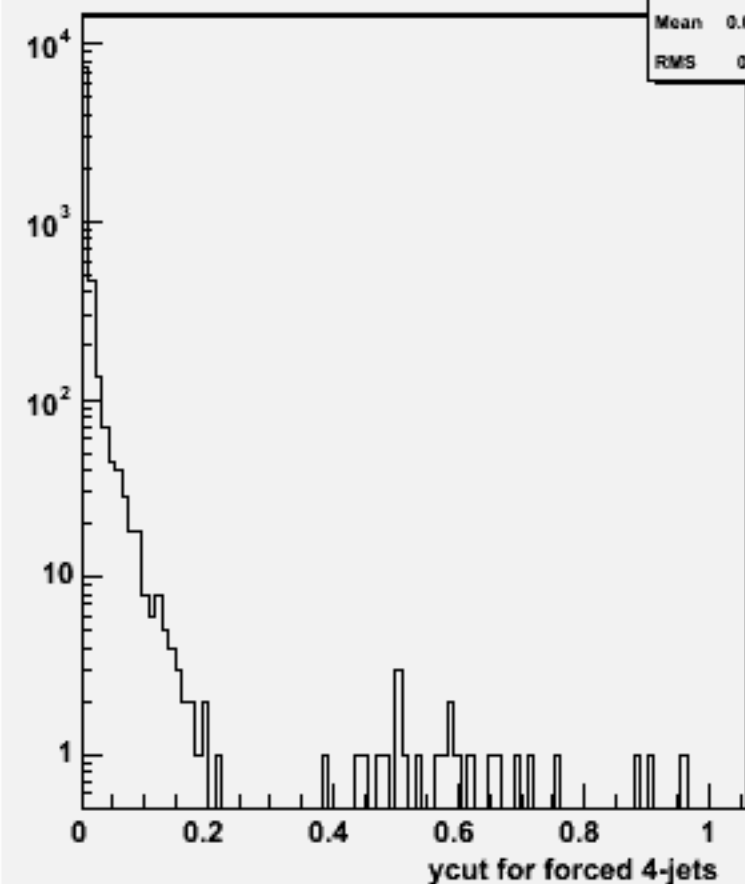
Ycut for 4-jets :w101844 n2n2n3n3cc_o
