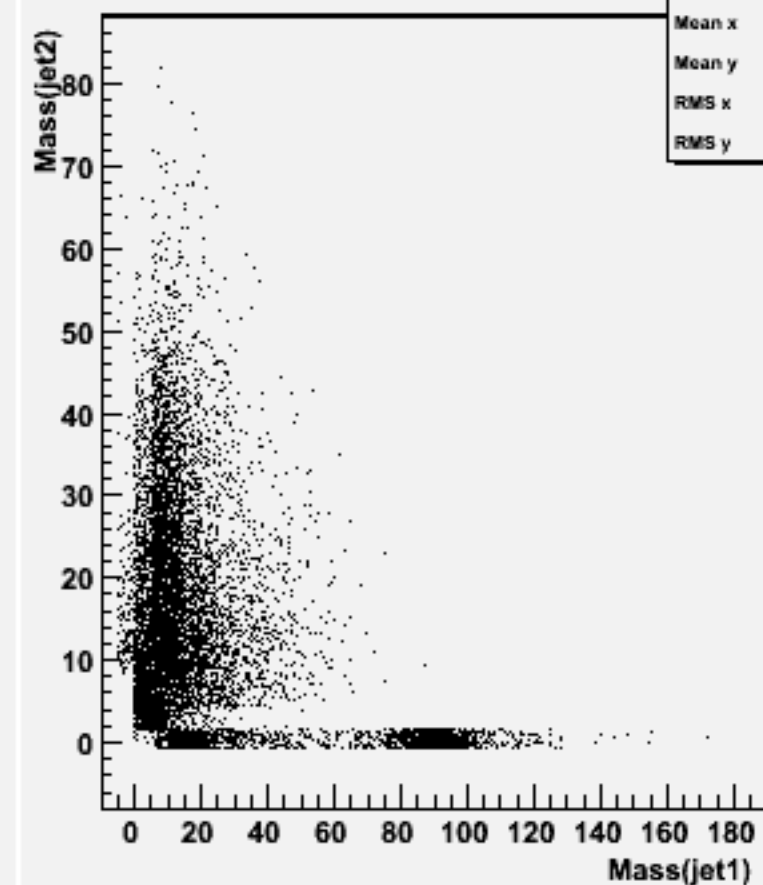
Jet mass for forced 2-jets : w101844 n2n2n3n3cc_o
