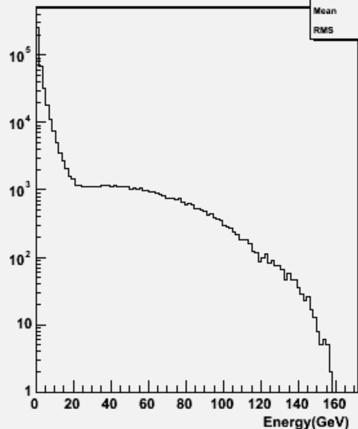
Particle Energy : w101844 n2n2n3n3cc_o
