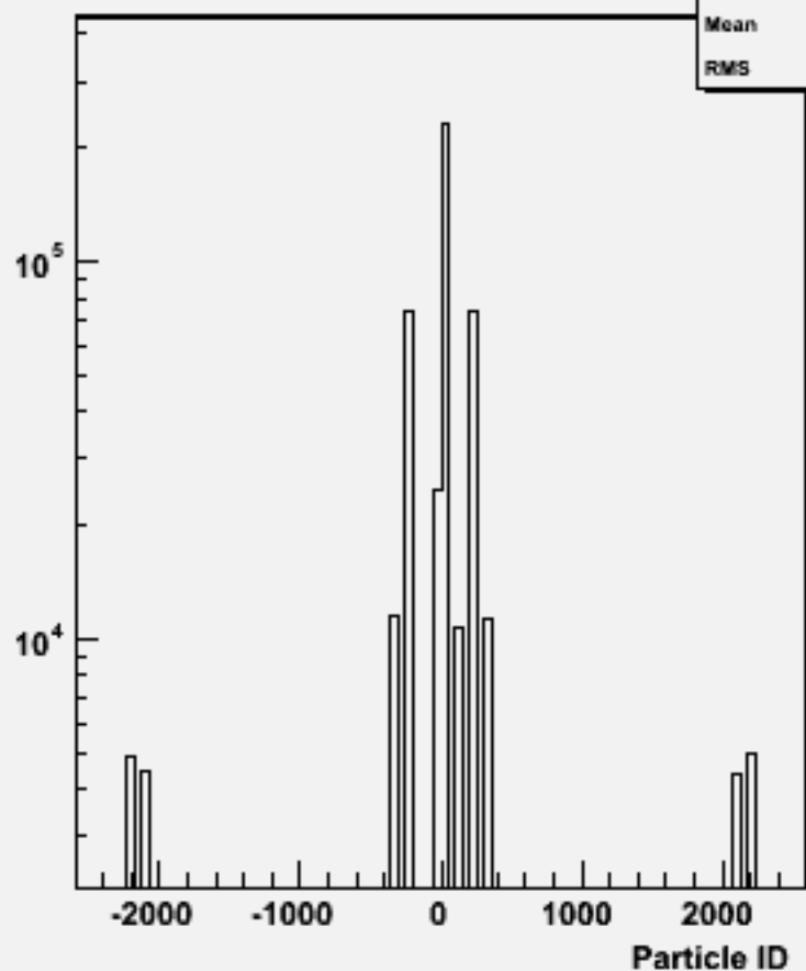
Particle ID : w101844 n2n2n3n3cc_o
