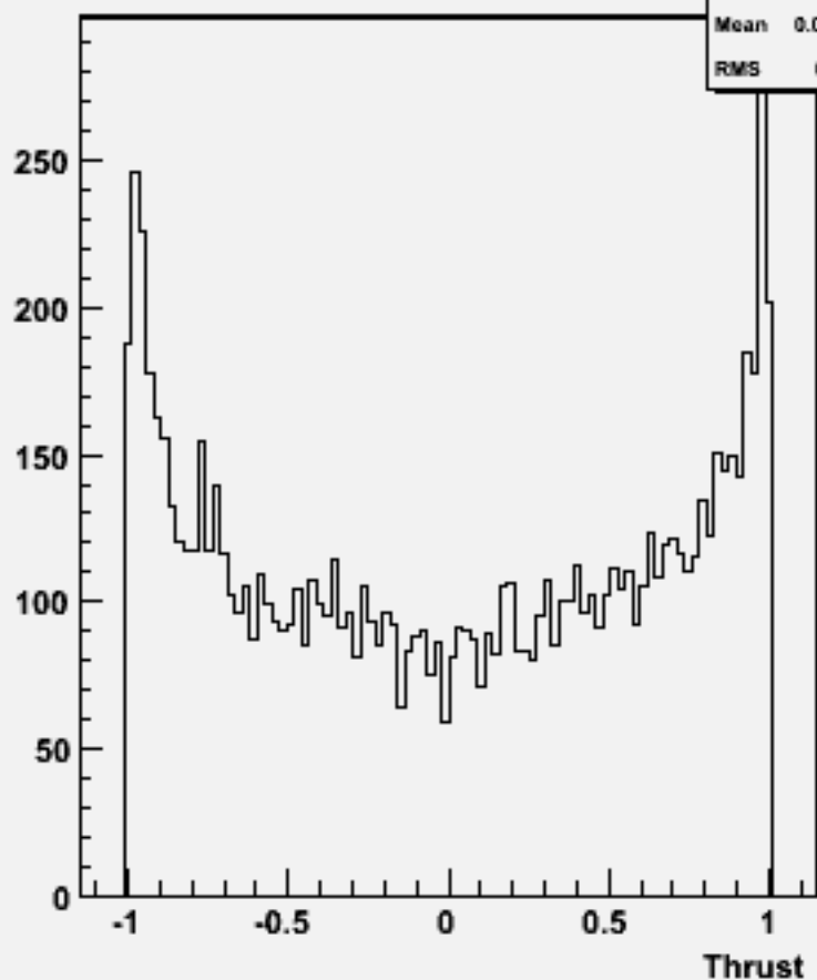
cos \Theta (thrust) w101844 n2n2n3n3cc_o
