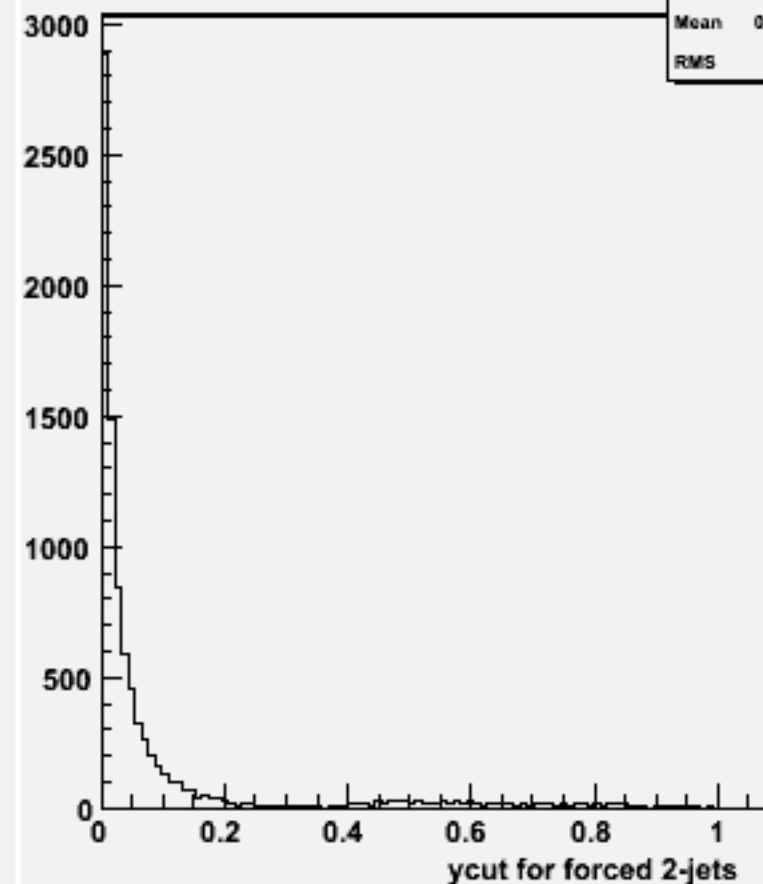
Ycut for 2-jets :w101844 n2n2n3n3cc_o
