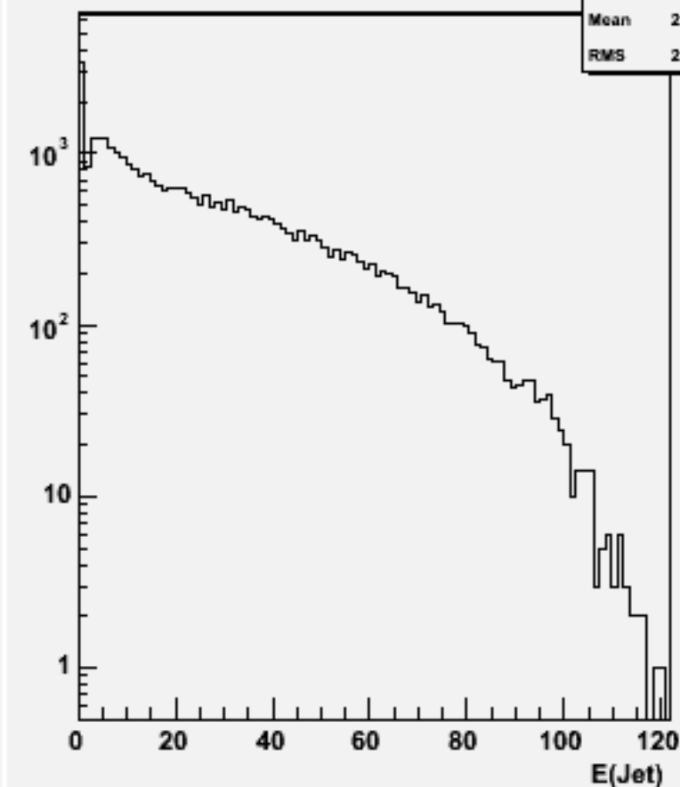
Jet energies(All jets)w101844 n2n2n3n3cc_o
