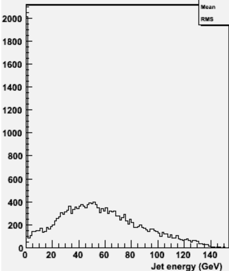
energy for 2-jets :w101844 n2n2n3n3cc_o
