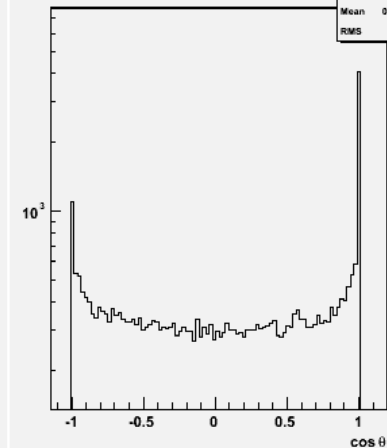
Jet cos \theta (All jets)w101844 n2n2n3n3cc_o
