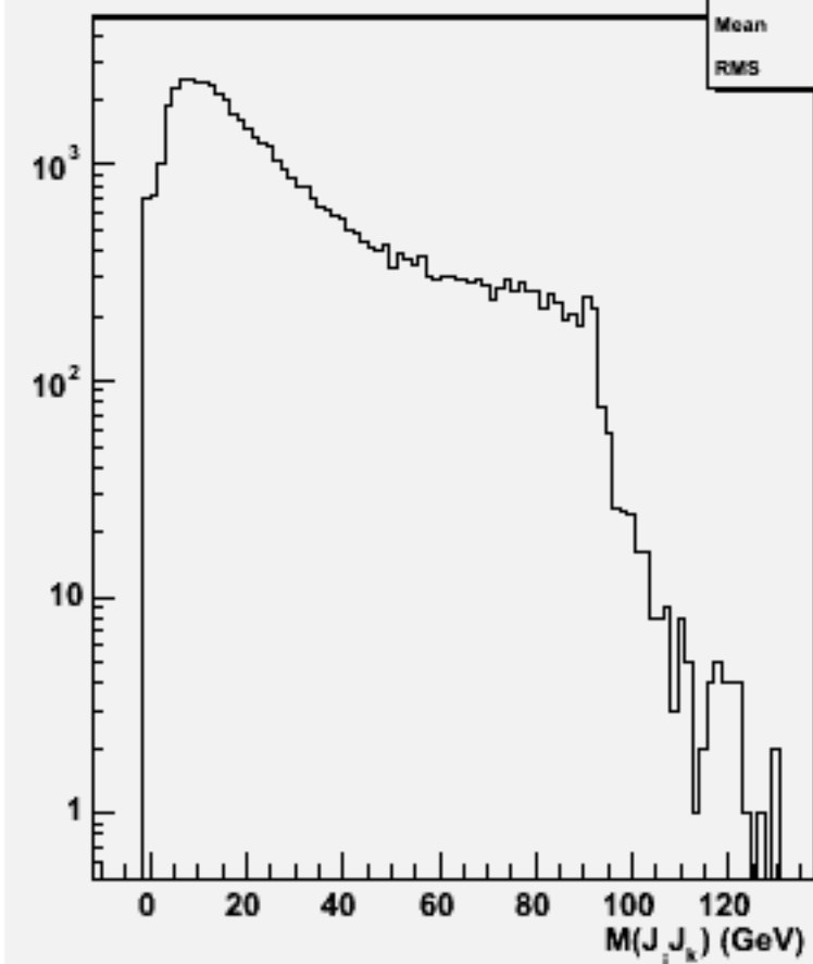
2jets mass(All comb)w101844 n2n2n3n3cc_o
