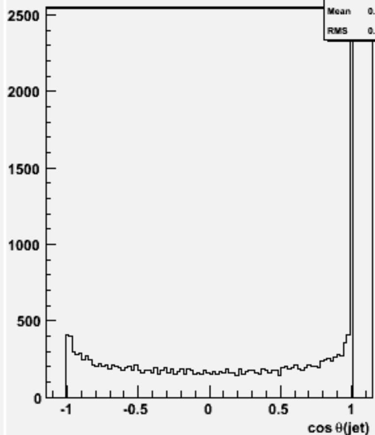
cos \theta for 2-jets :w101844 n2n2n3n3cc_o
