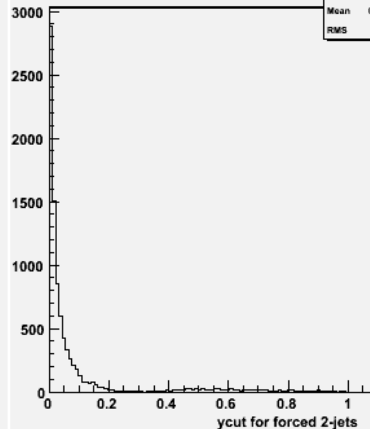
Ycut for 2-jets :w101840 n2n2n3n3uu_o
