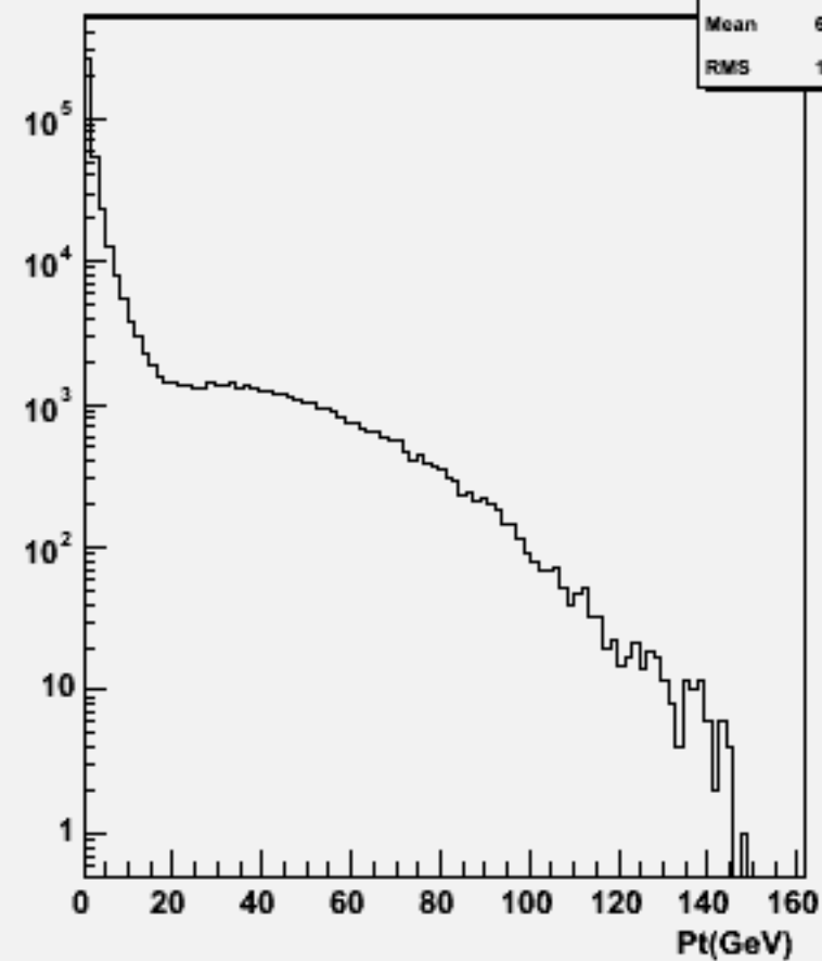
Particle Pt : w101840 n2n2n3n3uu_o
