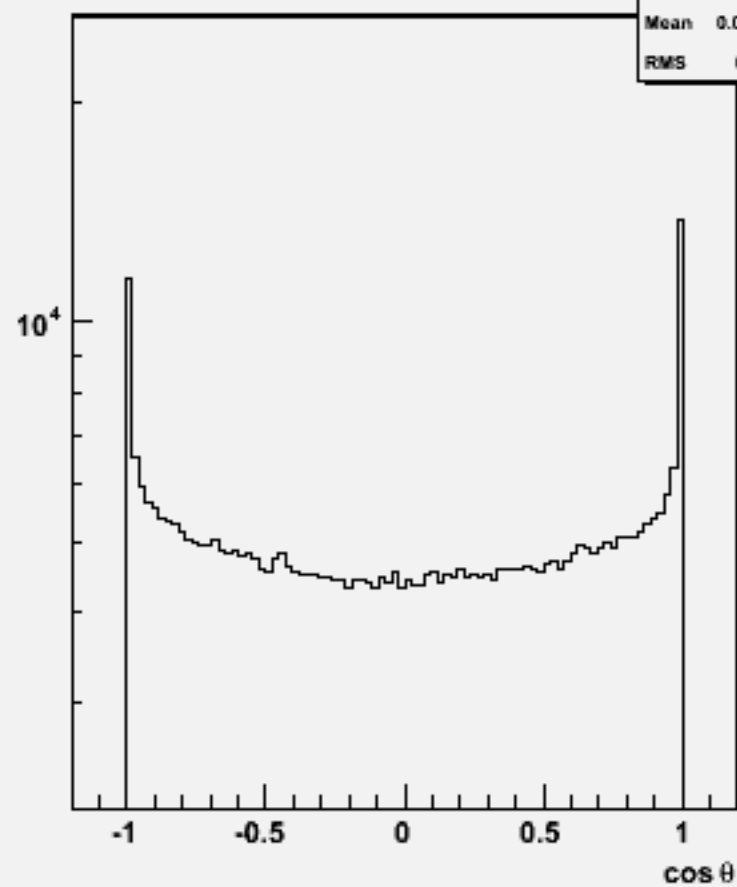
Particle cos \theta : w101840 n2n2n3n3uu_o
