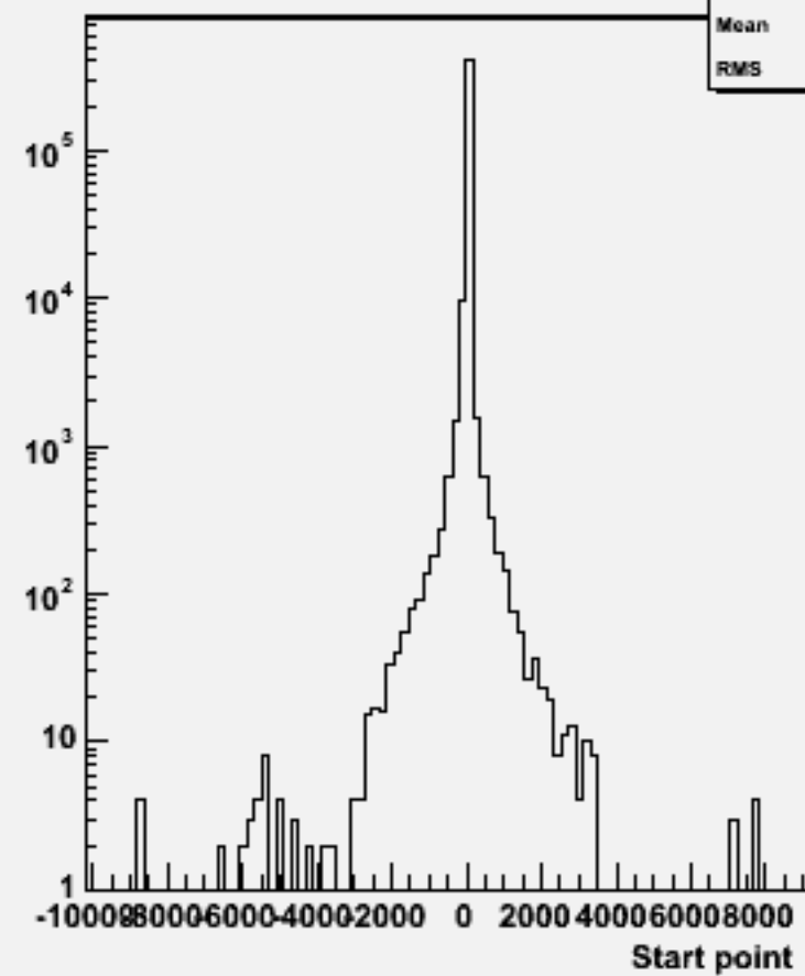
Start point Z : w101840 n2n2n3n3uu_o
