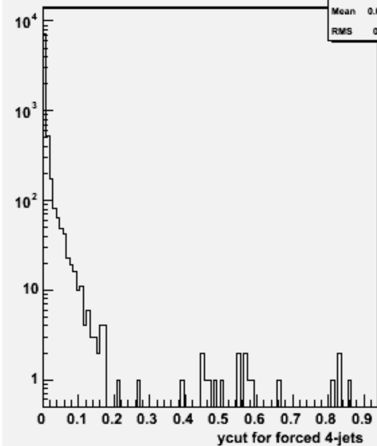
Ycut for 4-jets :w101840 n2n2n3n3uu_o
