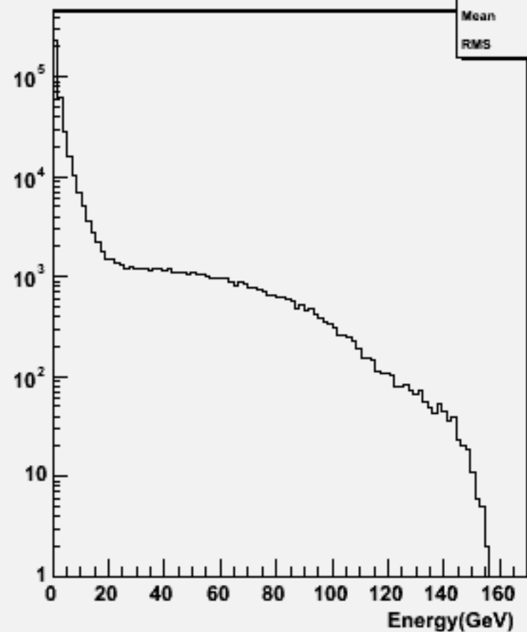
Particle Energy : w101840 n2n2n3n3uu_o
