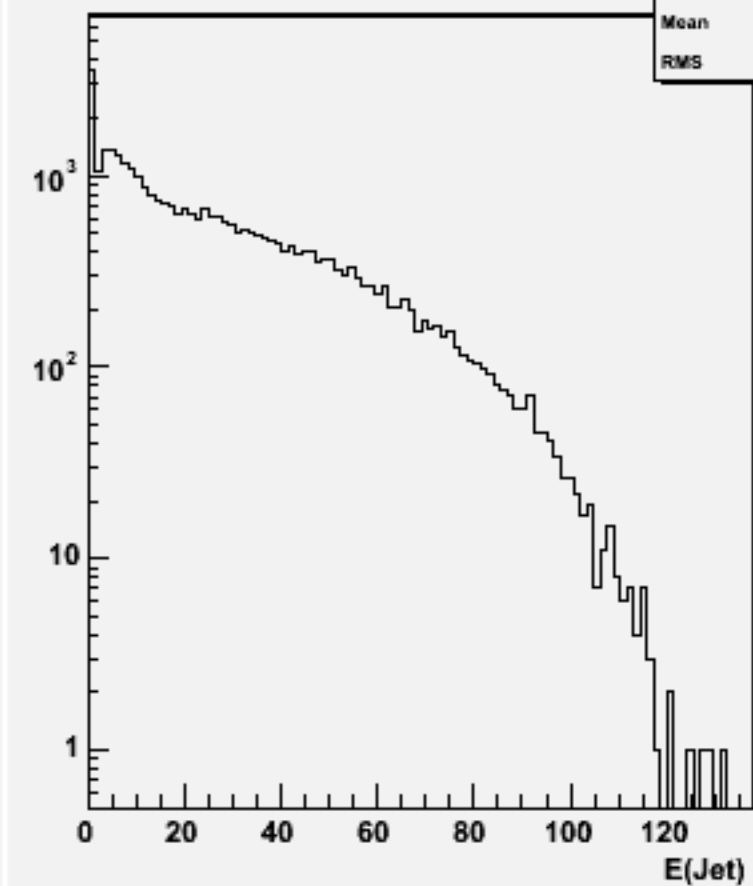
Jet energies(All jets)w101840 n2n2n3n3uu_o
