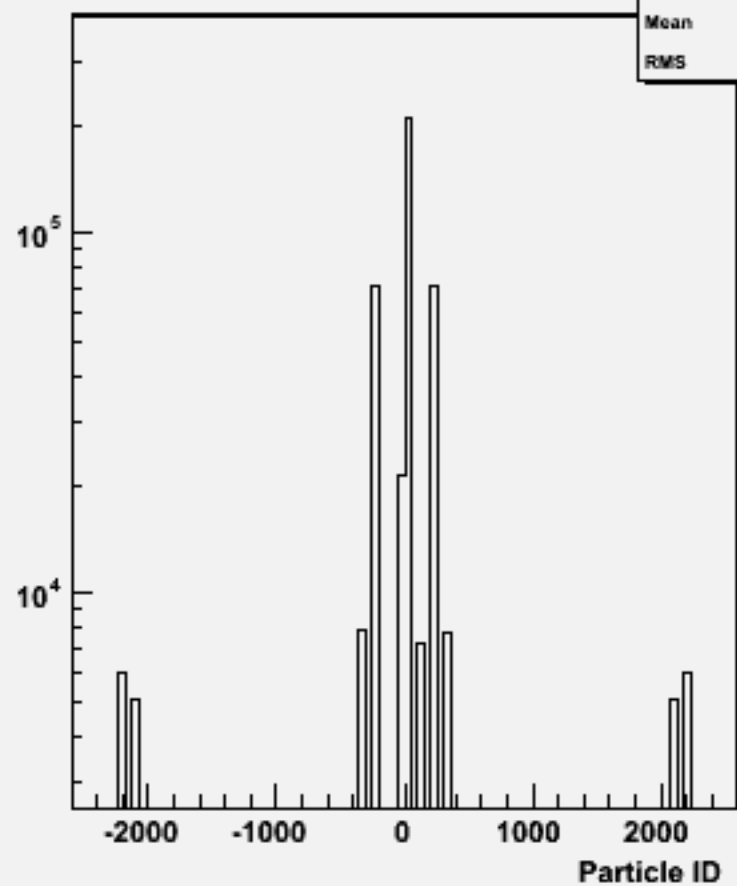
Particle ID : w101840 n2n2n3n3uu_o
