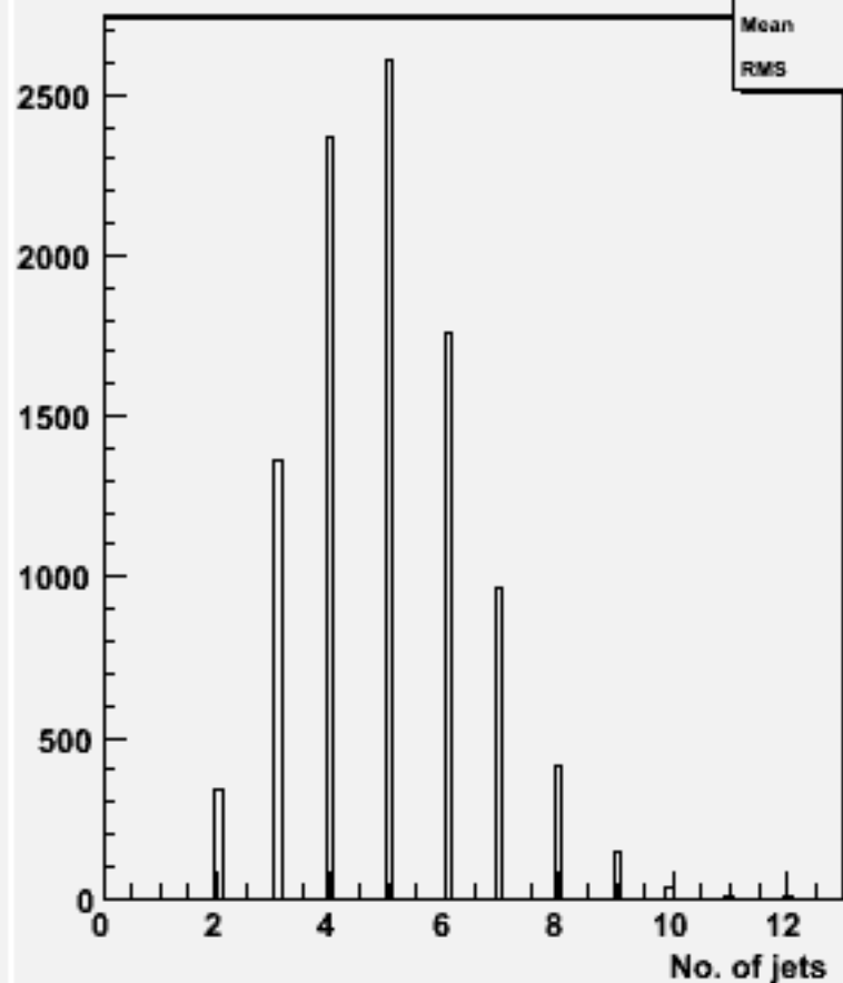
No. jets (ycut=0.001) : w101840 n2n2n3n3uu_o
