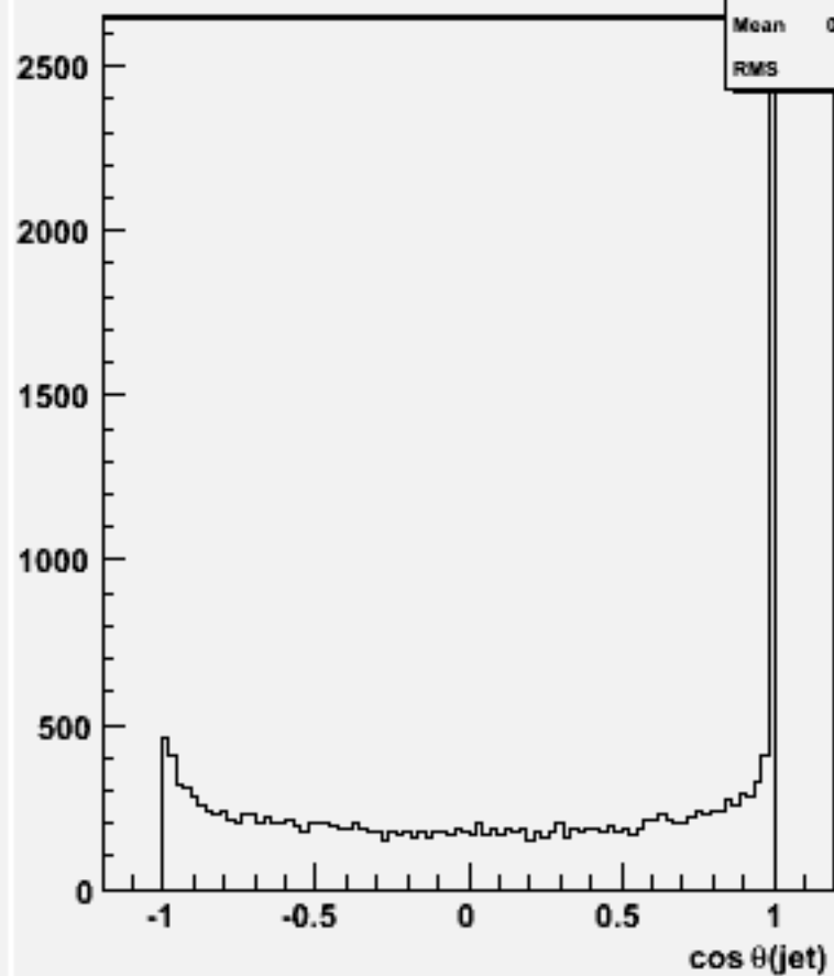
cos \theta for 2-jets :w101840 n2n2n3n3uu_o
