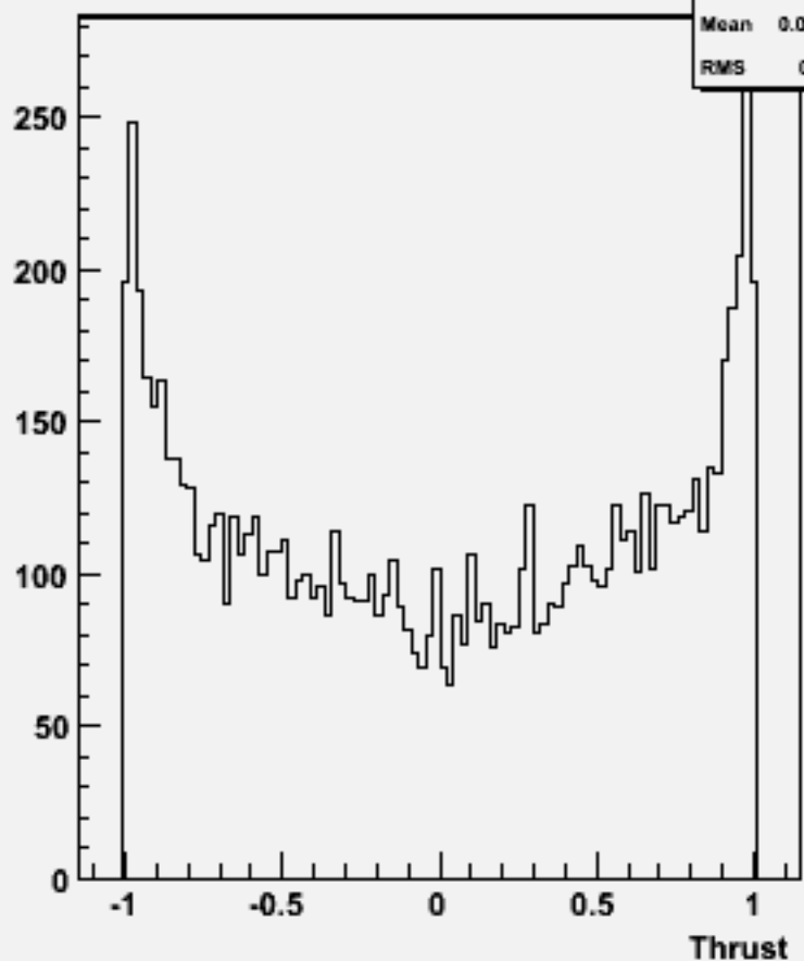
cos \Theta (thrust) w101840 n2n2n3n3uu_o
