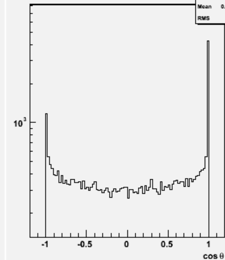
Jet cos \theta (All jets)w101840 n2n2n3n3uu_o
