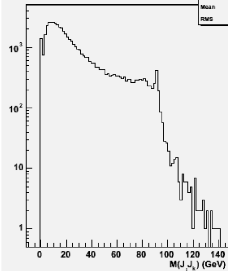
2jets mass(All comb)w101840 n2n2n3n3uu_o
