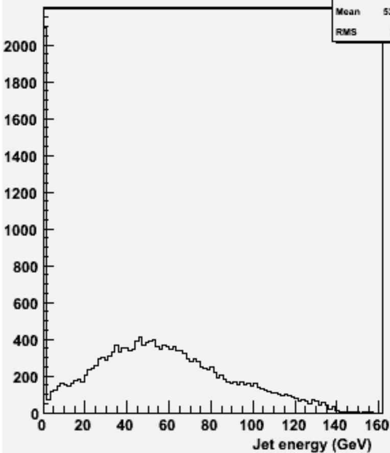
energy for 2-jets :w101840 n2n2n3n3uu_o
