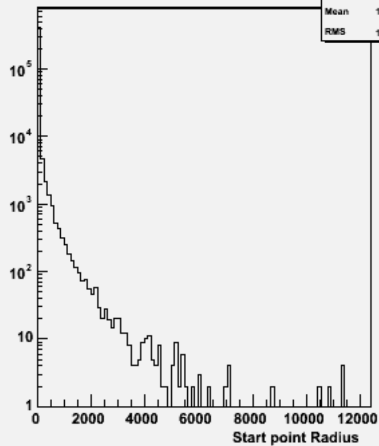
Start point R : w101840 n2n2n3n3uu_o
