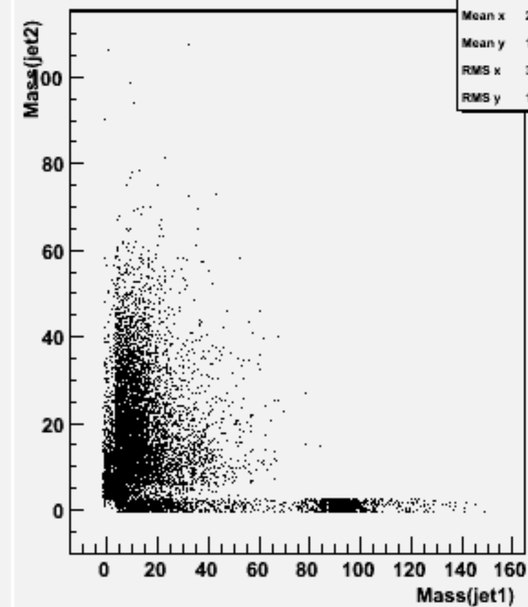
Jet mass for forced 2-jets : w101840 n2n2n3n3uu_o
