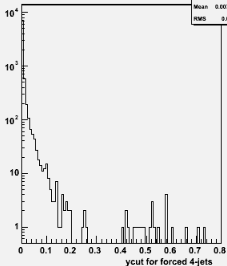
Ycut for 4-jets :w101836 n2n2n2n2cc_o
