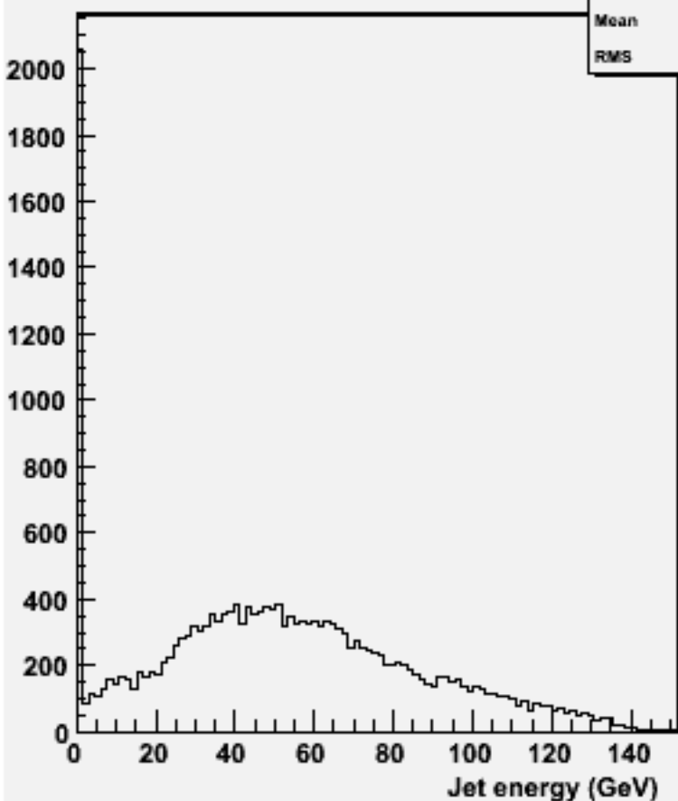
energy for 2-jets :w101836 n2n2n2n2cc_o
