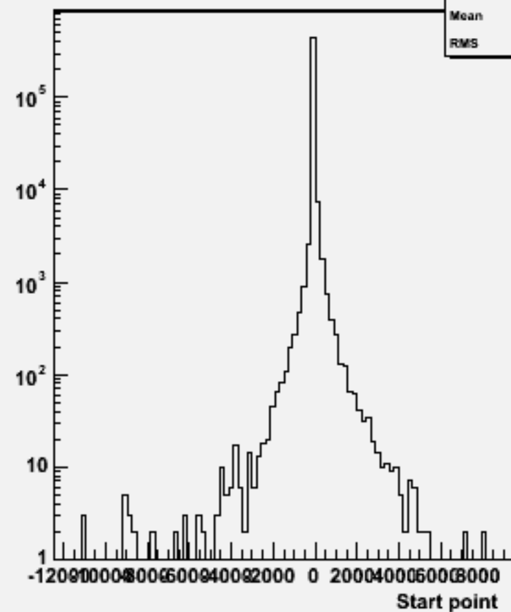
Start point Z : w101836 n2n2n2n2cc_o
