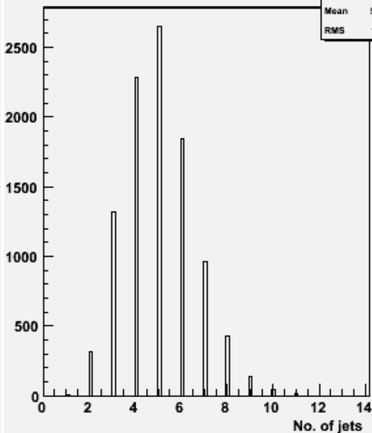
No. jets (ycut=0.001) : w101836 n2n2n2n2cc_o
