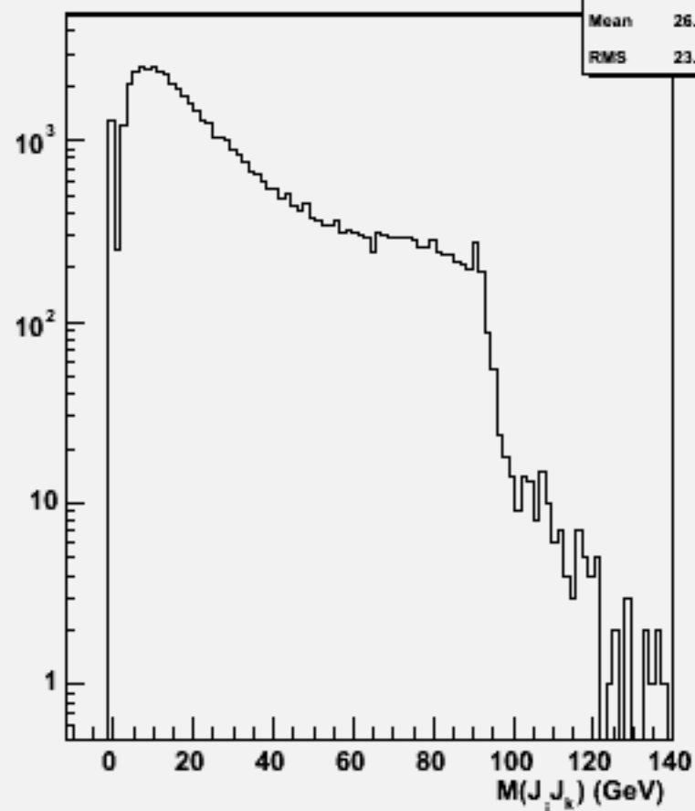
2jets mass(All comb)w101836 n2n2n2n2cc_o
