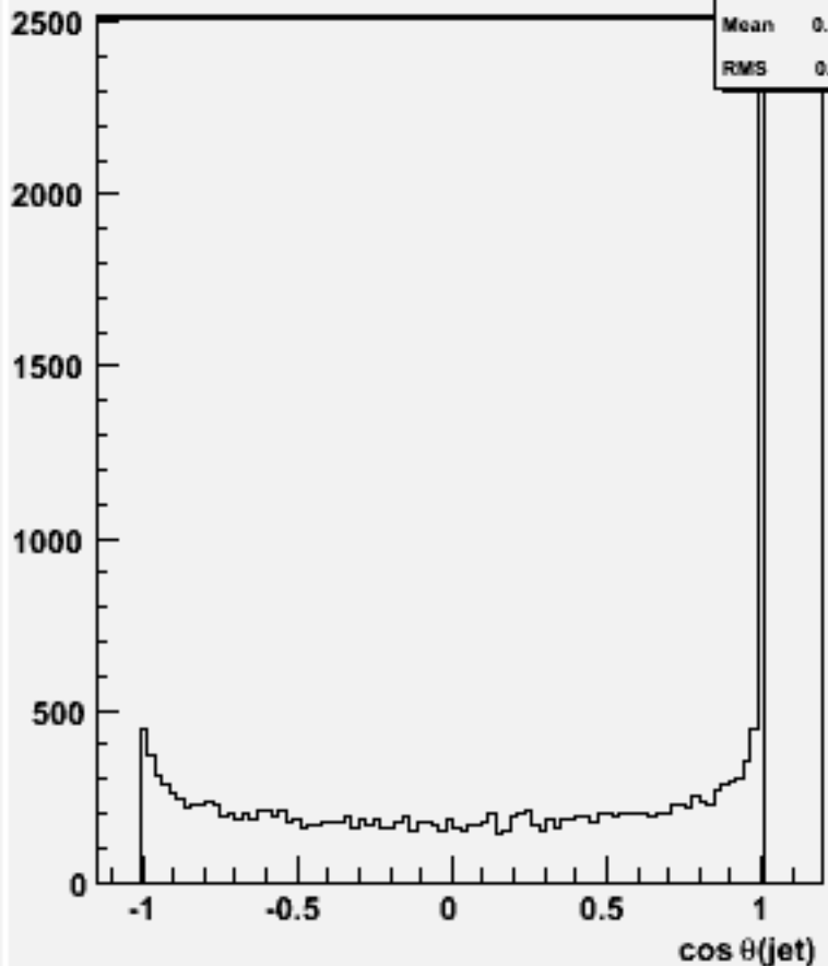
cos \theta for 2-jets :w101836 n2n2n2n2cc_o
