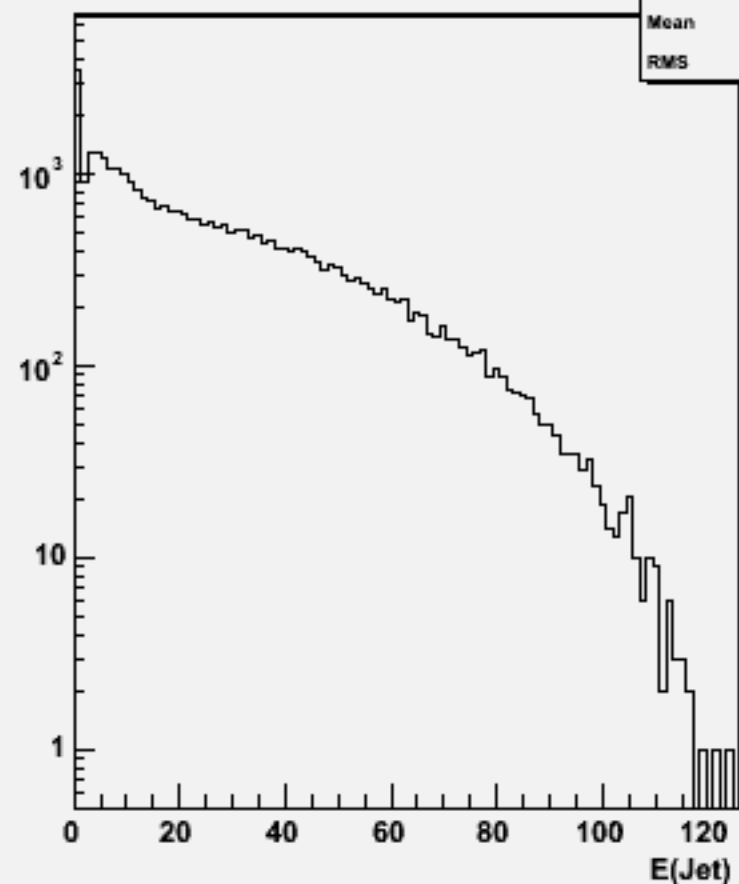
Jet energies(All jets)w101836 n2n2n2n2cc_o
