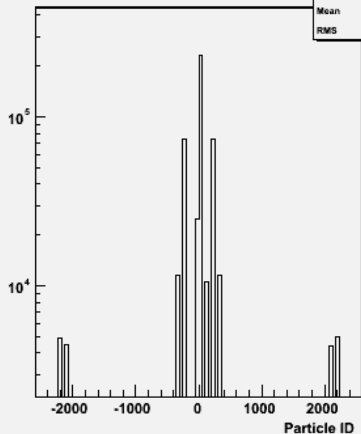
Particle ID : w101836 n2n2n2n2cc_o
