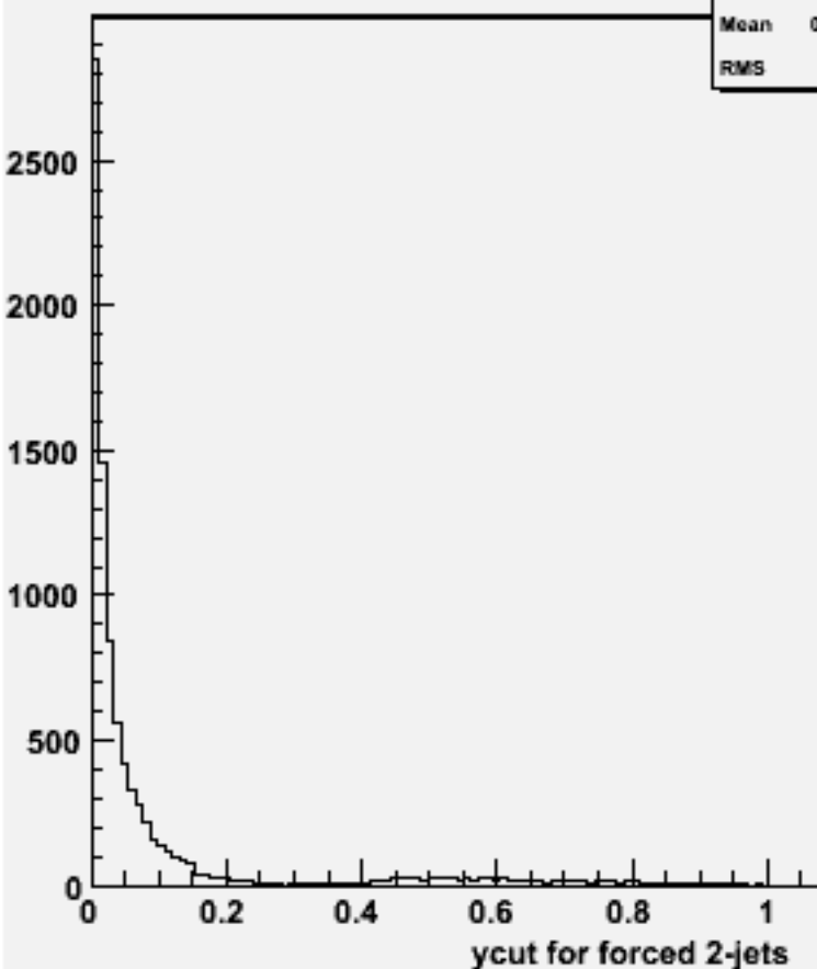
Ycut for 2-jets :w101836 n2n2n2n2cc_o
