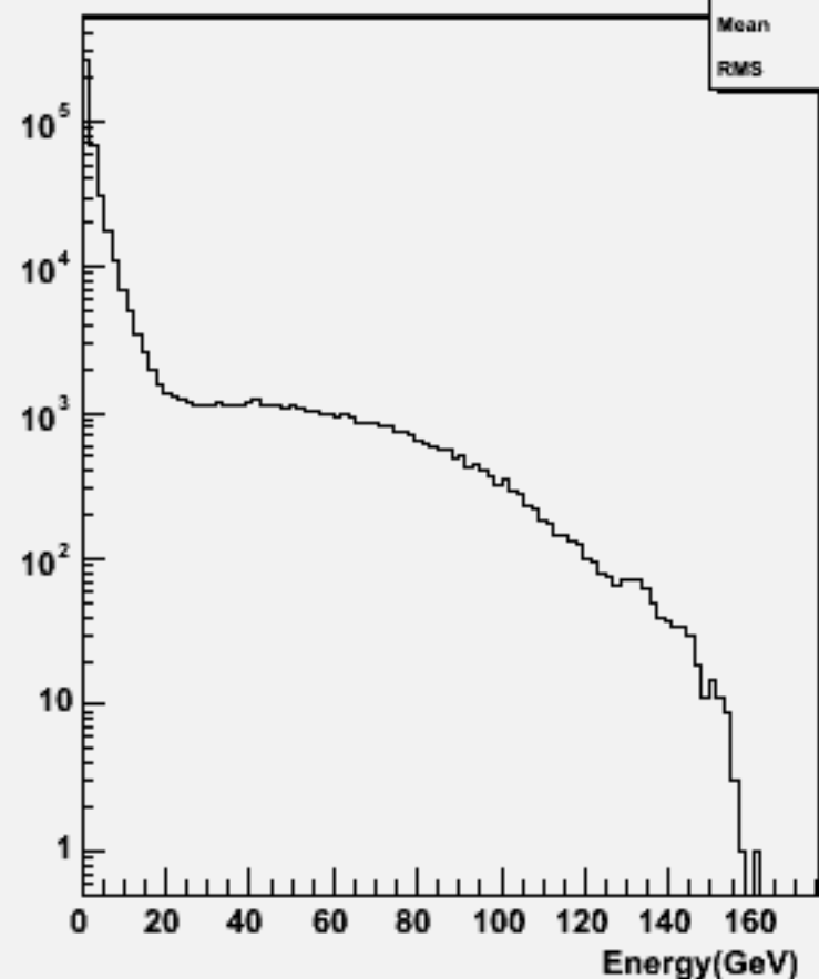
Particle Energy : w101836 n2n2n2n2cc_o
