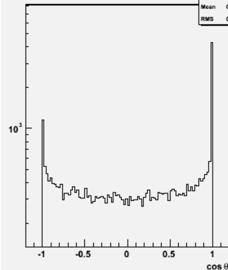
Jet cos \theta (All jets)w101836 n2n2n2n2cc_o
