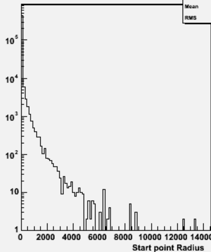
Start point R : w101836 n2n2n2n2cc_o
