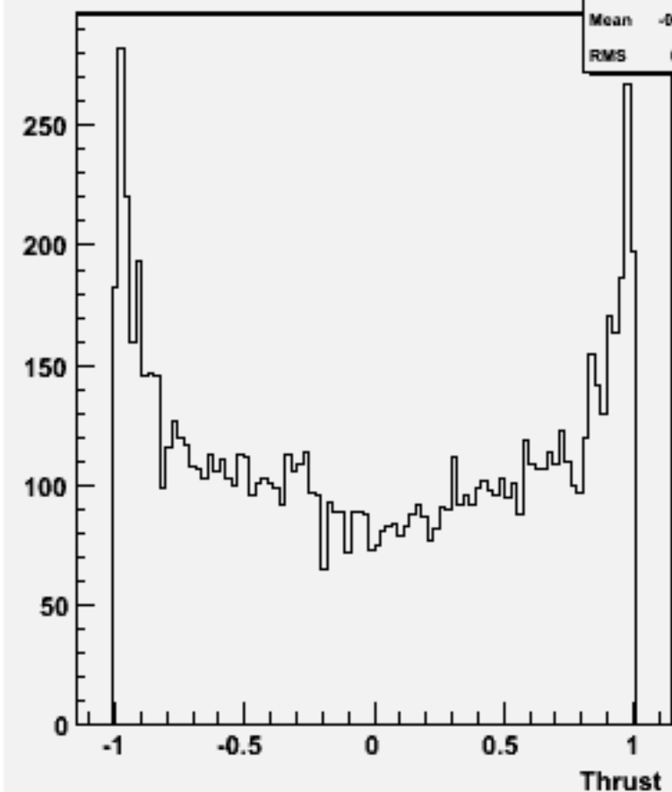
cos \Theta (thrust) w101836 n2n2n2n2cc_o
