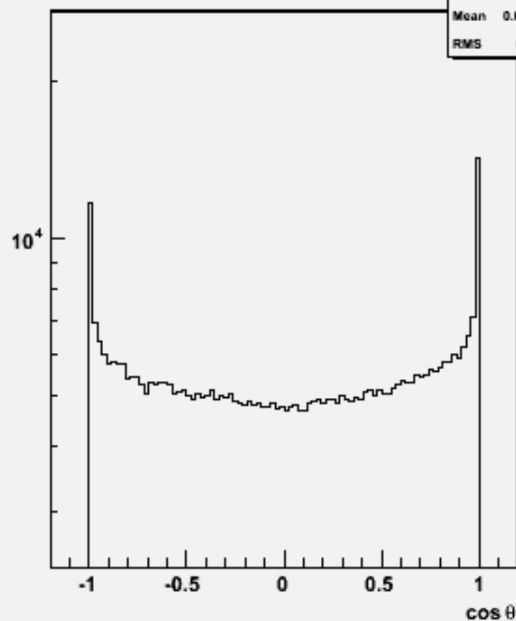
Particle cos \theta : w101836 n2n2n2n2cc_o
