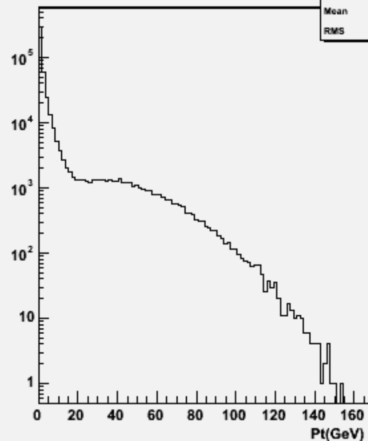
Particle Pt : w101836 n2n2n2n2cc_o
