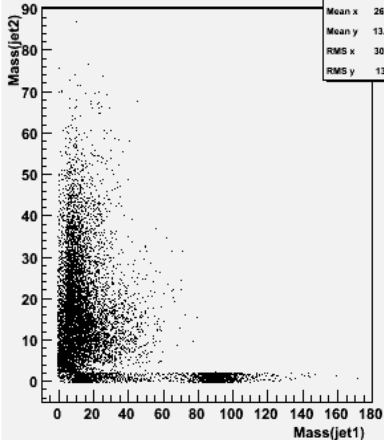
Jet mass for forced 2-jets : w101836 n2n2n2n2cc_o
