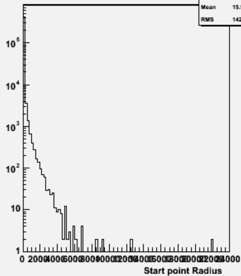
Start point R : w101832 n2n2n2n2uu_o
