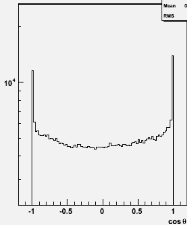
Particle cos \theta : w101832 n2n2n2n2uu_o
