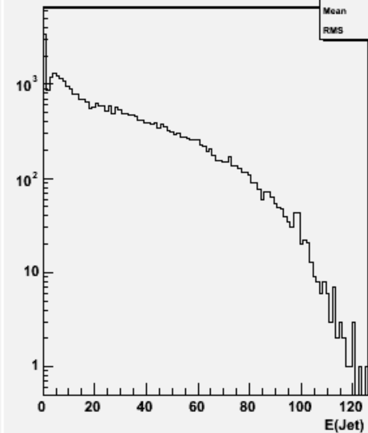
Jet energies(All jets)w101832 n2n2n2n2uu_o
