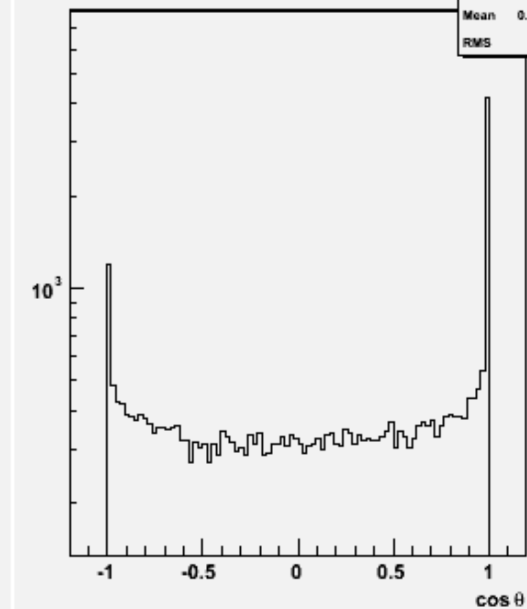
Jet cos \theta (All jets)w101832 n2n2n2n2uu_o
