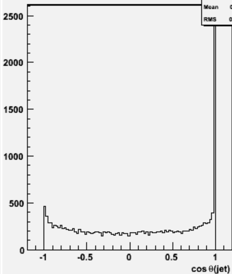
cos \theta for 2-jets :w101832 n2n2n2n2uu_o
