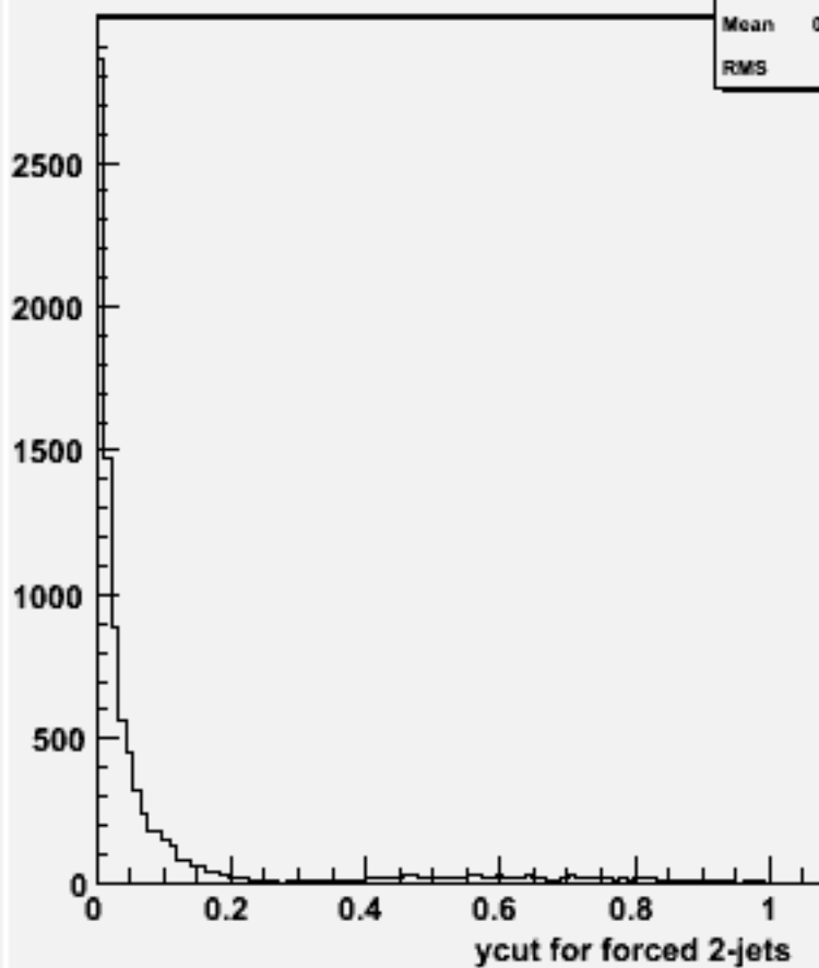
Ycut for 2-jets :w101832 n2n2n2n2uu_o
