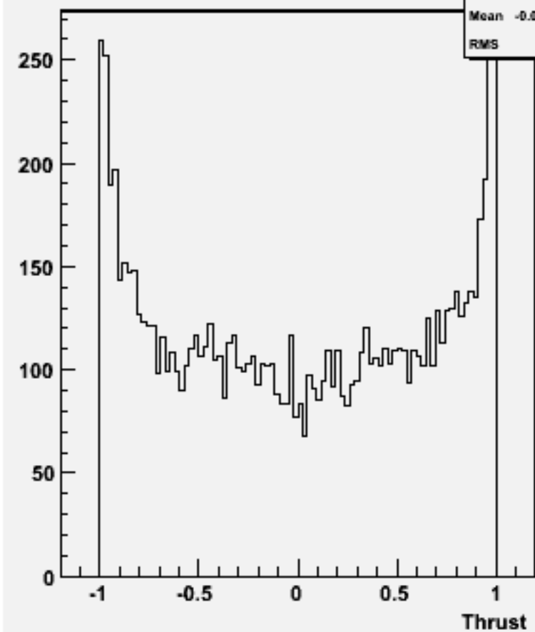
cos \Theta (thrust) w101832 n2n2n2n2uu_o
