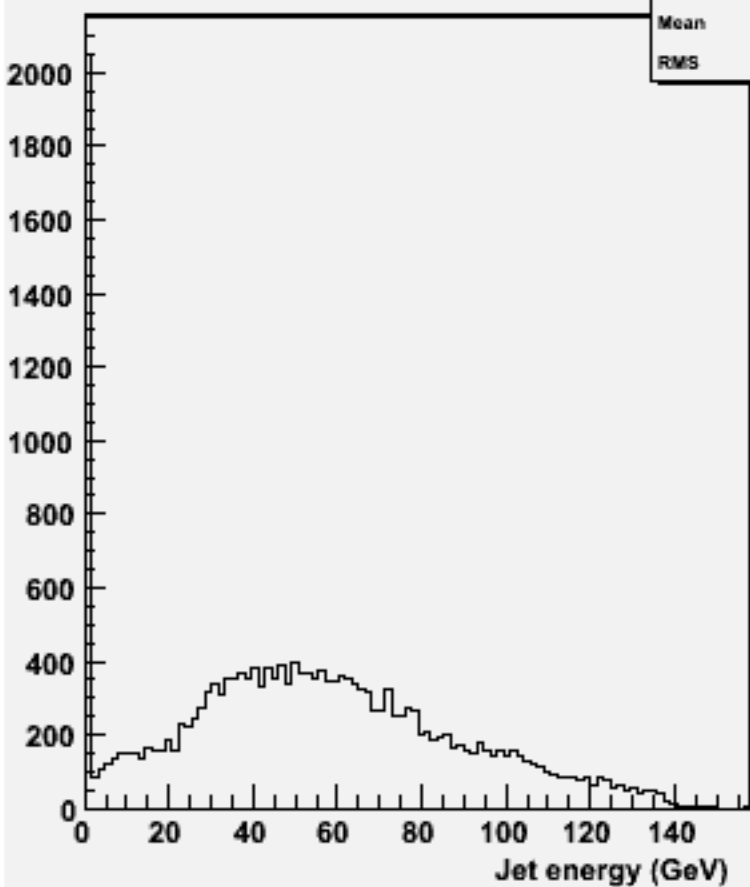
energy for 2-jets :w101832 n2n2n2n2uu_o
