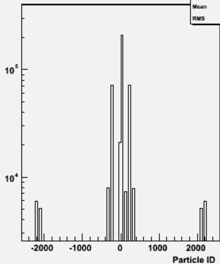
Particle ID : w101832 n2n2n2n2uu_o
