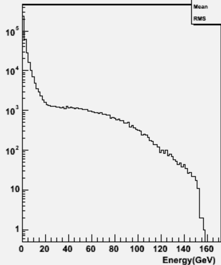
Particle Energy : w101832 n2n2n2n2uu_o
