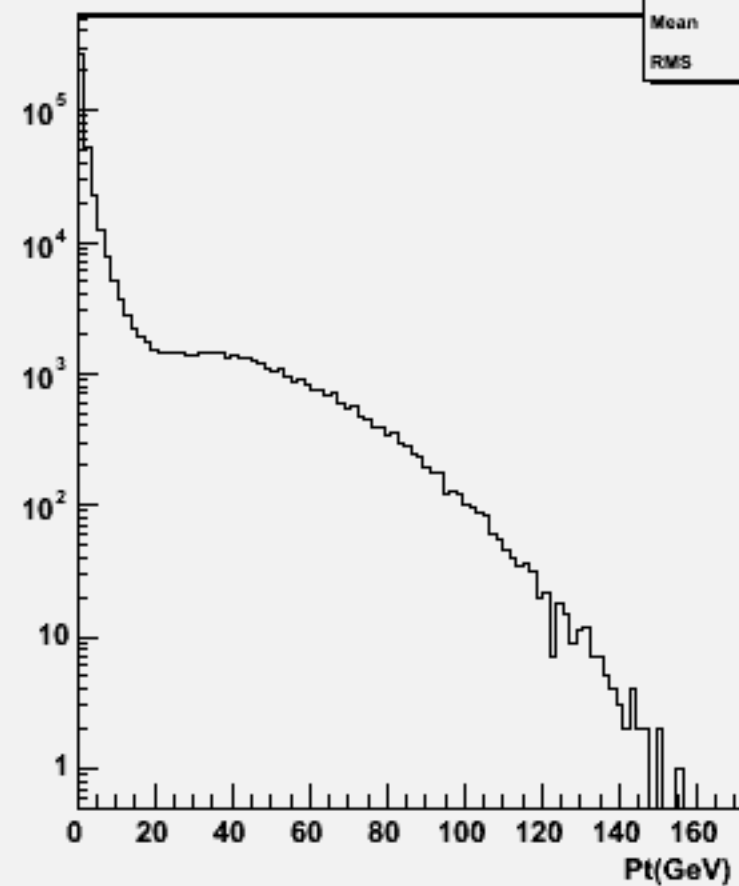
Particle Pt : w101832 n2n2n2n2uu_o
