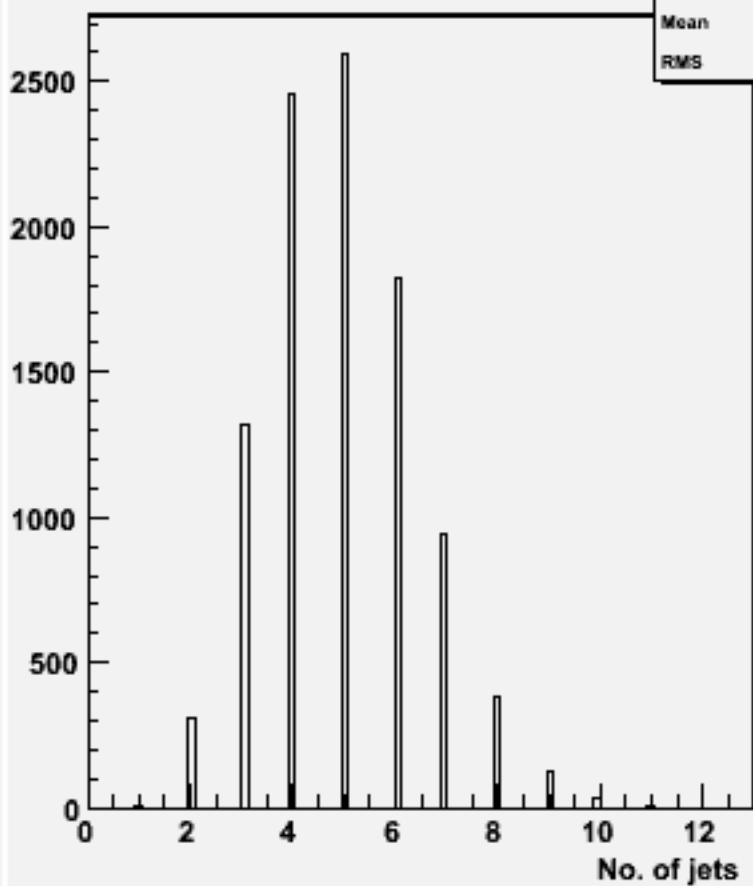
No. jets (ycut=0.001) : w101832 n2n2n2n2uu_o
