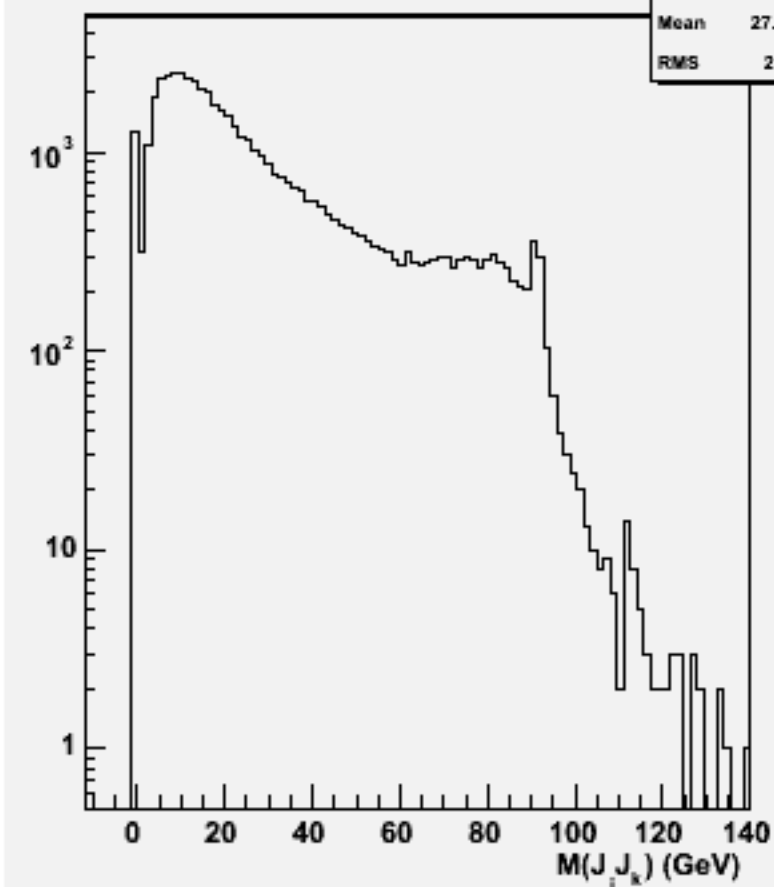
2jets mass(All comb)w101832 n2n2n2n2uu_o
