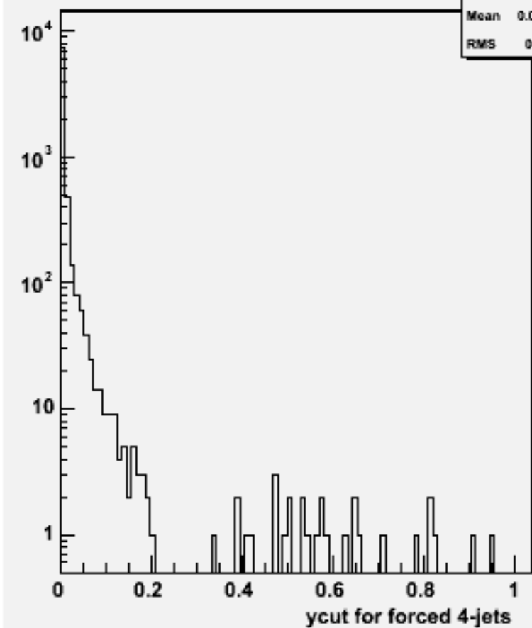
Ycut for 4-jets :w101832 n2n2n2n2uu_o
