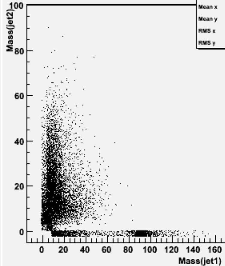
Jet mass for forced 2-jets : w101832 n2n2n2n2uu_o
