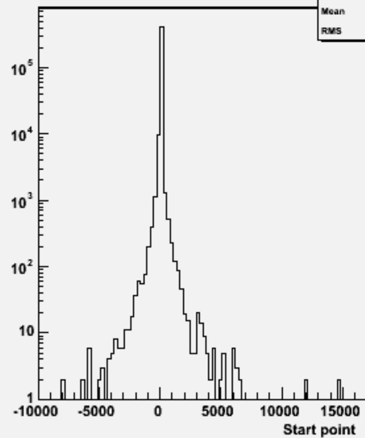
Start point Z : w101832 n2n2n2n2uu_o
