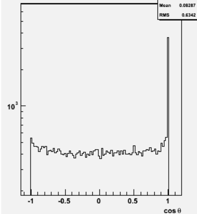
Jet cosθ (All jets)w101828 n1n1cccc_o
