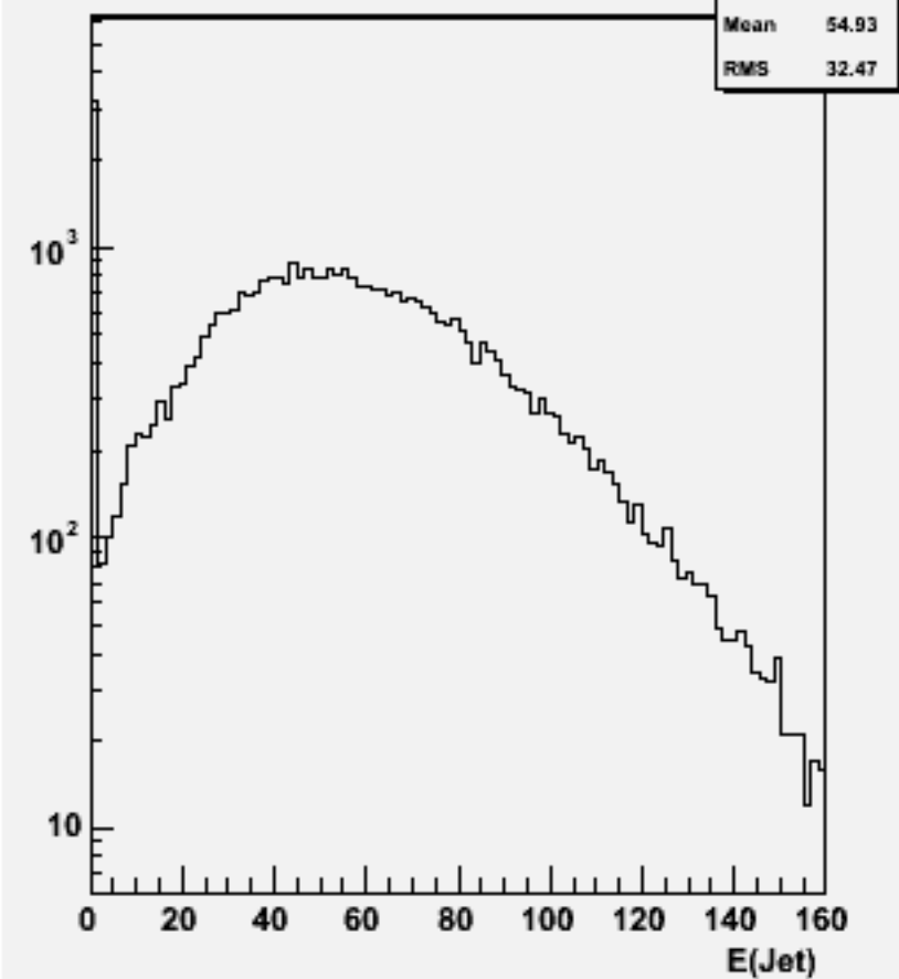
Jet energies(All jets)w101828 n1n1cccc_o
