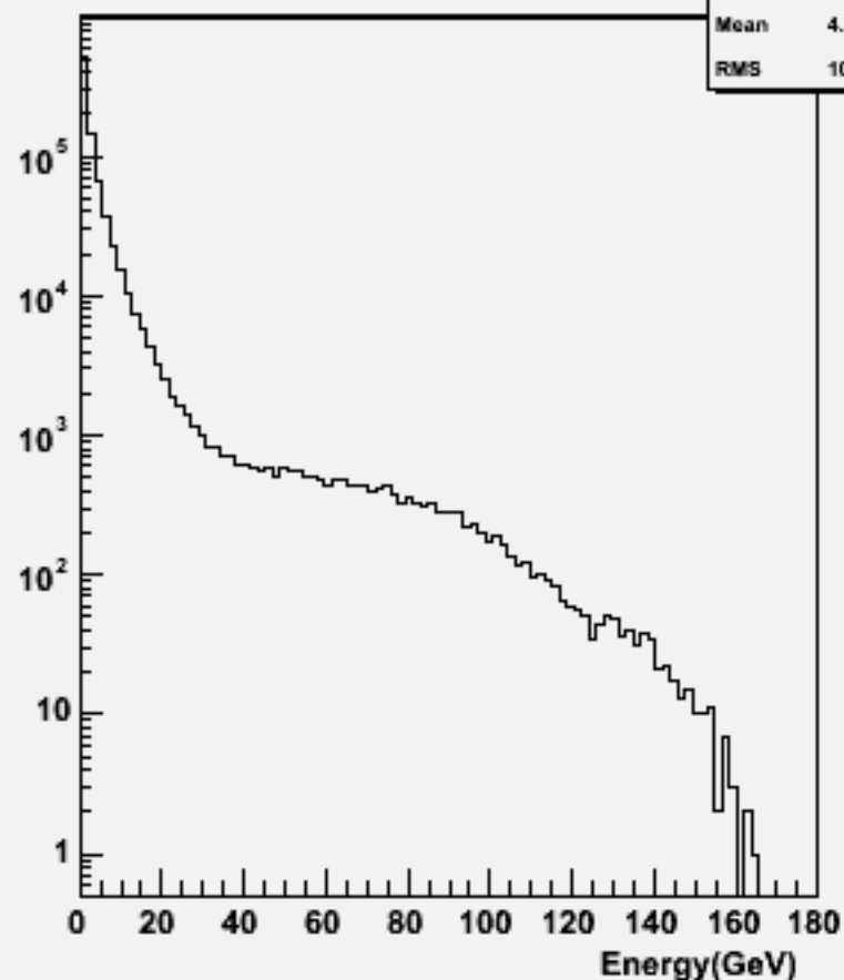
Particle Energy : w101828 n1n1cccc_o
