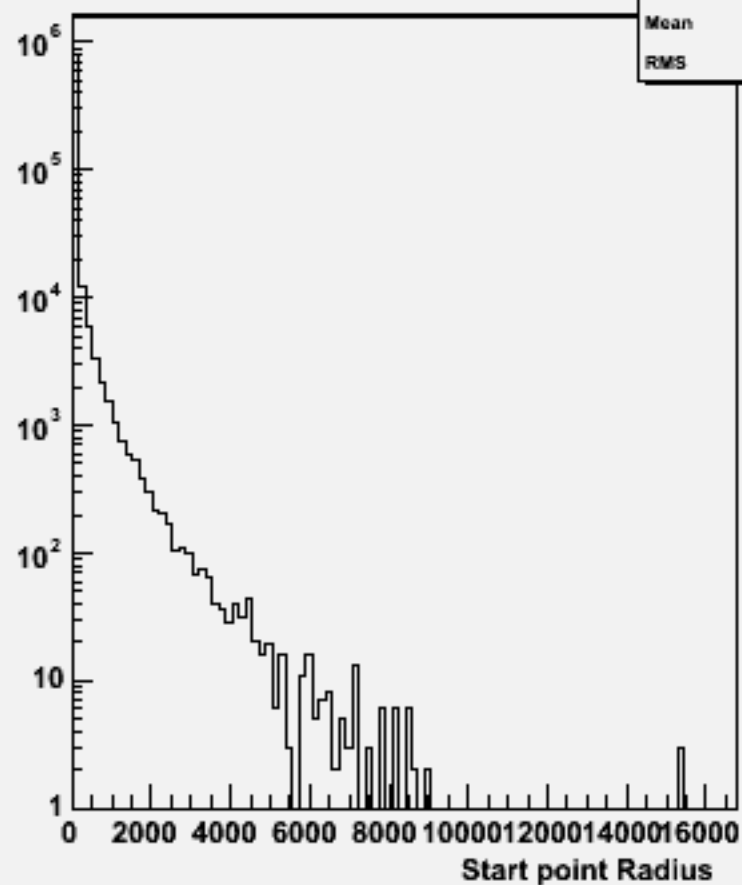
Start point R : w101828 n1n1cccc_o
