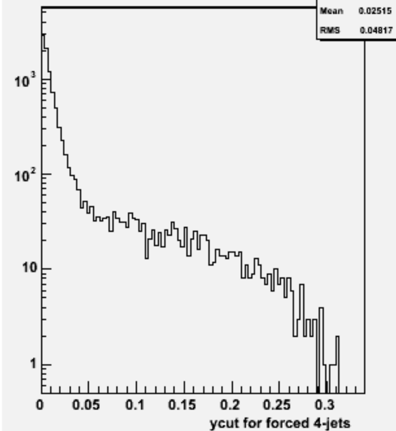
Ycut for 4-jets :w101828 n1n1cccc_o
