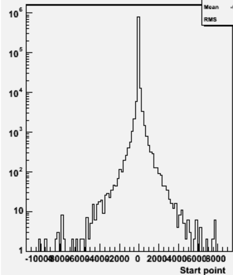
Start point Z : w101828 n1n1cccc_o
