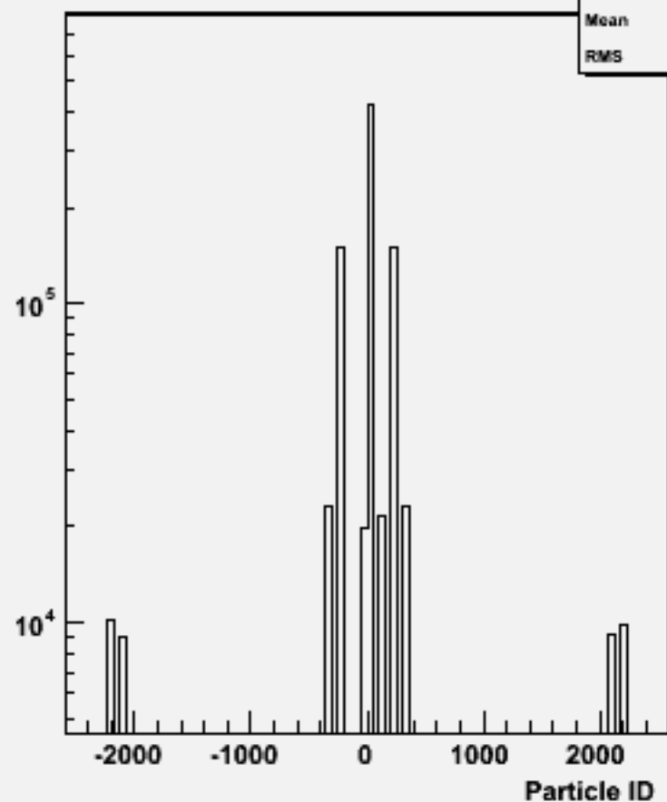
Particle ID : w101828 n1n1cccc_o
