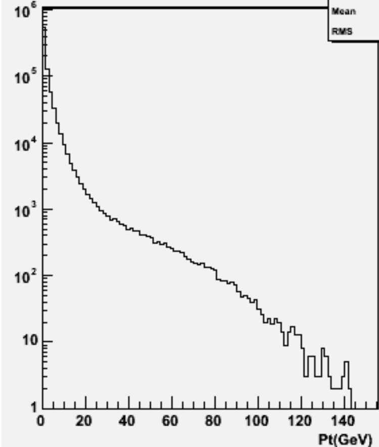
Particle Pt : w101828 n1n1cccc_o
