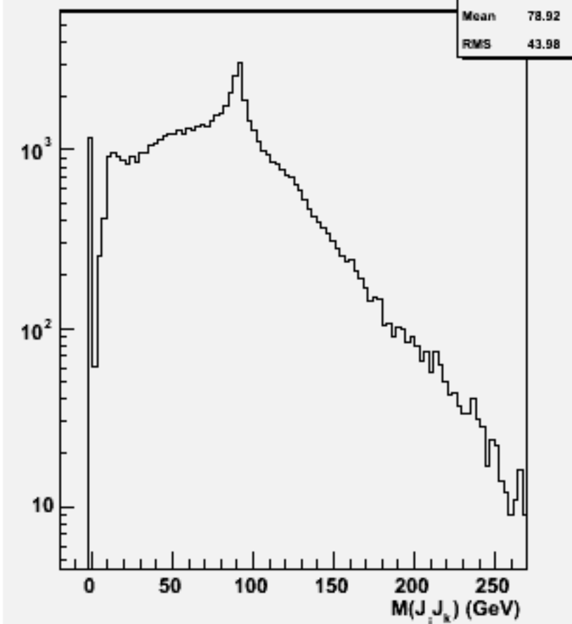
2jets mass(All comb)w101828 n1n1cccc_o
