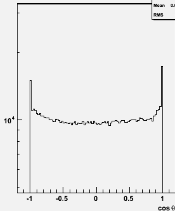
Particle cos \theta : w101828 n1n1cccc_o
