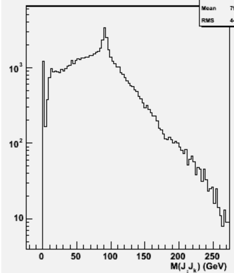
2jets mass(All comb)w101824 n1n1uucc_o
