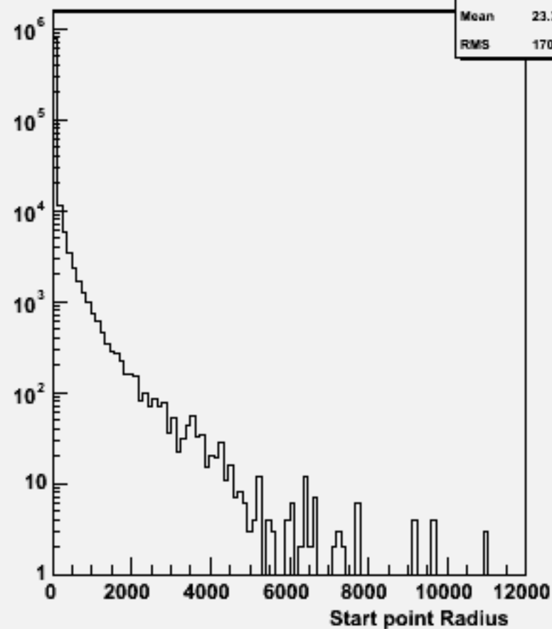
Start point R : w101824 n1n1uucc_o
