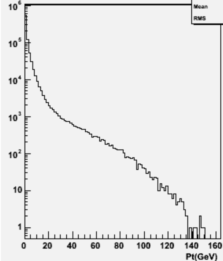
Particle Pt : w101824 n1n1uucc_o
