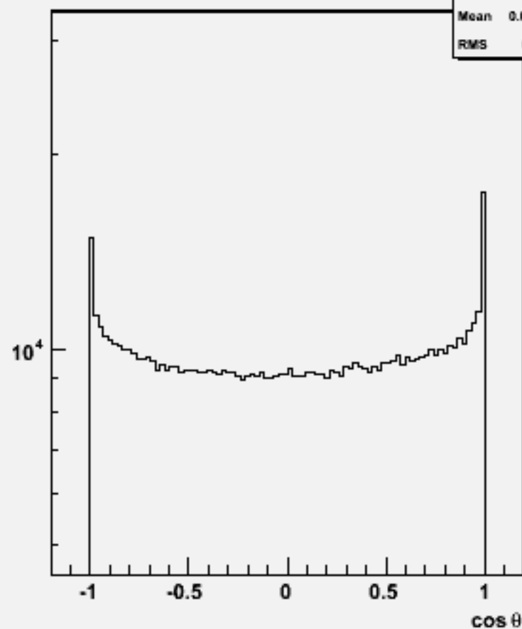
Particle cos \theta : w101824 n1n1uucc_o
