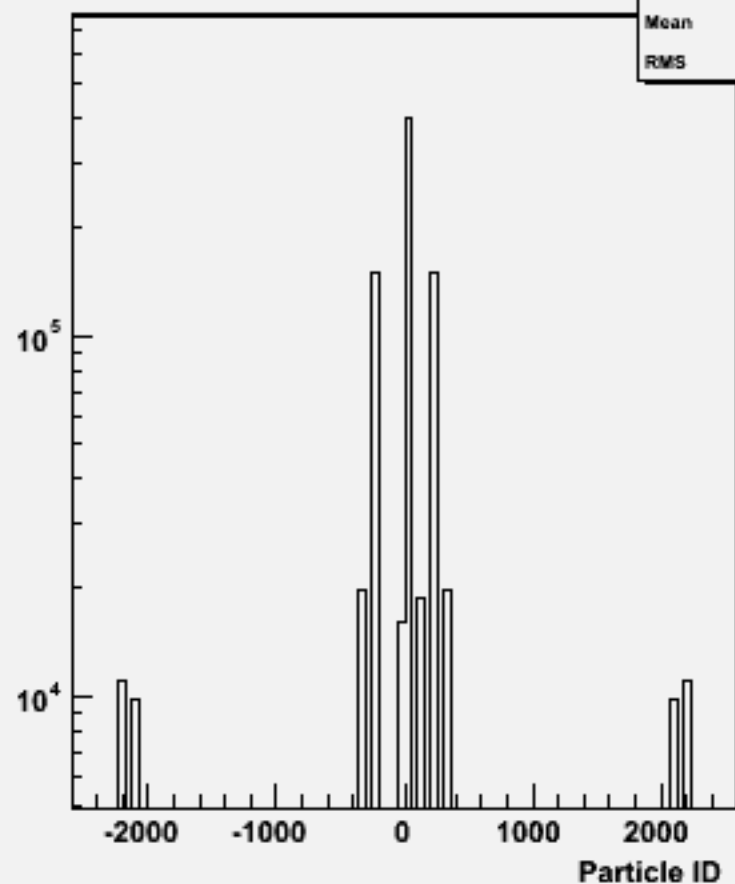
Particle ID : w101824 n1n1uucc_o
