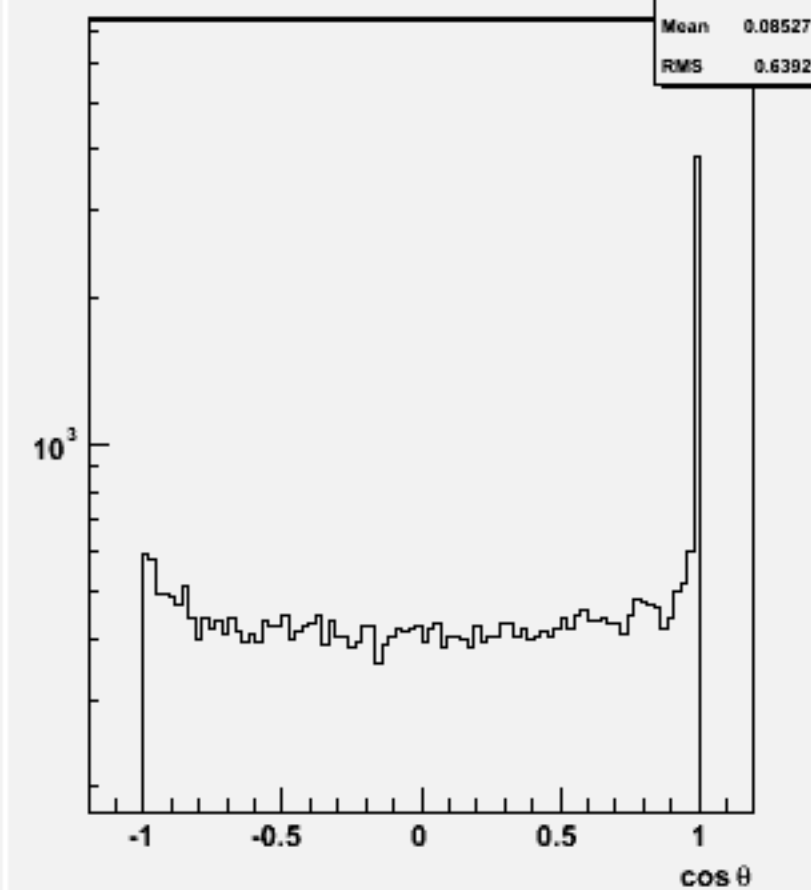
Jet cosθ (All jets)w101824 n1n1uucc_o
