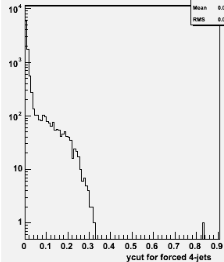
Ycut for 4-jets :w101824 n1n1uucc_o
