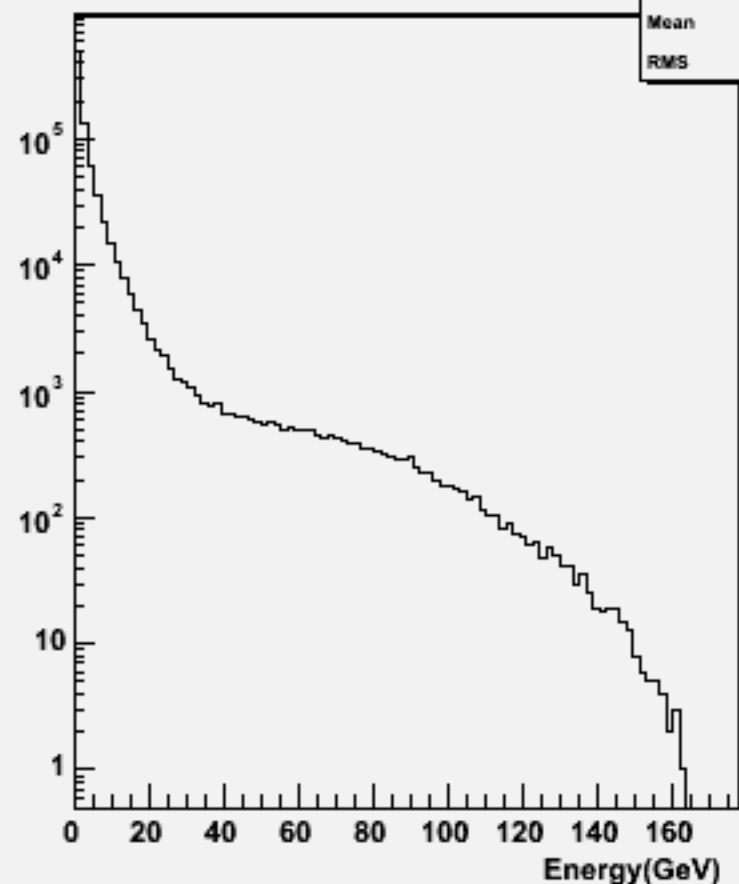
Particle Energy : w101824 n1n1uucc_o
