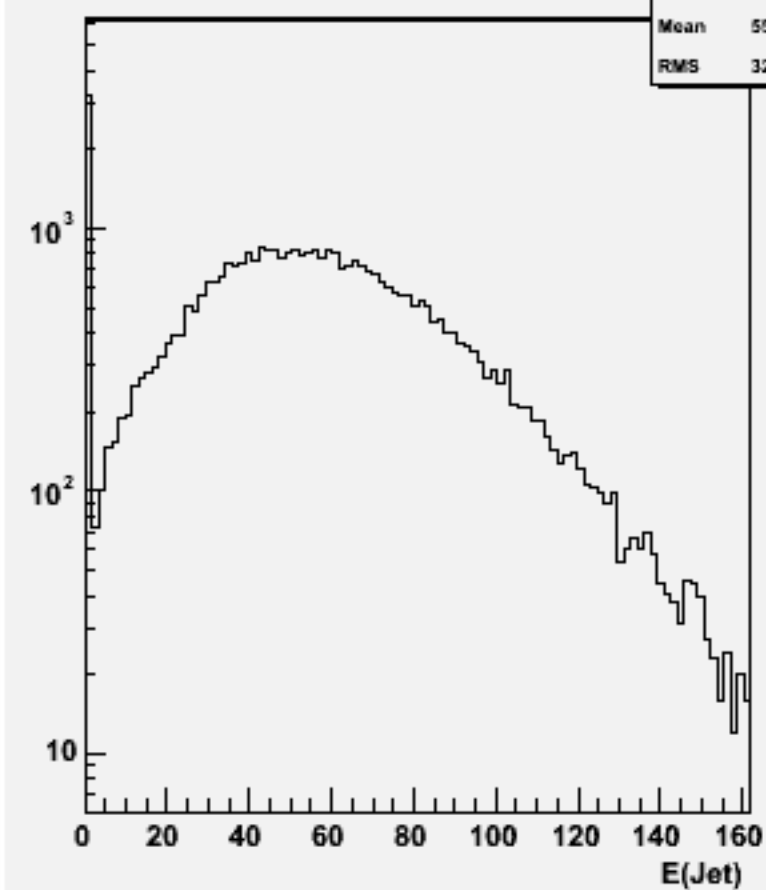
Jet energies(All jets)w101824 n1n1uucc_o
