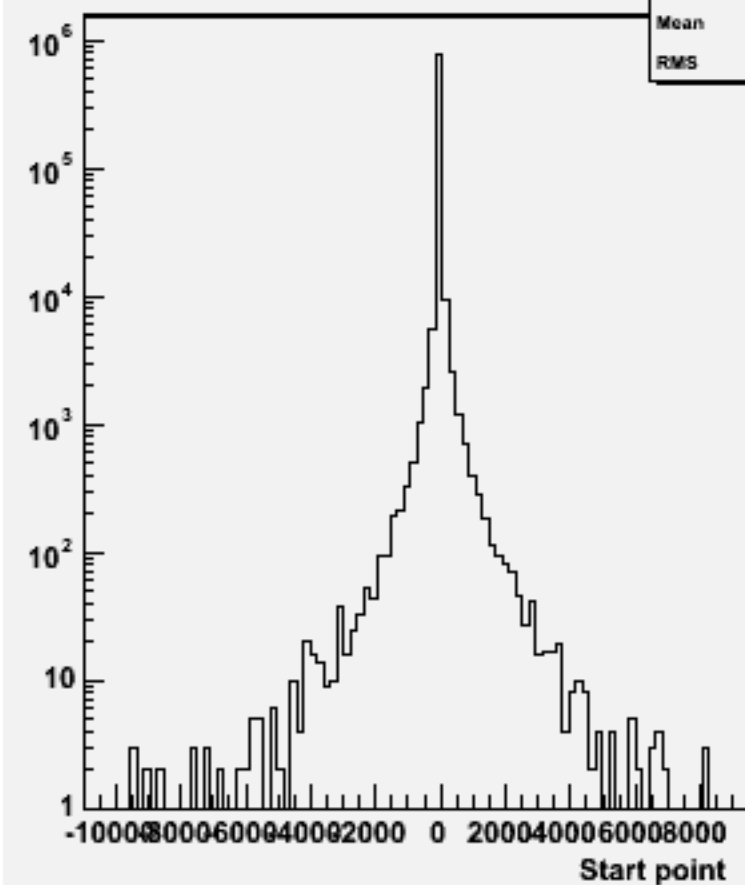
Start point Z : w101824 n1n1uucc_o
