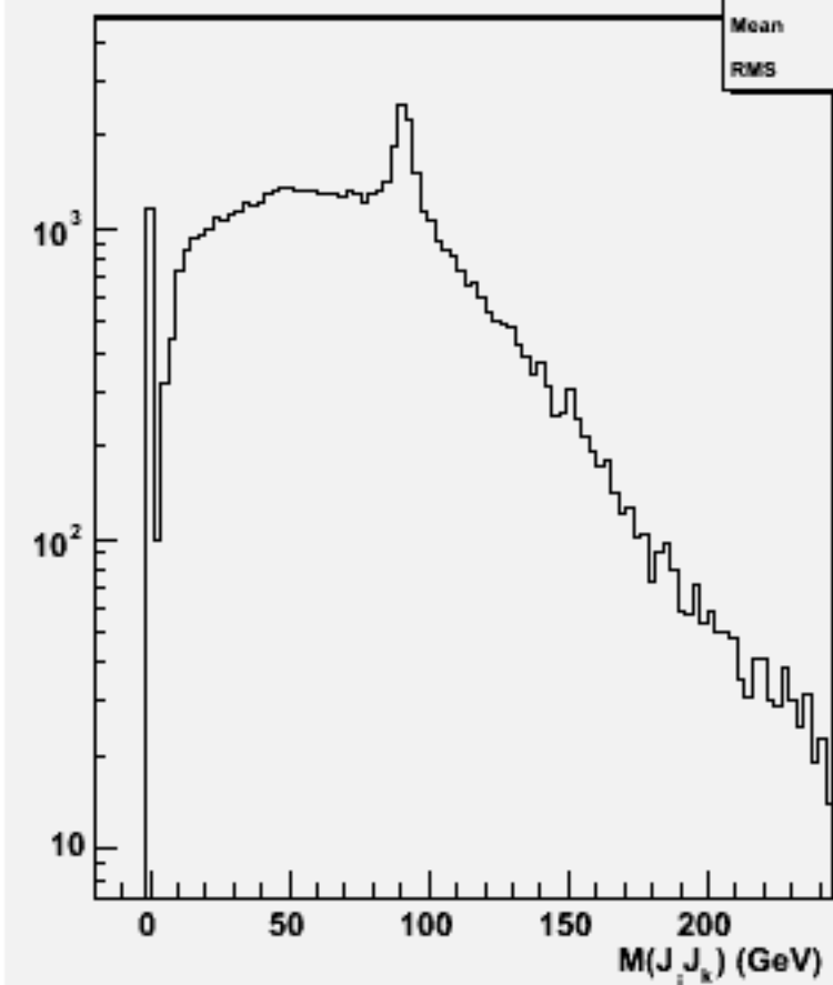
2jets mass(All comb)w101821 n1n1uuuu_o
