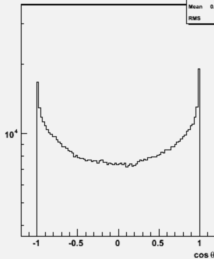
Particle cos \theta : w101821 n1n1uuuu_o
