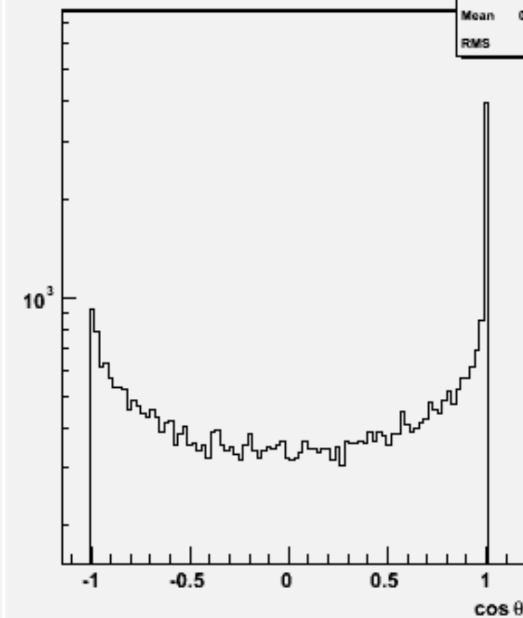
Jet cos \theta (All jets)w101821 n1n1uuuu_o
