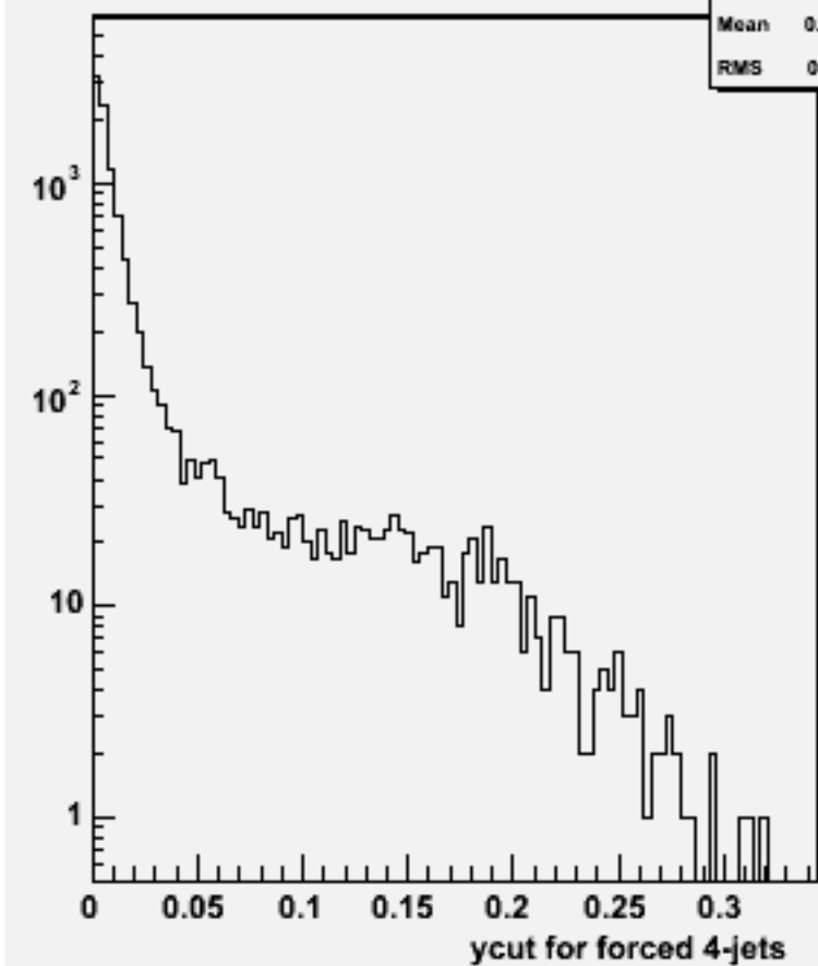
Ycut for 4-jets :w101821 n1n1uuuu_o
