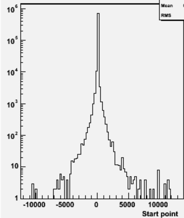
Start point Z : w101821 n1n1uuuu_o
