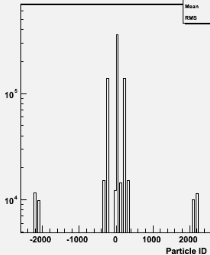
Particle ID : w101821 n1n1uuuu_o
