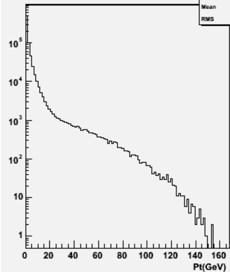
Particle Pt : w101821 n1n1uuuu_o
