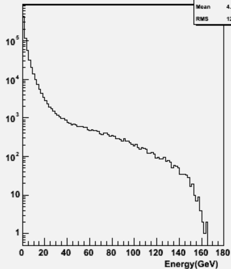
Particle Energy : w101821 n1n1uuuu_o
