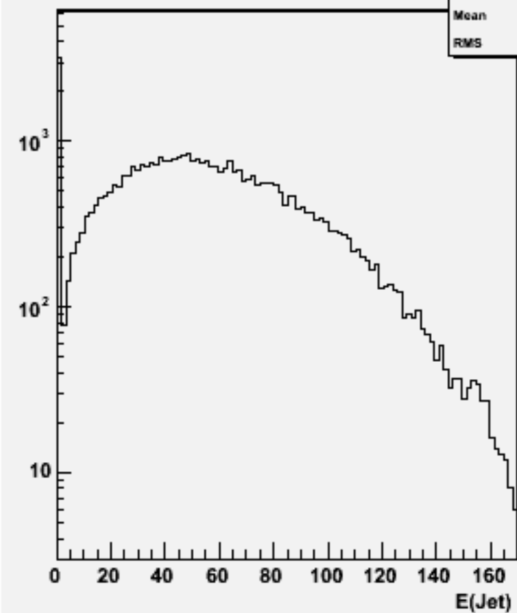
Jet energies(All jets)w101821 n1n1uuuu_o
