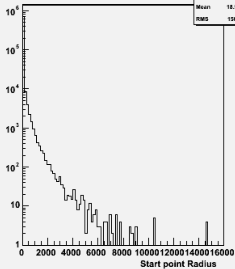
Start point R : w101821 n1n1uuuu_o
