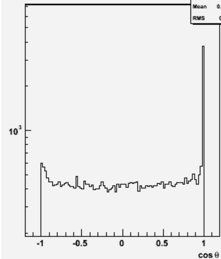
Jet cosθ (All jets)w101820 n1n1uuuu_o
