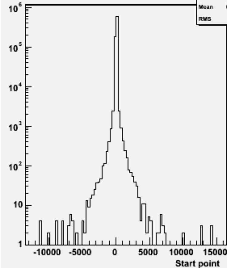
Start point Z : w101820 n1n1uuuu_o
