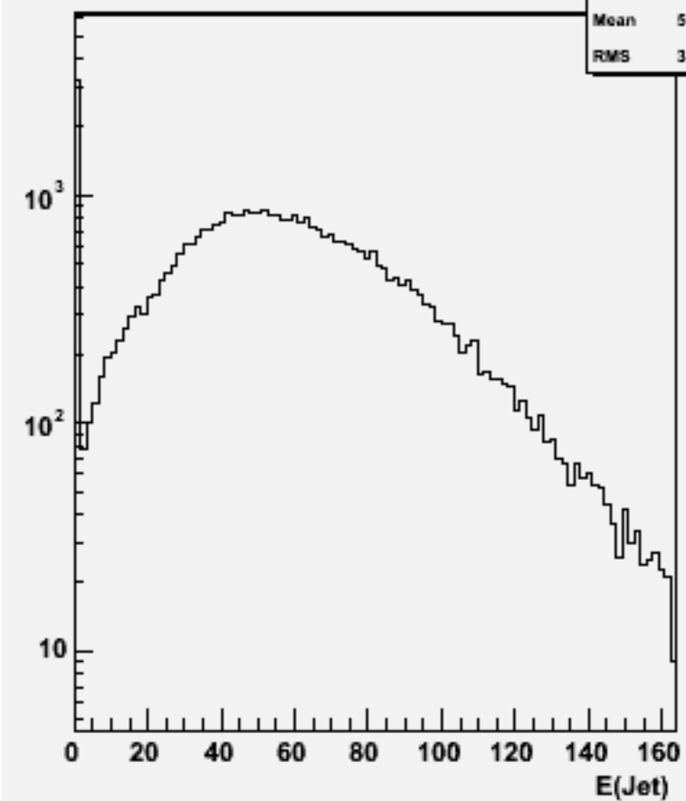
Jet energies(All jets)w101820 n1n1uuuu_o
