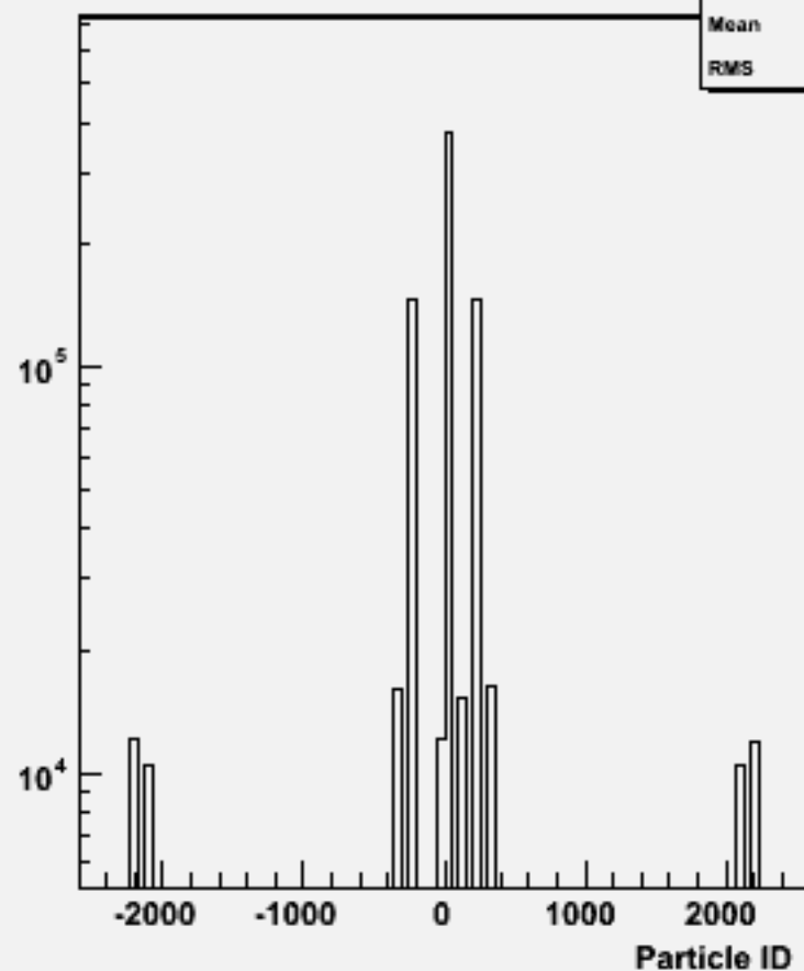
Particle ID : w101820 n1n1uuuu_o
