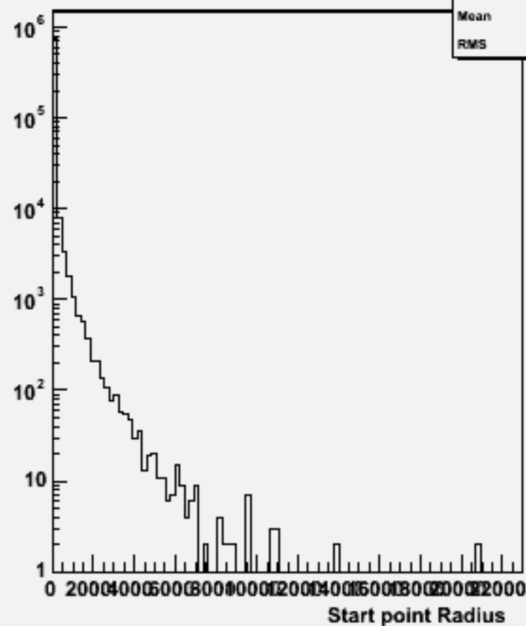
Start point R : w101820 n1n1uuuu_o
