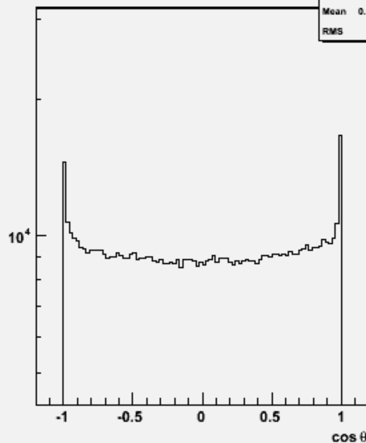
Particle cos \theta : w101820 n1n1uuuu_o
