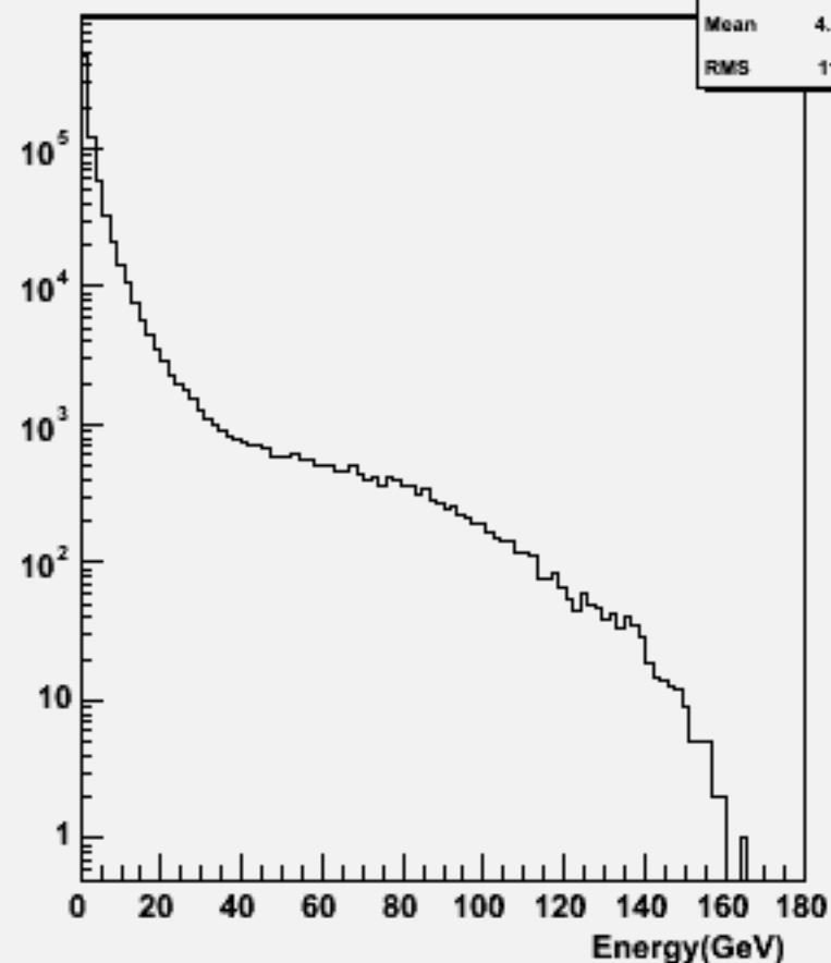
Particle Energy : w101820 n1n1uuuu_o
