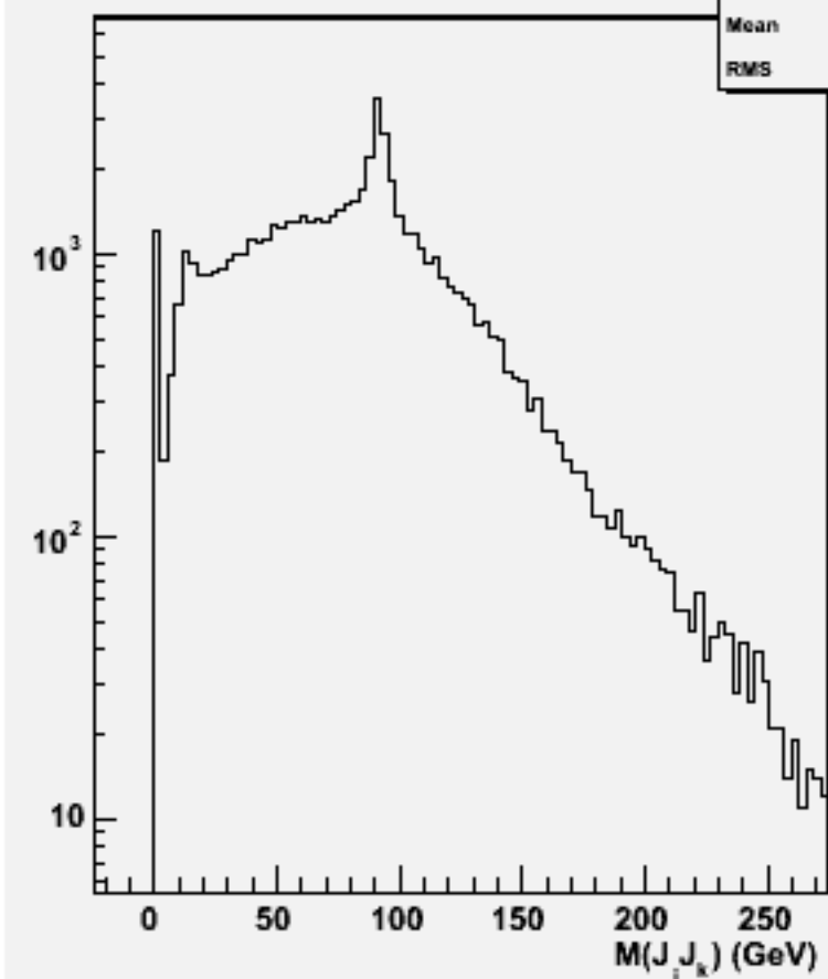
2jets mass(All comb)w101820 n1n1uuuu_o
