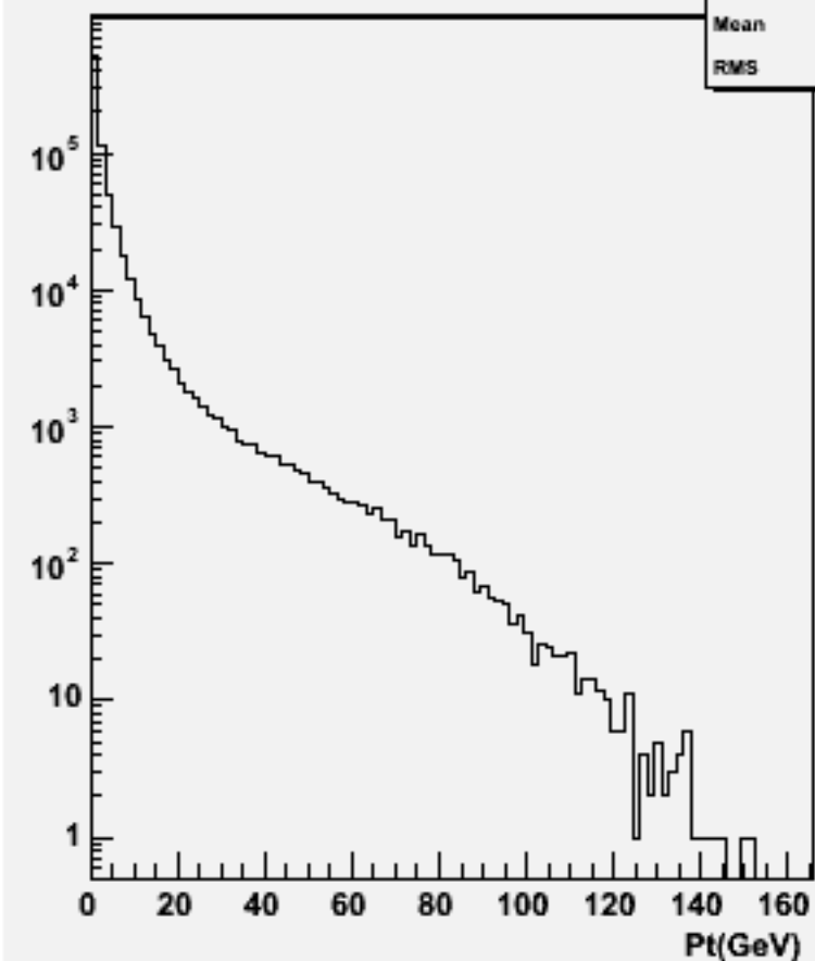
Particle Pt : w101820 n1n1uuuu_o
