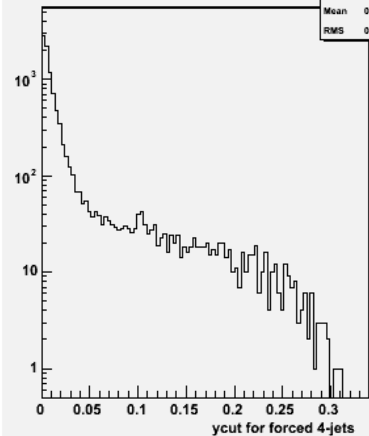
Ycut for 4-jets :w101820 n1n1uuuu_o
