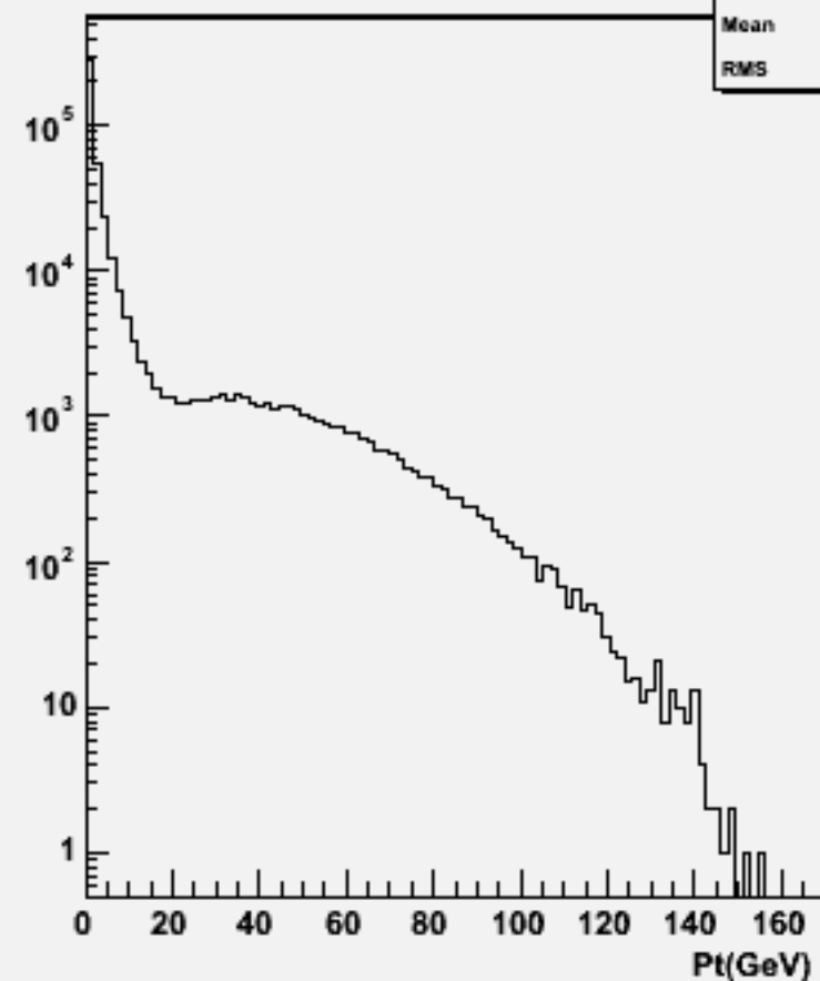
Start point Z : w101817 n1n1n3n3cc_o
