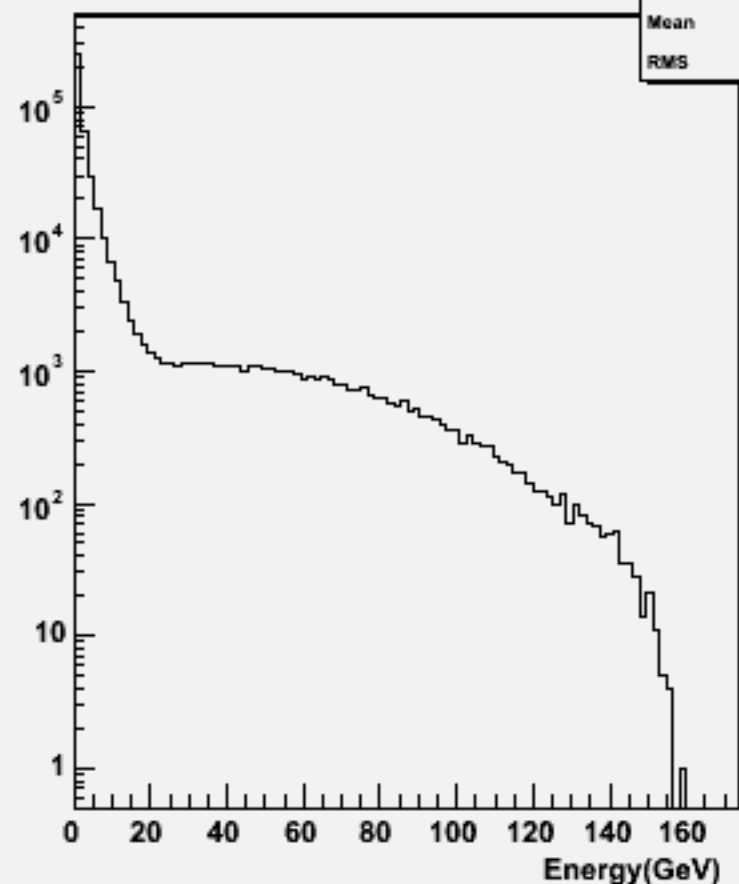
Start point R : w101817 n1n1n3n3cc_o
