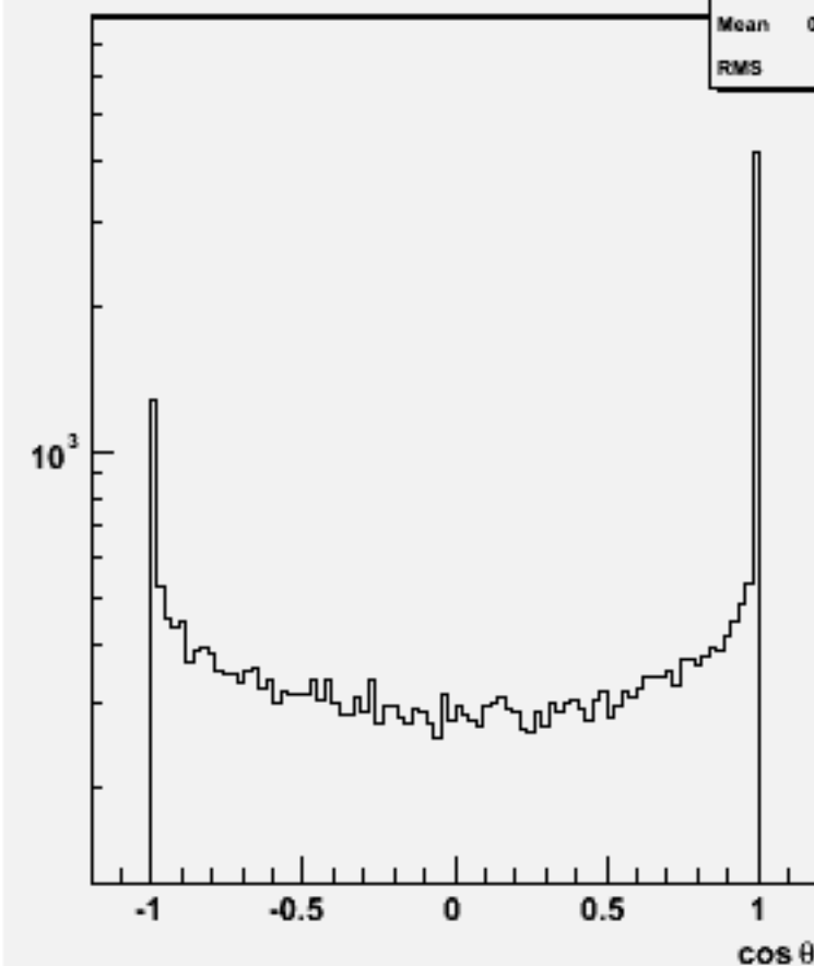
Jet cos \theta (All jets)w101817 n1n1n3n3cc_o
