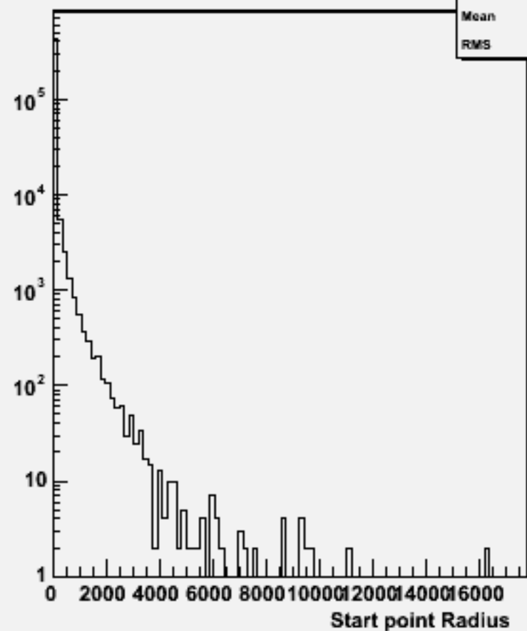
Start point R : w101817 n1n1n3n3cc_o
