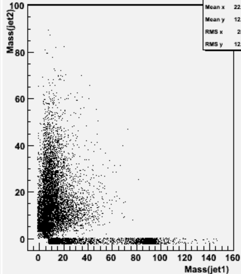
Jet mass for forced 2-jets : w101817 n1n1n3n3cc_o
