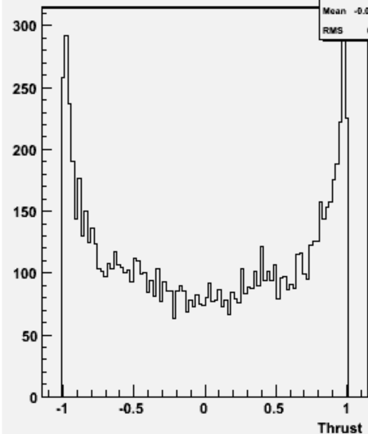
cos \Theta (thrust) w101817 n1n1n3n3cc_o
