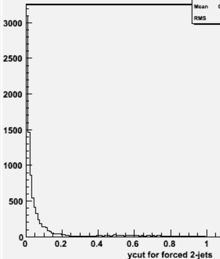
Ycut for 2-jets :w101817 n1n1n3n3cc_o
