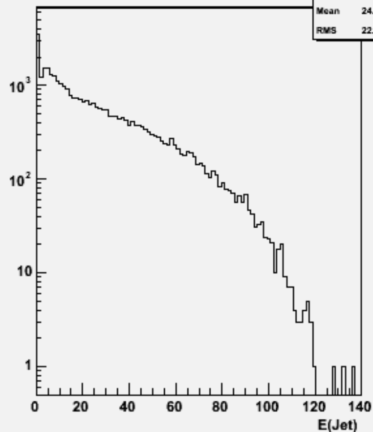
Jet energies(All jets)w101817 n1n1n3n3cc_o
