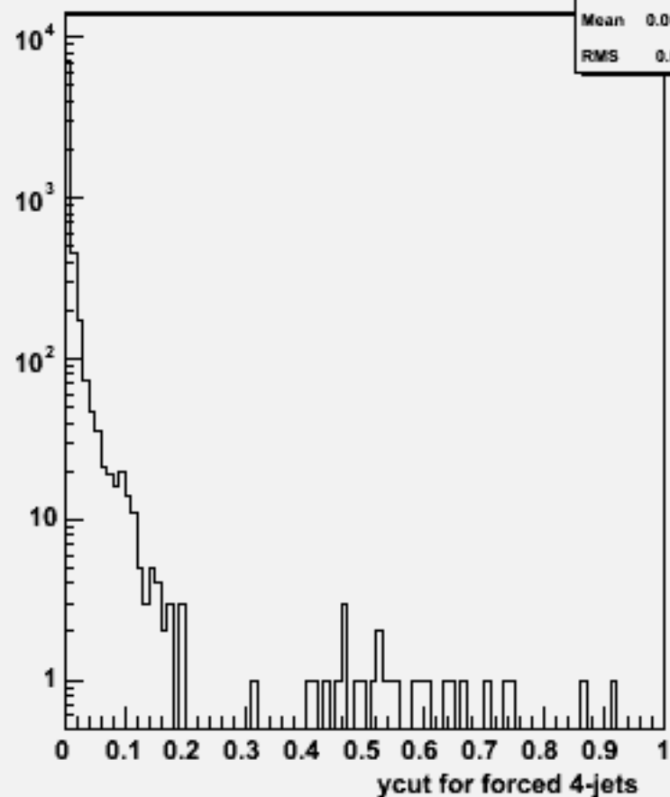
Ycut for 4-jets :w101817 n1n1n3n3cc_o
