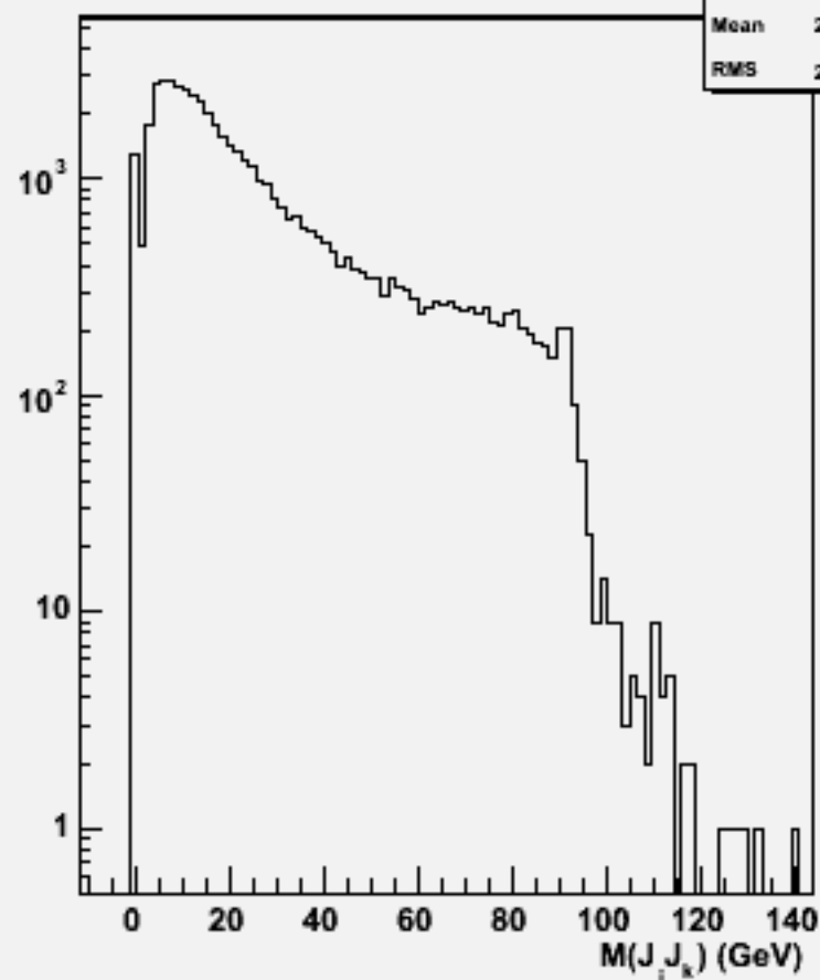
2jets mass(All comb)w101817 n1n1n3n3cc_o
