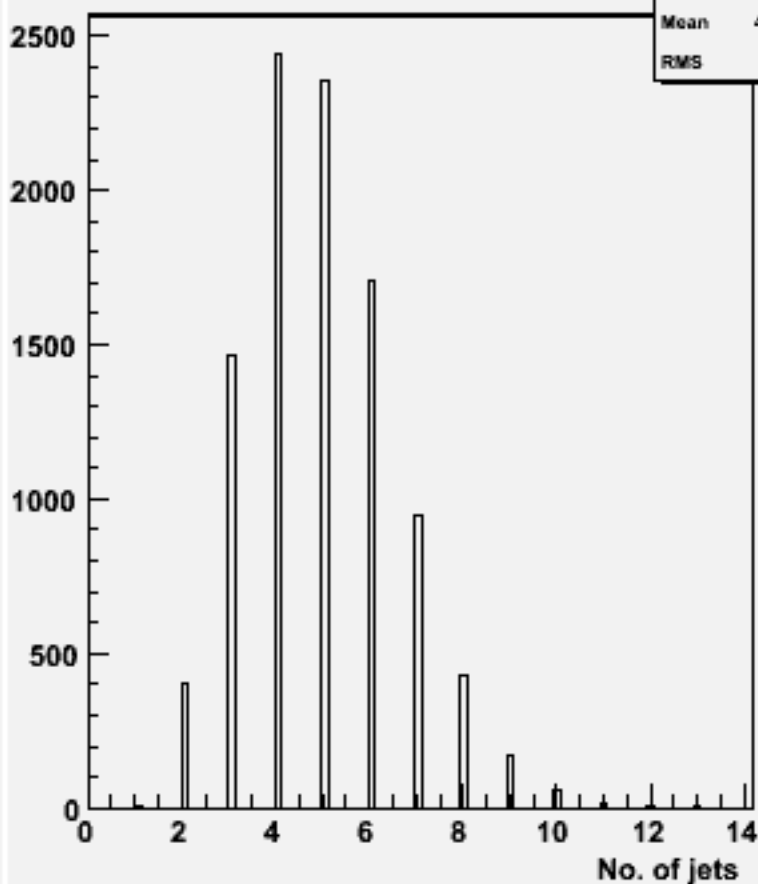
No. jets (ycut=0.001) : w101817 n1n1n3n3cc_o
