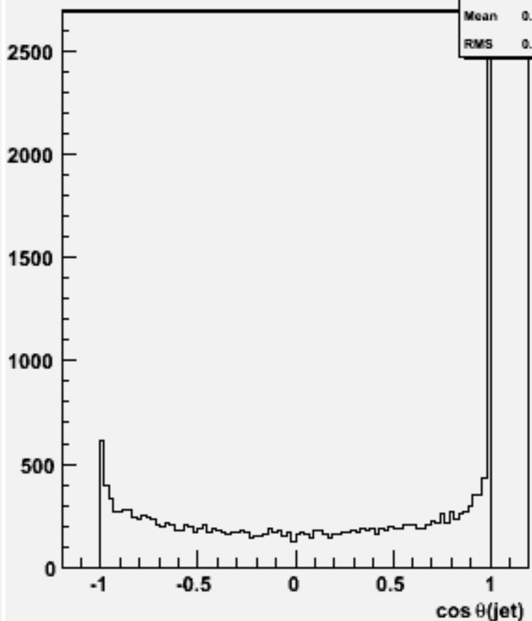
cos \theta for 2-jets :w101817 n1n1n3n3cc_o
