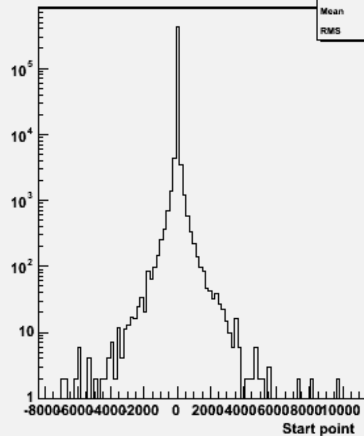
Start point Z : w101817 n1n1n3n3cc_o
