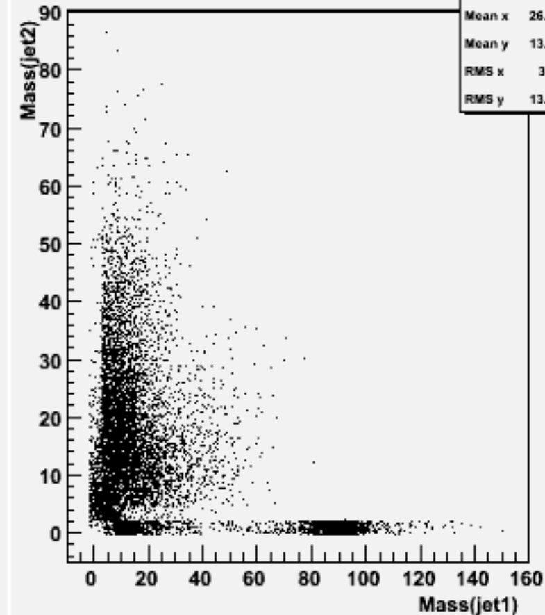
Jet mass for forced 2-jets : w101816 n1n1n3n3cc_o
