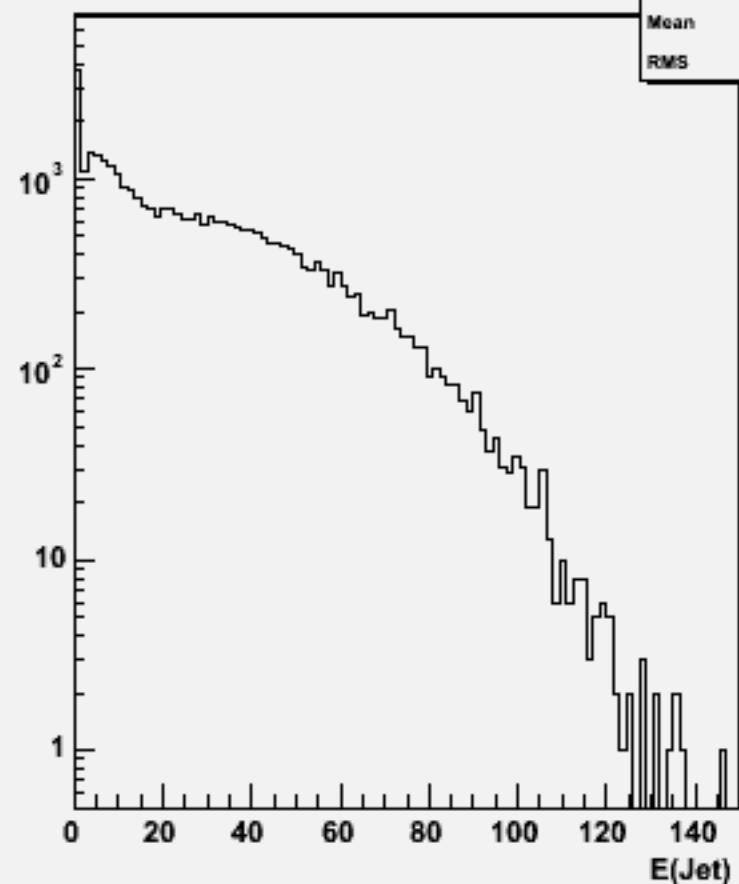
Jet energies(All jets)w101816 n1n1n3n3cc_o
