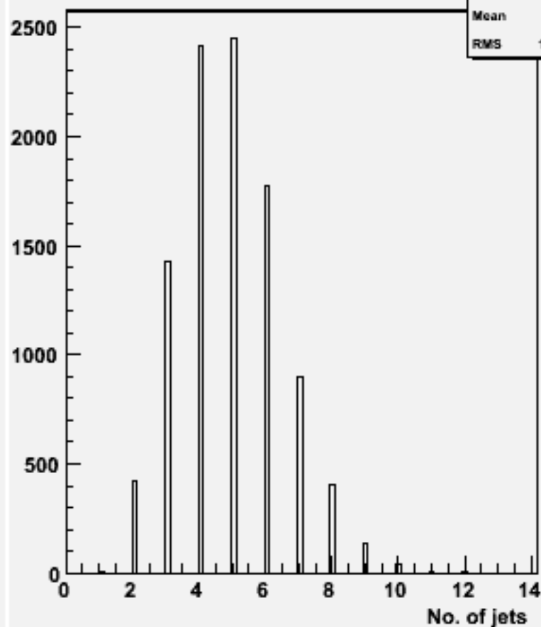
No. jets (ycut=0.001) : w101816 n1n1n3n3cc_o
