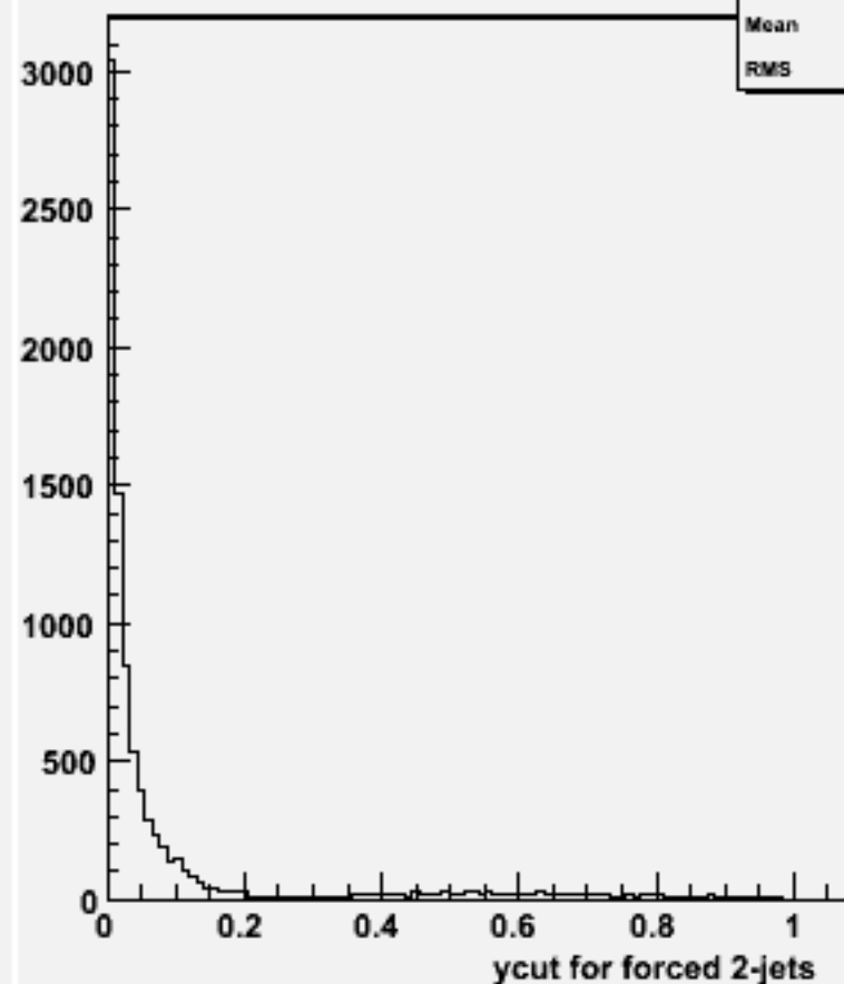
Ycut for 2-jets :w101816 n1n1n3n3cc_o
