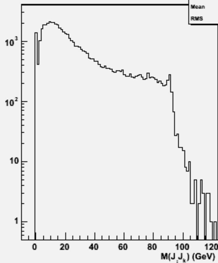
2jets mass(All comb)w101816 n1n1n3n3cc_o
