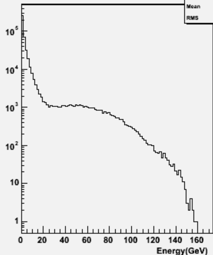
Start point R : w101816 n1n1n3n3cc_o
