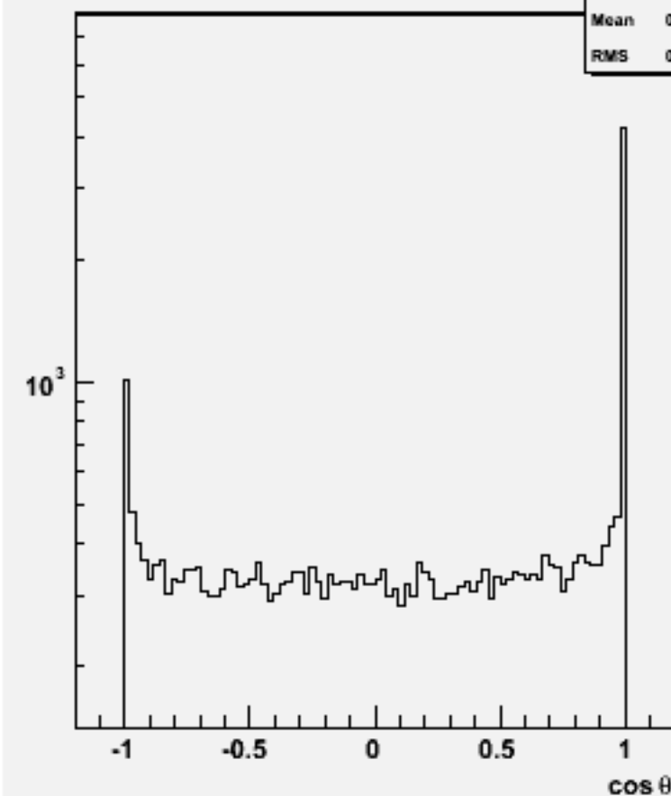
Jet cos \theta (All jets)w101816 n1n1n3n3cc_o
