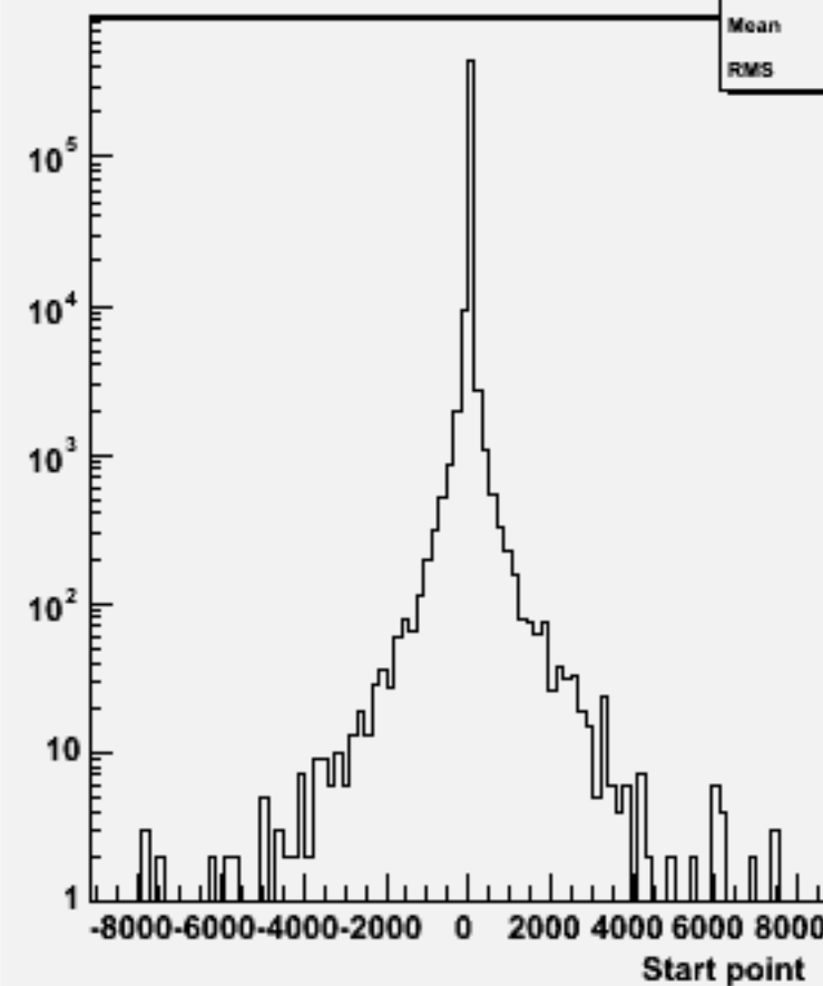
Start point Z : w101816 n1n1n3n3cc_o
