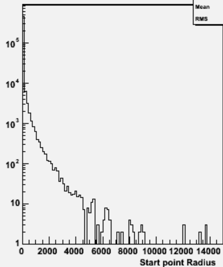
Start point R : w101816 n1n1n3n3cc_o
