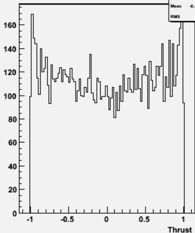
cos \Theta (thrust) w101816 n1n1n3n3cc_o
