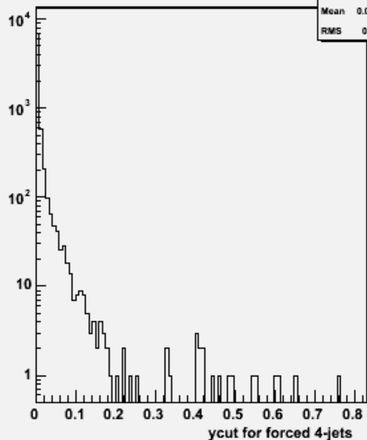
Ycut for 4-jets :w101816 n1n1n3n3cc_o
