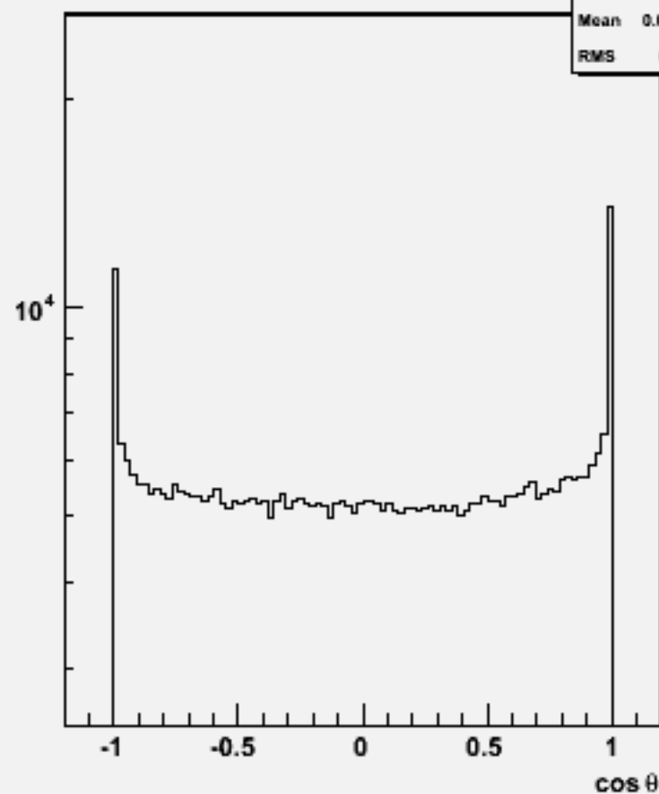
Particle cosθ : w101816 n1n1n3n3cc_o
