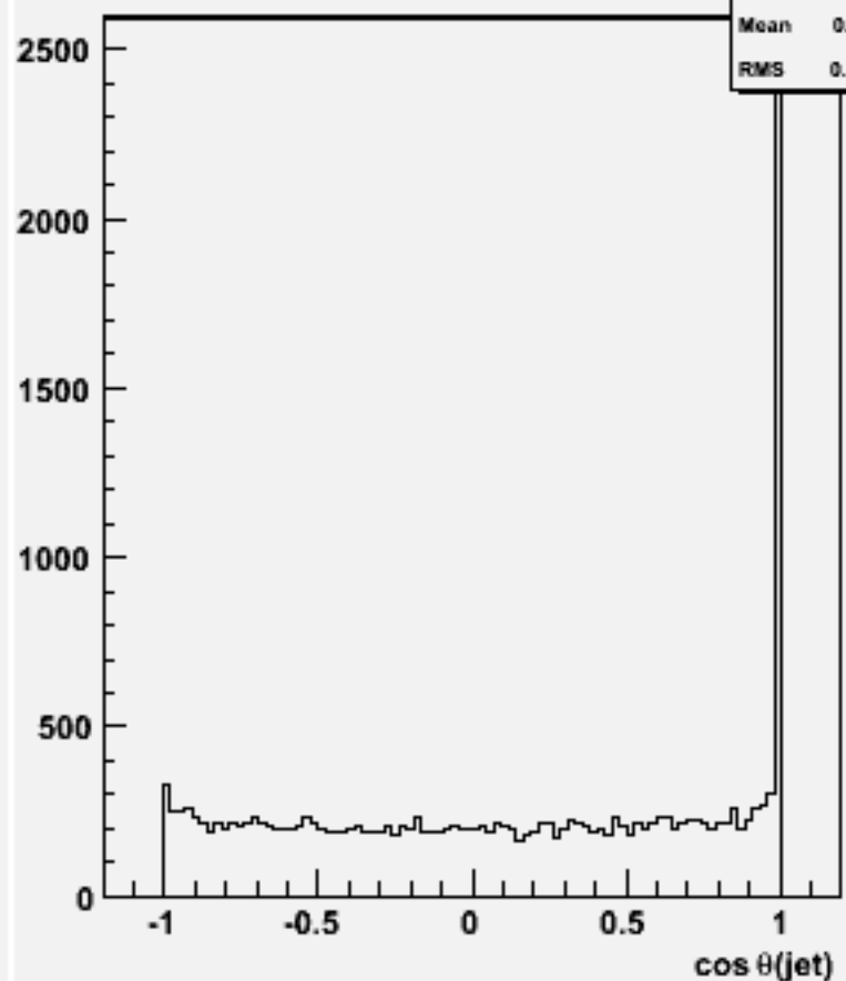
cos \theta for 2-jets :w101816 n1n1n3n3cc_o
