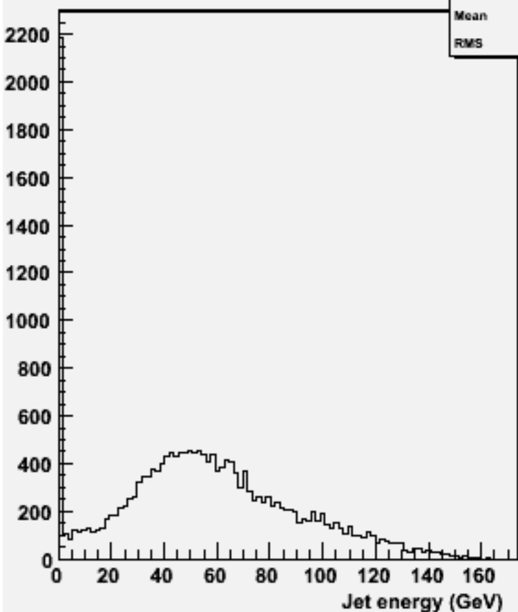
energy for 2-jets :w101816 n1n1n3n3cc_o
