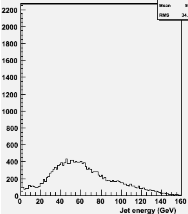
energy for 2-jets :w101812 n1n1n3n3uu_o
