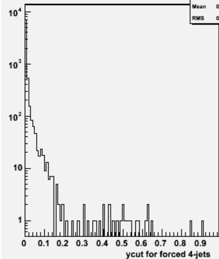
Ycut for 4-jets :w101812 n1n1n3n3uu_o
