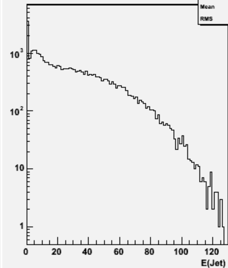
Jet energies(All jets)w101812 n1n1n3n3uu_o
