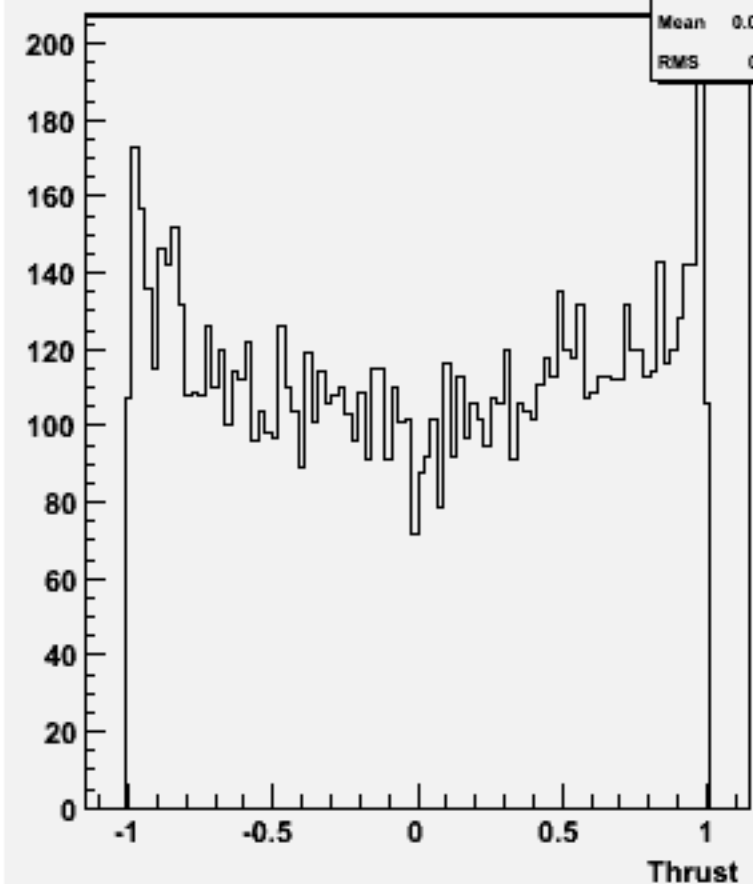
cos \Theta (thrust) w101812 n1n1n3n3uu_o
