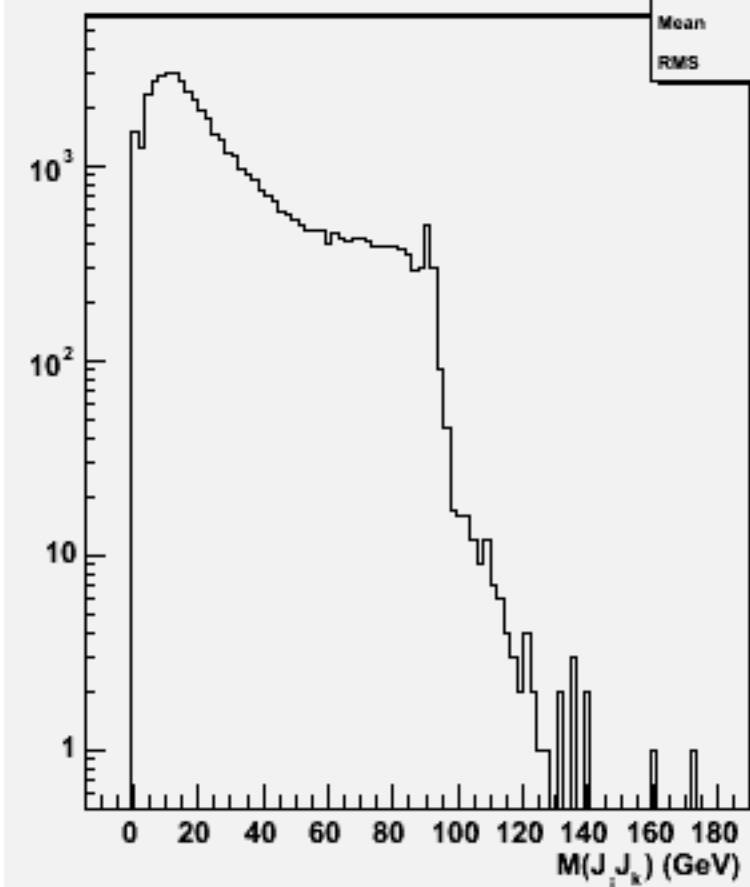
2jets mass(All comb)w101812 n1n1n3n3uu_o
