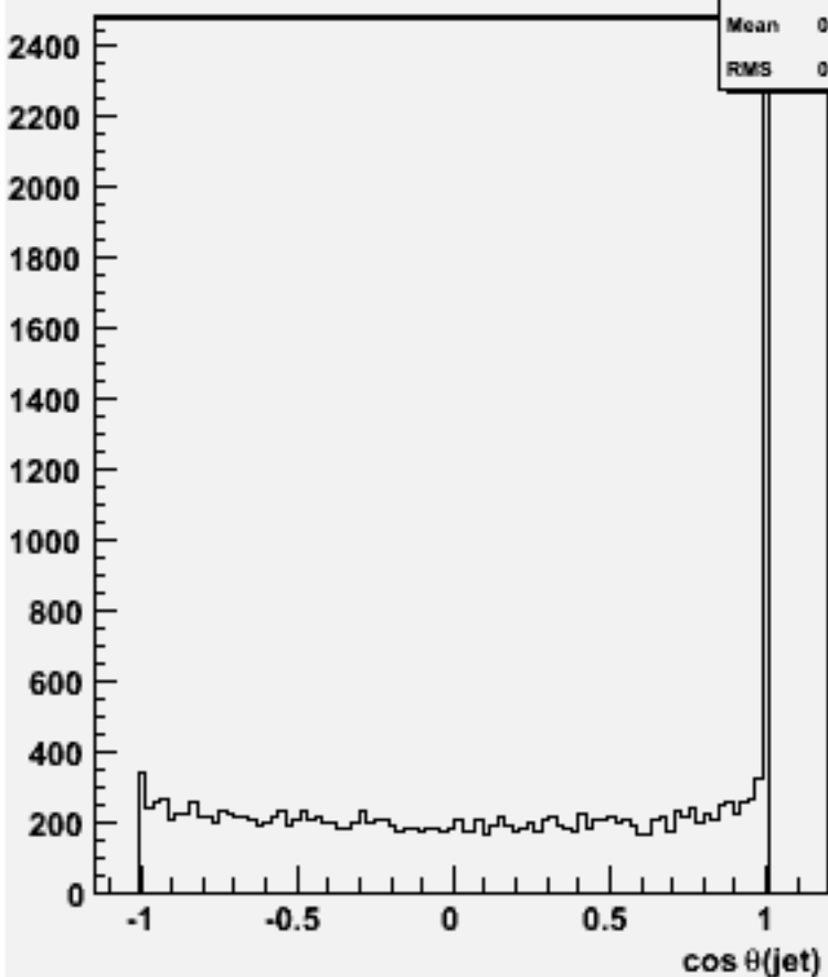
cos \theta for 2-jets :w101812 n1n1n3n3uu_o
