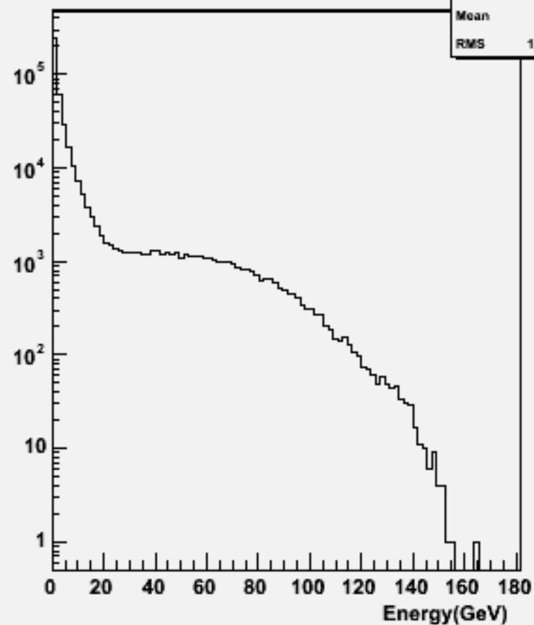
Particle Energy : w101812 n1n1n3n3uu_o
