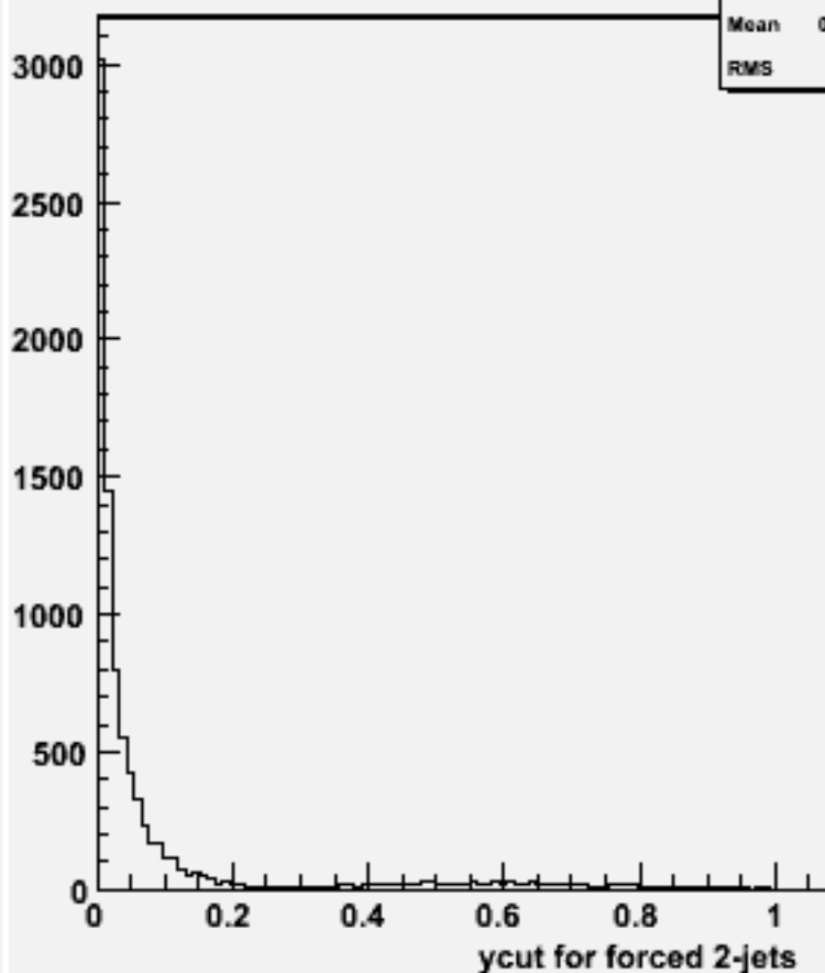
Ycut for 2-jets :w101812 n1n1n3n3uu_o
