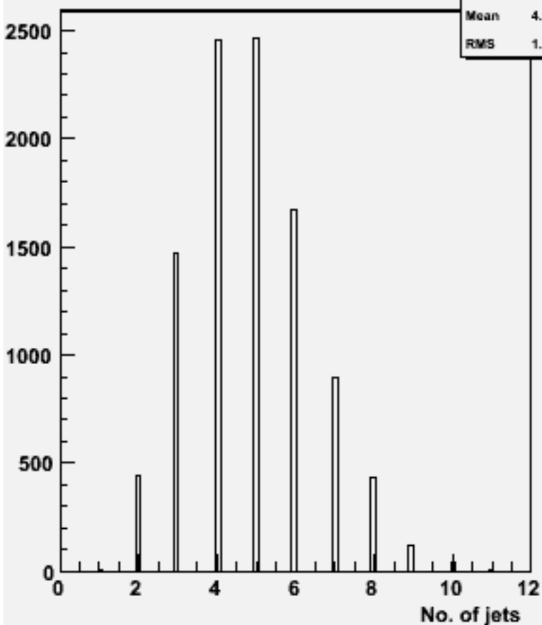
No. jets (ycut=0.001) : w101812 n1n1n3n3uu_o
