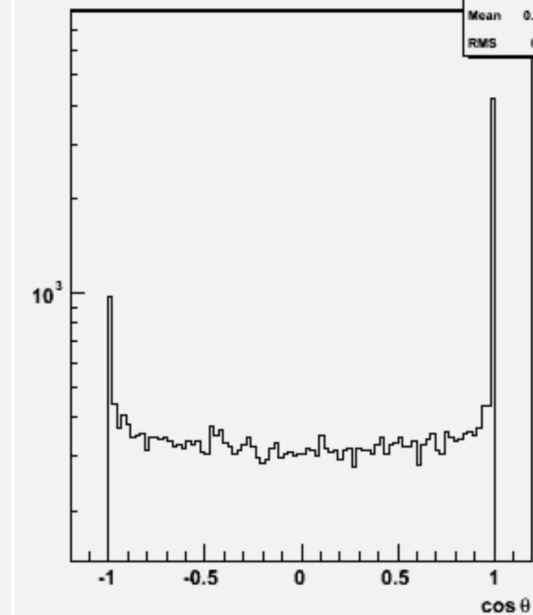
Jet cos \theta (All jets)w101812 n1n1n3n3uu_o
