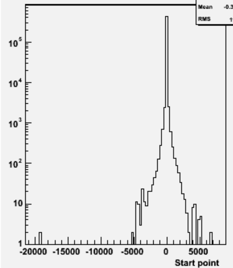
Start point Z : w101812 n1n1n3n3uu_o
