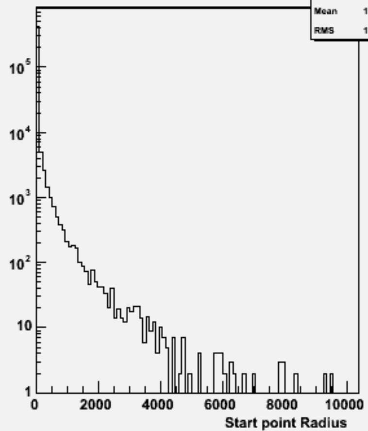
Start point R : w101812 n1n1n3n3uu_o
