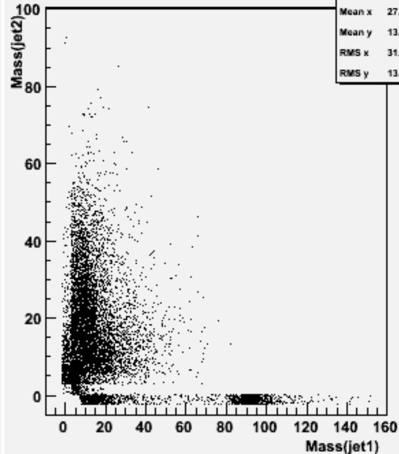
Jet mass for forced 2-jets : w101812 n1n1n3n3uu_o
