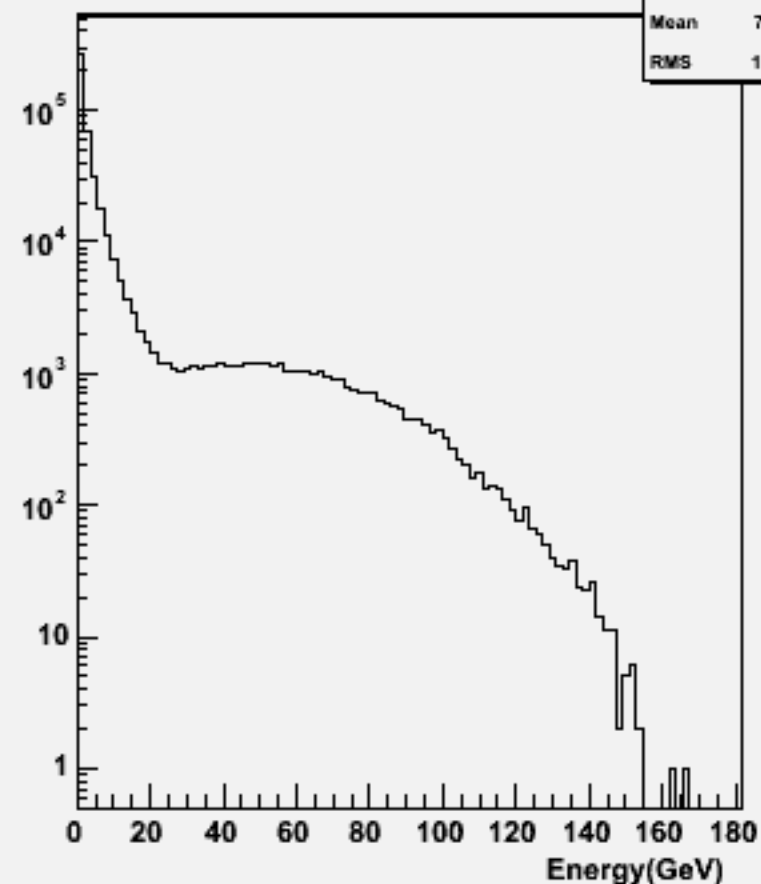
Start point R : w101808 n1n1n2n2cc_o
