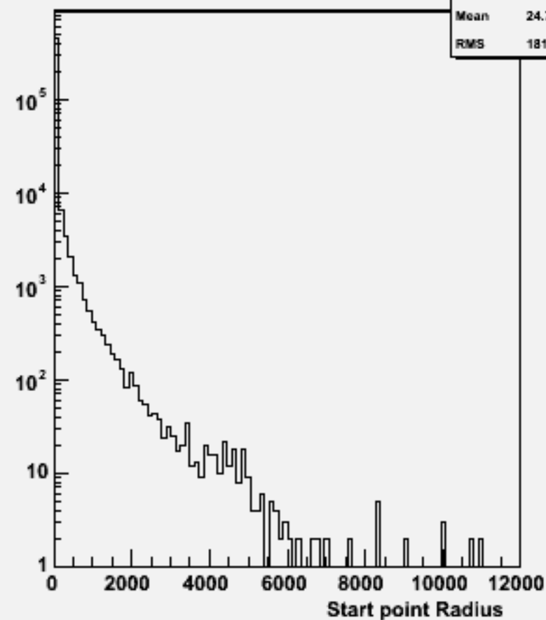
Start point R : w101808 n1n1n2n2cc_o
