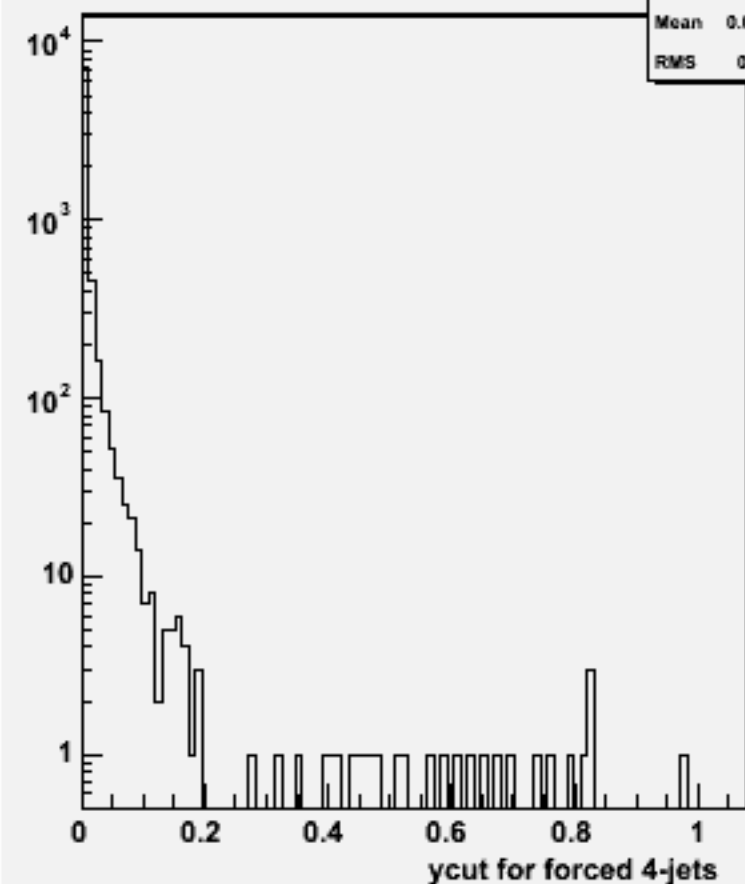
Ycut for 4-jets :w101808 n1n1n2n2cc_o
