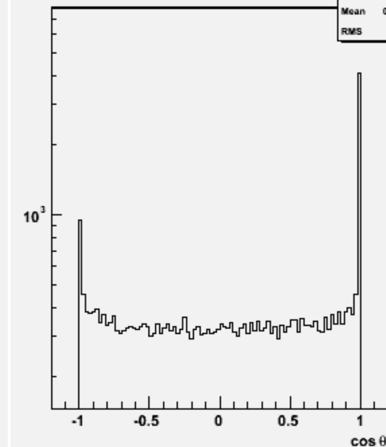
Jet cos \theta (All jets)w101808 n1n1n2n2cc_o
