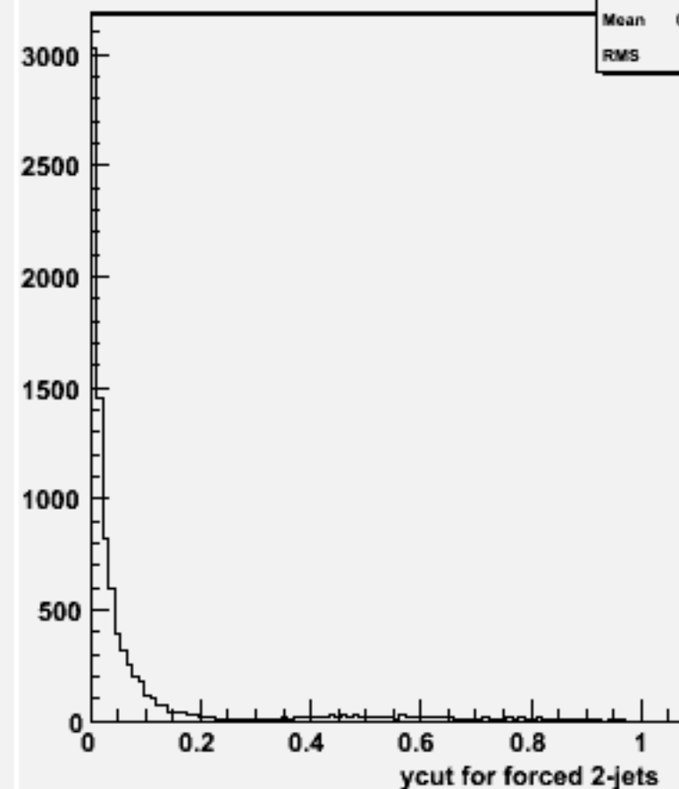
Ycut for 2-jets :w101808 n1n1n2n2cc_o
