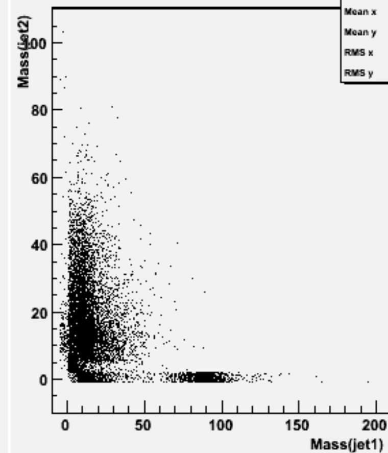
Jet mass for forced 2-jets : w101808 n1n1n2n2cc_o
