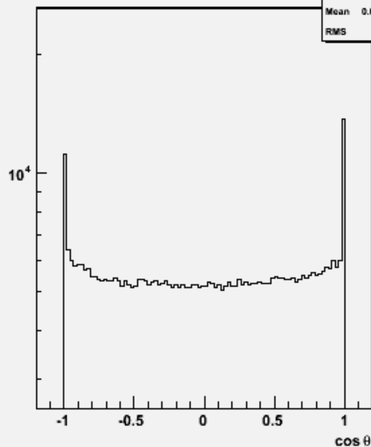
Particle cosθ : w101808 n1n1n2n2cc_o
