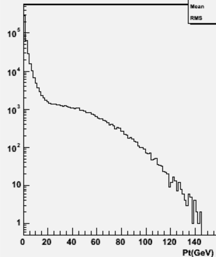
Start point Z : w101808 n1n1n2n2cc_o
