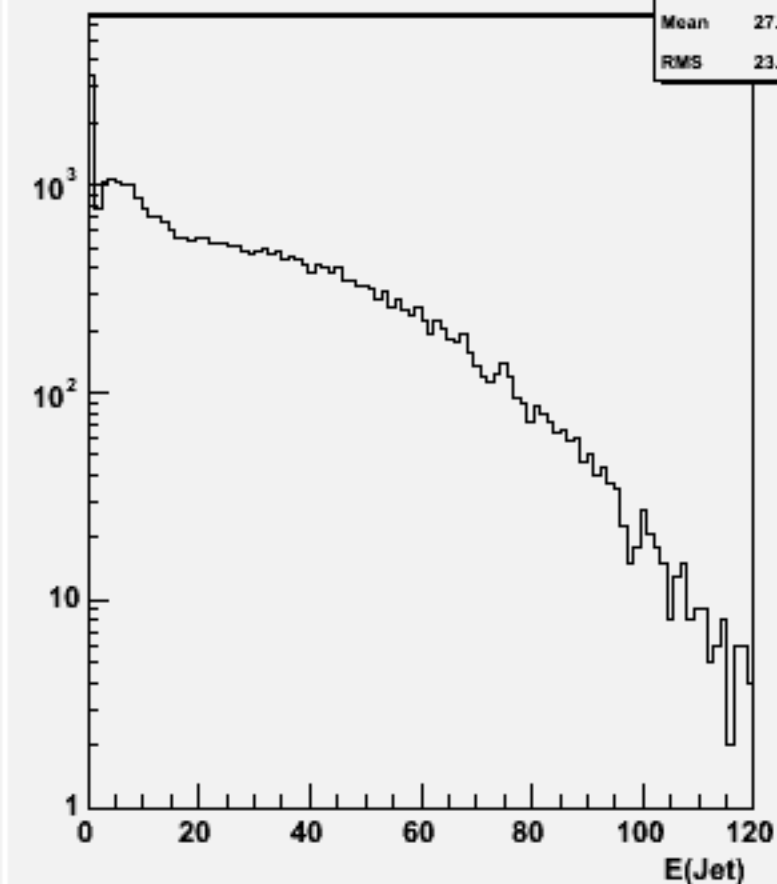
Jet energies(All jets)w101808 n1n1n2n2cc_o
