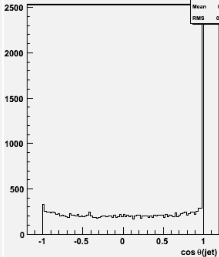
cos \theta for 2-jets :w101808 n1n1n2n2cc_o
