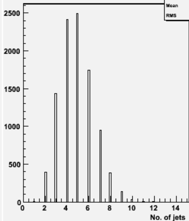
No. jets (ycut=0.001) : w101808 n1n1n2n2cc_o
