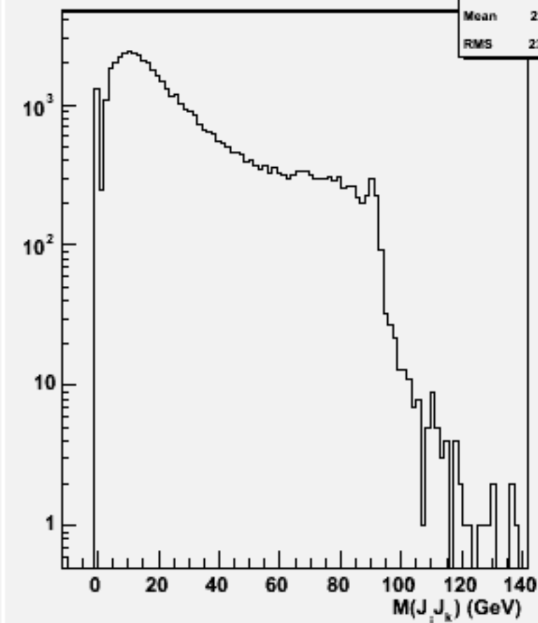
2jets mass(All comb)w101808 n1n1n2n2cc_o
