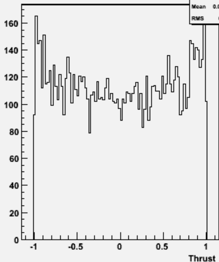
cos \Theta (thrust) w101808 n1n1n2n2cc_o
