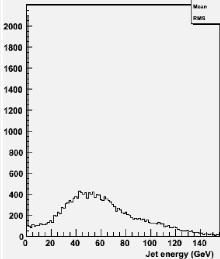
energy for 2-jets :w101808 n1n1n2n2cc_o
