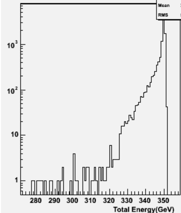
Pt Sum: w101805 n1n1n2n2uu_o
