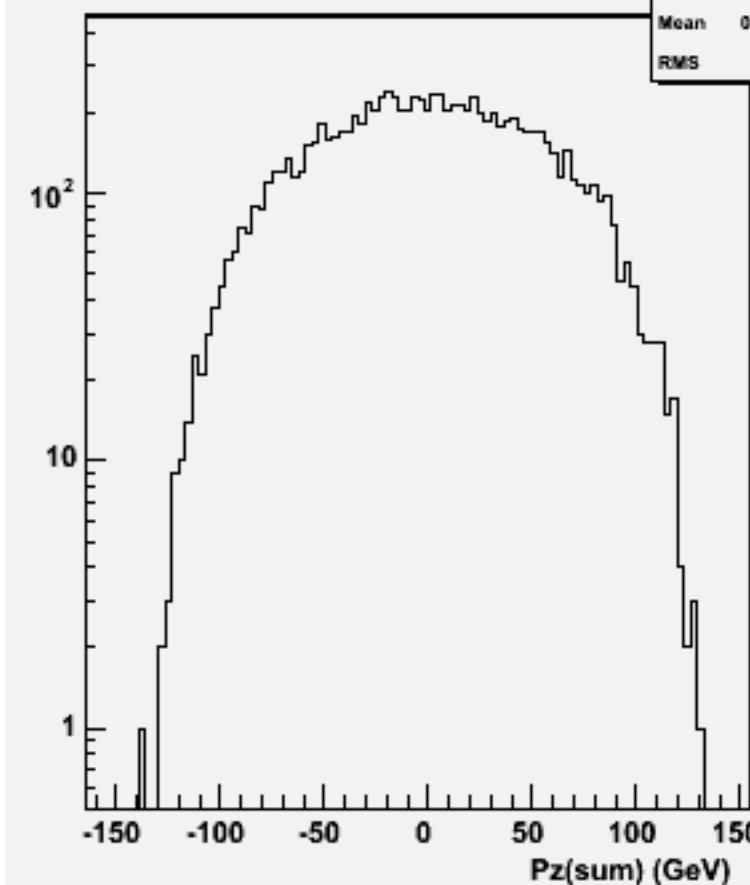
Pz Sum: w101805 n1n1n2n2uu_o
