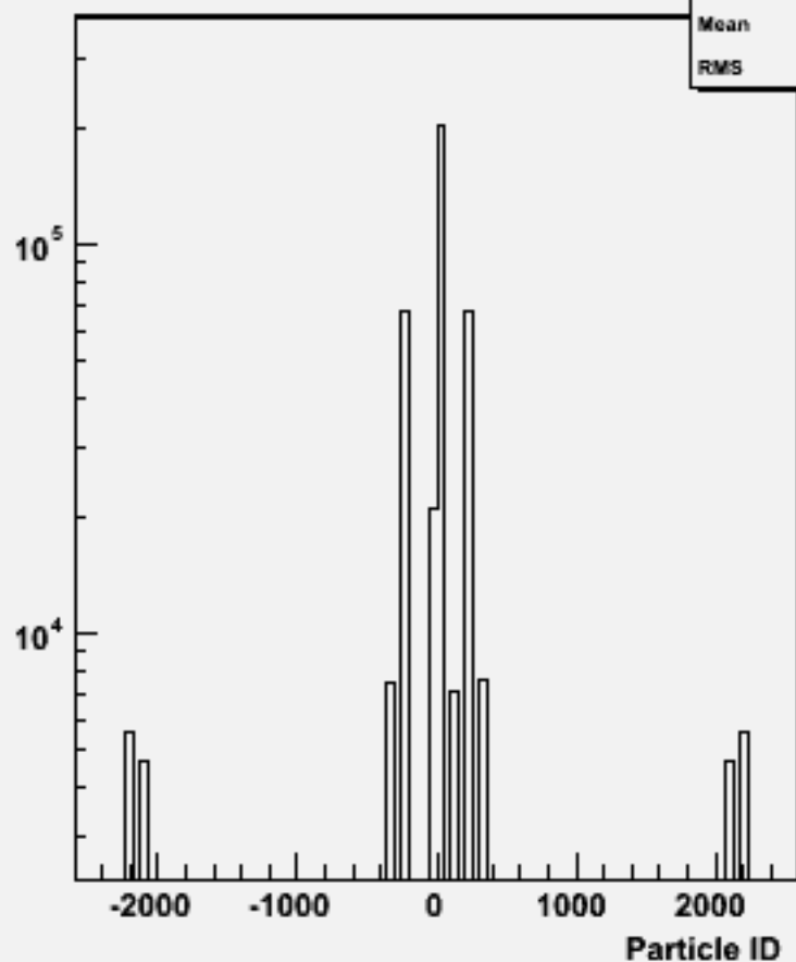
Particle ID : w101805 n1n1n2n2uu_o
