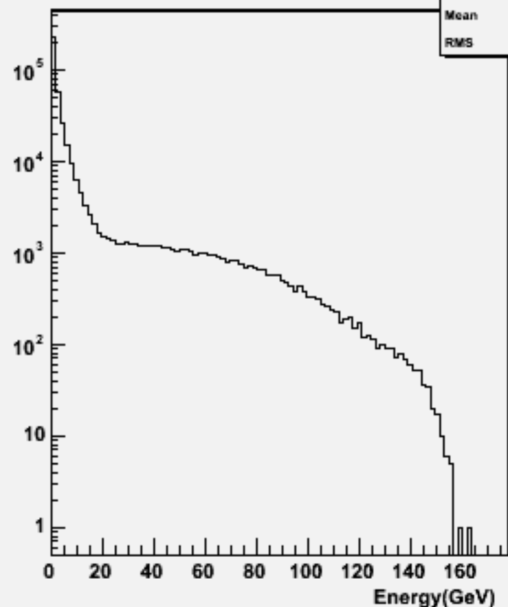
Particle Energy : w101805 n1n1n2n2uu_o
