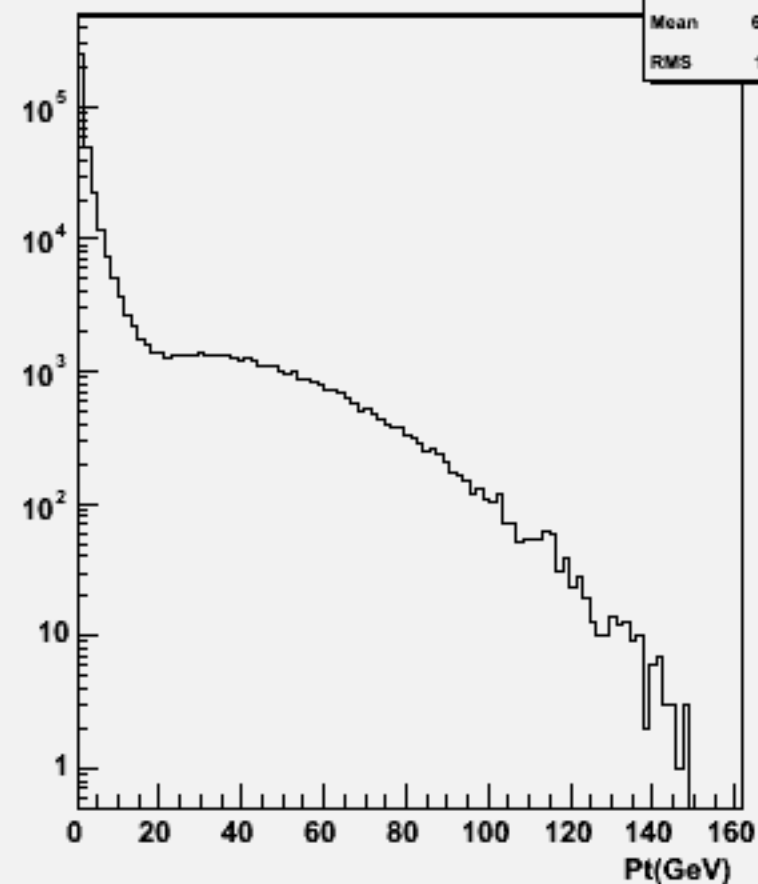
Particle Pt : w101805 n1n1n2n2uu_o
