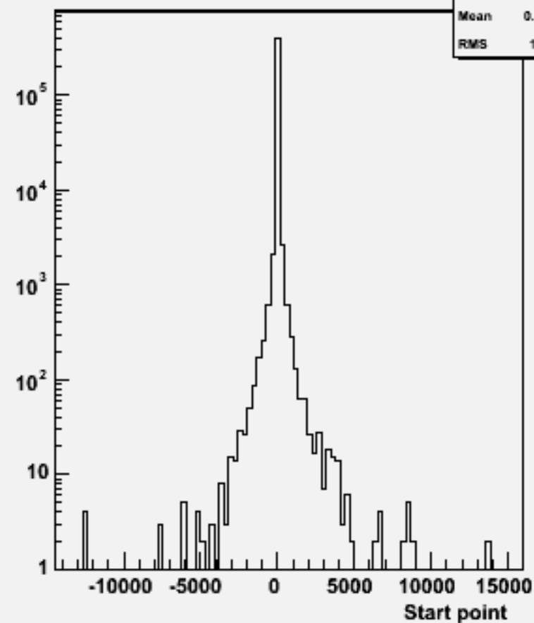
Start point Z : w101805 n1n1n2n2uu_o
