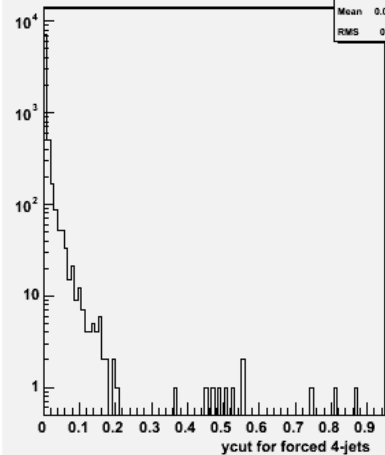
Ycut for 4-jets :w101805 n1n1n2n2uu_o
