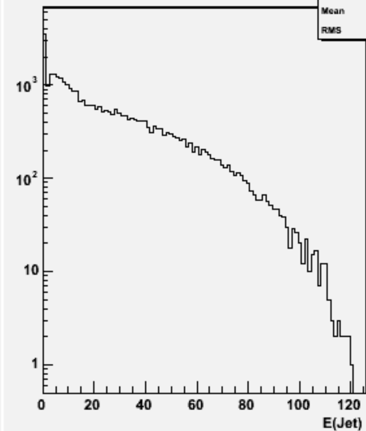
Jet energies(All jets)w101805 n1n1n2n2uu_o
