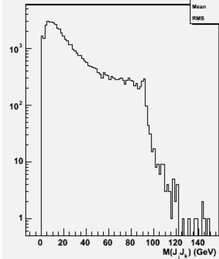
2jets mass(All comb)w101805 n1n1n2n2uu_o
