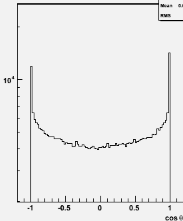
Particle cos \theta : w101805 n1n1n2n2uu_o
