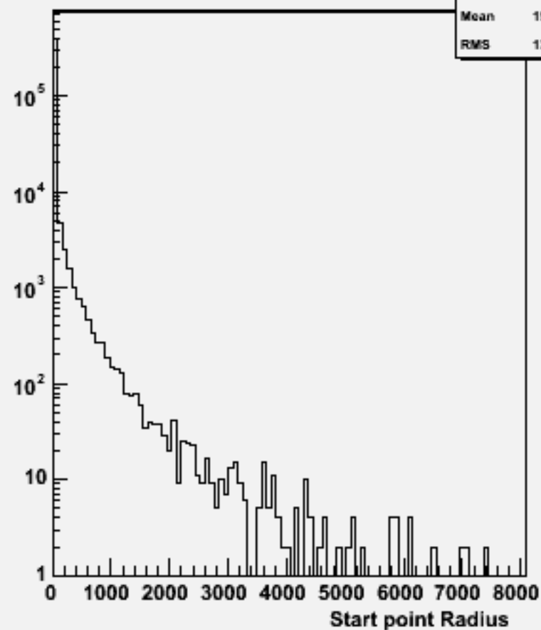
Start point R : w101805 n1n1n2n2uu_o
