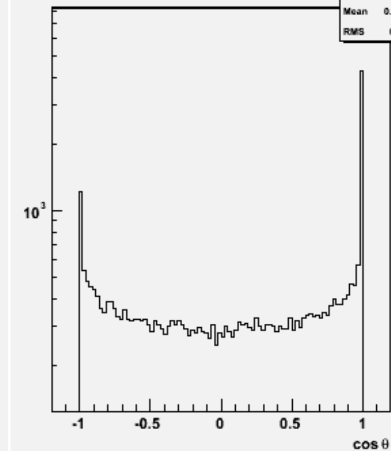
Jet cos \theta (All jets)w101805 n1n1n2n2uu_o
