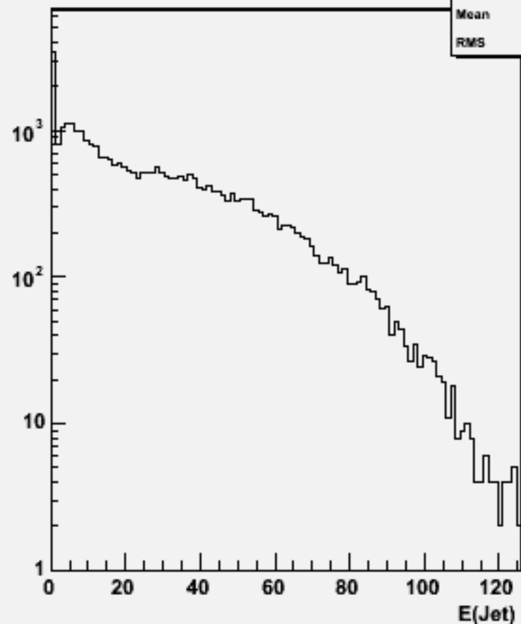
Jet energies(All jets)w101804 n1n1n2n2uu_o
