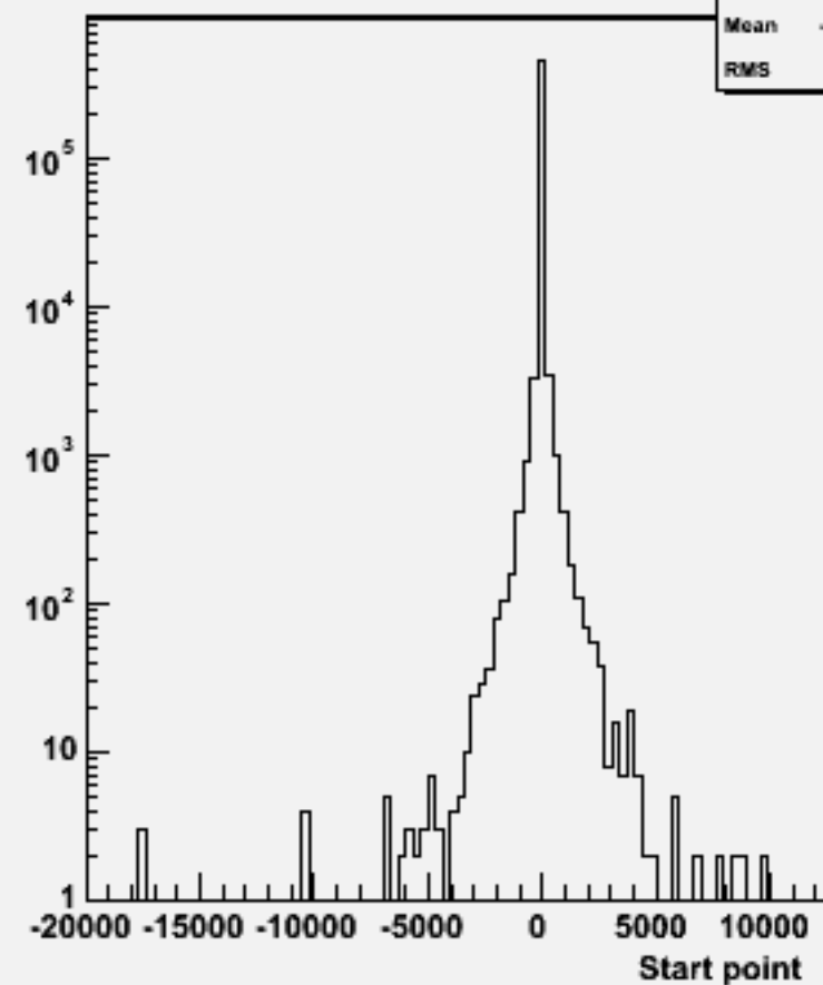
Start point Z : w101800 n1n1n1n1cc_o
