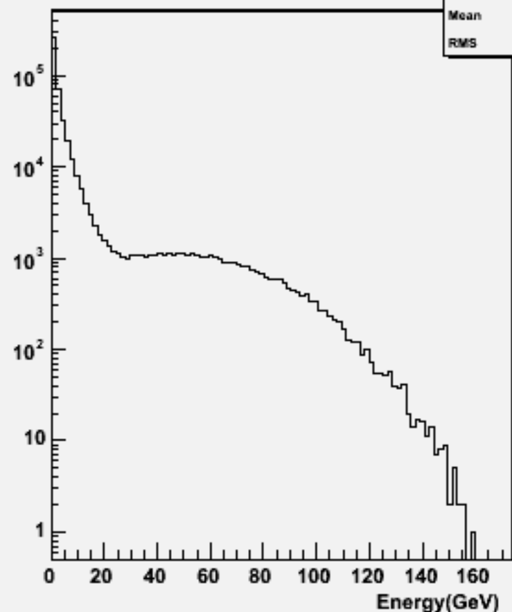
Particle Energy : w101800 n1n1n1n1cc_o
