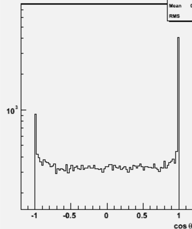
Jet cos \theta (All jets)w101800 n1n1n1n1cc_o
