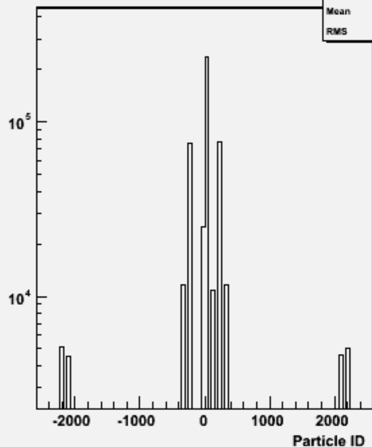
Particle ID : w101800 n1n1n1n1cc_o
