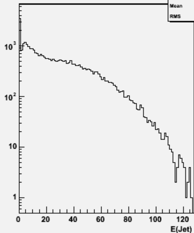
Jet energies(All jets)w101800 n1n1n1n1cc_o
