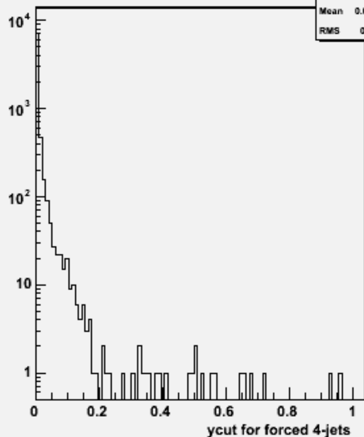
Ycut for 4-jets :w101800 n1n1n1n1cc_o
