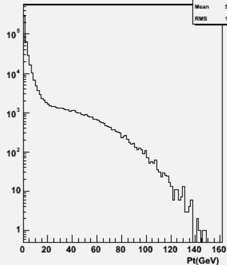
Particle Pt : w101800 n1n1n1n1cc_o
