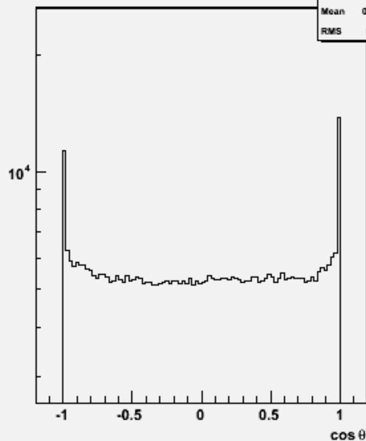
Particle cosθ : w101800 n1n1n1n1cc_o
