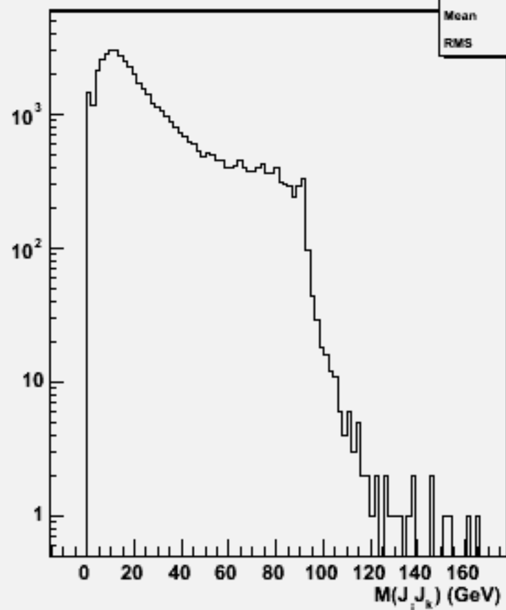
2jets mass(All comb)w101800 n1n1n1n1cc_o
