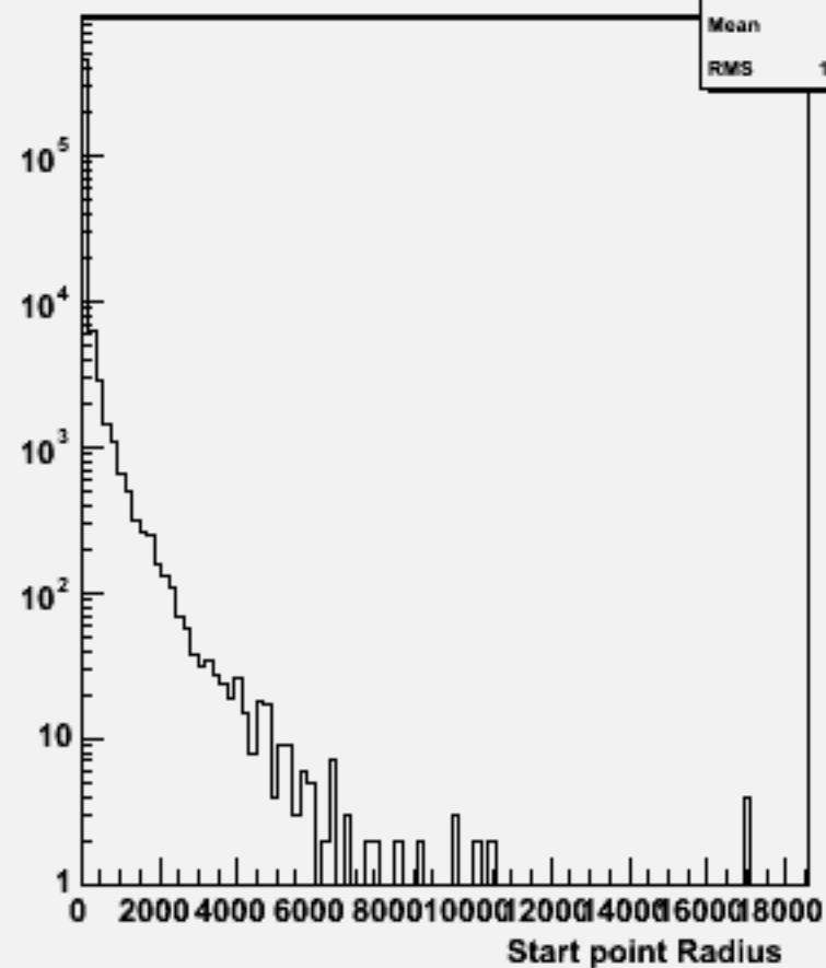
Start point R : w101800 n1n1n1n1cc_o
