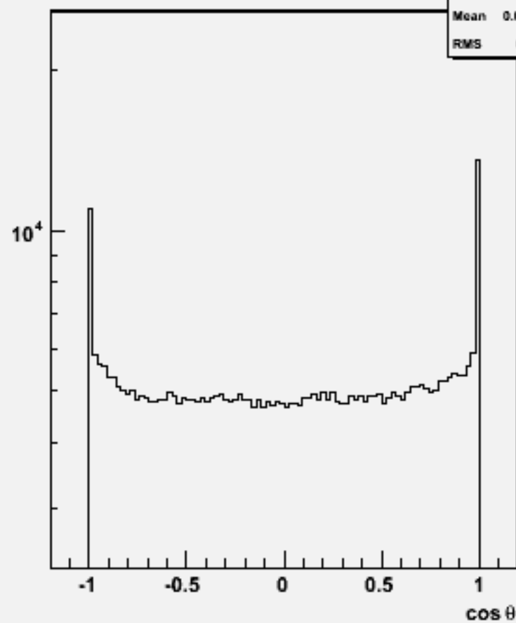
Particle cosθ : w101796 n1n1n1n1uu_o
