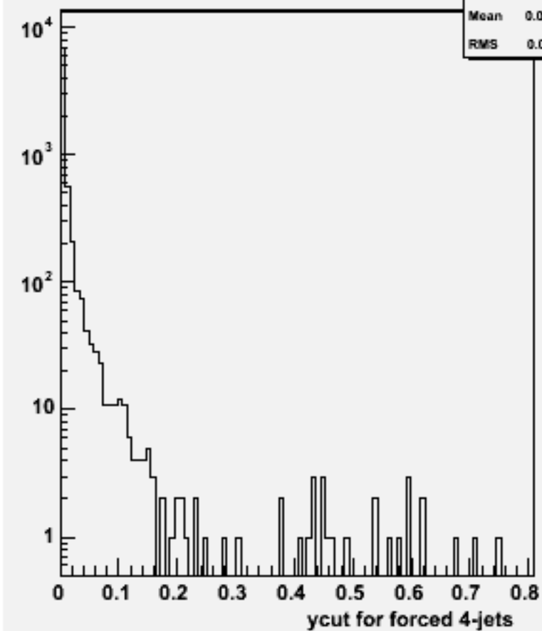
Ycut for 4-jets :w101796 n1n1n1n1uu_o
