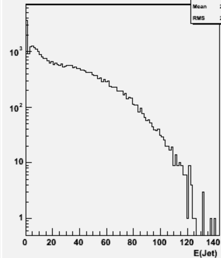
Jet energies(All jets)w101796 n1n1n1n1uu_o
