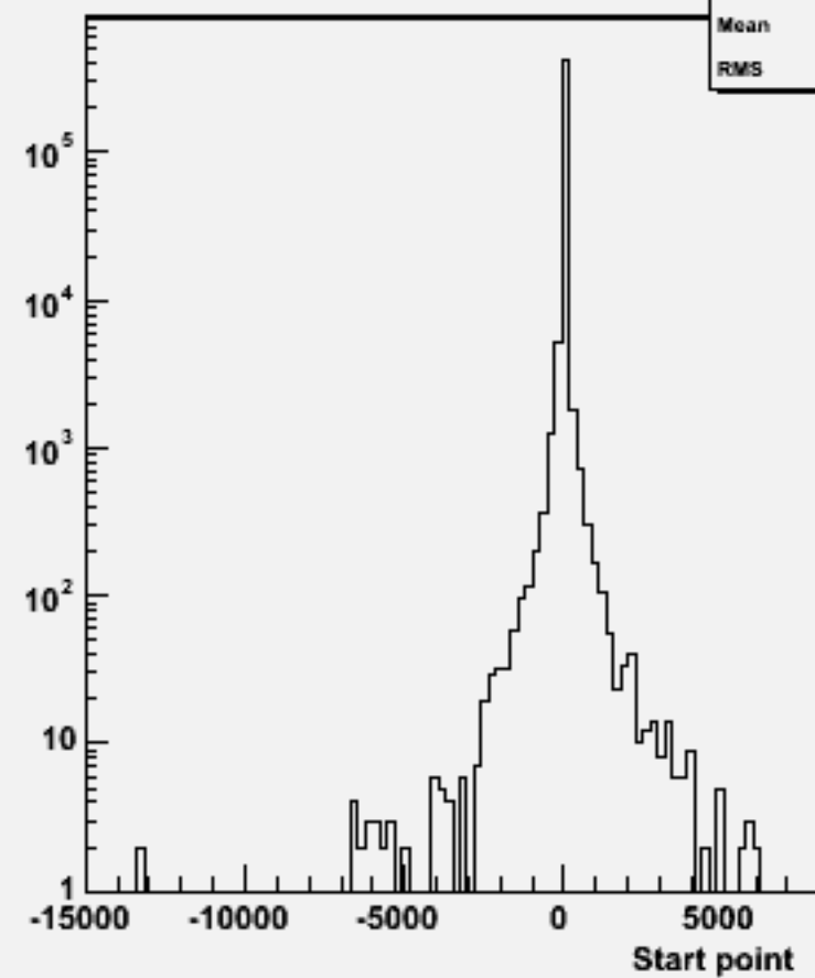
Start point Z : w101796 n1n1n1n1uu_o
