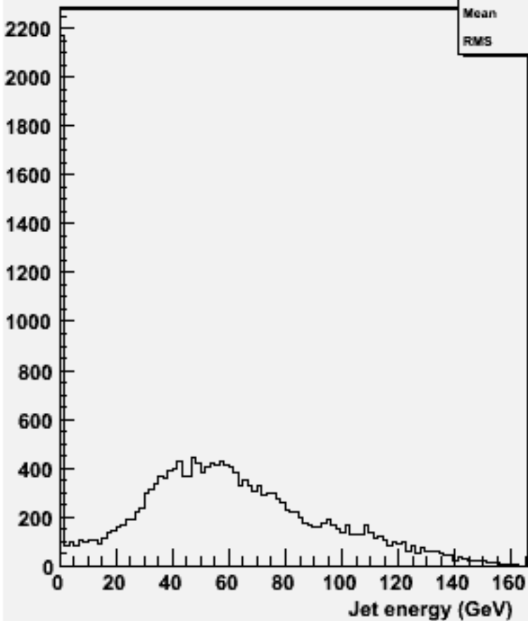
energy for 2-jets :w101796 n1n1n1n1uu_o
