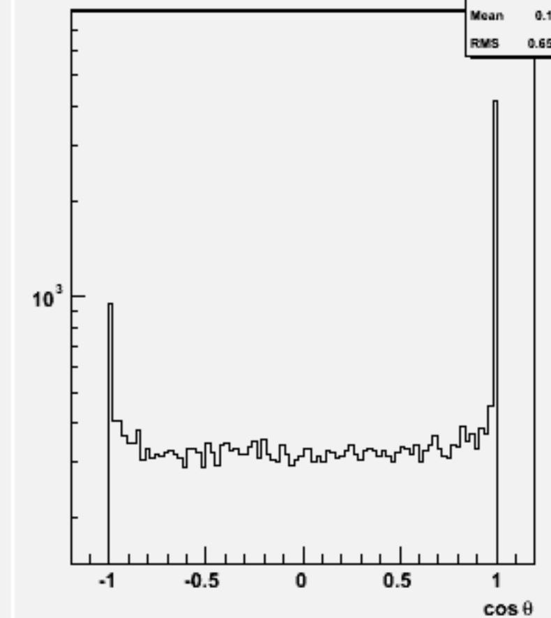
Jet cos \theta (All jets)w101796 n1n1n1n1uu_o
