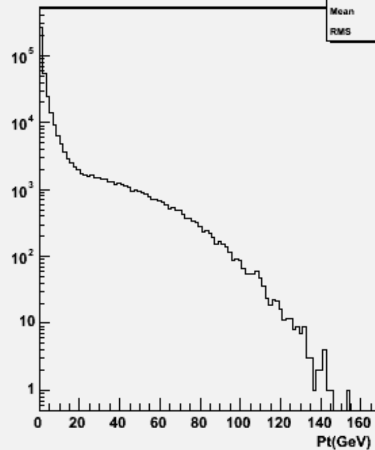
Particle Pt : w101796 n1n1n1n1uu_o
