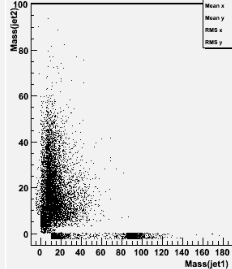
Jet mass for forced 2-jets : w101796 n1n1n1n1uu_o
