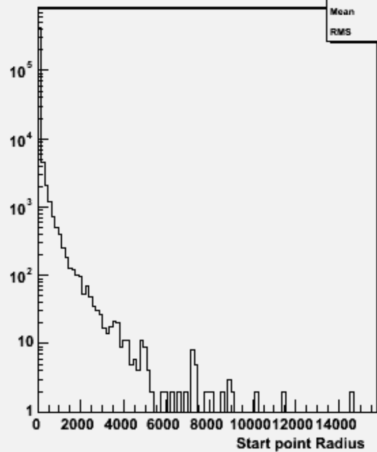
Start point R : w101796 n1n1n1n1uu_o
