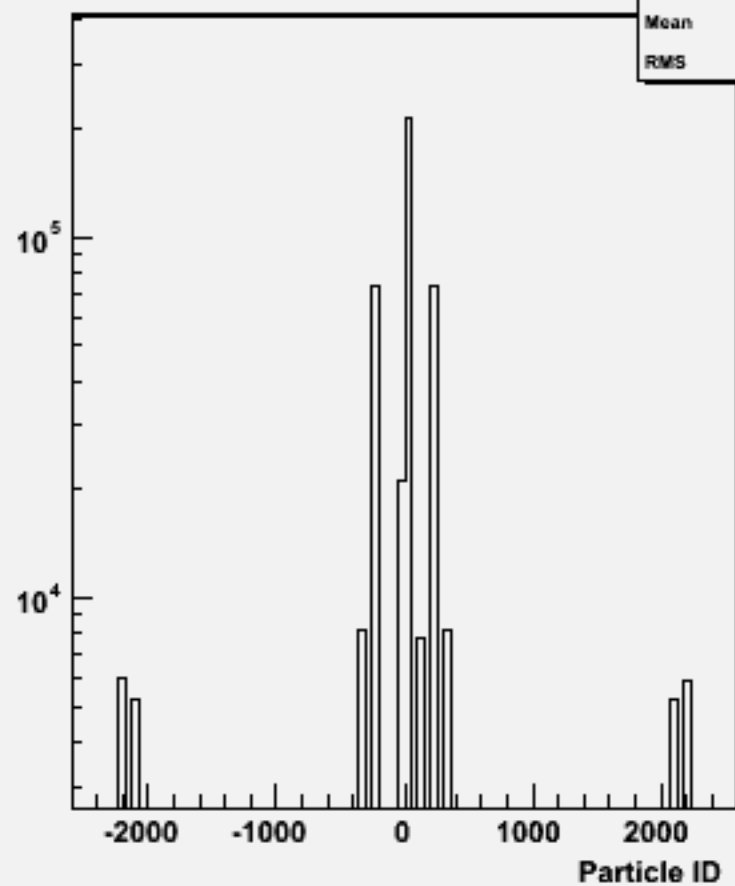
Particle ID : w101796 n1n1n1n1uu_o
