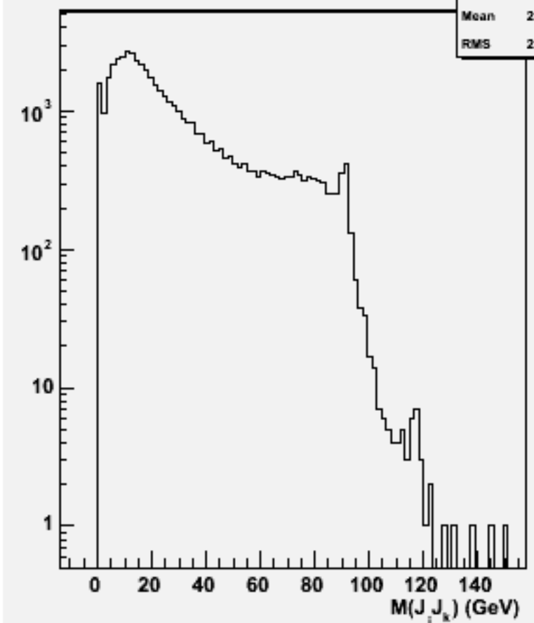
2jets mass(All comb)w101796 n1n1n1n1uu_o
