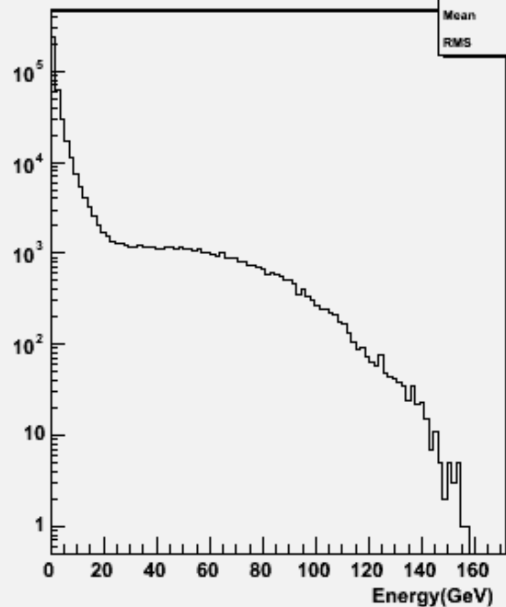
Particle Energy : w101796 n1n1n1n1uu_o
