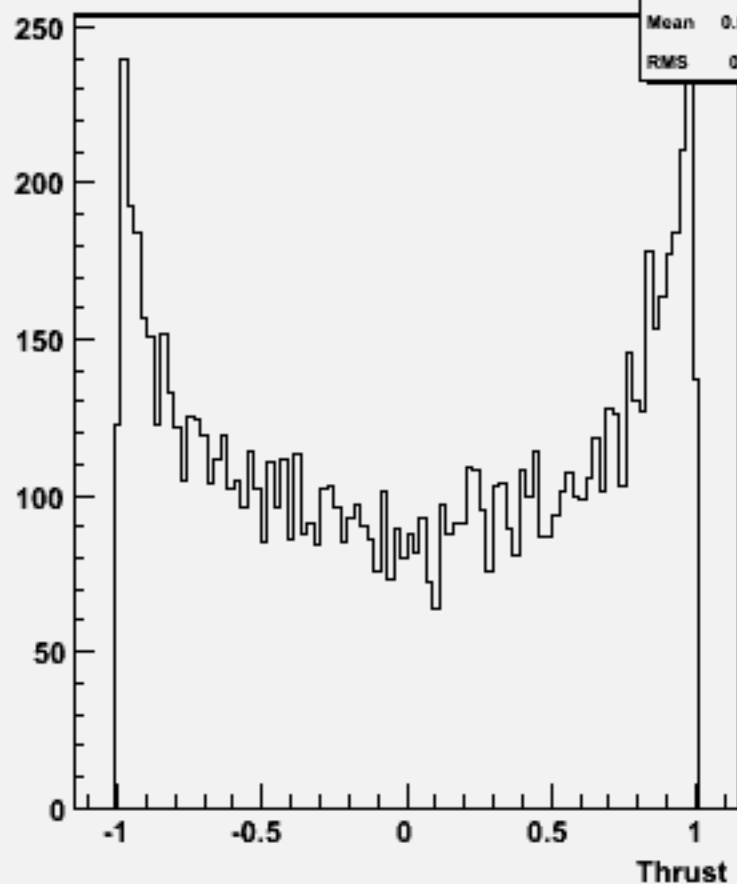
cos \Theta (thrust) w101793 cccssc_o
