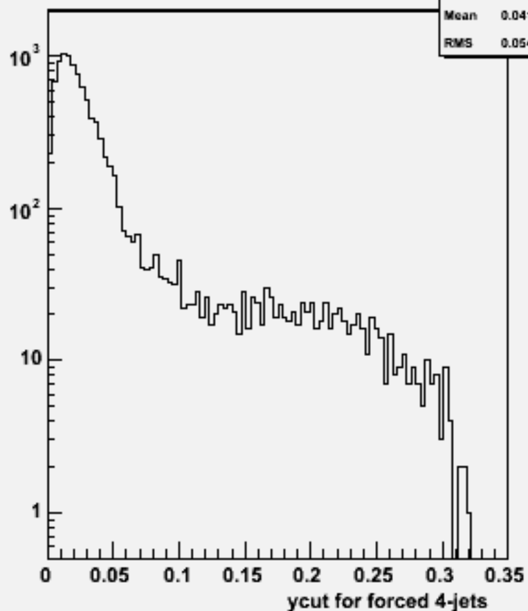
Ycut for 4-jets :w101793 cccssc_o
