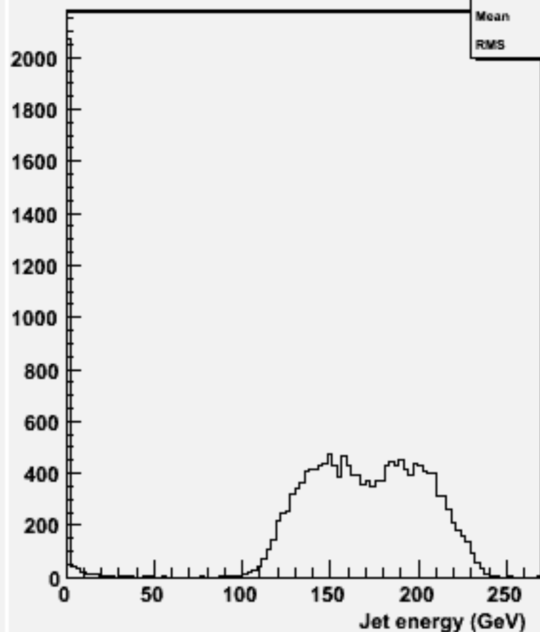
energy for 2-jets :w101793 cccssc_o
