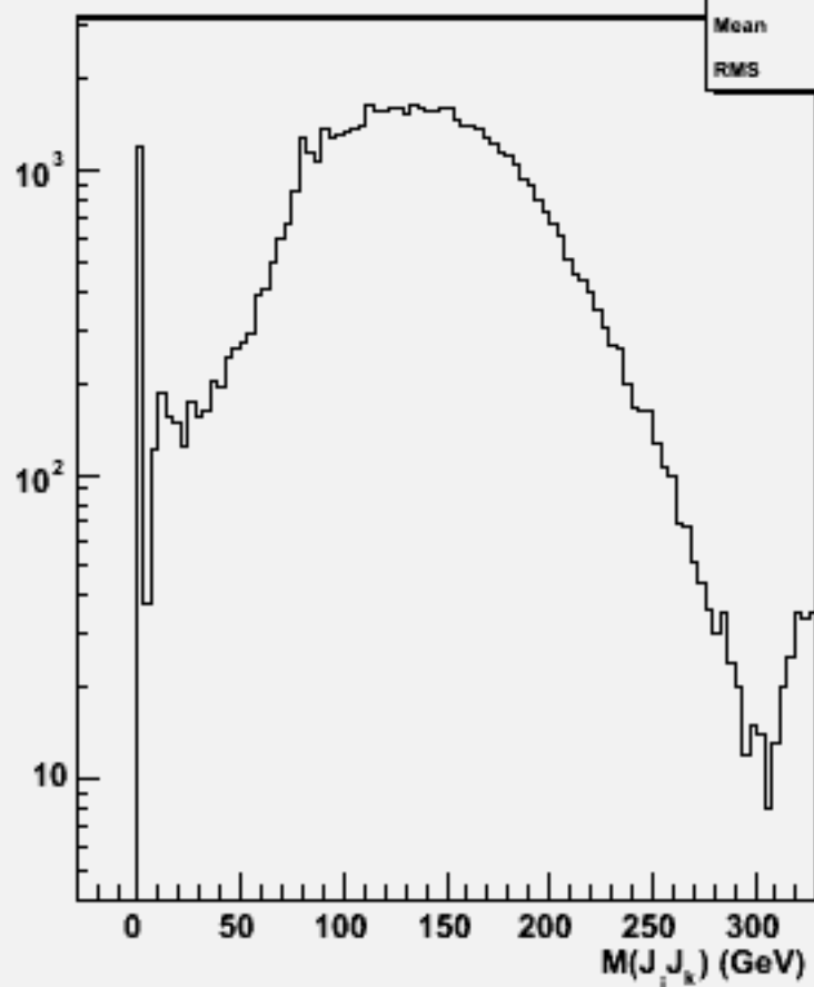
2jets mass(All comb)w101793 cccssc_o
