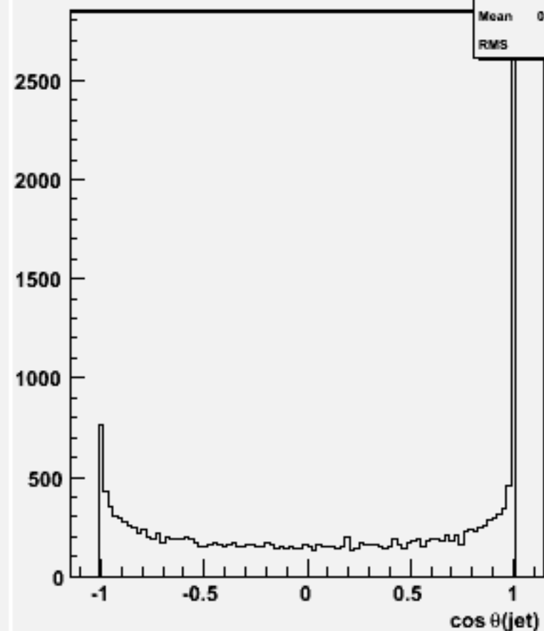
cos \theta for 2-jets :w101793 cccssc_o
