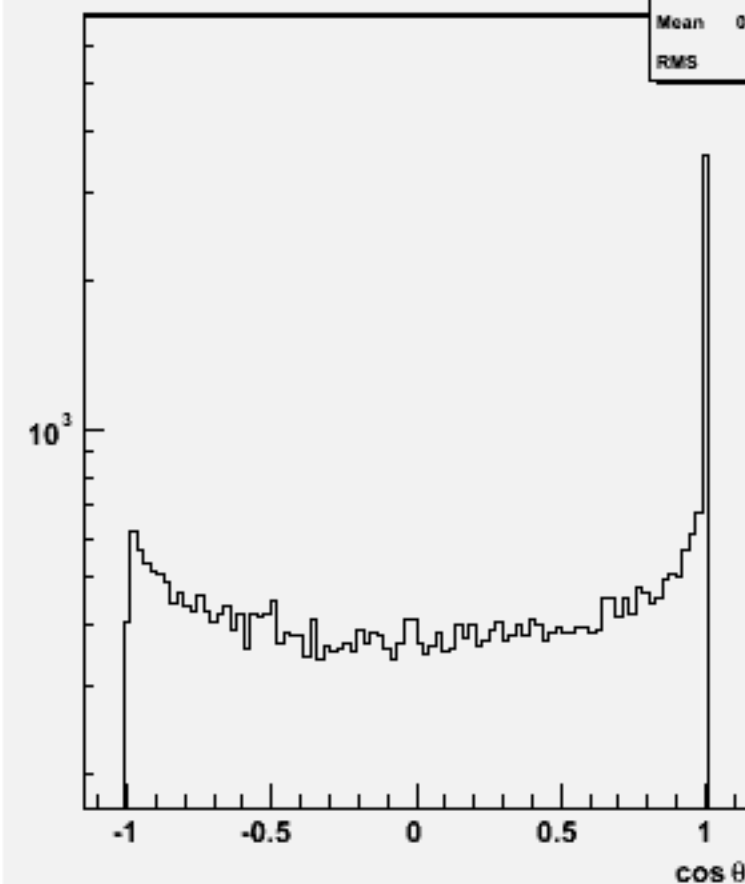
Jet cosθ (All jets)w101793 cccssc_o
