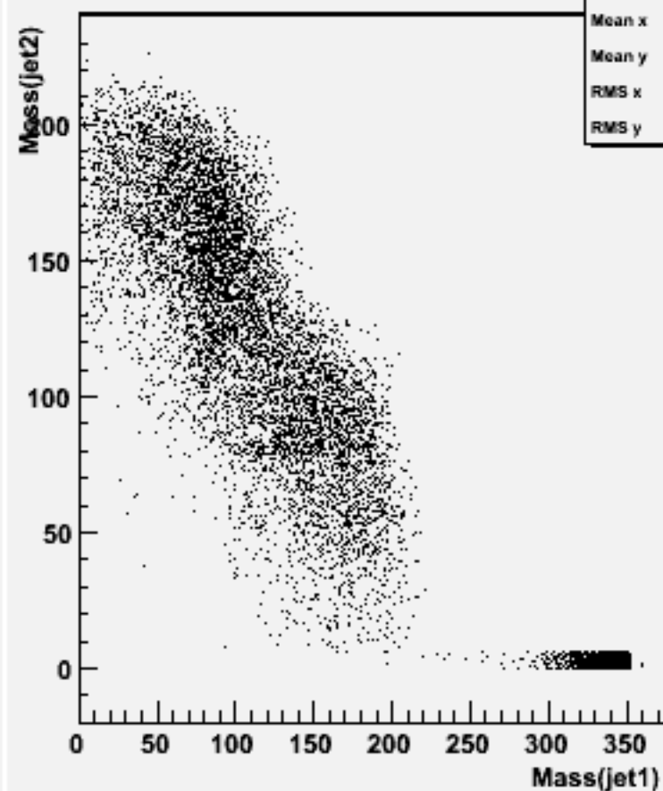
Jet mass for forced 2-jets : w101793 cccssc_o
