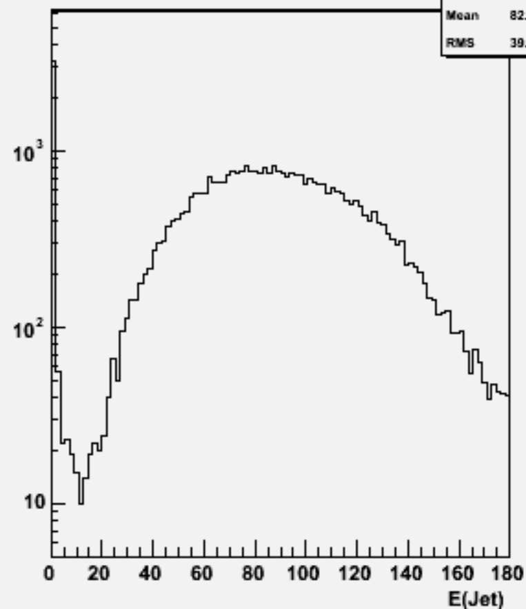
Jet energies(All jets)w101793 cccssc_o
