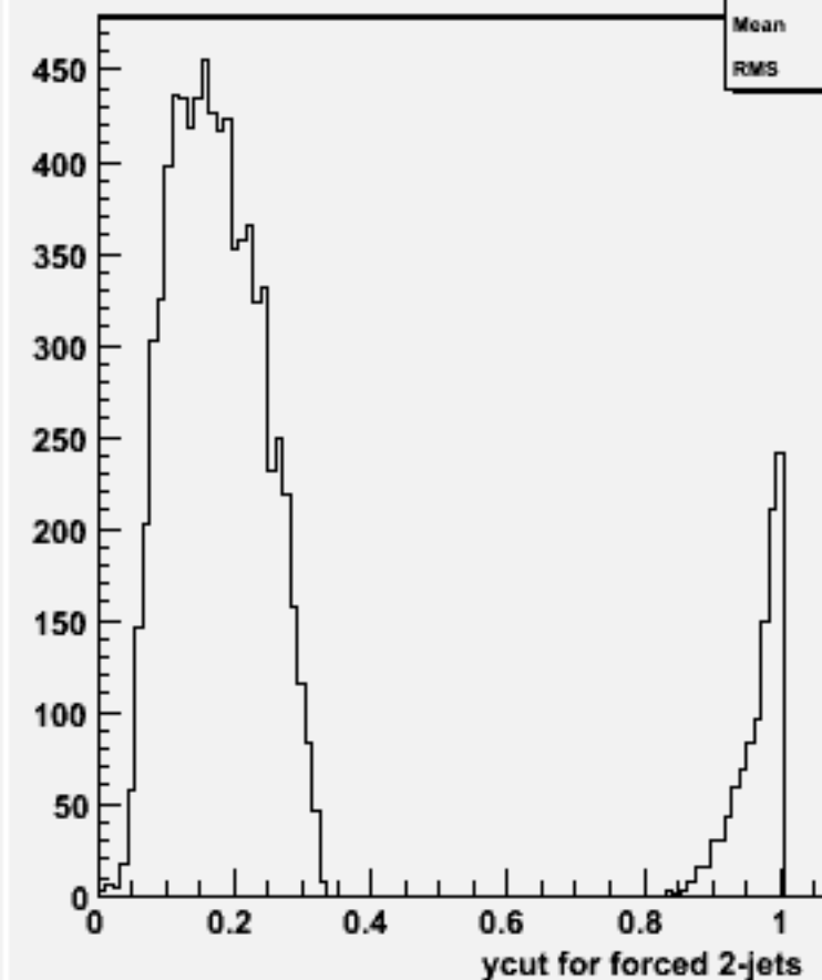
Ycut for 2-jets :w101793 cccssc_o
