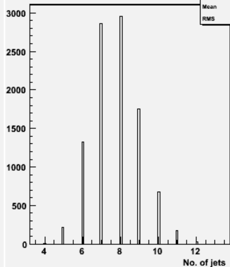
No. jets (ycut=0.001) : w101793 cccssc_o
