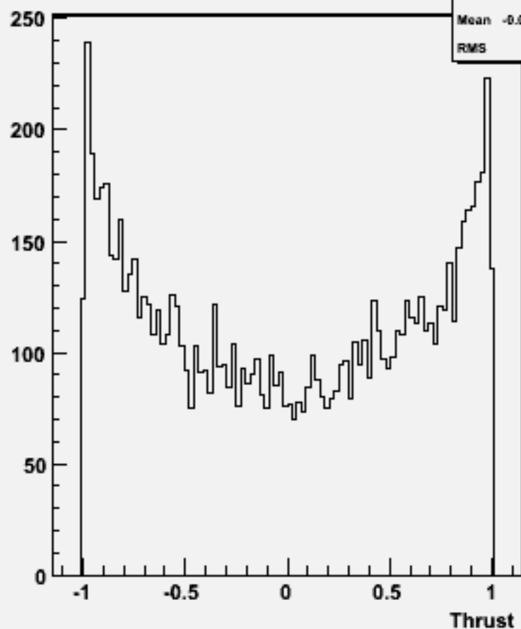
cos \Theta (thrust) w101792 cccssc_o
