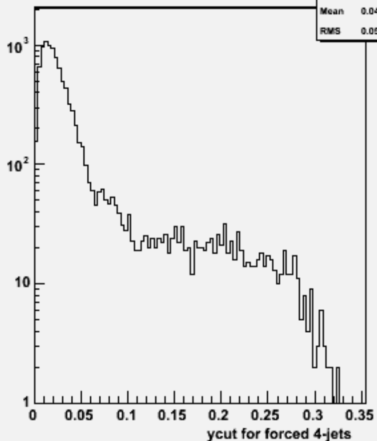
Ycut for 4-jets :w101792 cccssc_o
