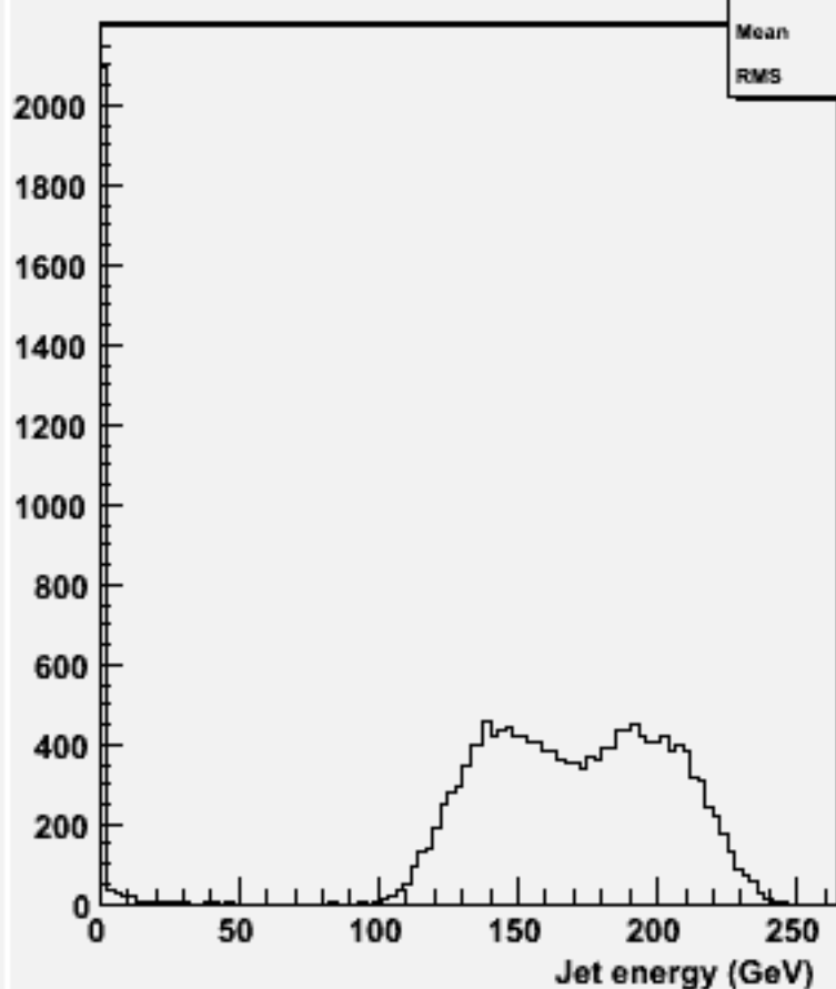
energy for 2-jets :w101792 cccssc_o
