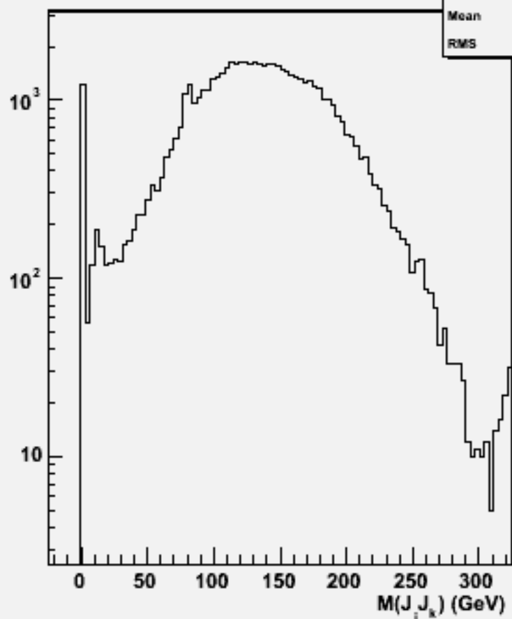
2jets mass(All comb)w101792 cccssc_o
