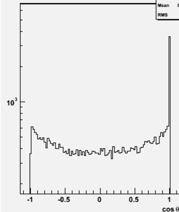
Jet cosθ (All jets)w101792 cccssc_o
