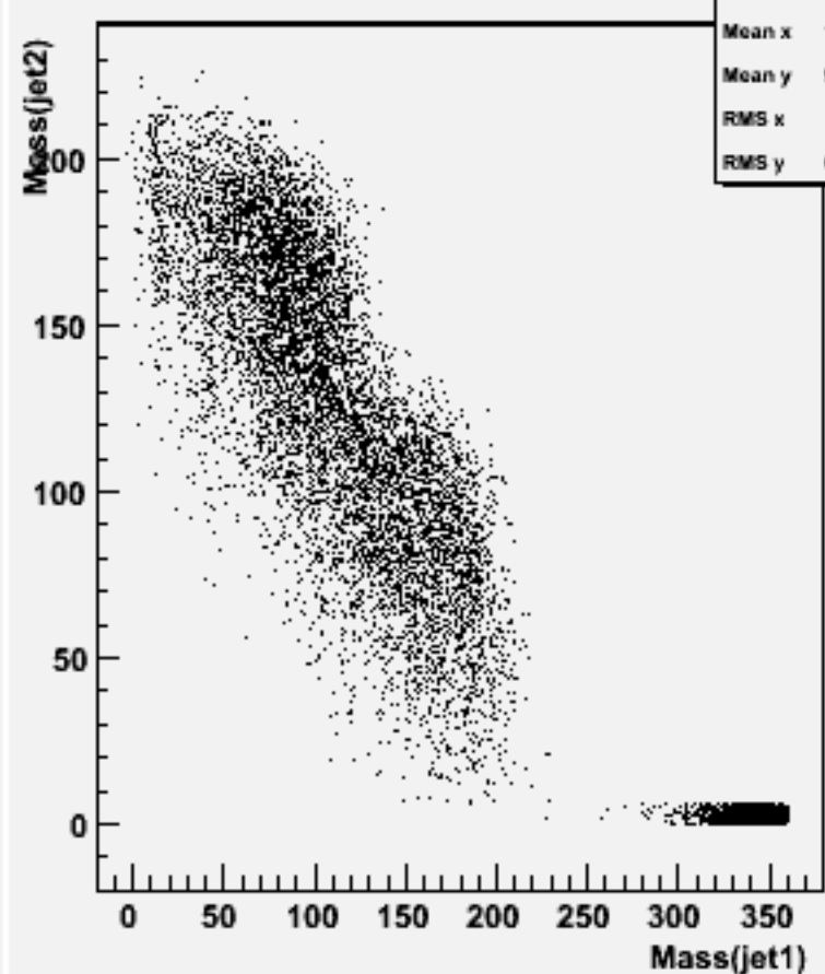
Jet mass for forced 2-jets : w101792 cccssc_o
