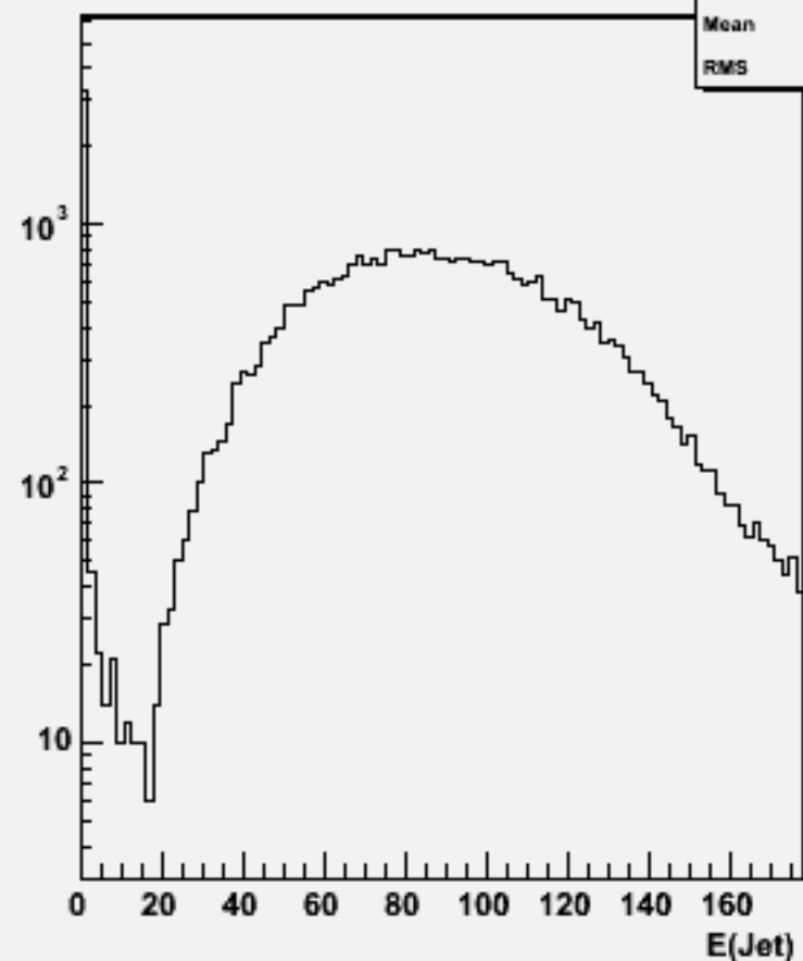
Jet energies(All jets)w101792 cccssc_o
