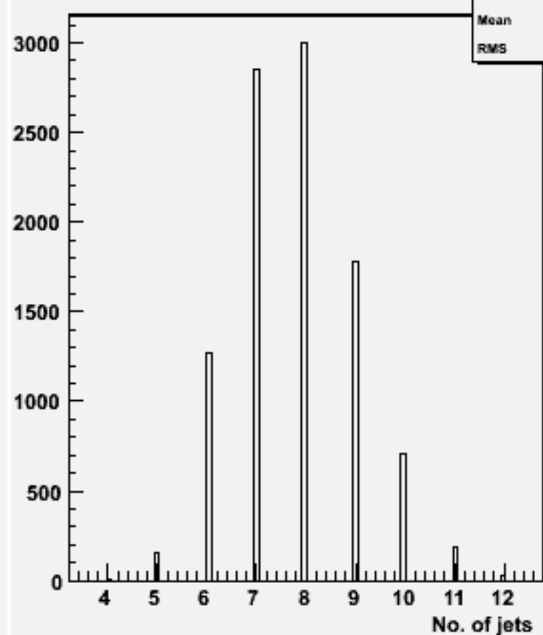
No. jets (ycut=0.001) : w101792 cccssc_o
