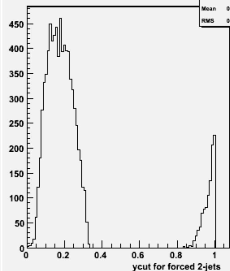
Ycut for 2-jets :w101792 cccssc_o
