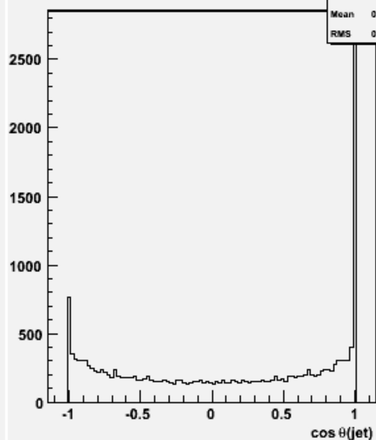
cos \theta for 2-jets :w101792 cccssc_o
