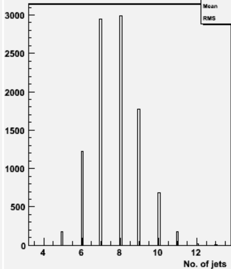
No. jets (ycut=0.001) : w101789 cccsdu_o
