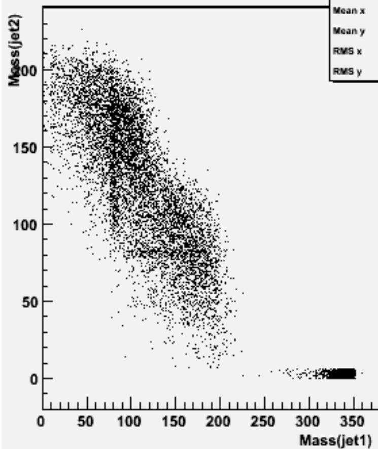
Jet mass for forced 2-jets : w101789 cccsdu_o
