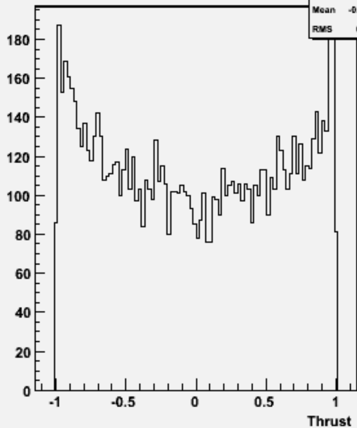
cos \Theta (thrust) w101789 cccsdu_o
