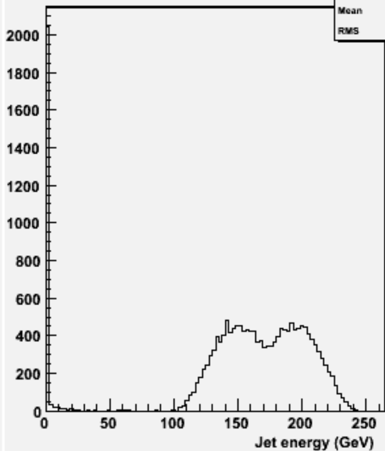
energy for 2-jets :w101789 cccsdu_o
