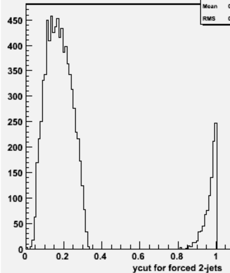
Ycut for 2-jets :w101789 cccsdu_o
