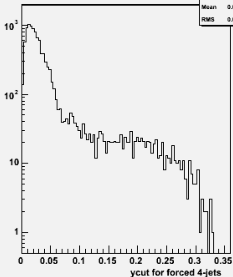
Ycut for 4-jets :w101789 cccsdu_o
