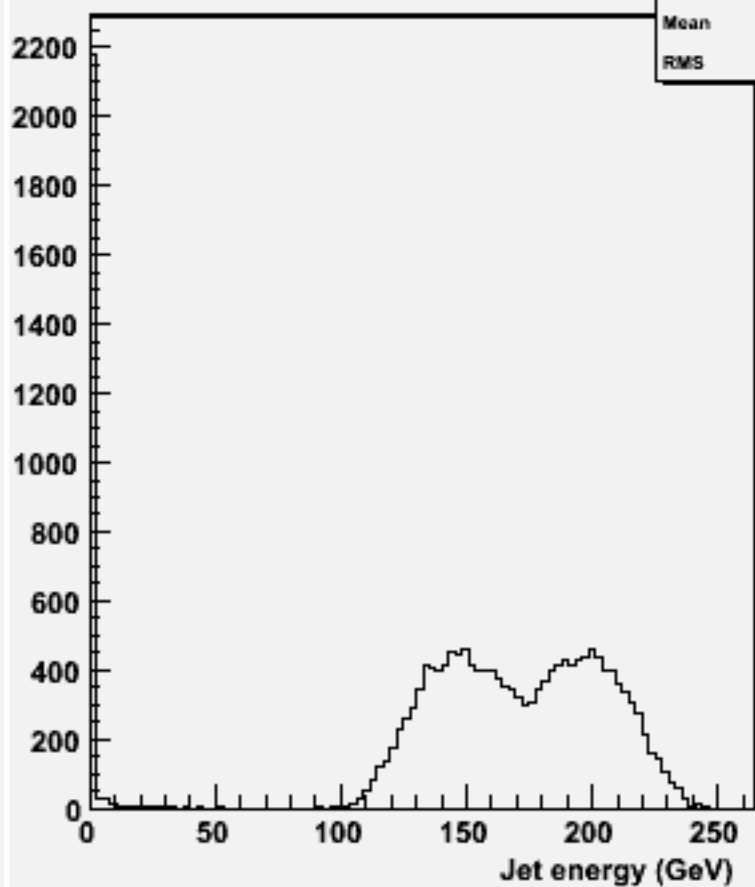
energy for 2-jets :w101788 cccsdu_o
