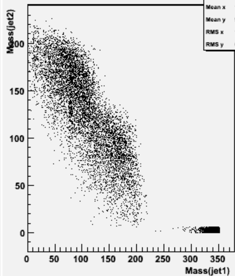
Jet mass for forced 2-jets : w101788 cccsdu_o
