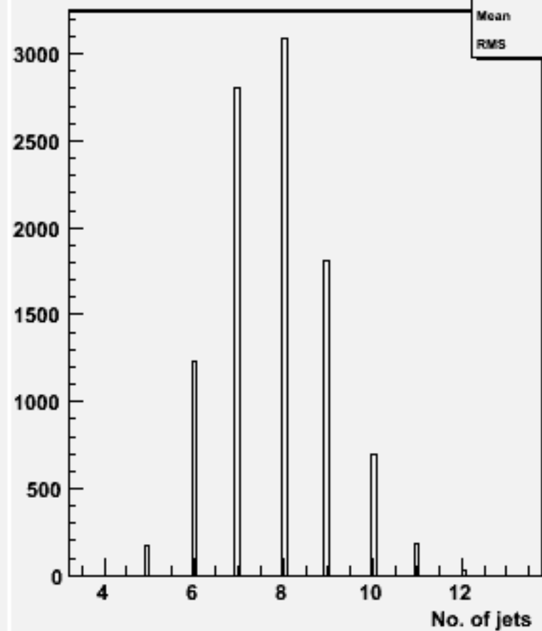
No. jets (ycut=0.001) : w101788 cccsdu_o
