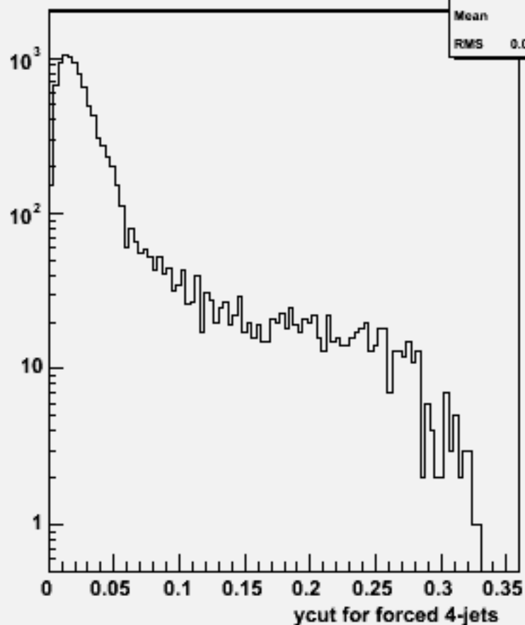
Ycut for 4-jets :w101788 cccsdu_o
