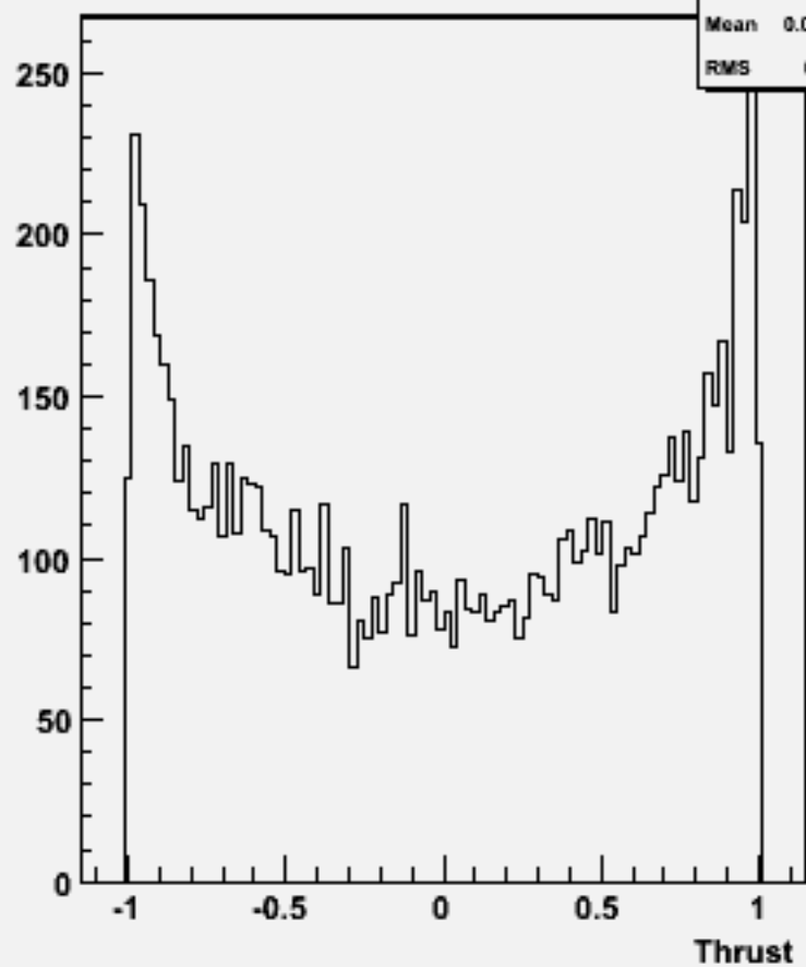
cos \Theta (thrust) w101788 cccsdu_o
