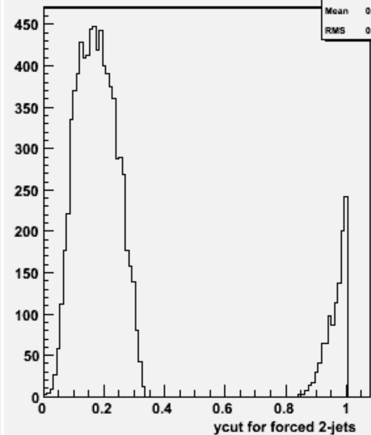
Ycut for 2-jets :w101788 cccsdu_o
