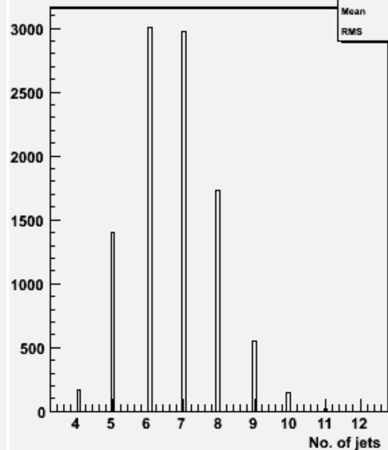
No. jets (ycut=0.001) : w101781 cccse2n2_o
