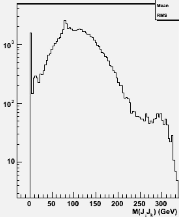
2jets mass(All comb)w101781 cccse2n2_o
