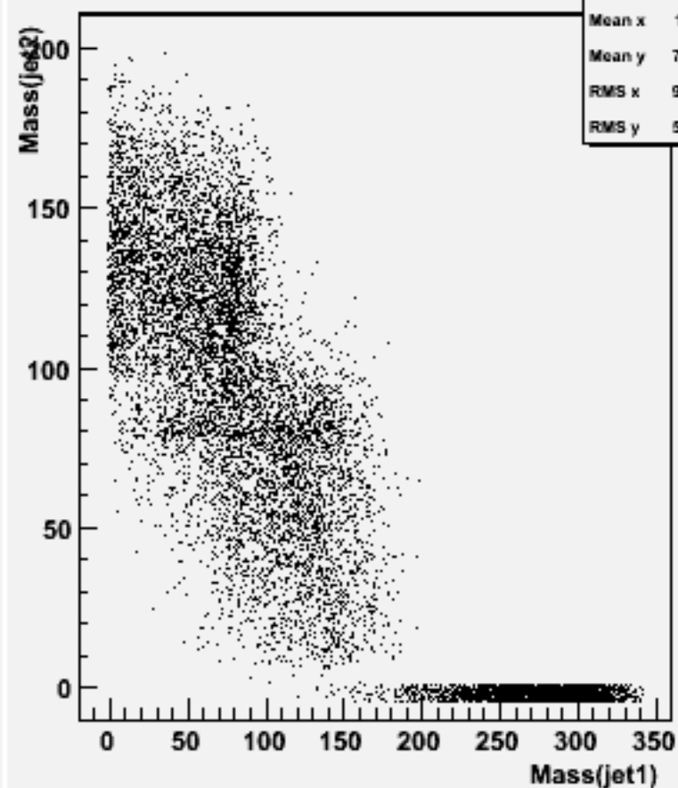
Jet mass for forced 2-jets : w101781 cccse2n2_o
