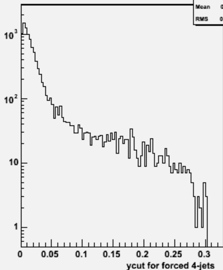
Ycut for 4-jets :w101781 cccse2n2_o
