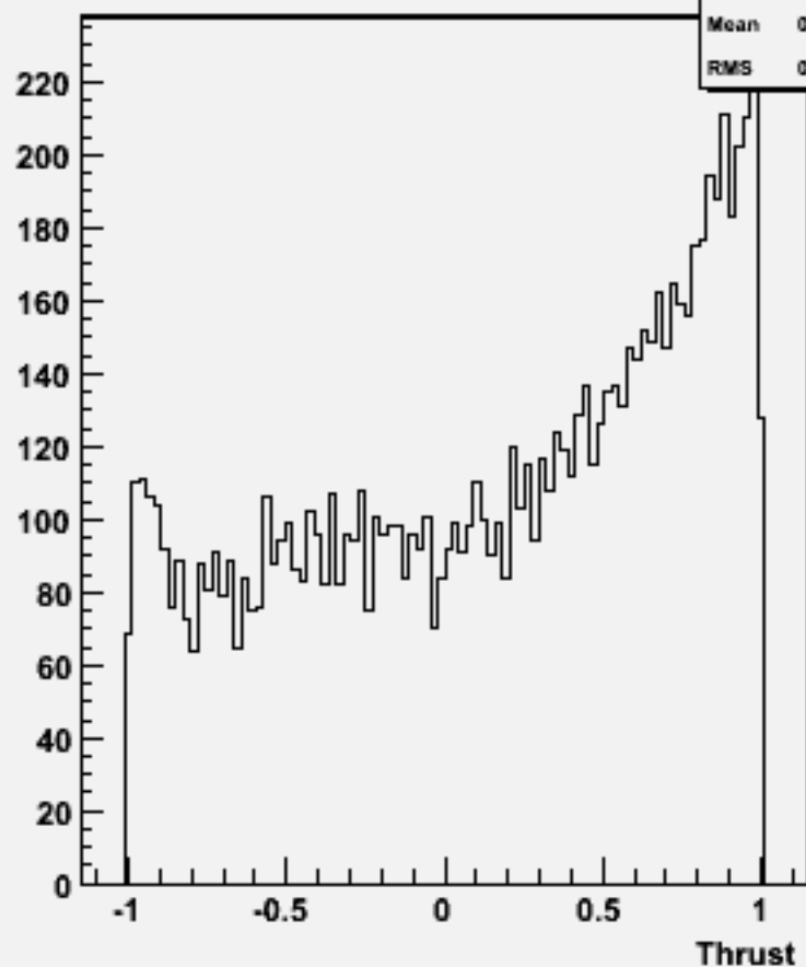
cos \Theta (thrust) w101781 cccse2n2_o
