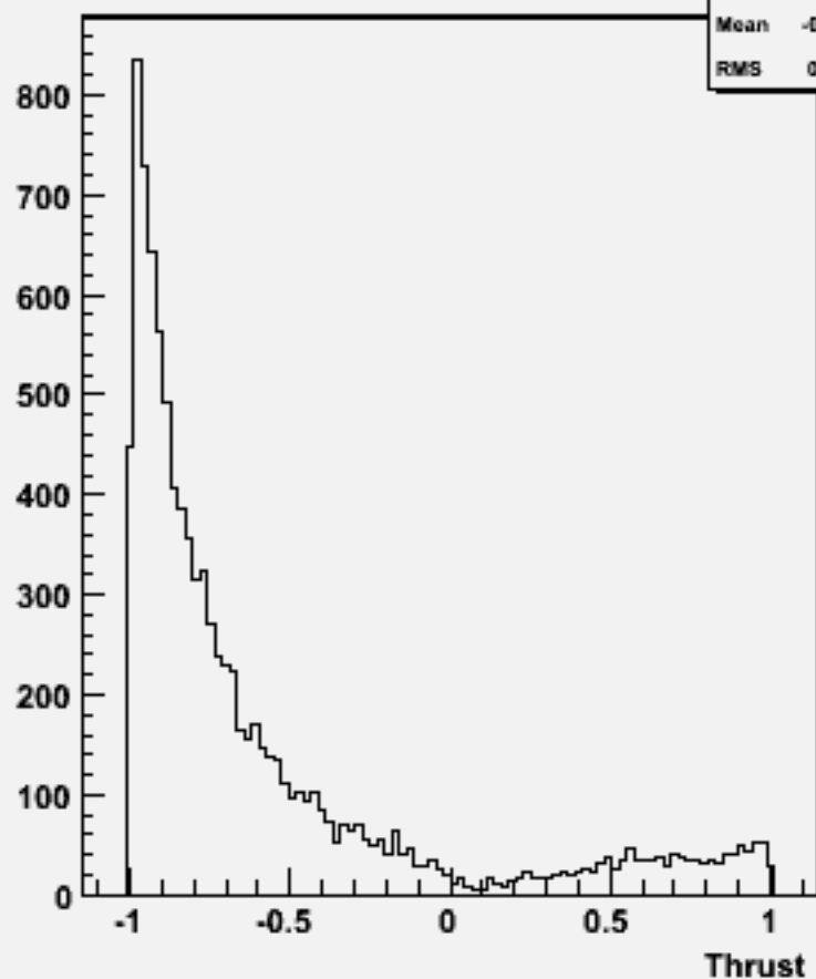
cos \Theta (thrust) w101778 cccse1n1_o
