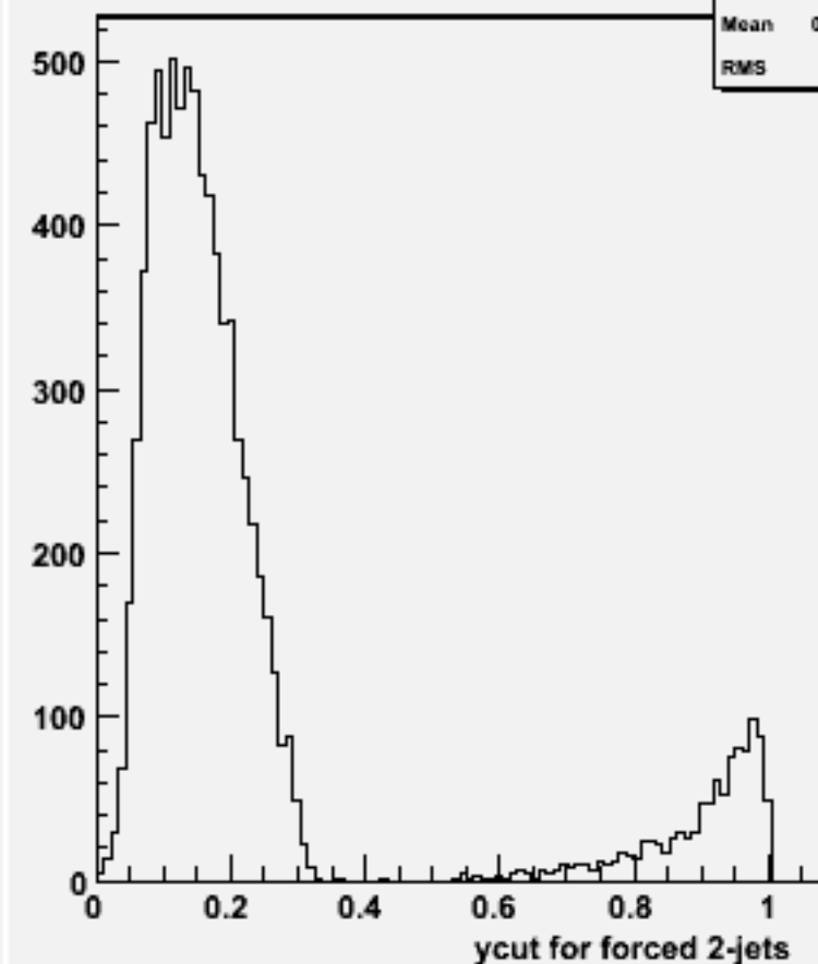
Ycut for 2-jets :w101778 cccse1n1_o
