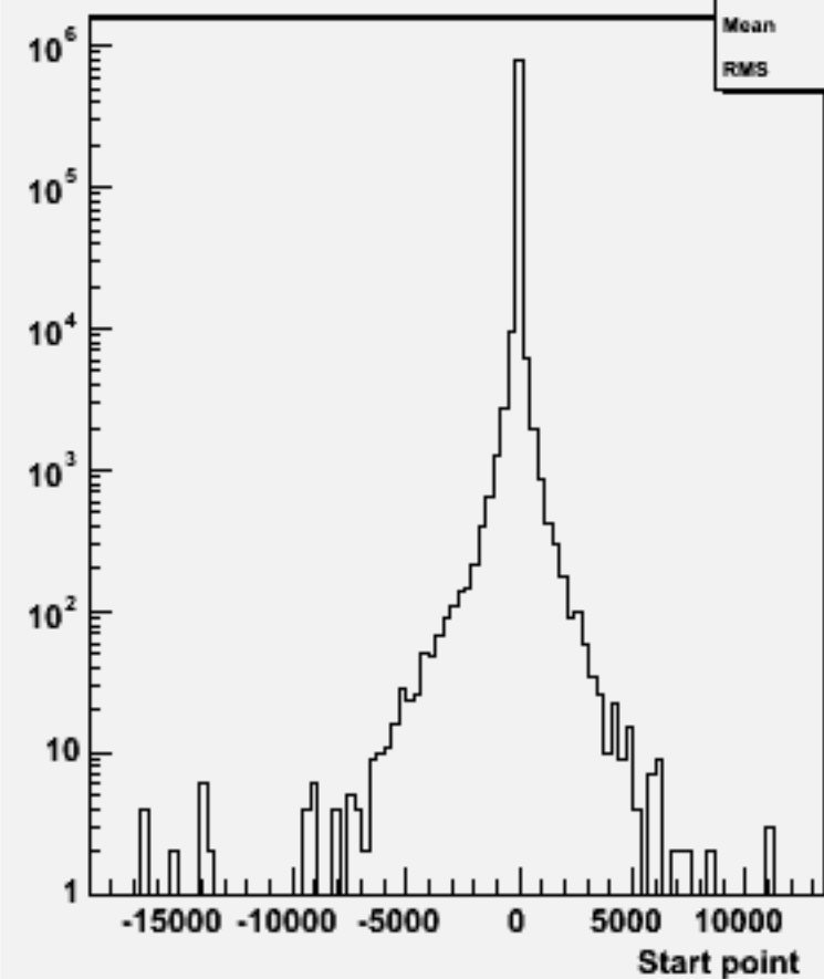
Start point Z : w101778 cccse1n1_o
