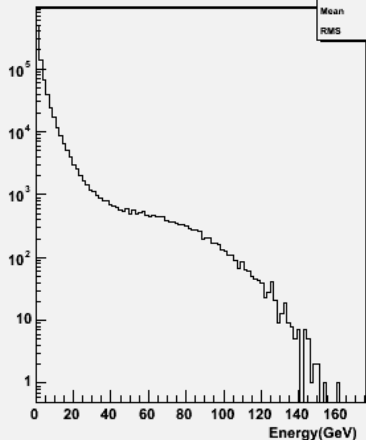
Particle Energy : w101778 cccse1n1_o
