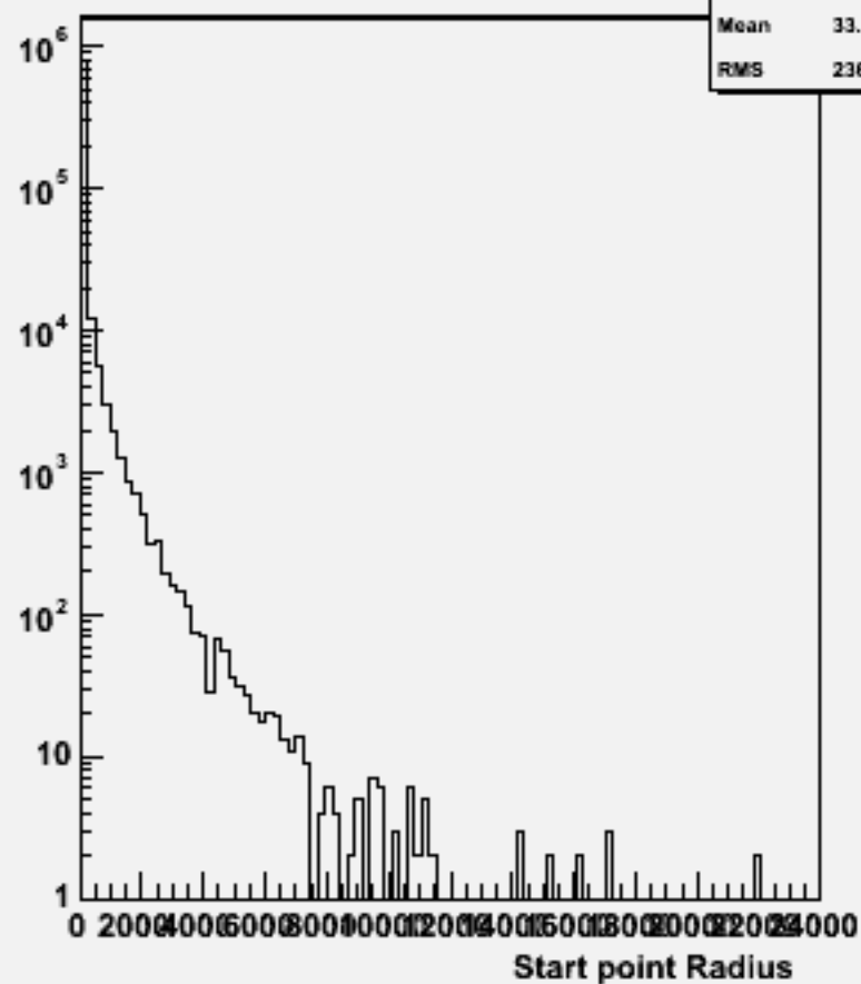
Start point R : w101778 cccse1n1_o
