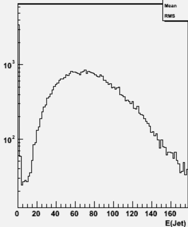
Jet energies(All jets)w101778 cccse1n1_o
