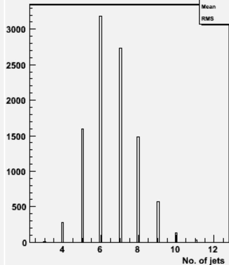
No. jets (ycut=0.001) : w101778 cccse1n1_o
