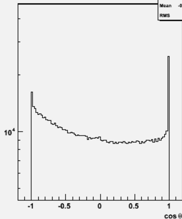
Particle cosθ : w101778 cccse1n1_o
