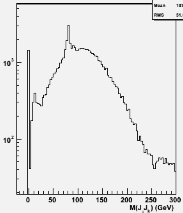
2jets mass(All comb)w101778 cccse1n1_o
