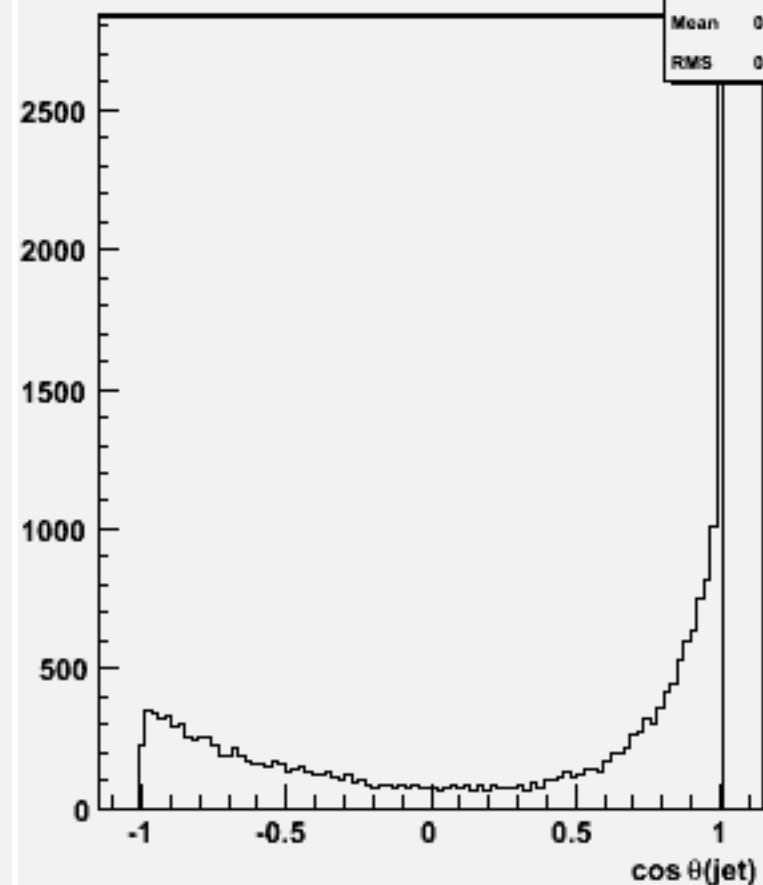
cos \theta for 2-jets :w101778 cccse1n1_o
