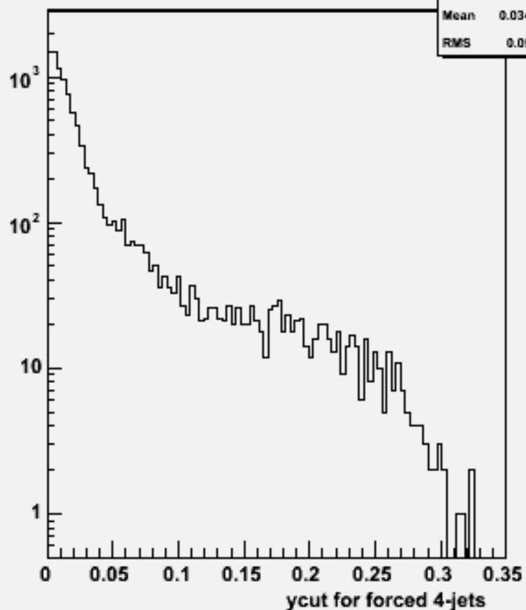
Ycut for 4-jets :w101778 cccse1n1_o
