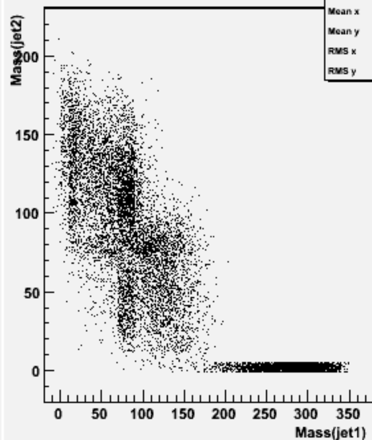
Jet mass for forced 2-jets : w101778 cccse1n1_o
