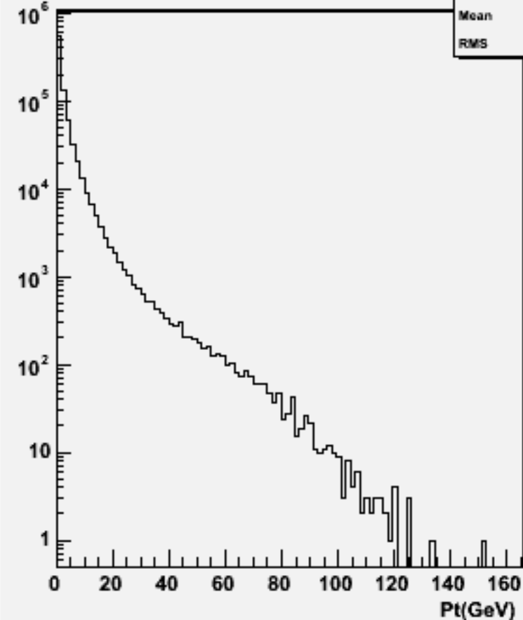
Particle Pt : w101778 cccse1n1_o
