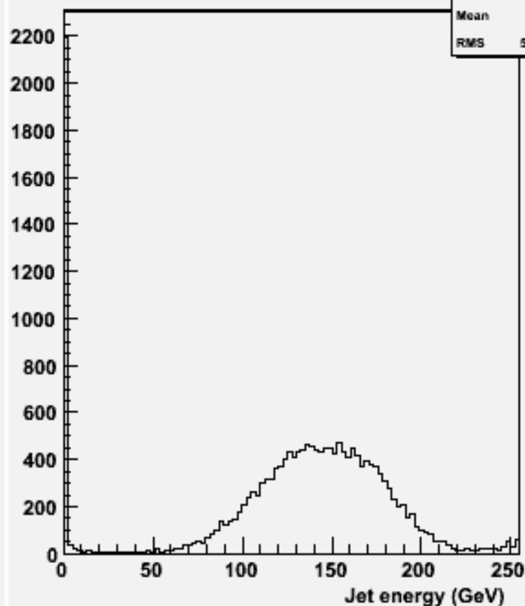
energy for 2-jets :w101778 cccse1n1_o
