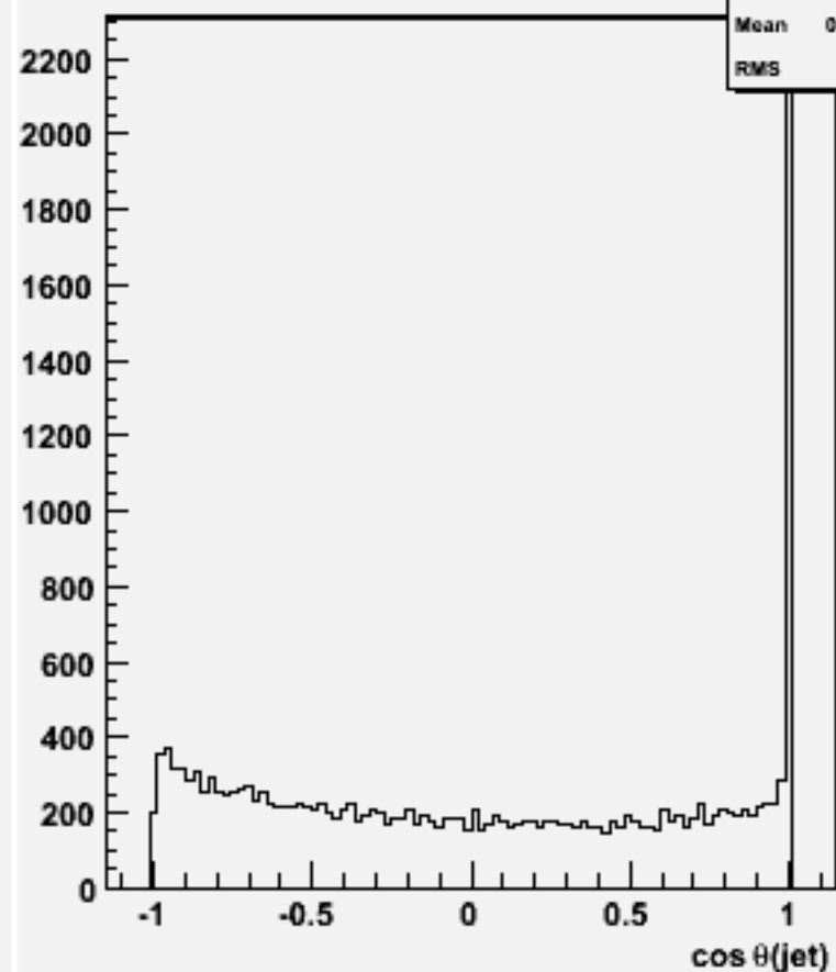
cos \theta for 2-jets :w101777 cccse1n1_o
