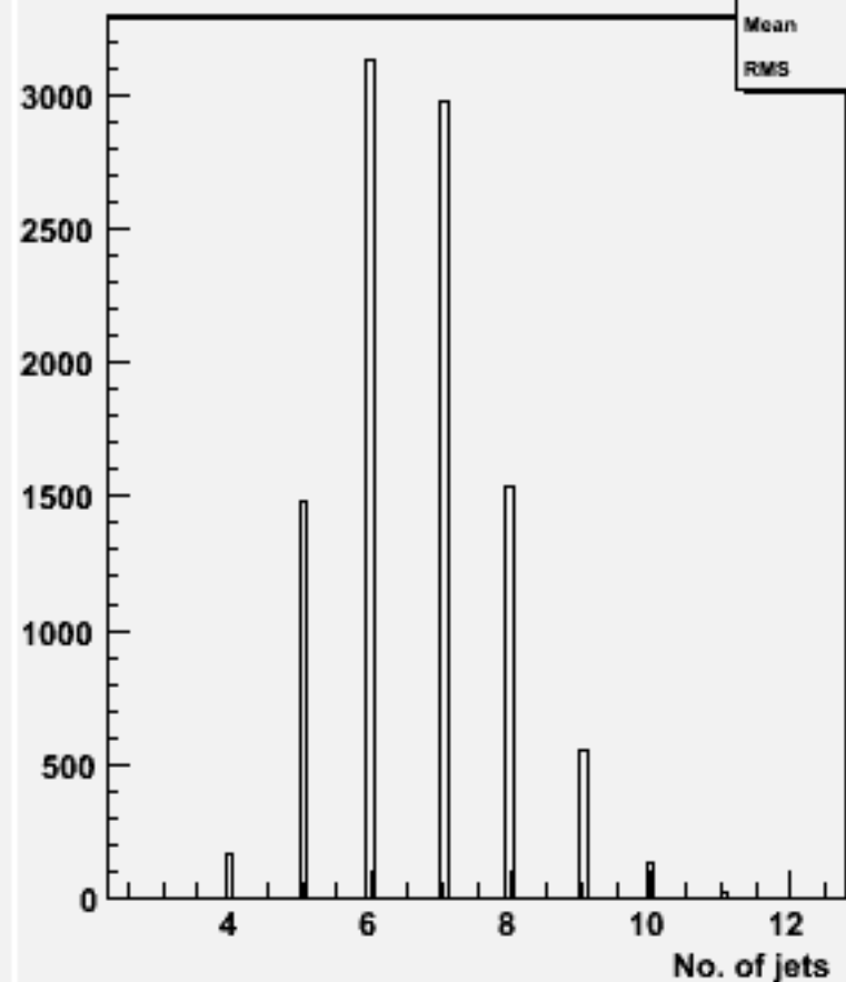
No. jets (ycut=0.001) : w101777 cccse1n1_o
