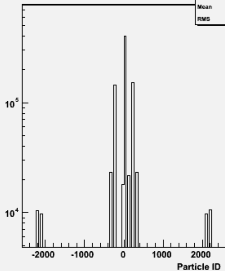
Particle ID : w101777 cccse1n1_o
