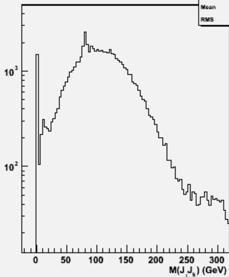
2jets mass(All comb)w101777 cccse1n1_o
