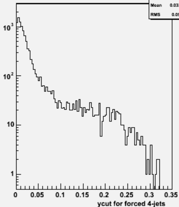
Ycut for 4-jets :w101777 cccse1n1_o
