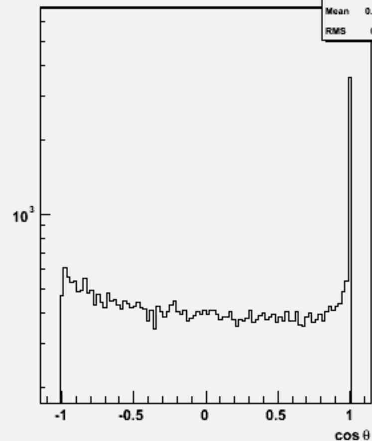
Jet cosθ (All jets)w101777 cccse1n1_o
