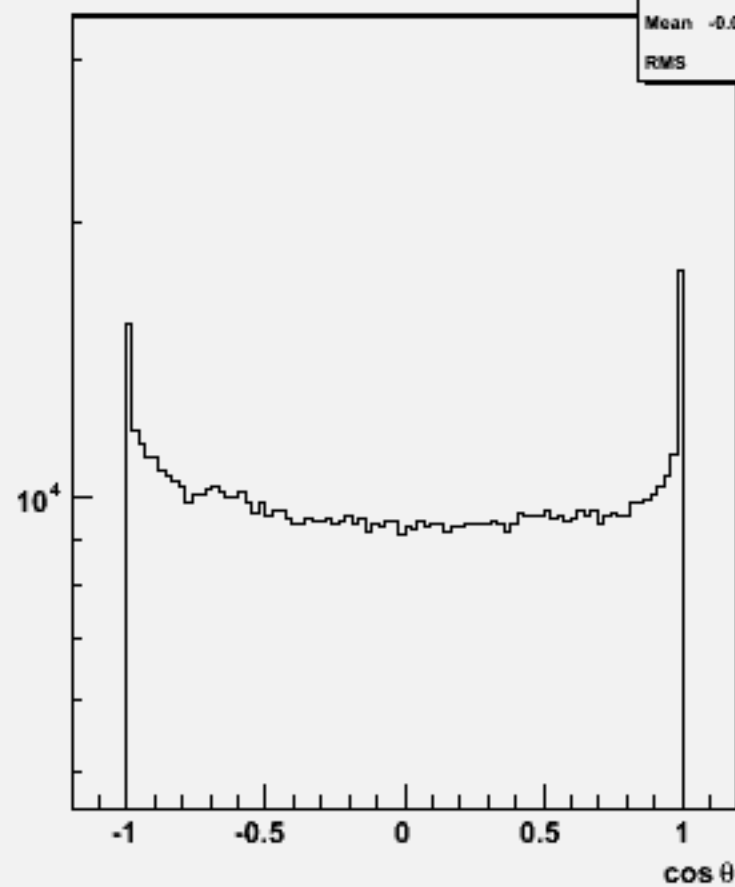
Particle cos \theta : w101777 cccse1n1_o
