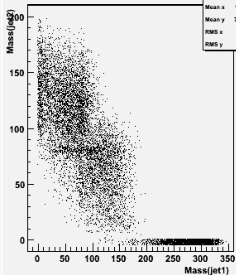
Jet mass for forced 2-jets : w101777 cccse1n1_o
