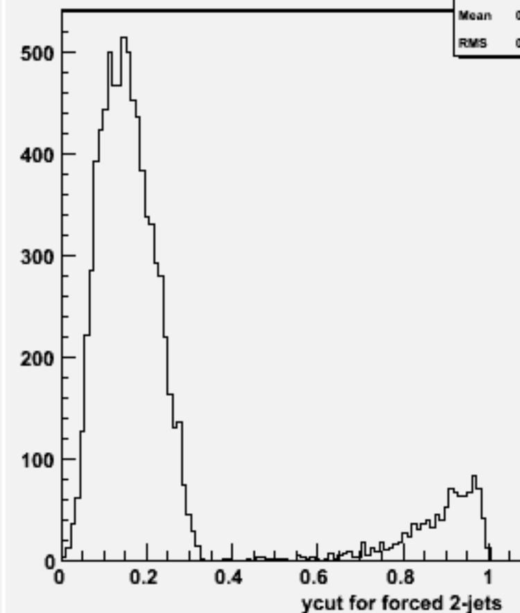
Ycut for 2-jets :w101777 cccse1n1_o
