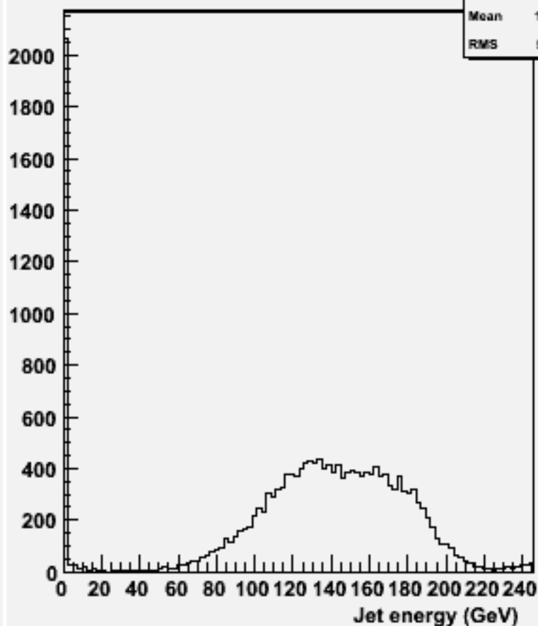
energy for 2-jets :w101777 cccse1n1_o
