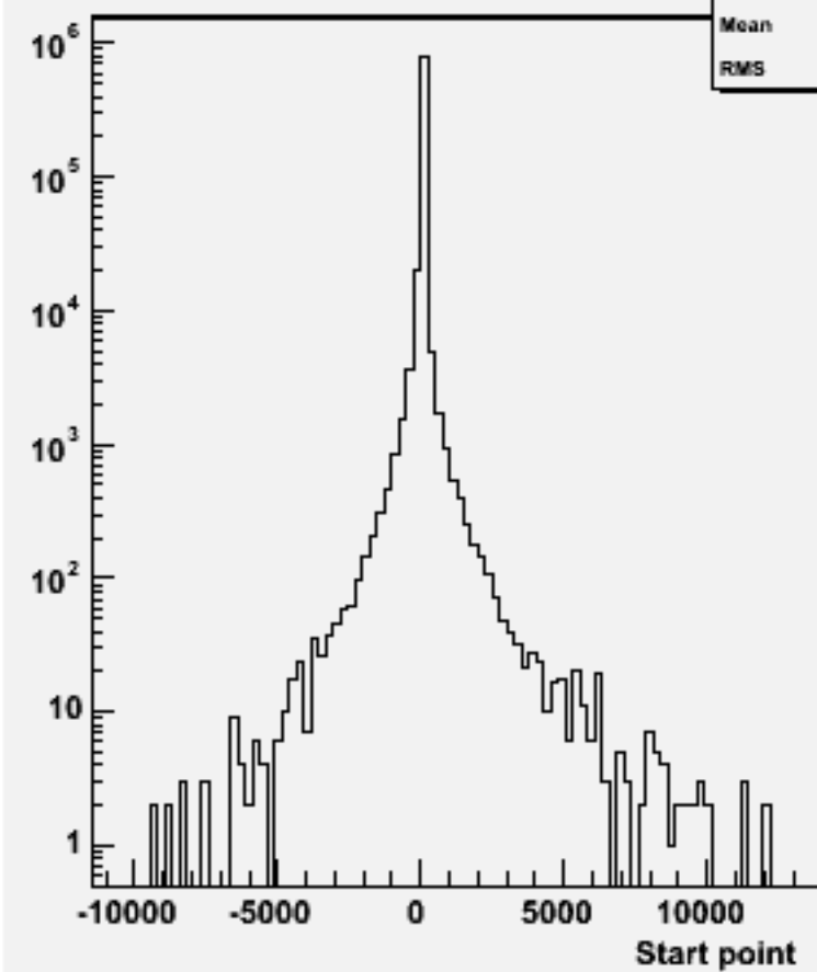
Start point Z : w101777 cccse1n1_o
