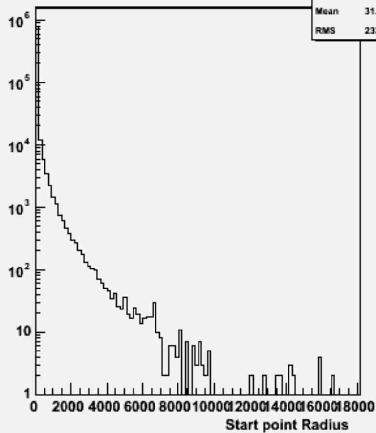
Start point R : w101777 cccse1n1_o
