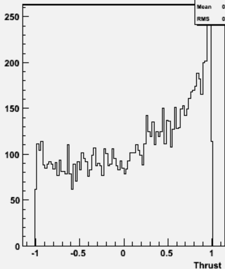
cos \Theta (thrust) w101777 cccse1n1_o
