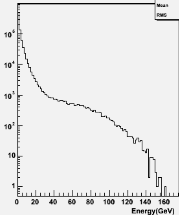
Start point R : w101777 cccse1n1_o
