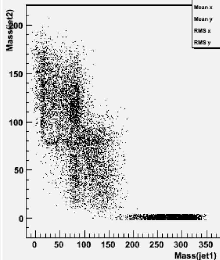
Jet mass for forced 2-jets : w101776 cccse1n1_o
