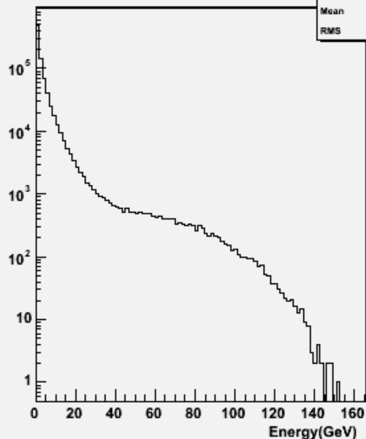
Particle Energy : w101776 cccse1n1_o
