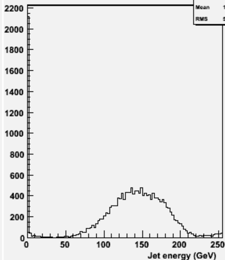
energy for 2-jets :w101776 cccse1n1_o
