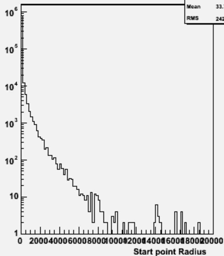
Start point R : w101776 cccse1n1_o
