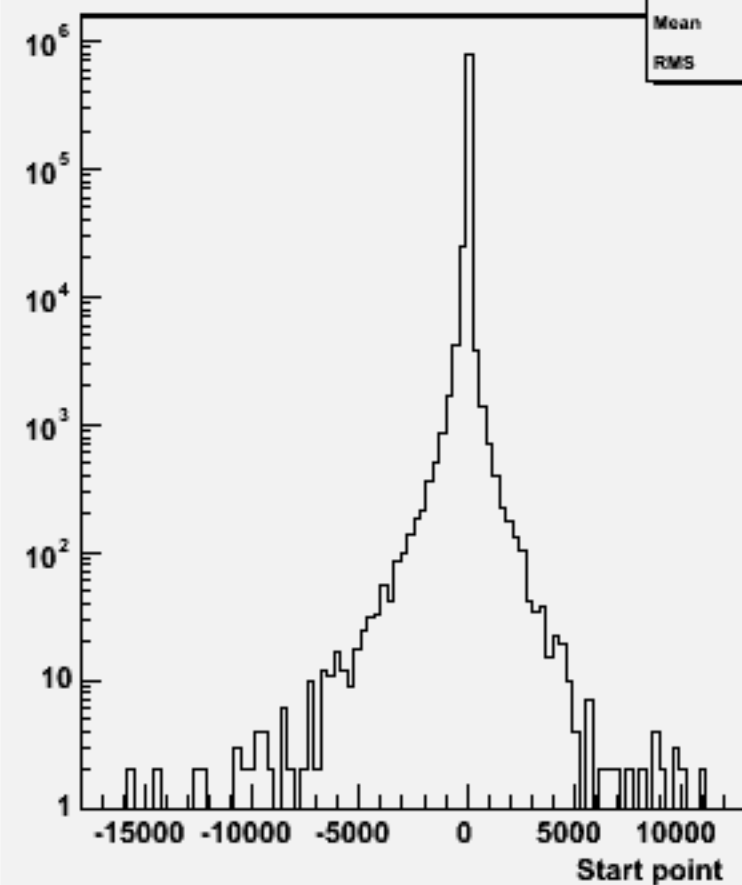
Start point Z : w101776 cccse1n1_o
