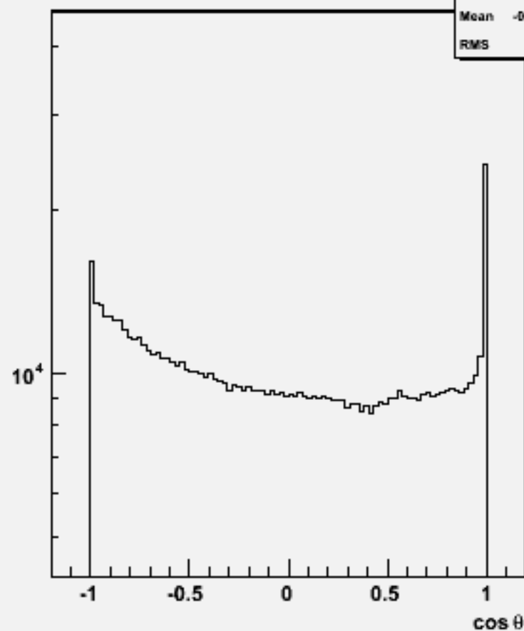
Particle cos \theta : w101776 cccse1n1_o
