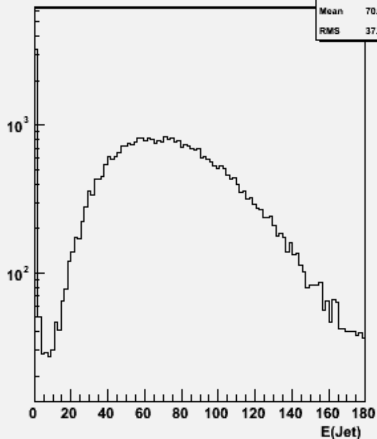
Jet energies(All jets)w101776 cccse1n1_o
