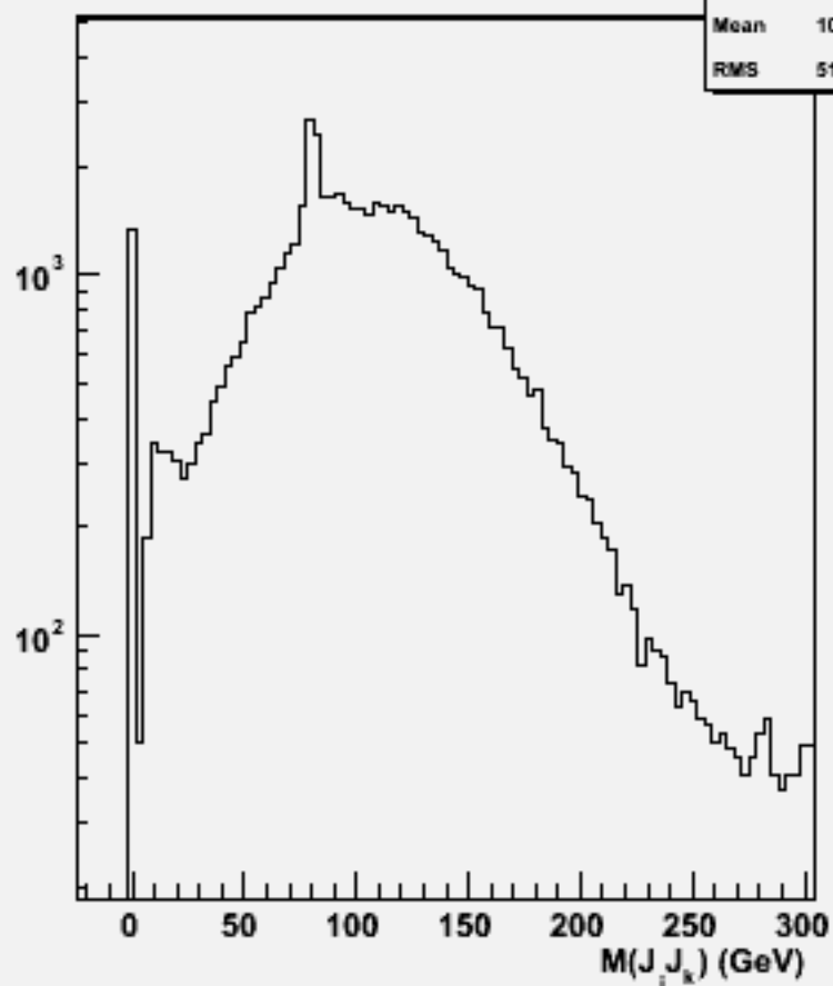
2jets mass(All comb)w101776 cccse1n1_o
