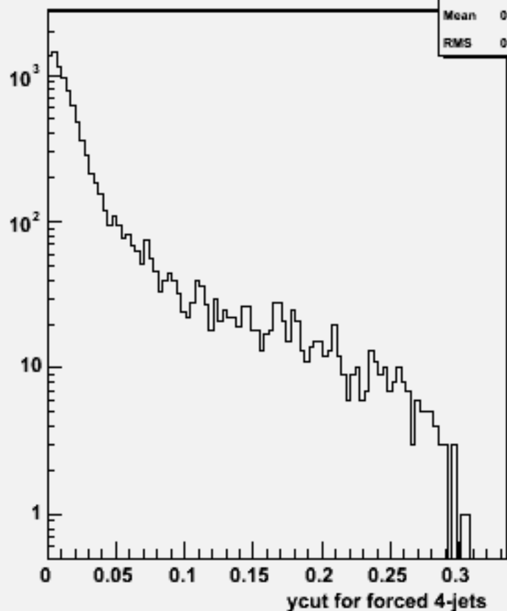
Ycut for 4-jets :w101776 cccse1n1_o
