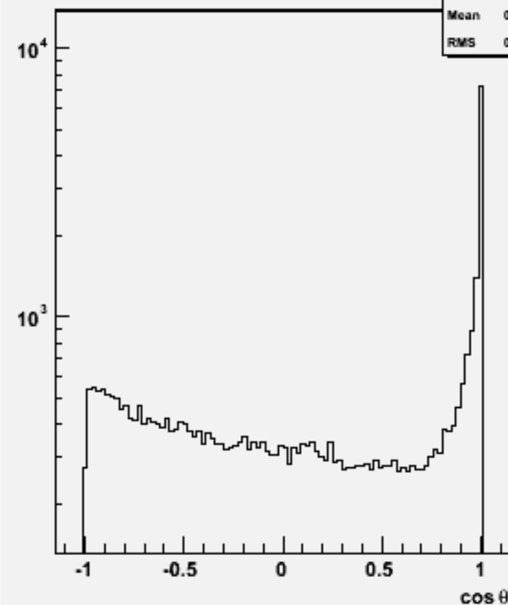
Jet cosθ (All jets)w101776 cccse1n1_o
