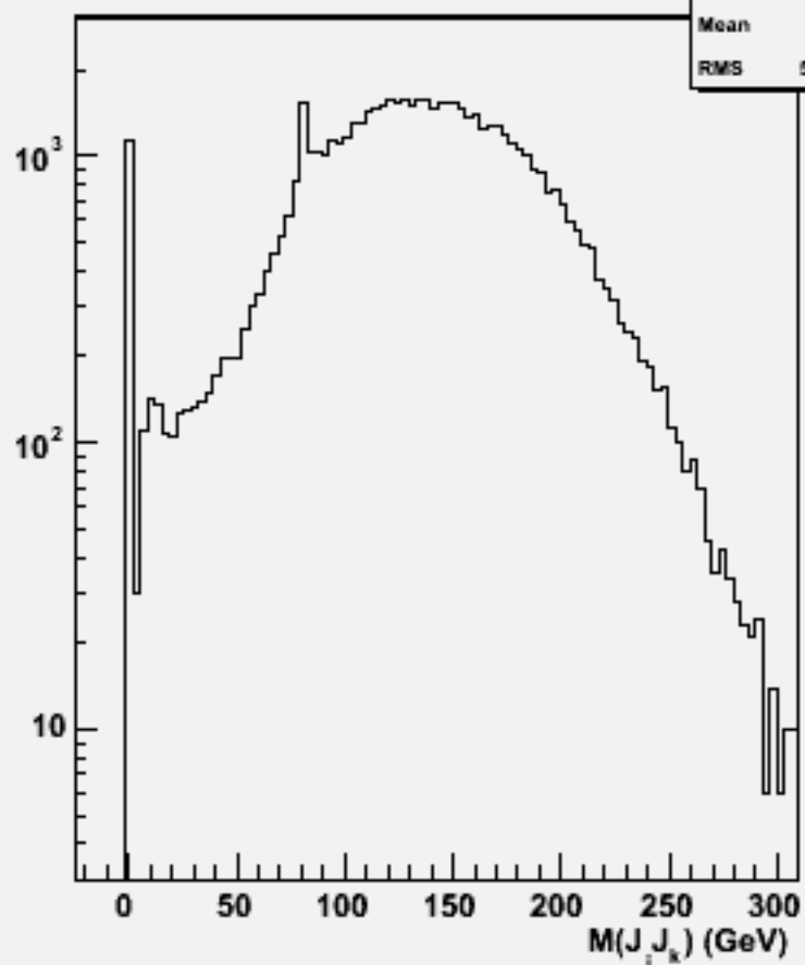
2jets mass(All comb)w101773 ccudsc_o
