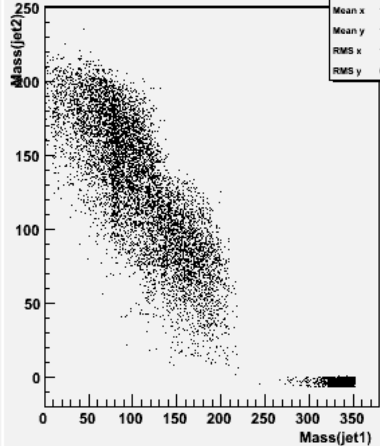
Jet mass for forced 2-jets : w101773 ccudsc_o
