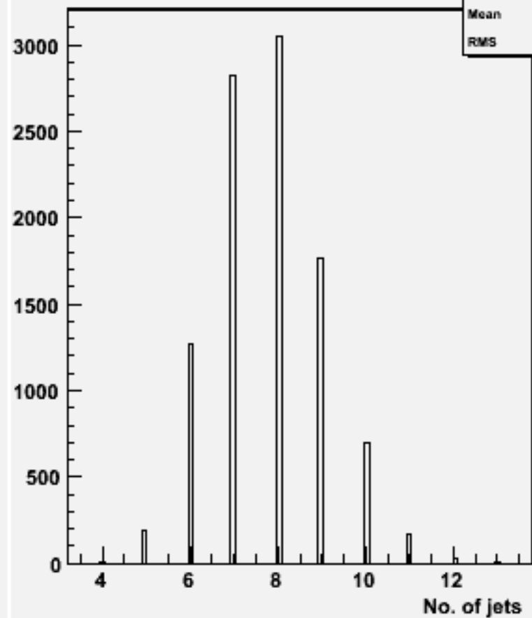
No. jets (ycut=0.001) : w101773 ccudsc_o
