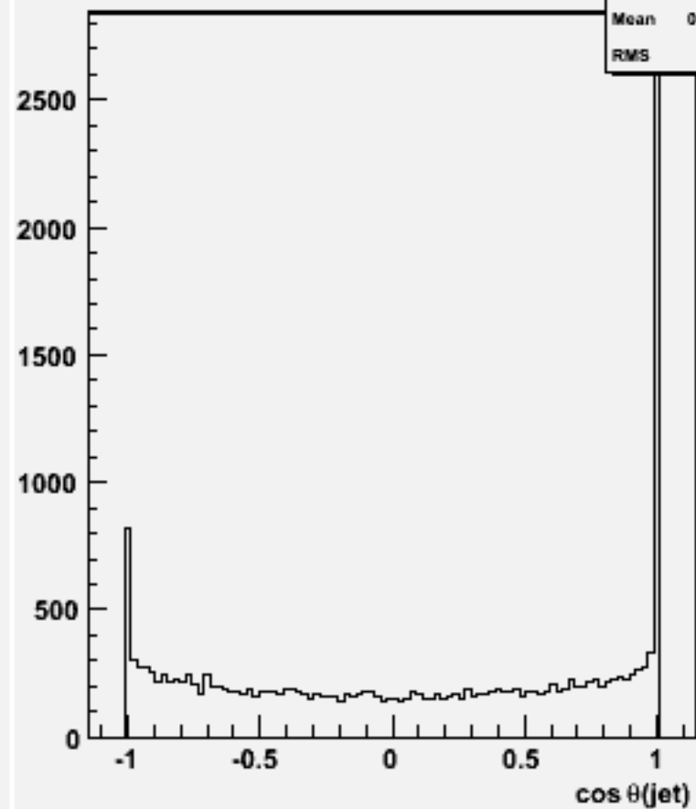
cos \theta for 2-jets :w101773 ccudsc_o
