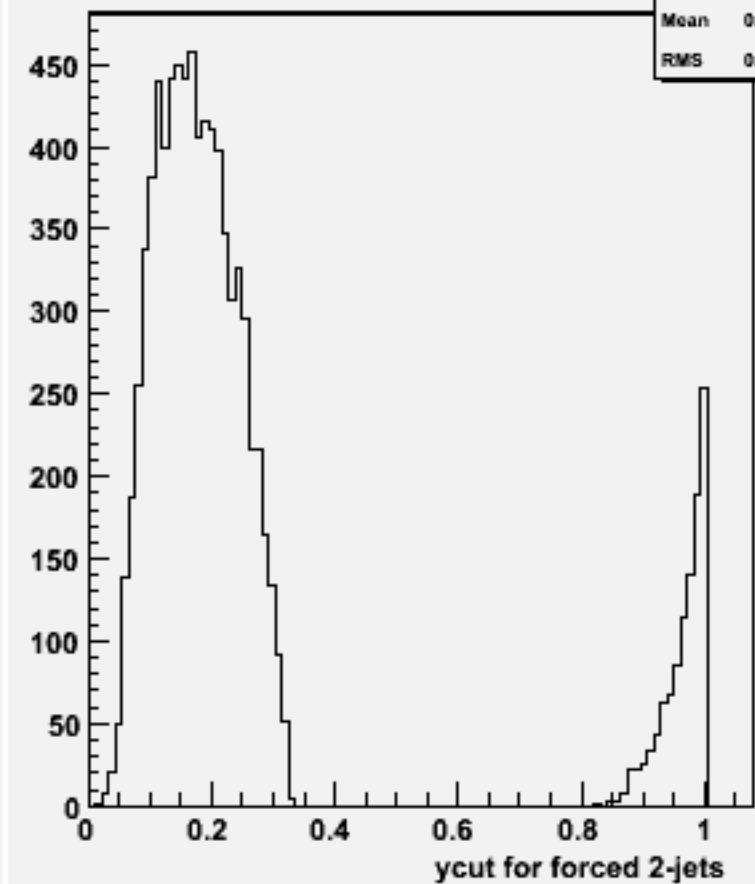
Ycut for 2-jets :w101773 ccudsc_o
