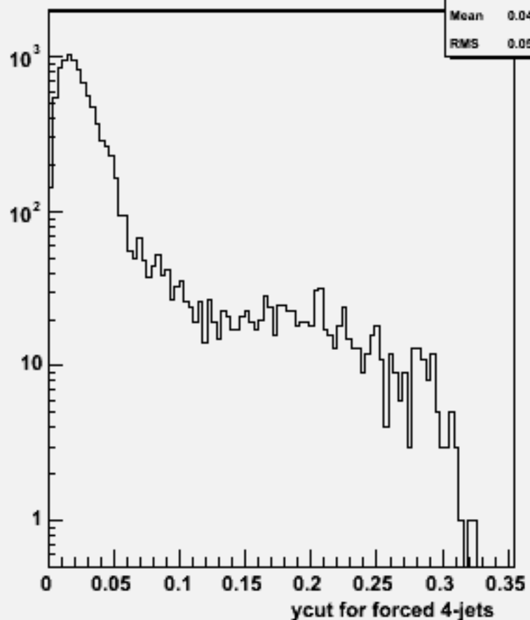
Ycut for 4-jets :w101773 ccudsc_o
