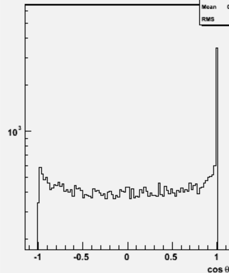
Jet cos \theta (All jets)w101773 ccudsc_o
