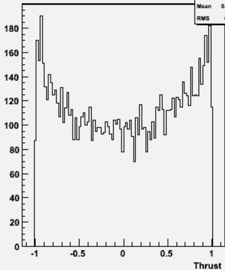
cos \Theta (thrust) w101773 ccudsc_o
