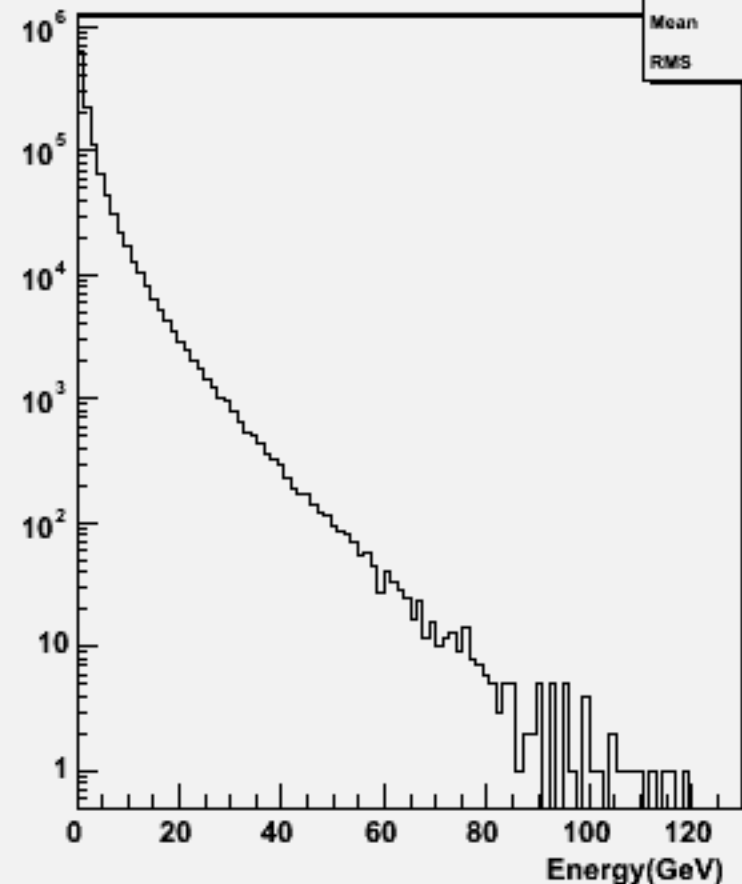
Particle Energy : w101773 ccudsc_o
