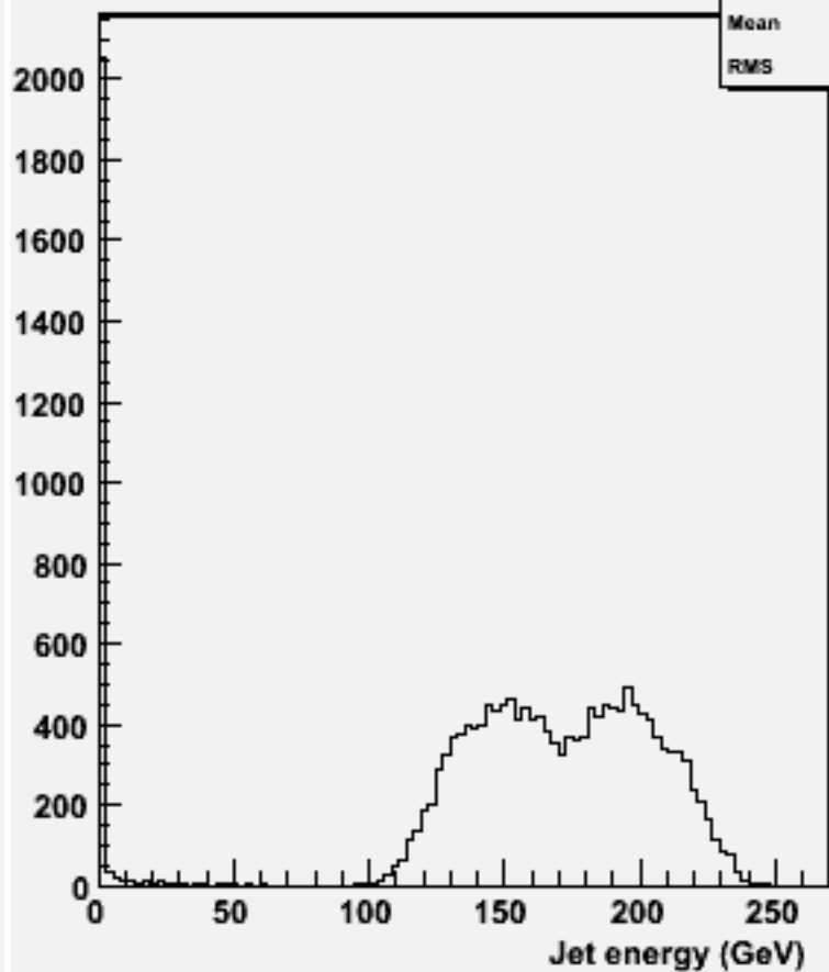
energy for 2-jets :w101773 ccudsc_o
