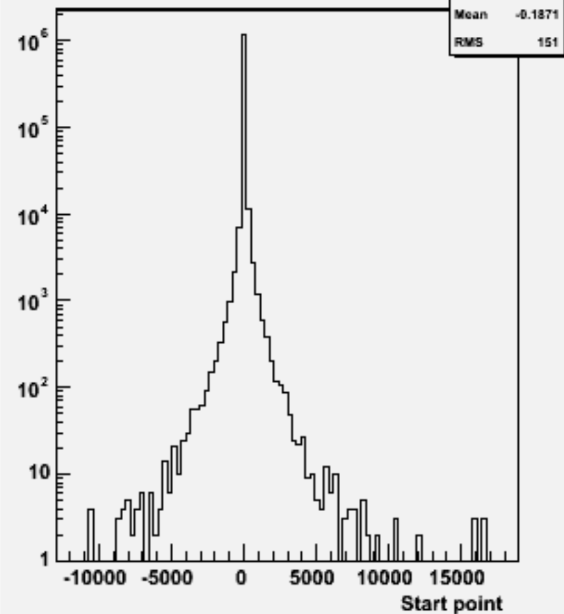
Start point Z : w101769 ccuddu_o
