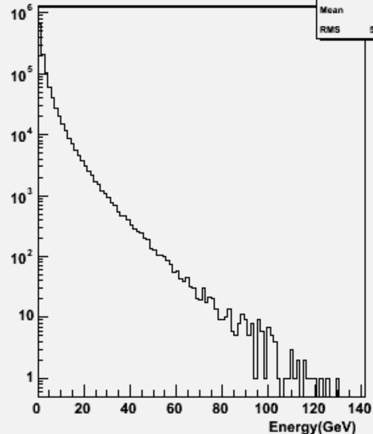
Particle Energy : w101769 ccuddu_o
