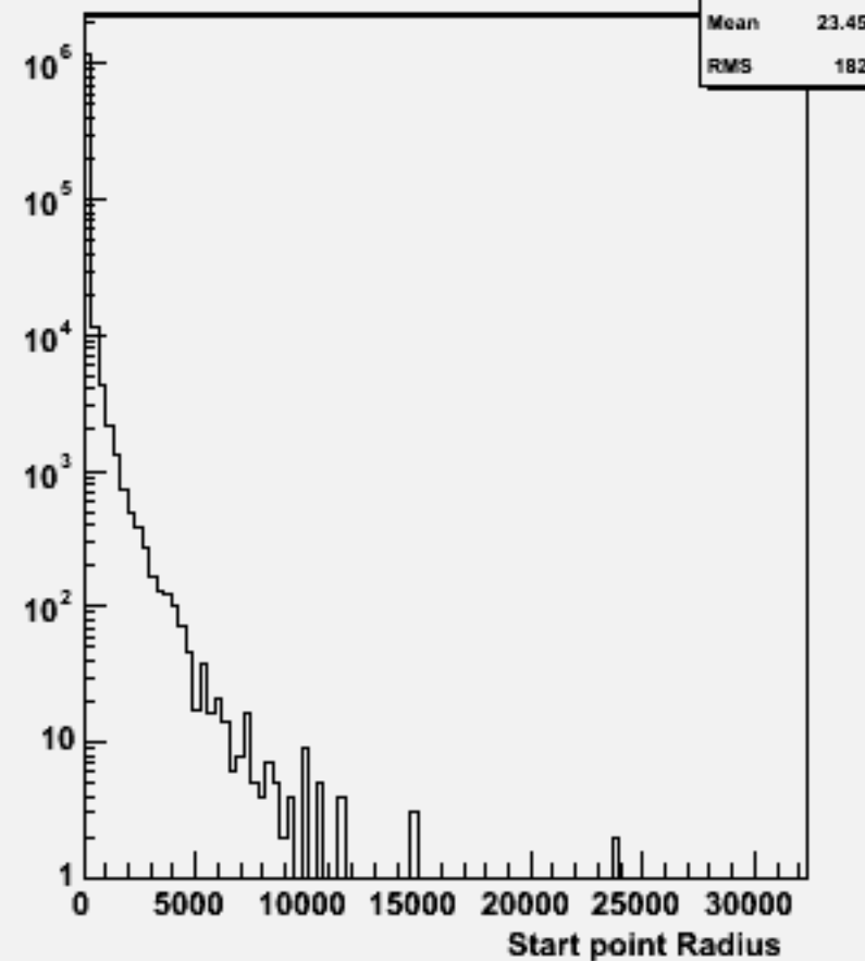
Start point R : w101769 ccuddu_o
