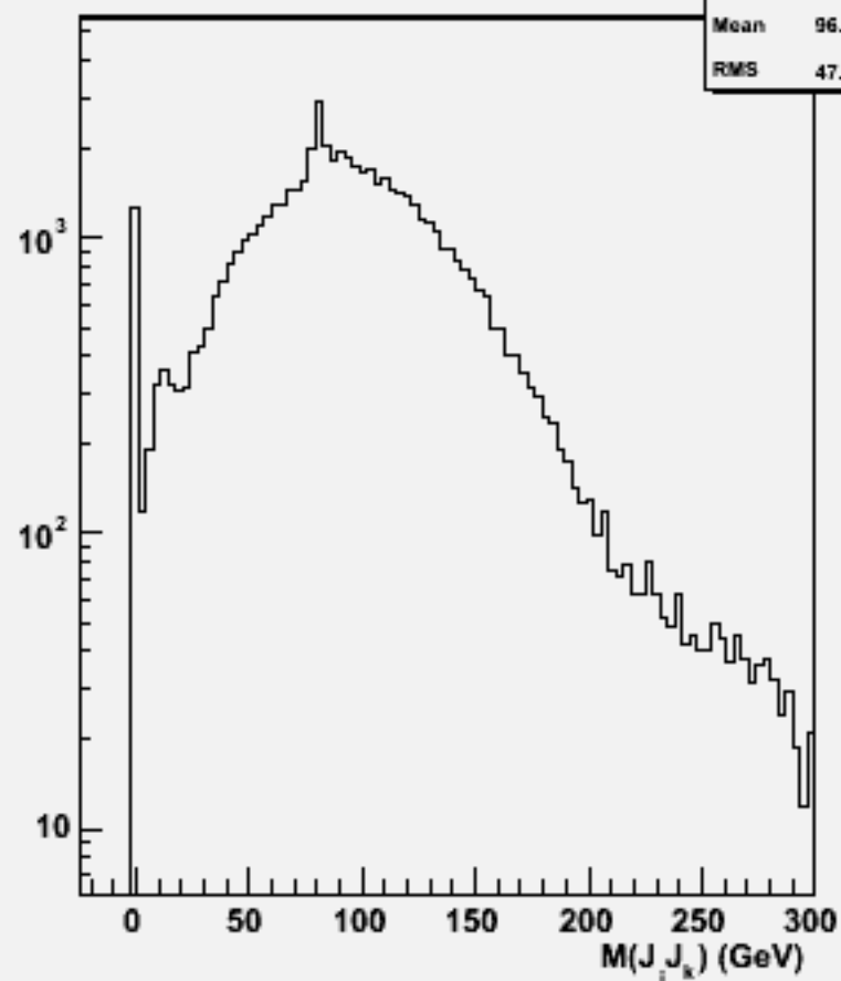
2jets mass(All comb)w101765 ccude3n3_o
