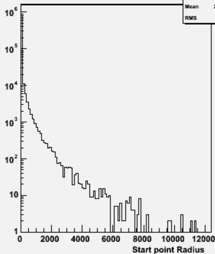
Start point R : w101765 ccude3n3_o
