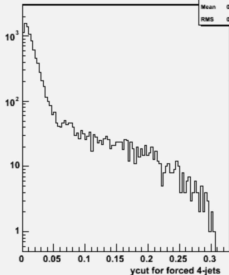
Ycut for 4-jets :w101765 ccude3n3_o
