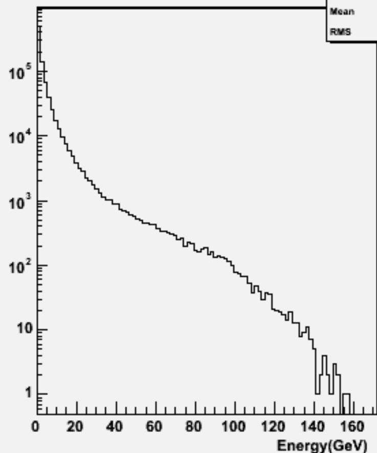
Particle Energy : w101765 ccude3n3_o
