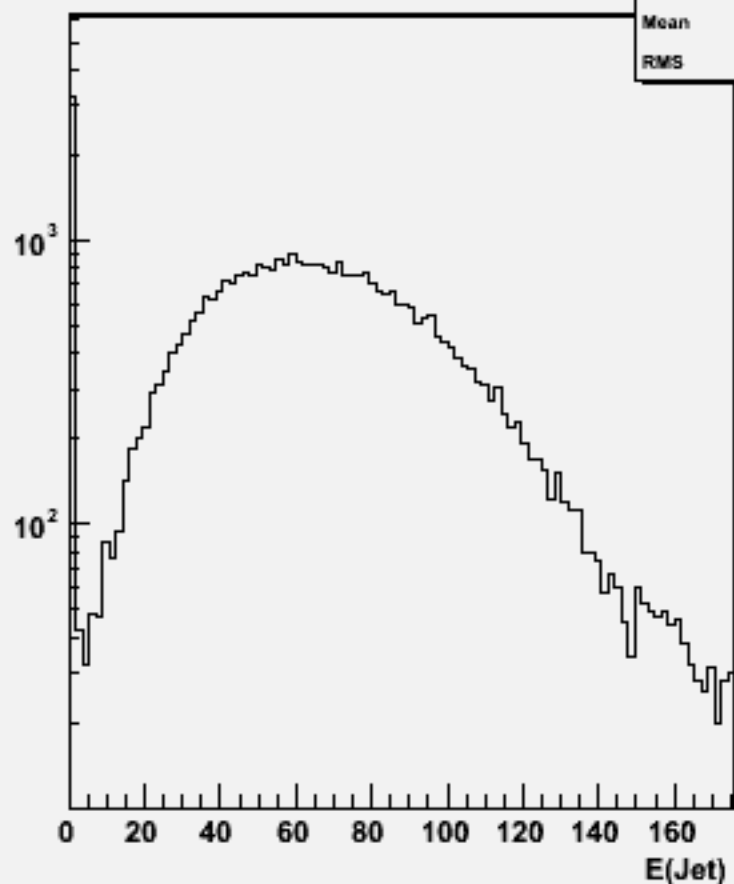
Jet energies(All jets)w101765 ccude3n3_o
