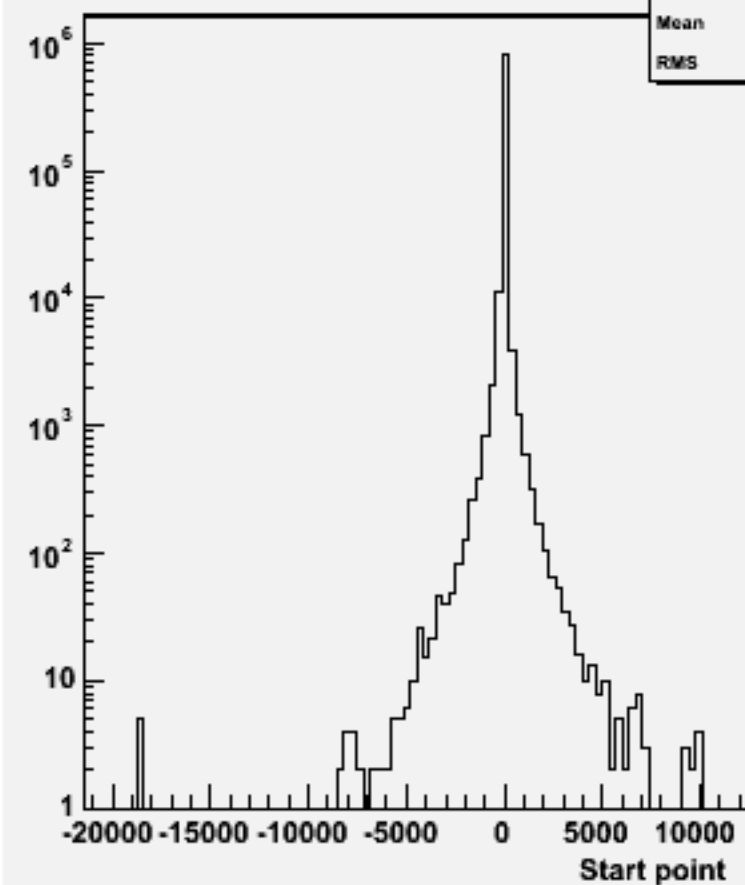
Start point Z : w101765 ccude3n3_o
