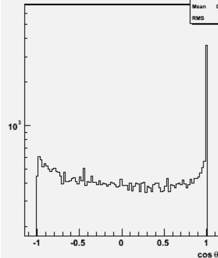
Jet cosθ (All jets)w101765 ccude3n3_o
