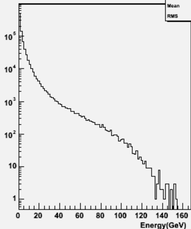
Particle Energy : w101764 ccude3n3_o
