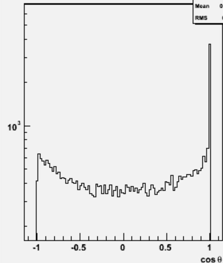
Jet cos \theta (All jets)w101764 ccude3n3_o
