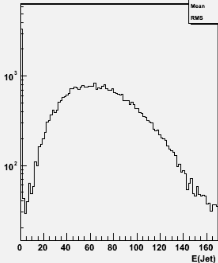
Jet energies(All jets)w101764 ccude3n3_o
