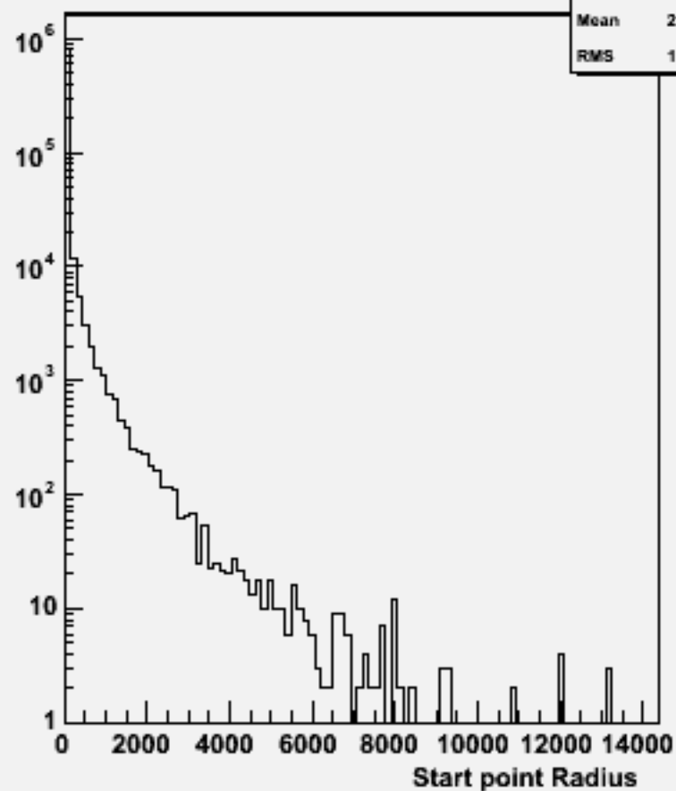
Start point R : w101764 ccude3n3_o
