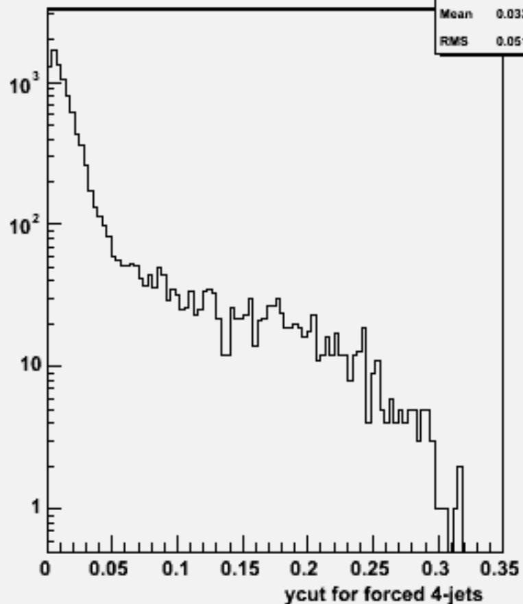
Ycut for 4-jets :w101764 ccude3n3_o
