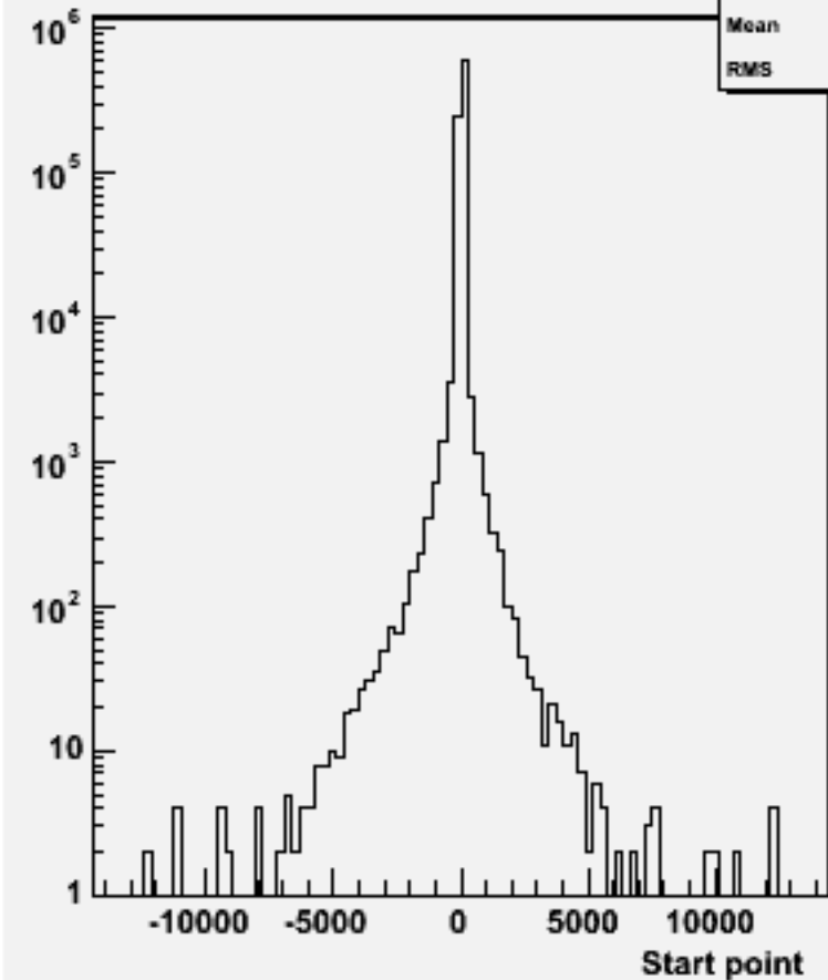
Start point Z : w101764 ccude3n3_o
