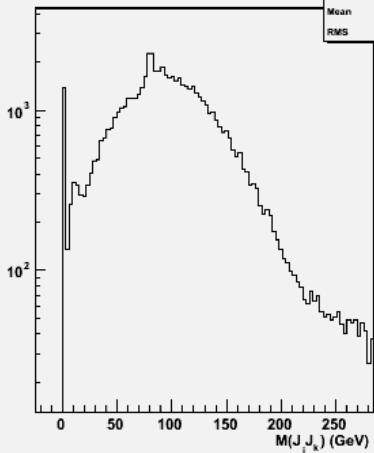
2jets mass(All comb)w101764 ccude3n3_o
