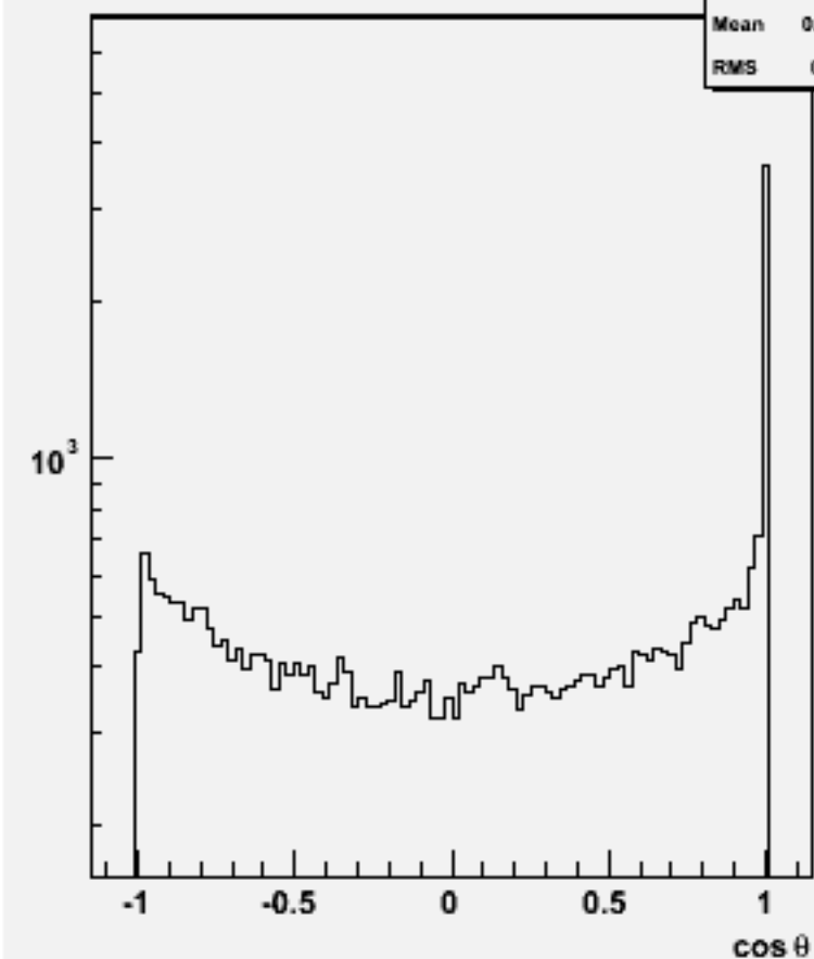
Jet cosθ (All jets)w101760 ccude2n2_o
