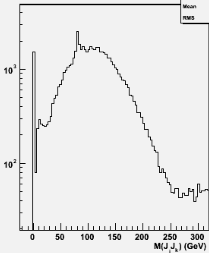
2jets mass(All comb)w101760 ccude2n2_o
