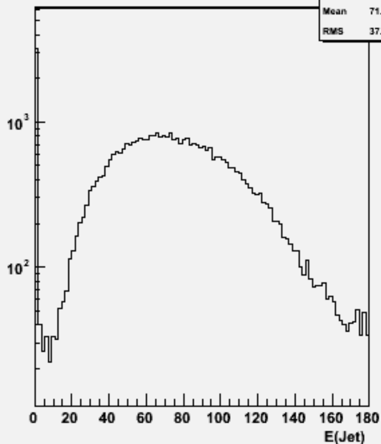
Jet energies(All jets)w101760 ccude2n2_o
