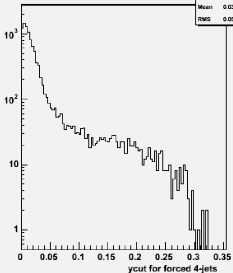
Ycut for 4-jets :w101760 ccude2n2_o
