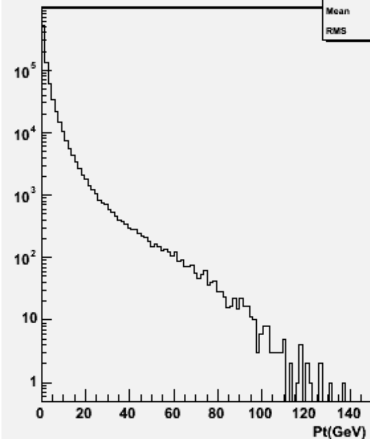
Particle Pt : w101758 ccude1n1_o
