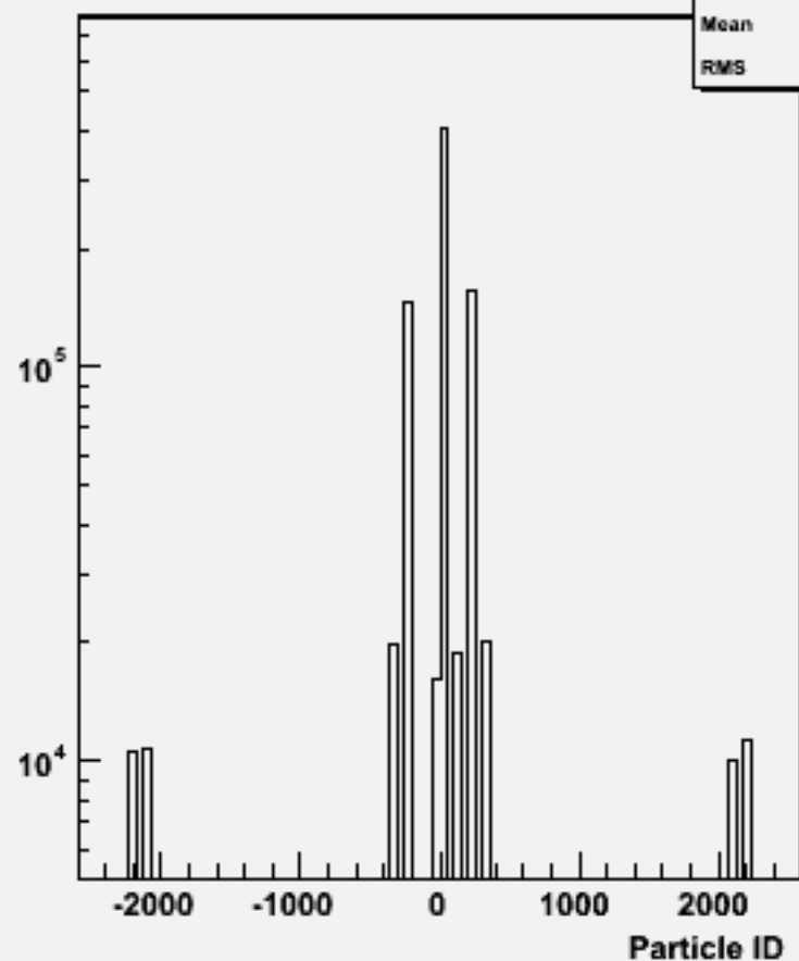
Particle ID : w101758 ccude1n1_o
