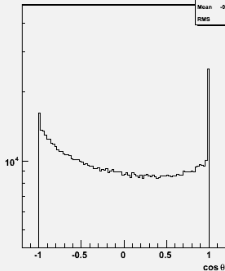
Particle cos \theta : w101758 ccude1n1_o
