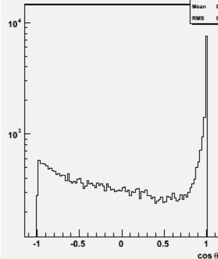
Jet cos \theta (All jets)w101758 ccude1n1_o
