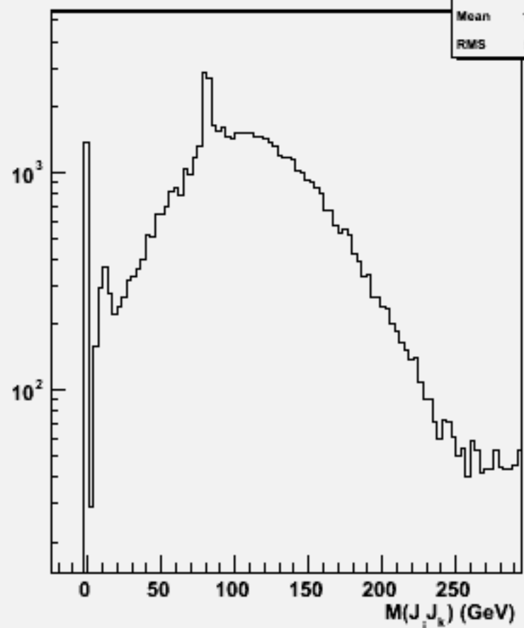
2jets mass(All comb)w101758 ccude1n1_o
