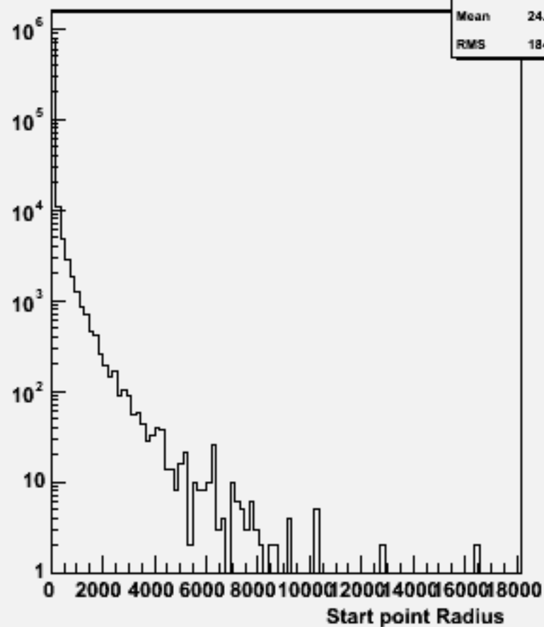
Start point R : w101758 ccude1n1_o
