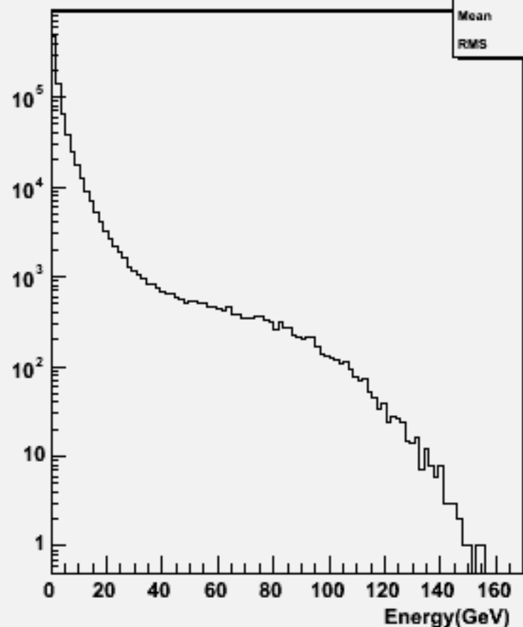
Particle Energy : w101758 ccude1n1_o
