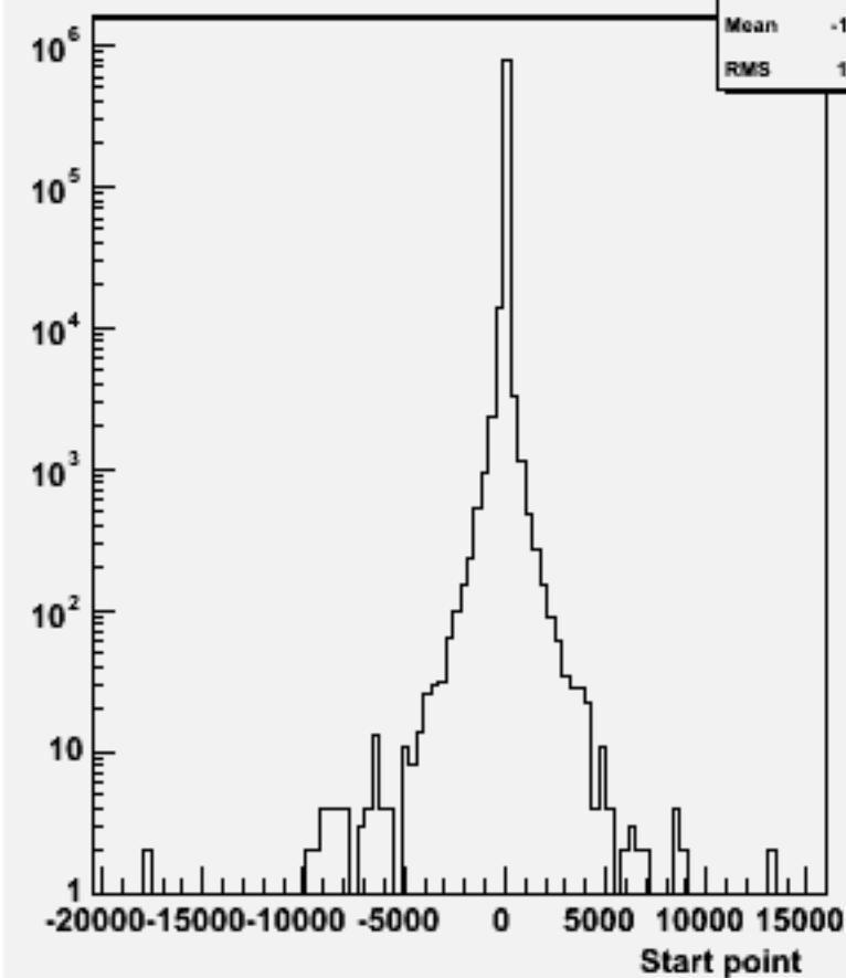
Start point Z : w101758 ccude1n1_o
