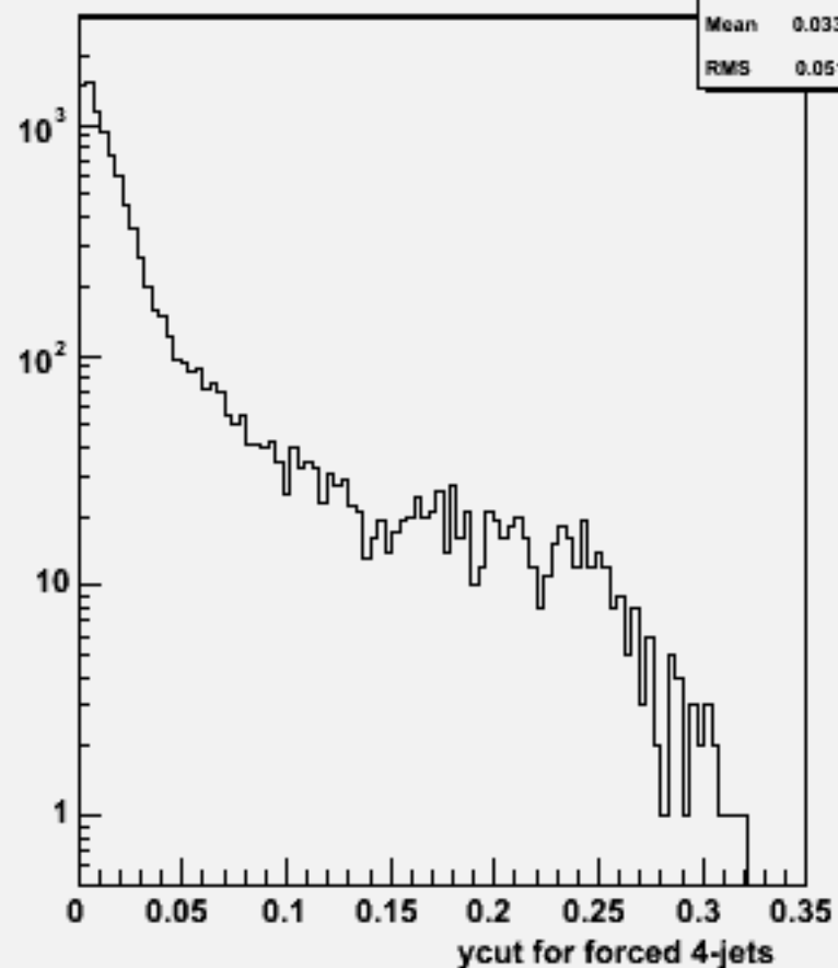
Ycut for 4-jets :w101758 ccude1n1_o
