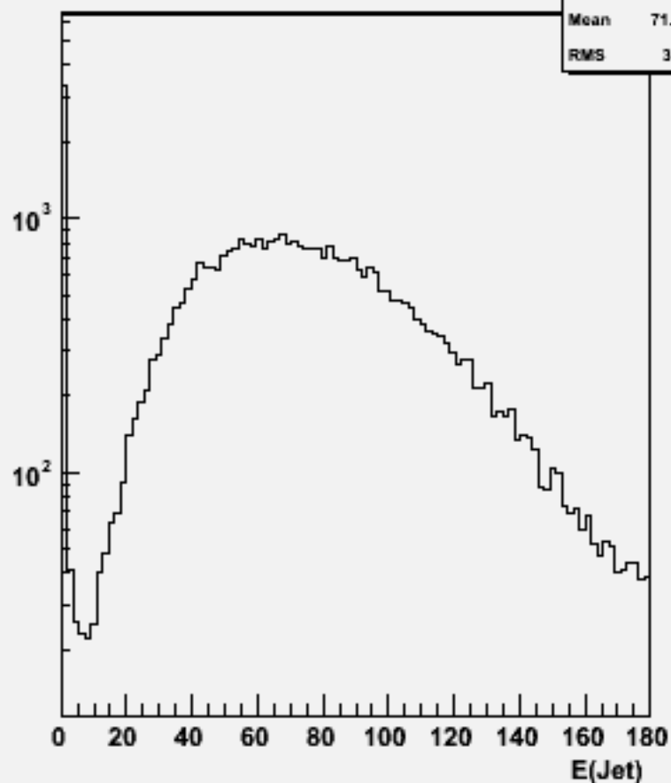
Jet energies(All jets)w101758 ccude1n1_o
