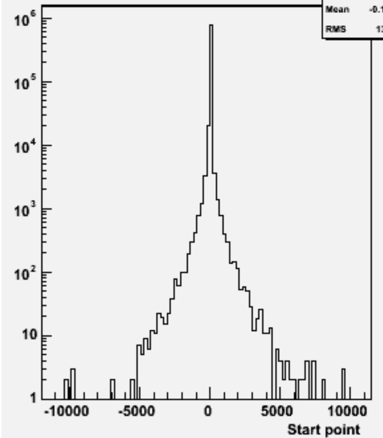
Start point Z : w101757 ccude1n1_o
