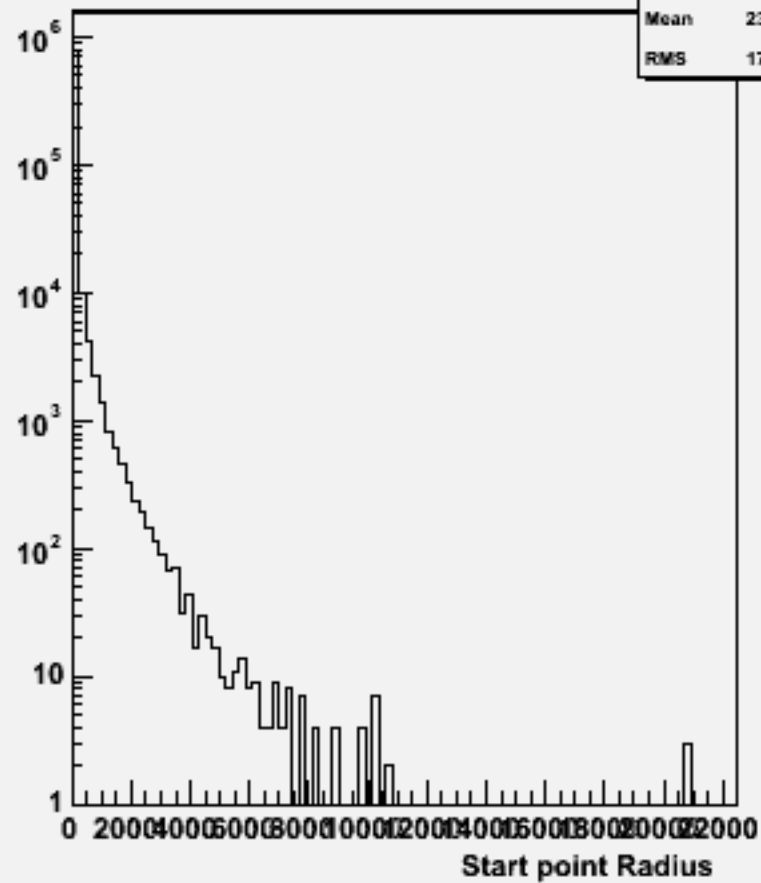
Start point R : w101757 ccude1n1_o
