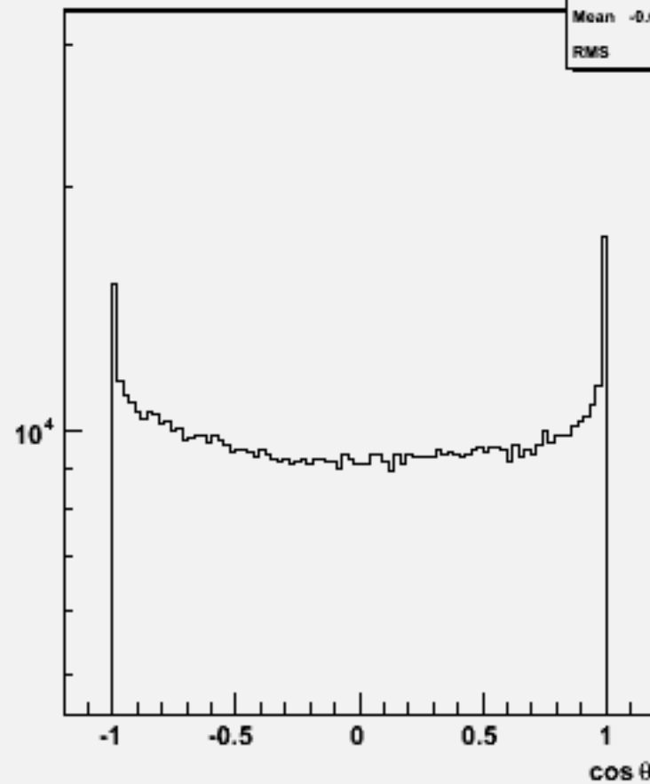
Particle cos \theta : w101757 ccude1n1_o
