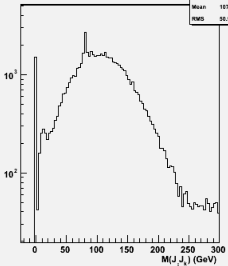
2jets mass(All comb)w101757 ccude1n1_o
