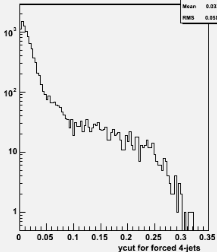
Ycut for 4-jets :w101757 ccude1n1_o
