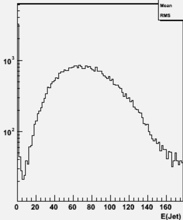
Jet energies(All jets)w101757 ccude1n1_o
