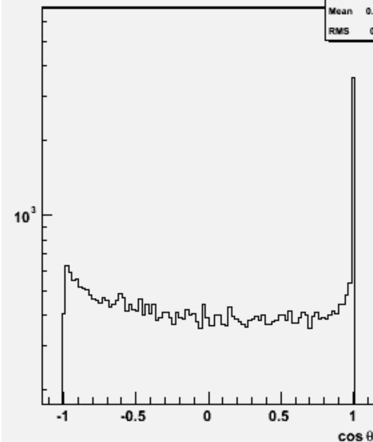
Jet cos \theta (All jets)w101757 ccude1n1_o
